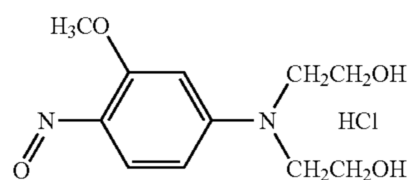
Nitrosoaniline Derivative (31.1144)
