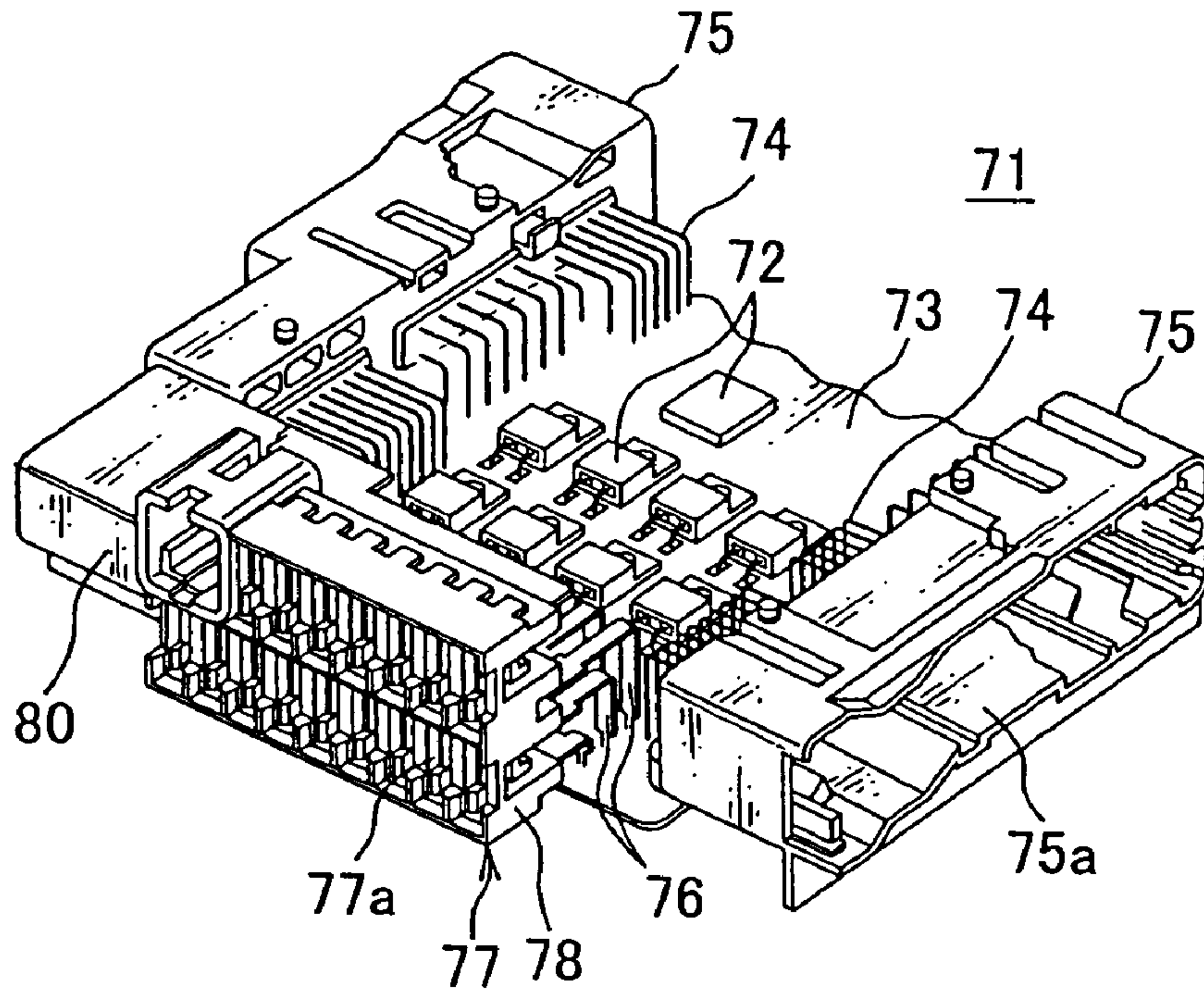
FIG. 8 PRIOR ART
