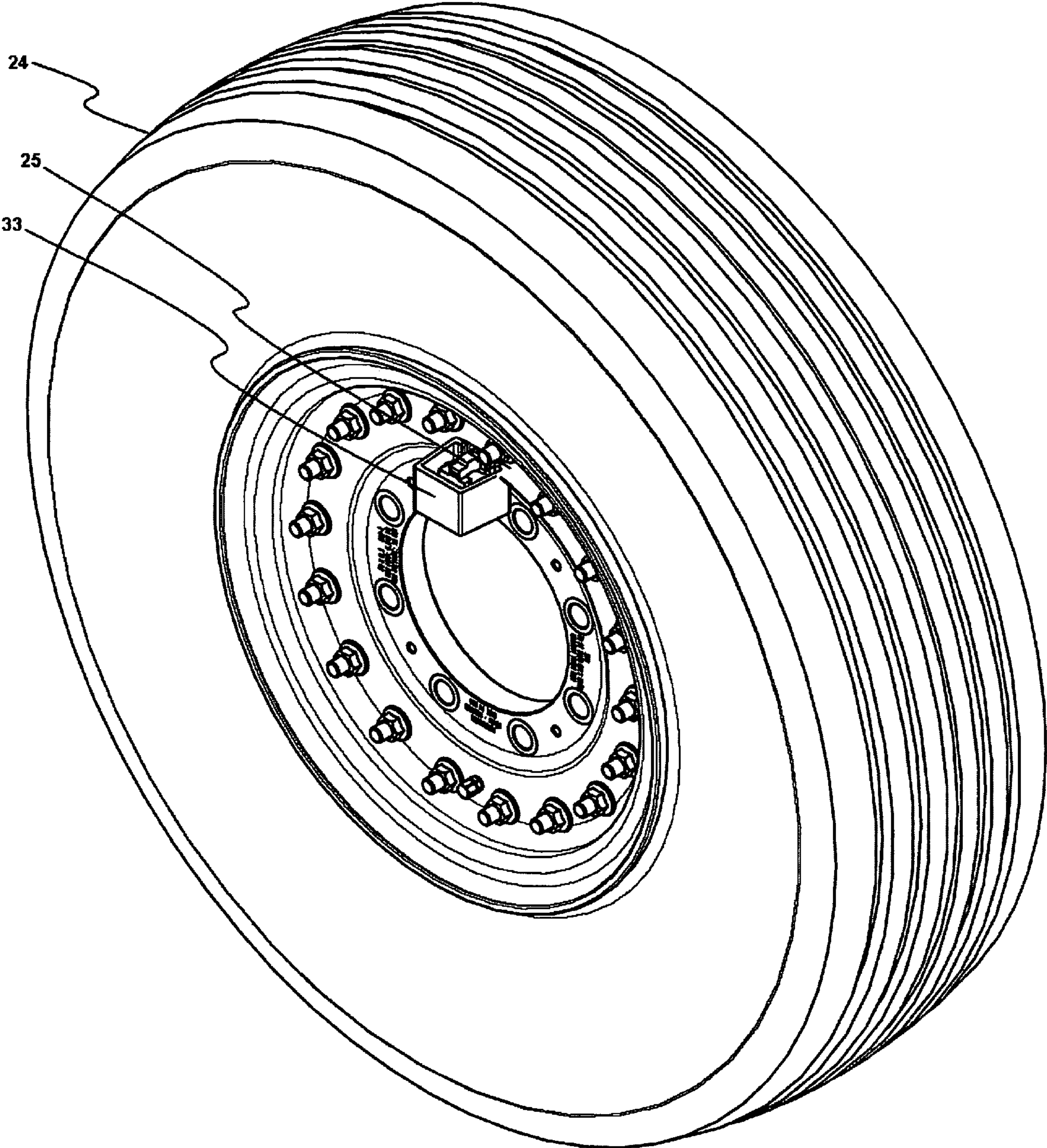
FIG. 4 (PRIOR ART)
