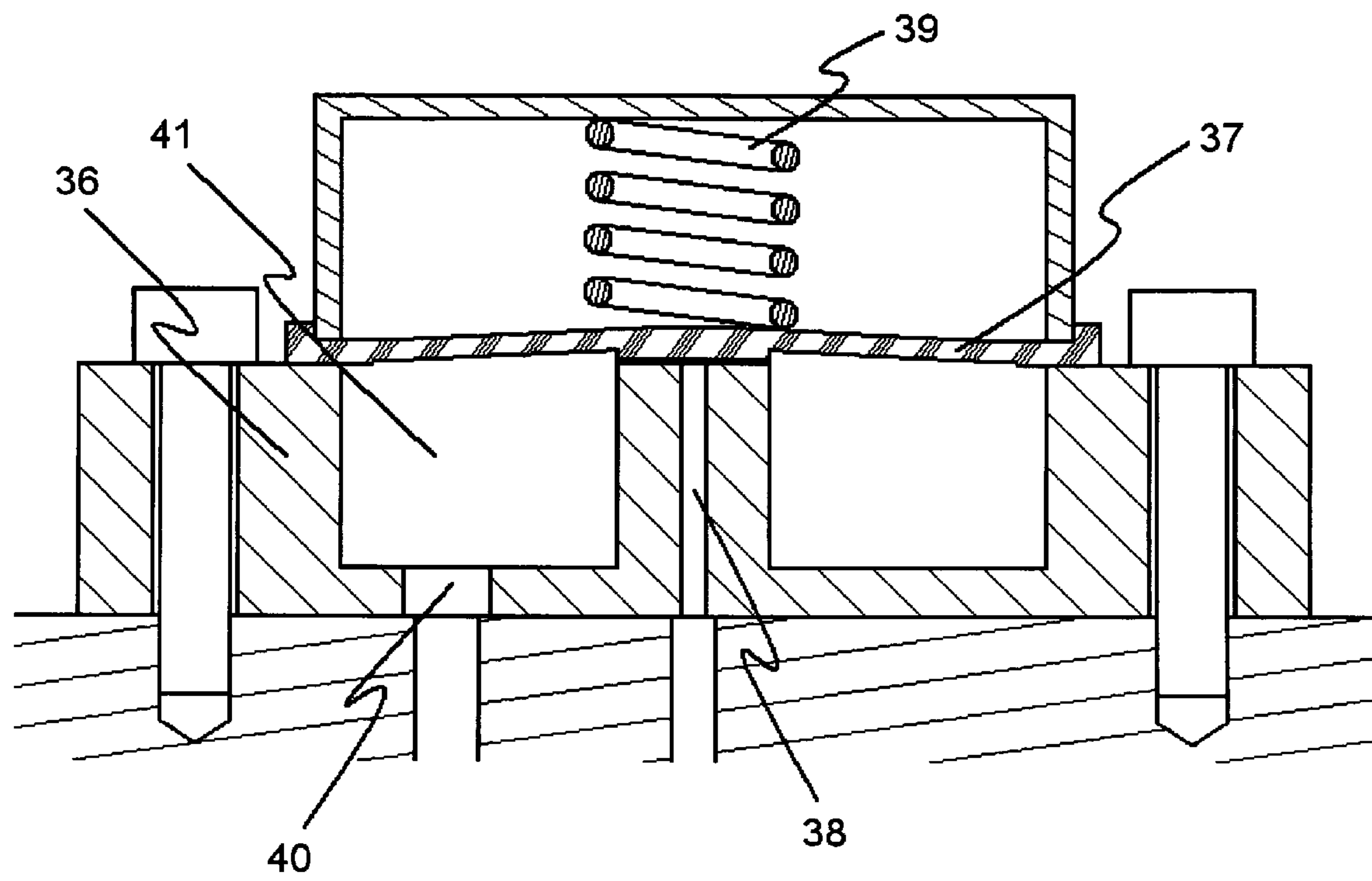
FIG. 6 (PRIOR ART)
