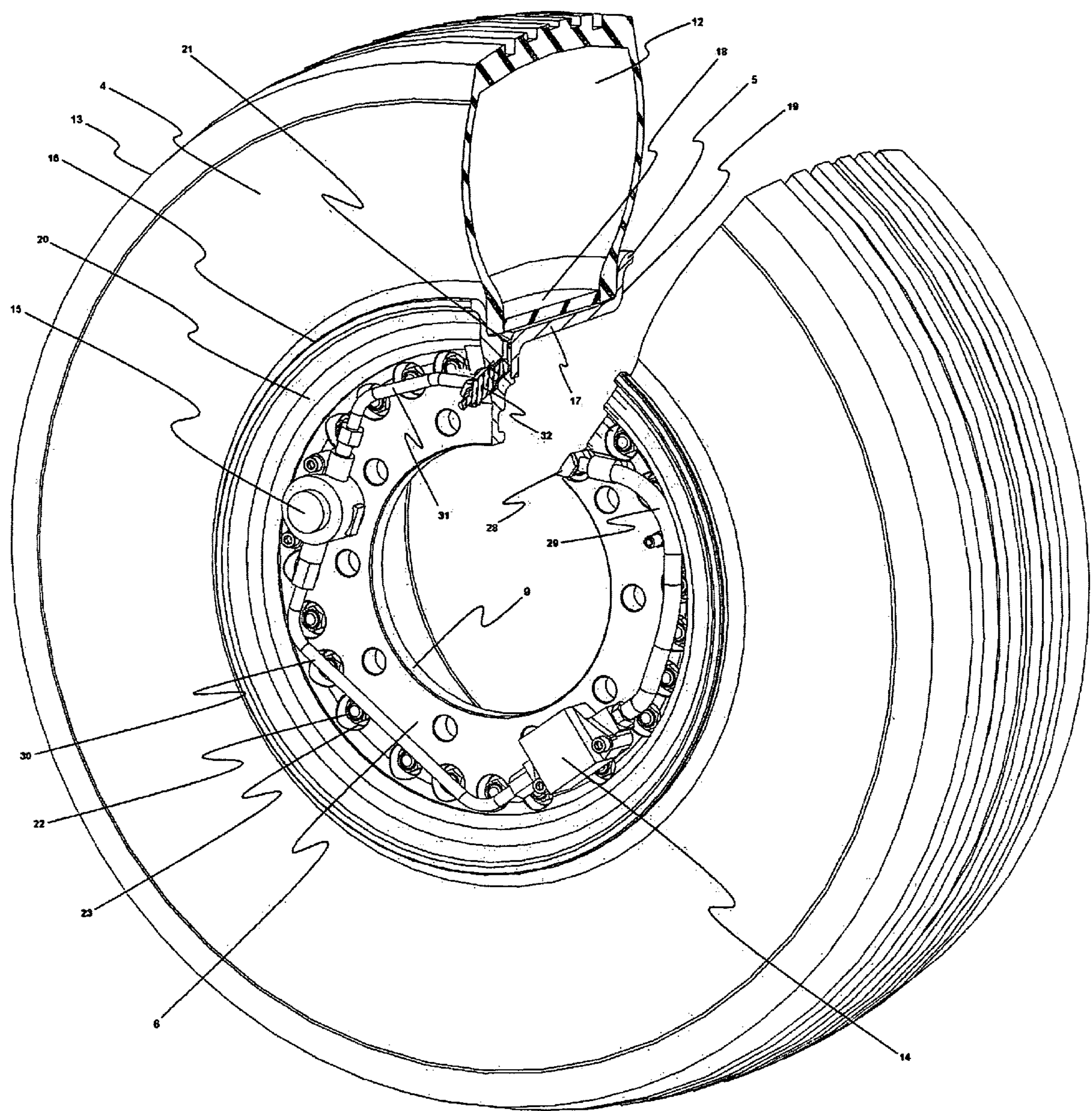
FIG. 2 (PRIOR ART)
