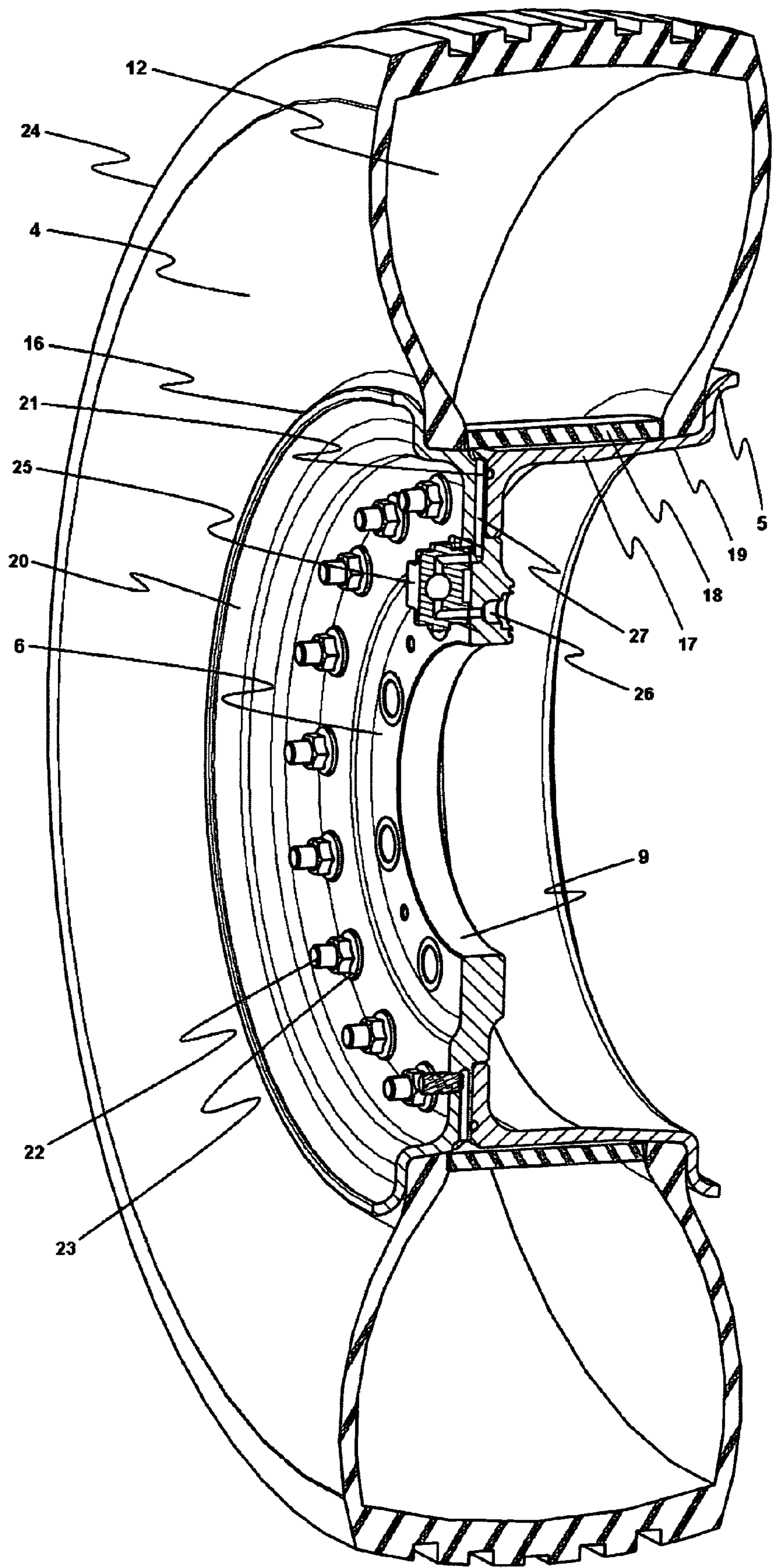
FIG. 3 (PRIOR ART)
