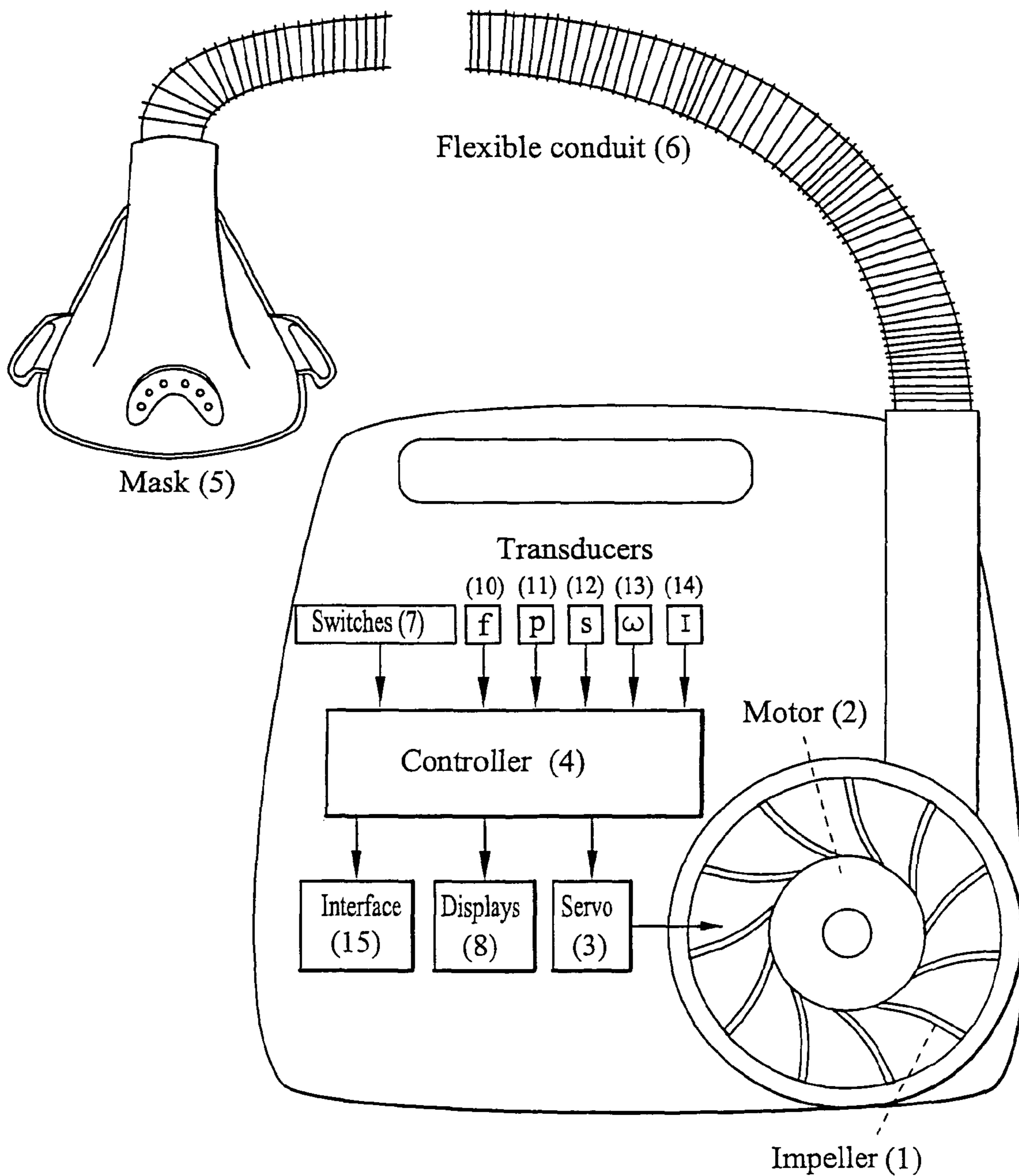
Figure 2: CPAP apparatus
