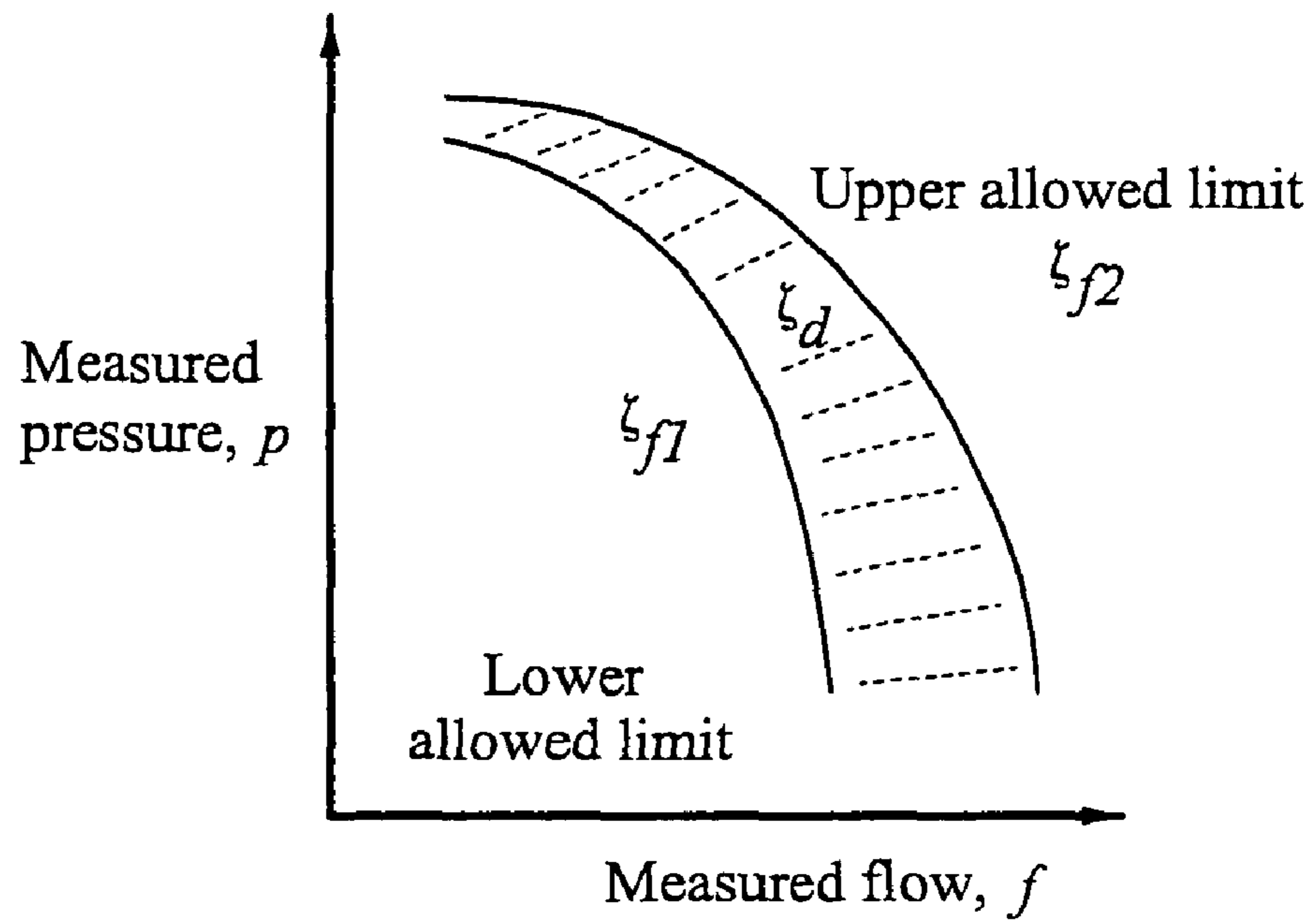
Figure 3a: High motor speed ( \omega ) operation
