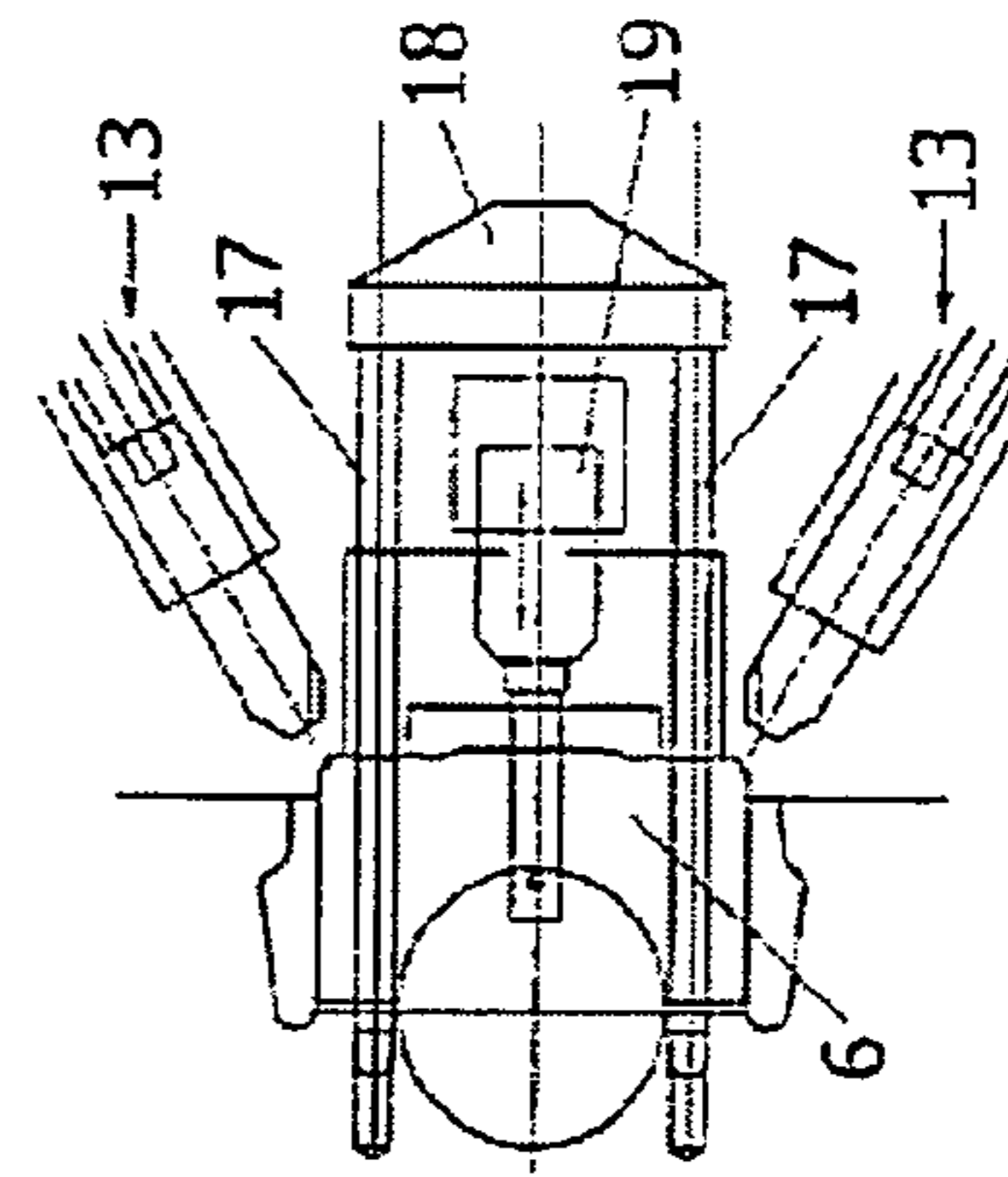
Fig. 3e Retracting auxiliary support Carrying out vibrating and impacting function
