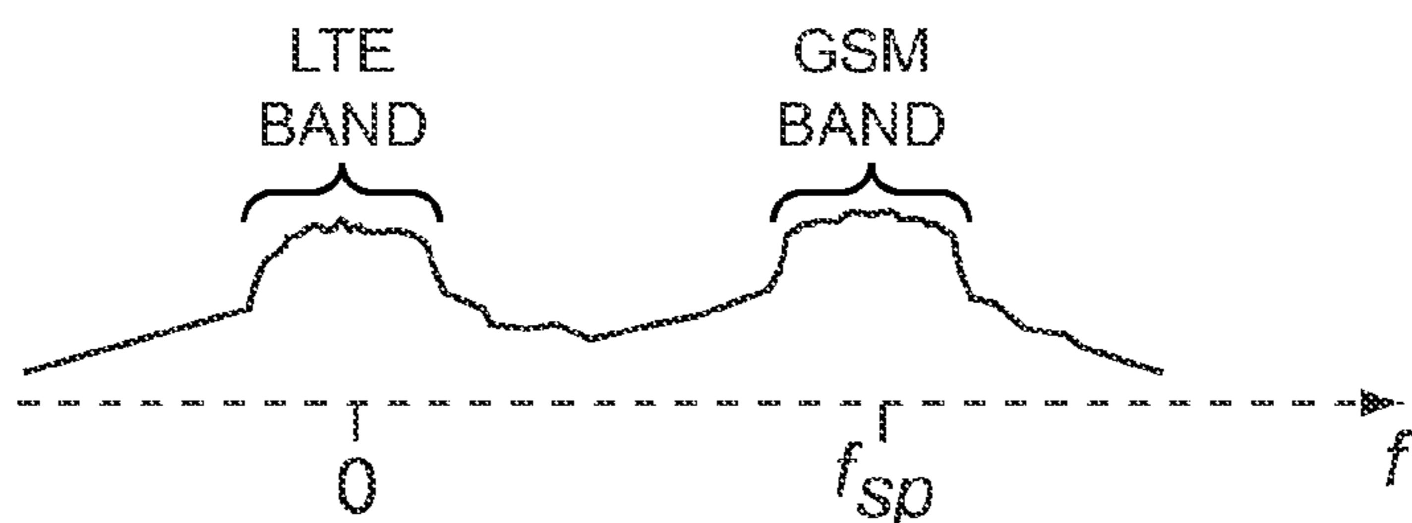
SPECTRUM OF PEAKS SIGNAL (C)
