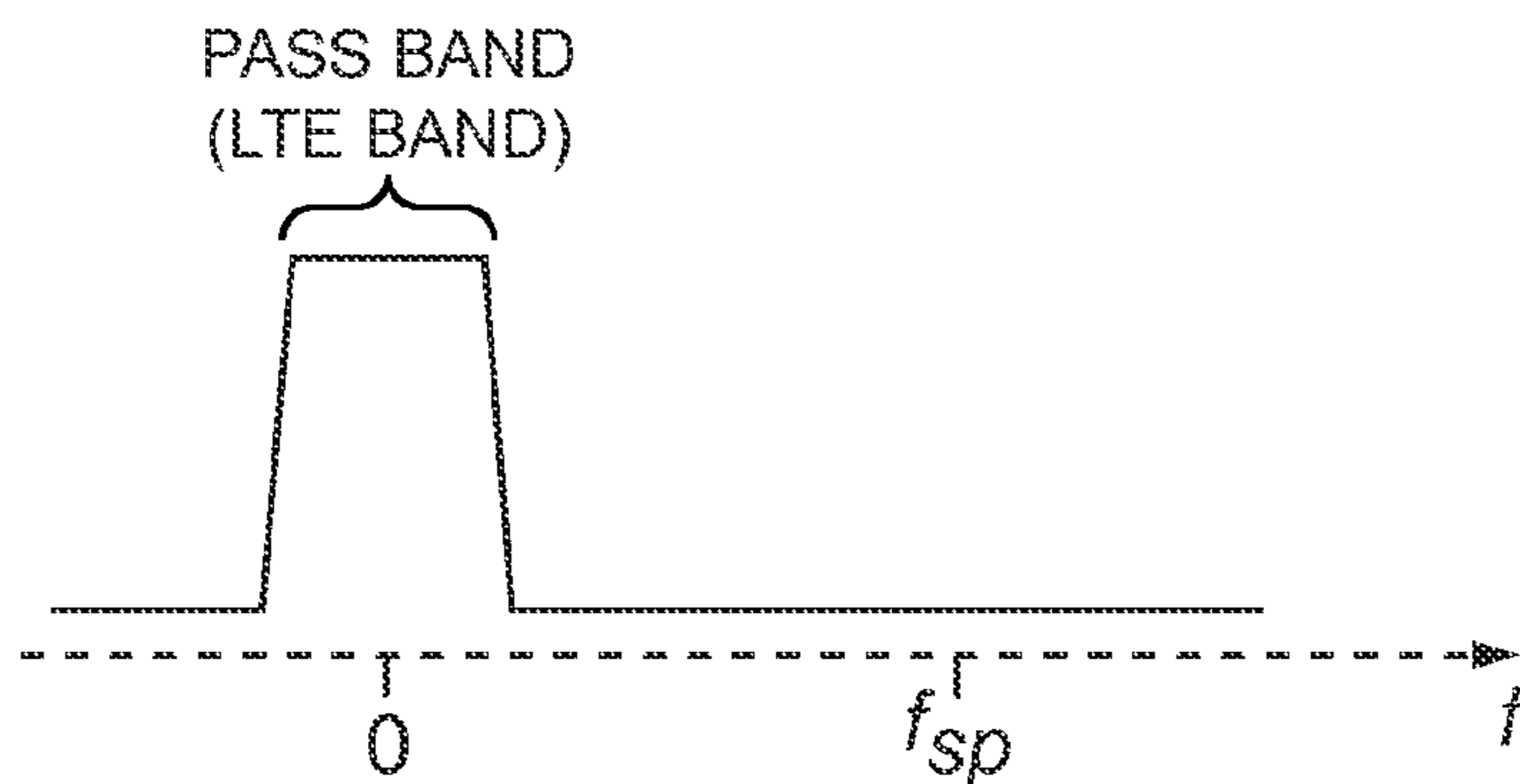
TRANSFER FUNCTION OF DISTORTION SELECTION FILTER
