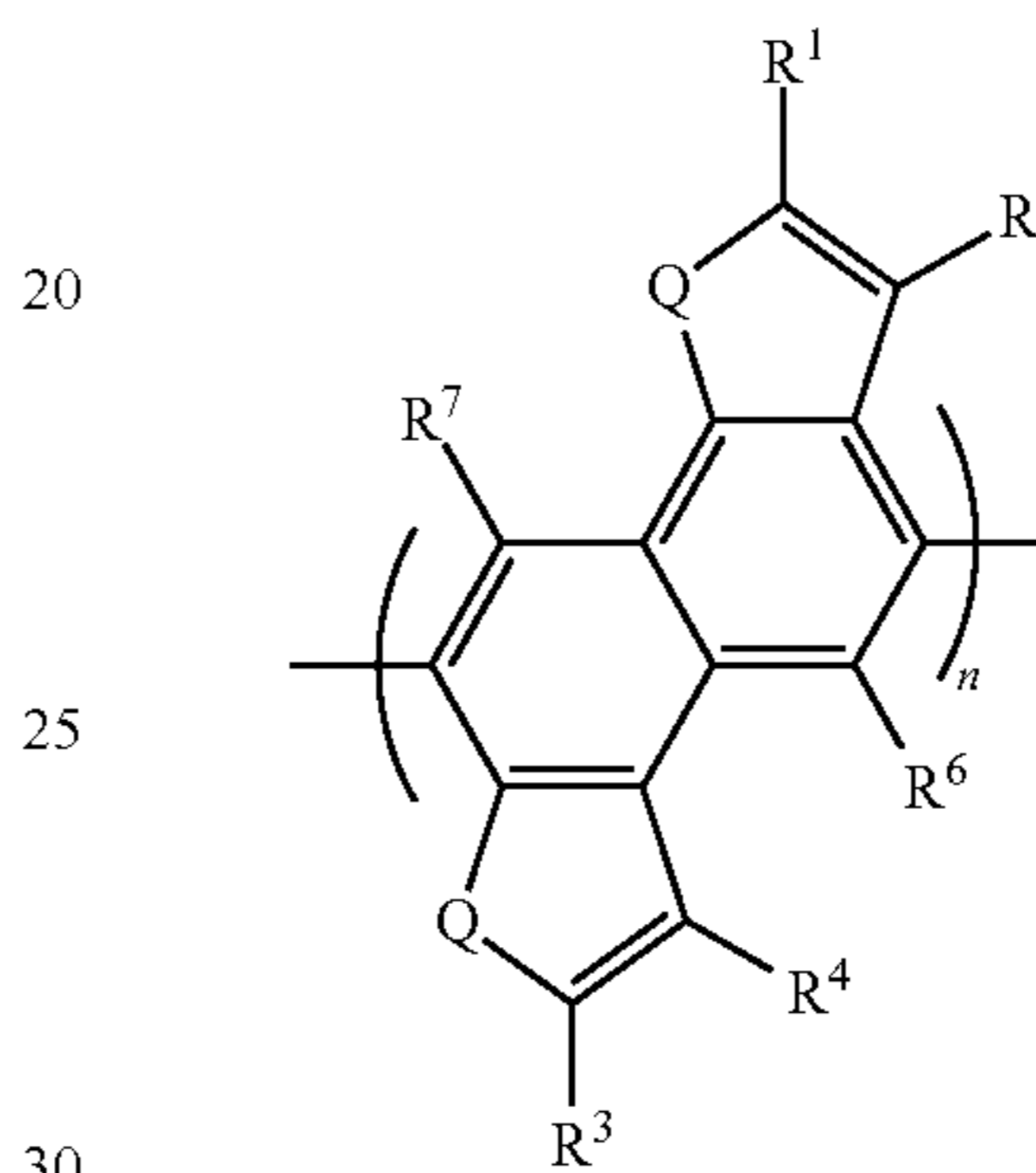
Compound 3
