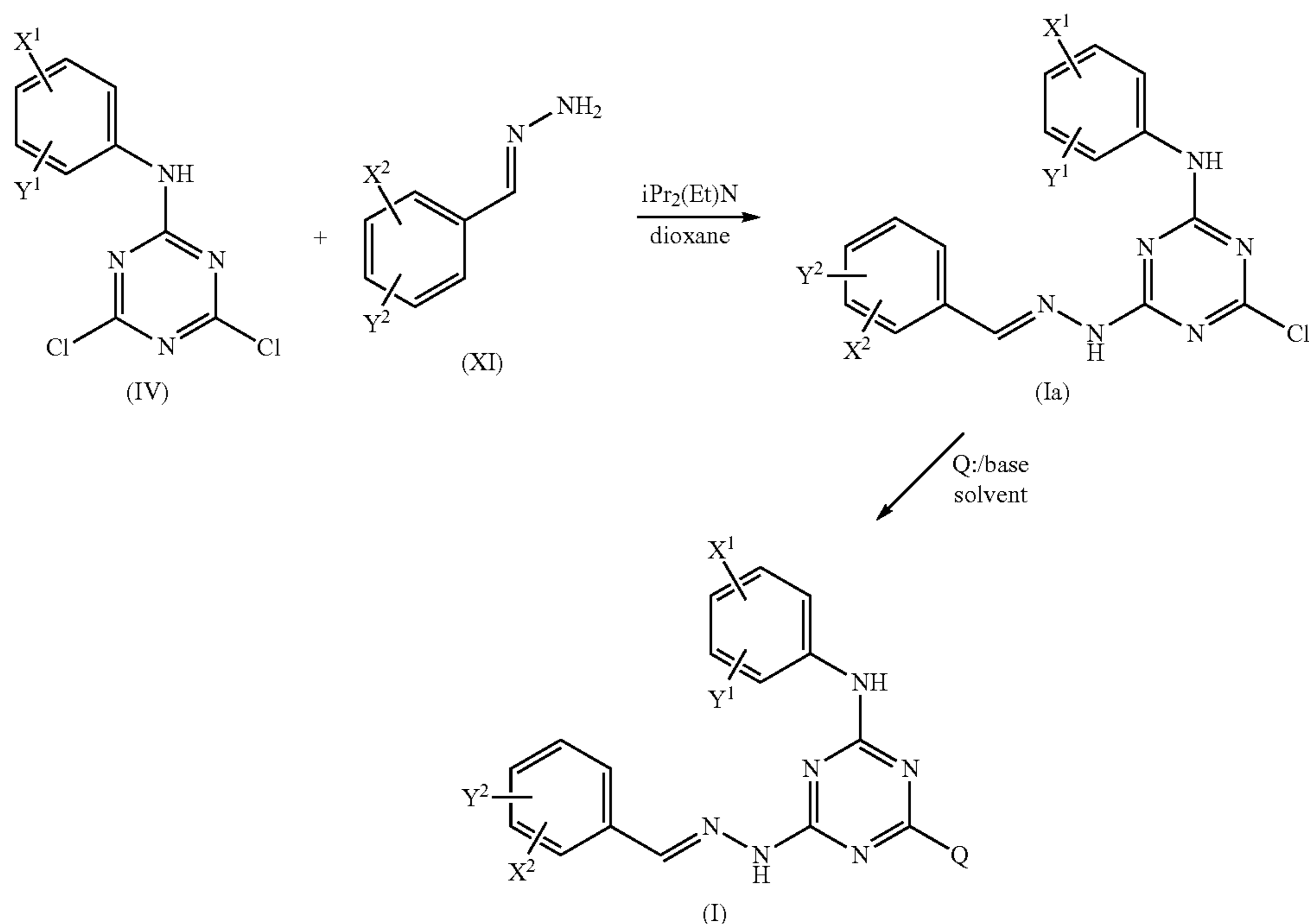
Scheme F
