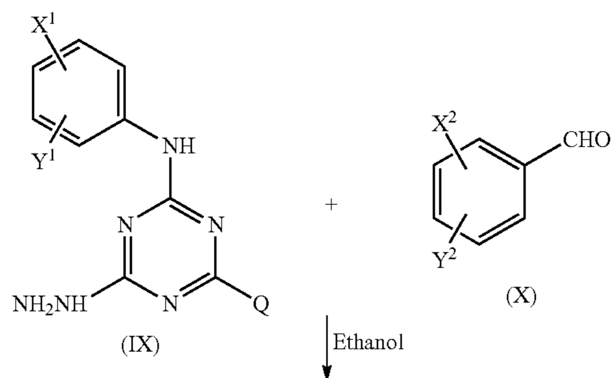
Scheme E
