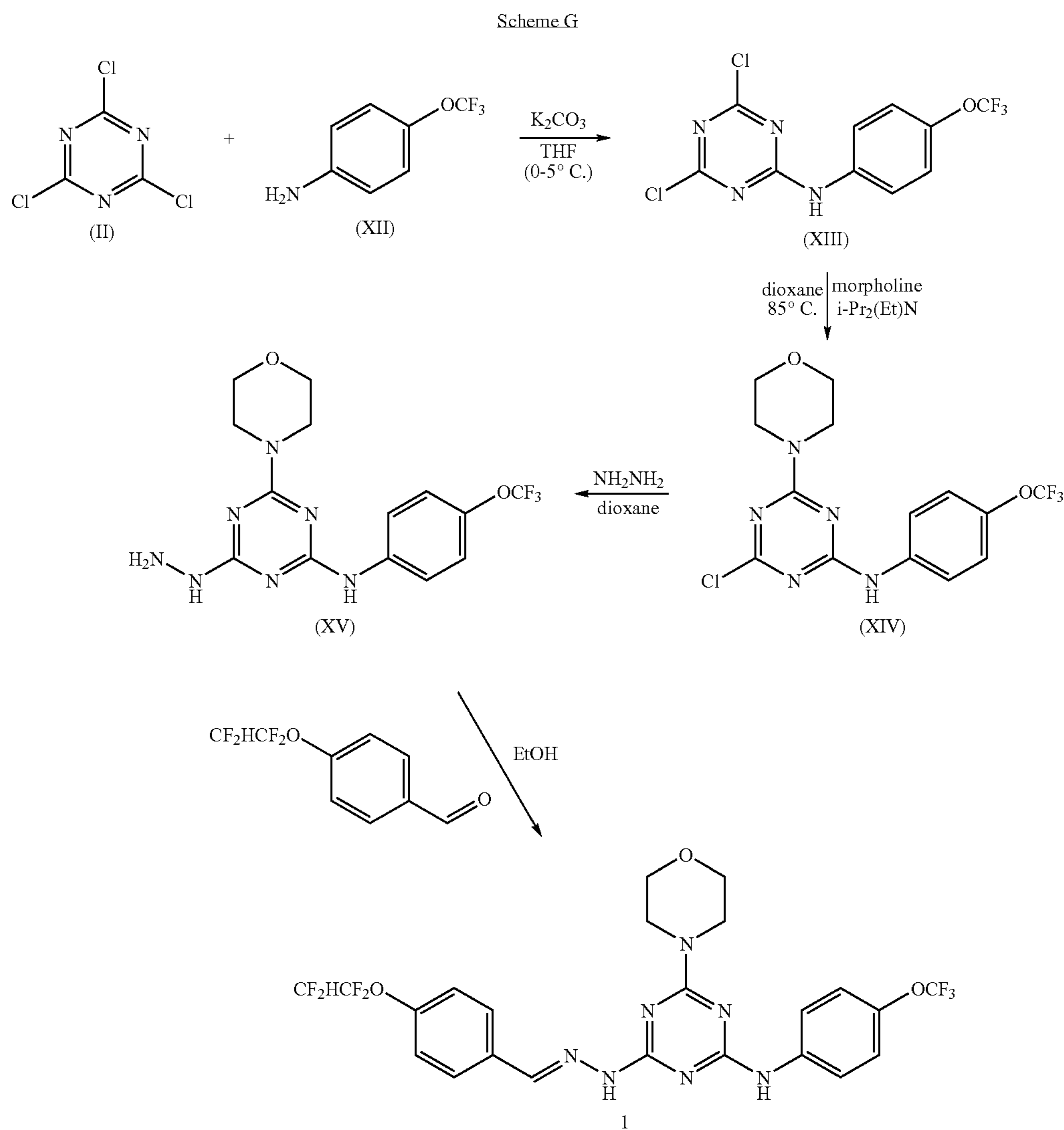
(4,6-Dichloro-1,3,5-triazin-2-yl)-(4-trifluoromethoxyphenyl)amine (XIII)
