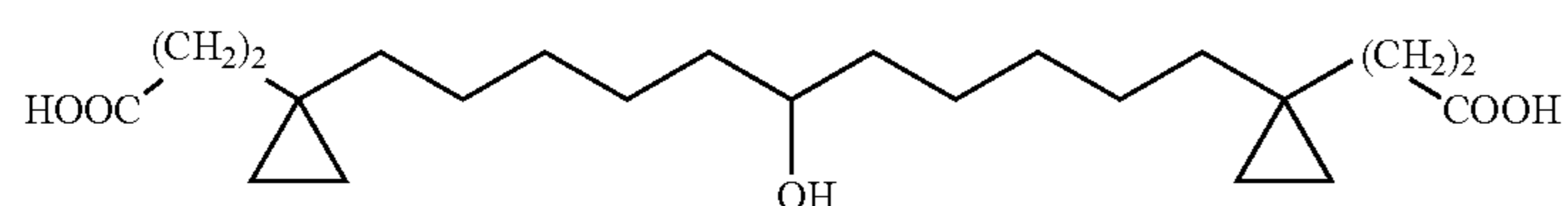
3-(1-{11-[1-(2-Carboxy-ethyl)-cyclopropyl]-6-hydroxy-undecyl}-cyclopropyl)-propionic acid
