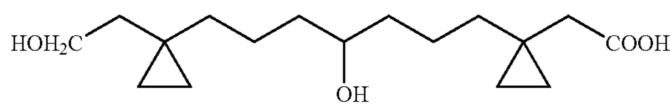
1-(4-Hydroxy-7-[1-(2-hydroxy-ethyl)-cyclopropyl]-heptyl)-cyclopropyl-acetic acid
