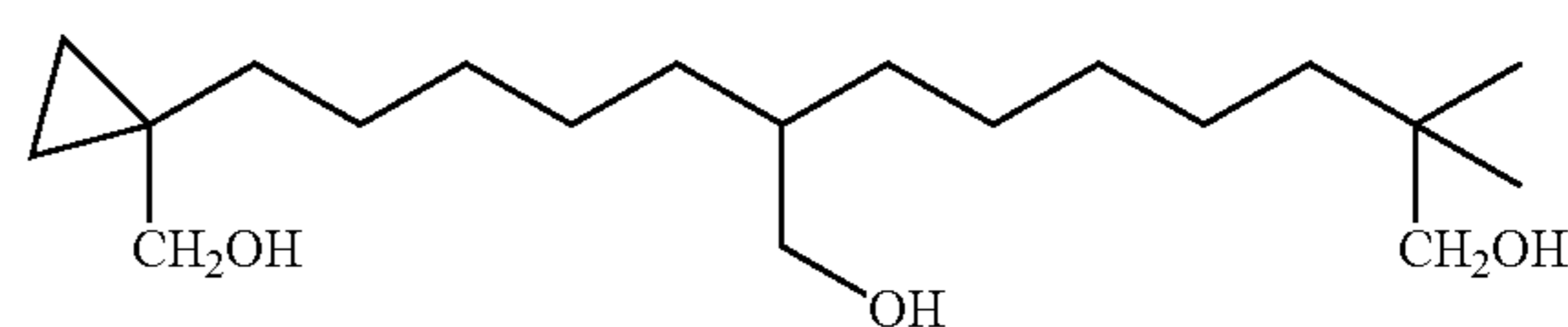
8-[5-(1-Hydroxymethyl-cyclopropyl)-pentyl]-2,2-dimethyl-nonane-1,9-diol
