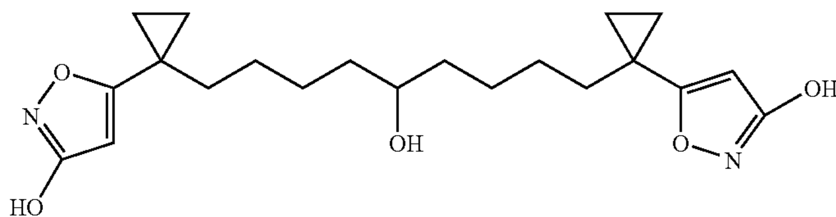
1,9-Bis-[1-(3-hydroxy-isoxazol-5-yl)-cyclopropyl]-nonan-5-ol
