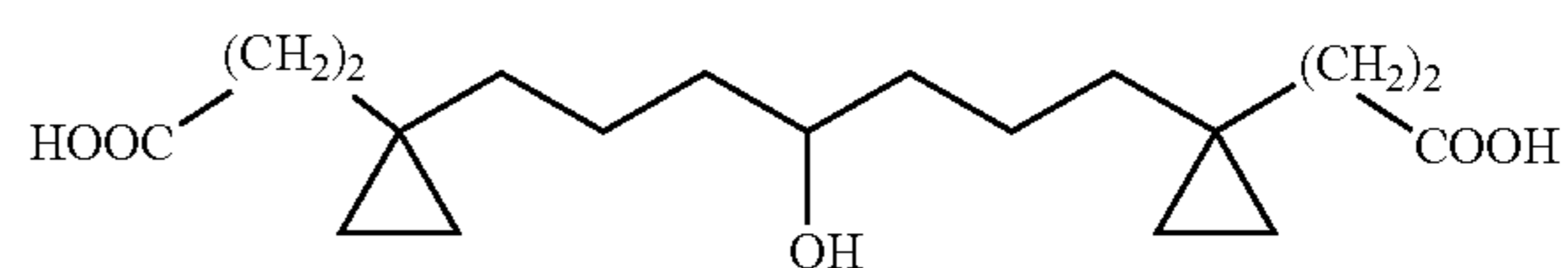
3-(1-{7-[1-(2-Carboxy-ethyl)-cyclopropyl]-4-hydroxy-heptyl}-cyclopropyl)-propionic acid
