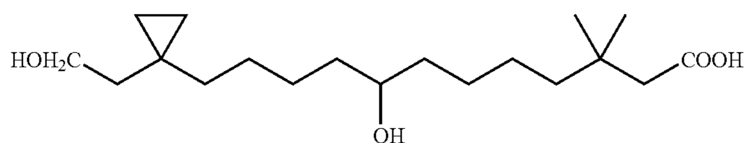
8-Hydroxy-12-[1-(2-hydroxy-ethyl)-cyclopropyl]-3,3-dimethyl-dodecanoic acid
