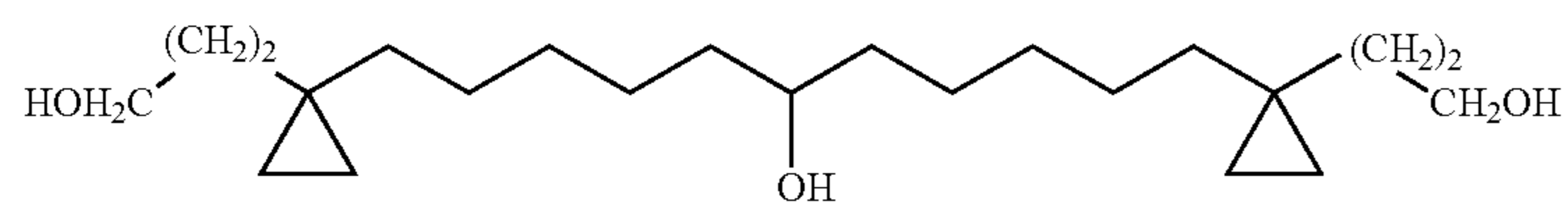
1,11-Bis-[1-(3-hydroxy-propyl)-cyclopropyl]-undecan-6-ol
