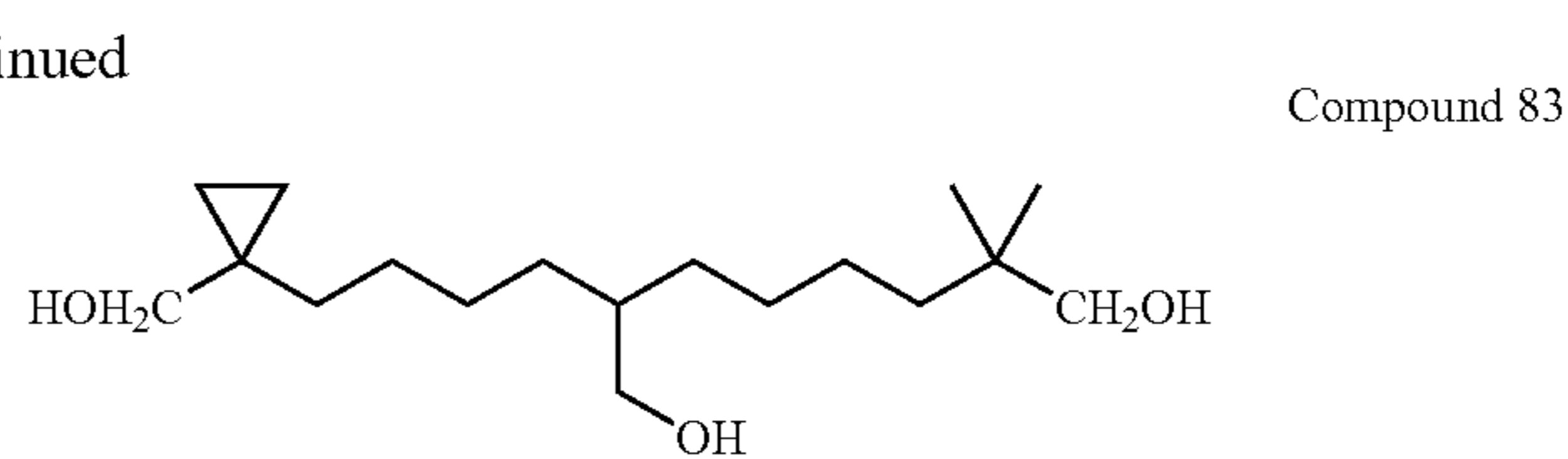
7-[4-(1-Hydroxymethyl-cyclopropyl)-butyl]2,2-dimethyl-octane-1,8-diol
