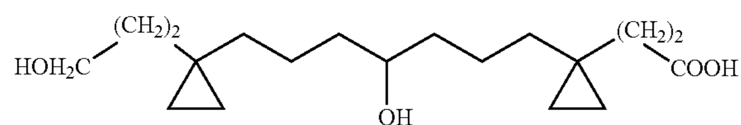
3-(1-{4-Hydroxy-7-[1-(3-hydroxy-propyl)-cyclopropyl]-heptyl}-cyclopropyl)-propionic acid
