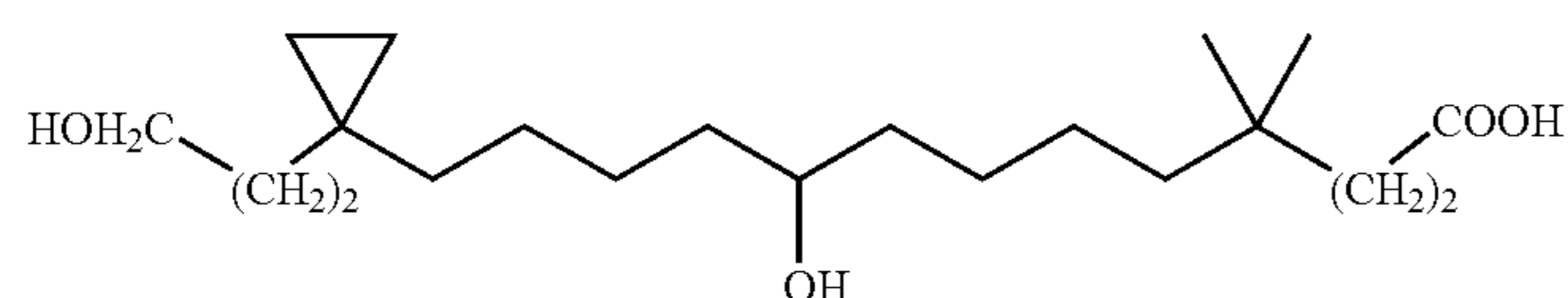
4,4-Dimethyl-9-hydroxy-13-[1-(3-hydroxypropyl)-cyclopropyl]-tridecanoic acid
