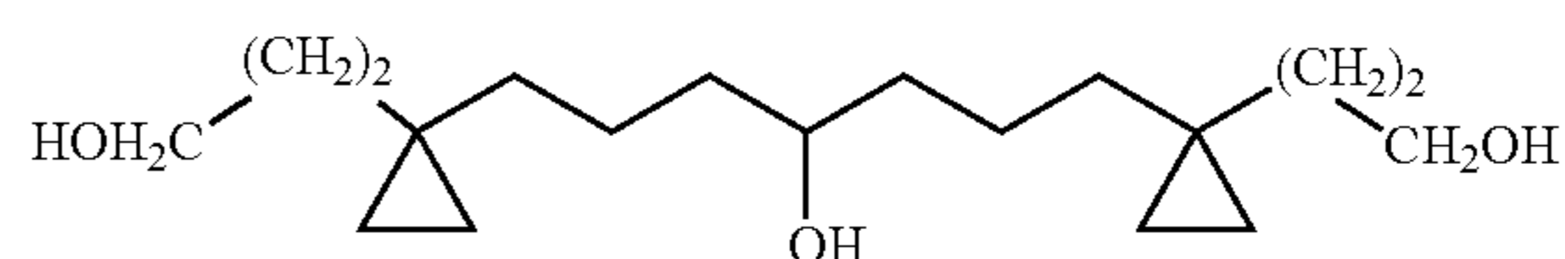
1,7-Bis-[1-(3-hydroxy-propyl)-cyclopropyl]-heptan-4-ol
