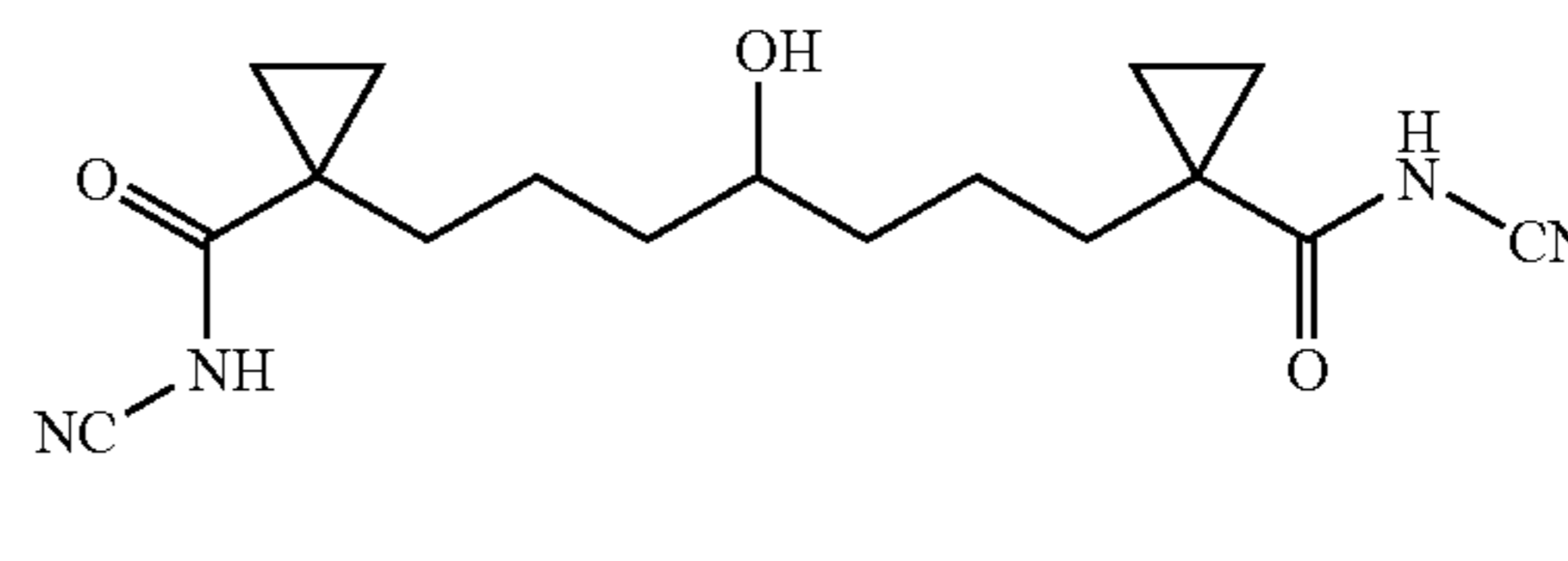
1,7-Bis-(1-dicyanimido-cyclopropyl)-4-hydroxy-heptane
