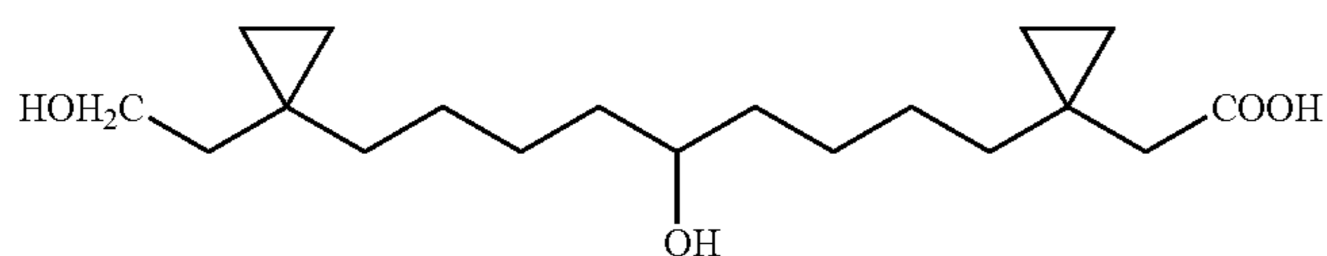
1-(5-Hydroxy-9-[1-(2-hydroxy-ethyl)-cyclopropyl]-nonyl)-cyclopropyl-acetic acid
