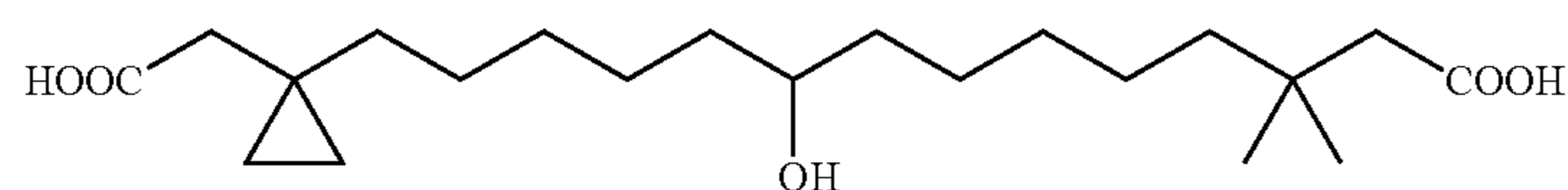
14-(1-Carboxymethyl-cyclopropyl)-9-hydroxy-3,3-dimethyl-tetradecanoic acid
