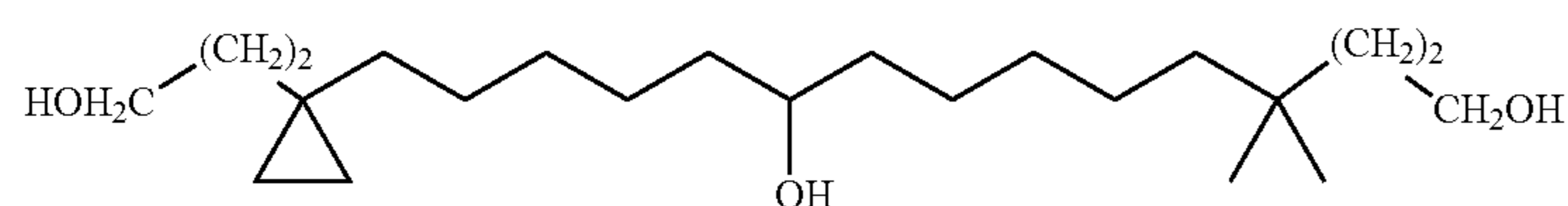
15-[1-(3-Hydroxy-propyl)-cyclopropyl]-4,4-dimethyl-pentadecane-1,10-diol
