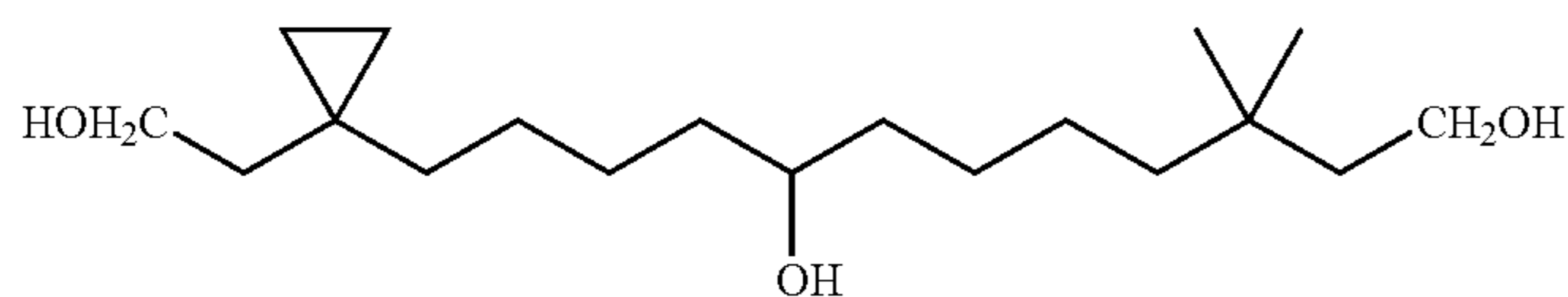
12-[1-(2-Hydroxy-ethyl)-cyclopropyl]-3,3-dimethyl-dodecane-1,8-diol
