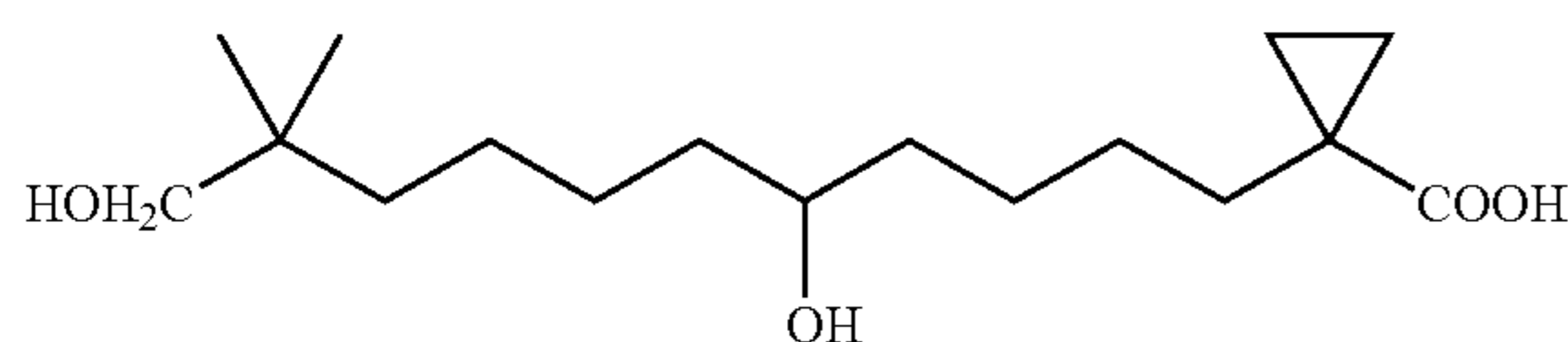
1-(5,11-Dihydroxy-10,10-dimethyl-undecyl)- cyclopropanecarboxylic acid
