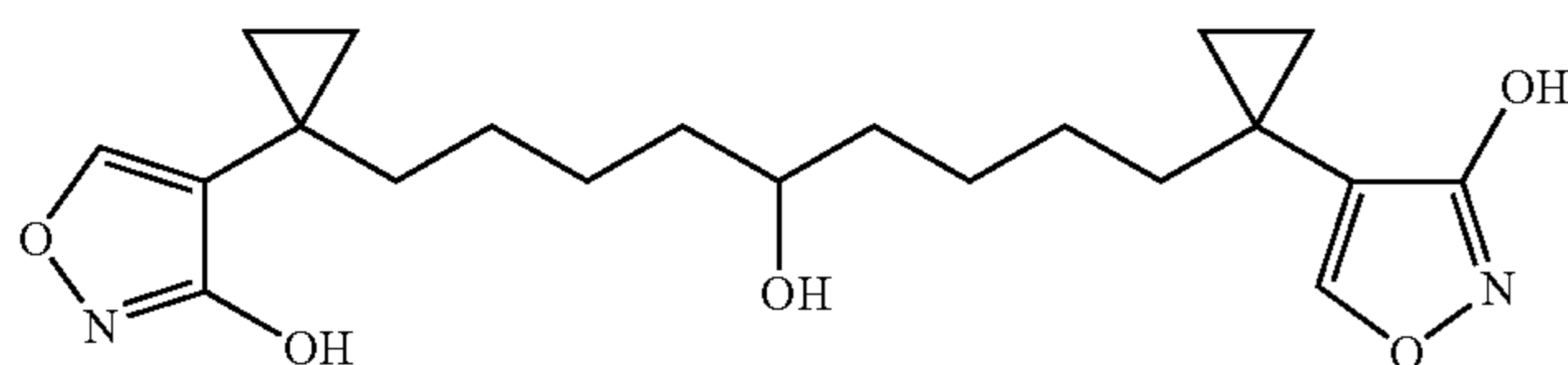
1,9-Bis-[1-(3-hydroxy-isoxazol-4-yl)-cyclopropyl]-nonan-5-ol
