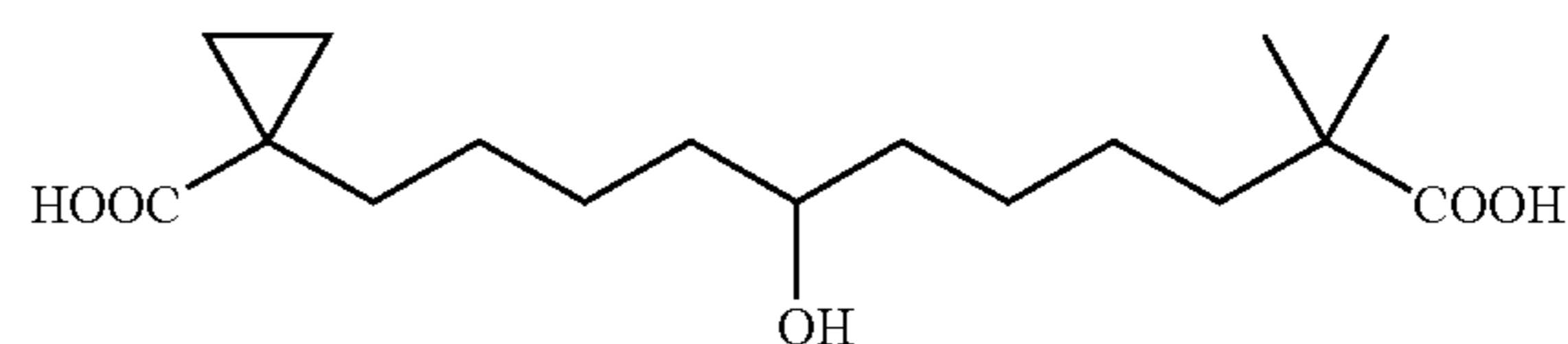
1-(10-Carboxy-5-hydroxy-10-methyl-undecyl)- cyclopropanecarboxylic acid
