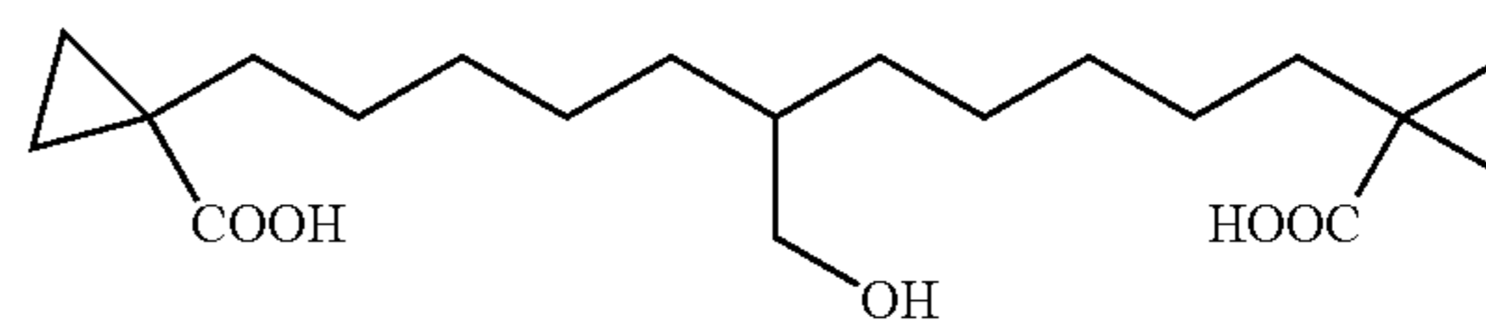
1-(12-Carboxy-6-hydroxymethyl-12-methyl-tridecyl)-cyclopropanecarboxylic acid
