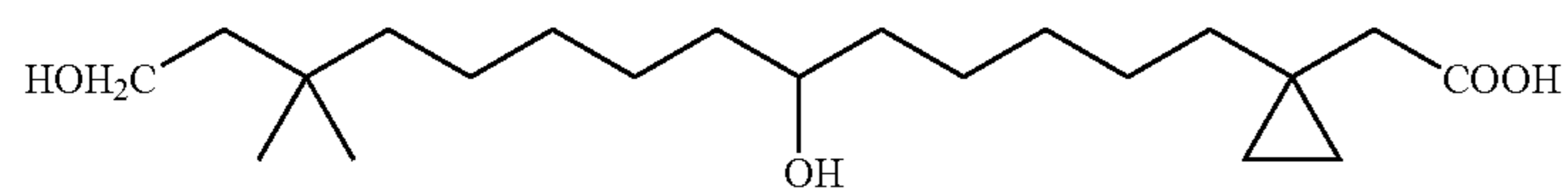
[1-(6,14-Dihydroxy-12,12-dimethyl-tetradecyl)-cyclopropyl]-acetic acid
