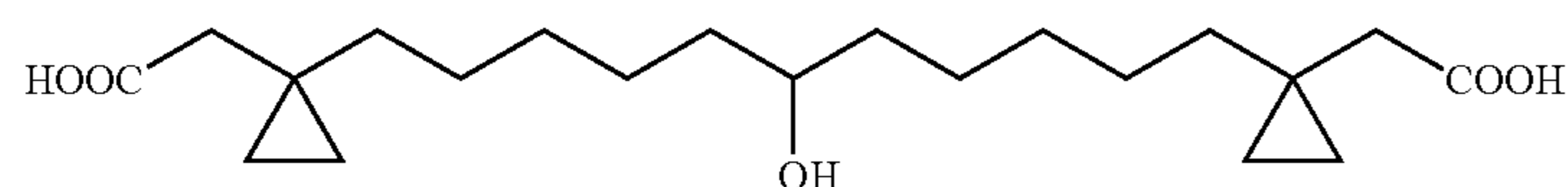
{1-11-(1-Carboxymethyl-cyclopropyl)-6-hydroxy-undecyl}-cyclopropyl}-acetic acid
