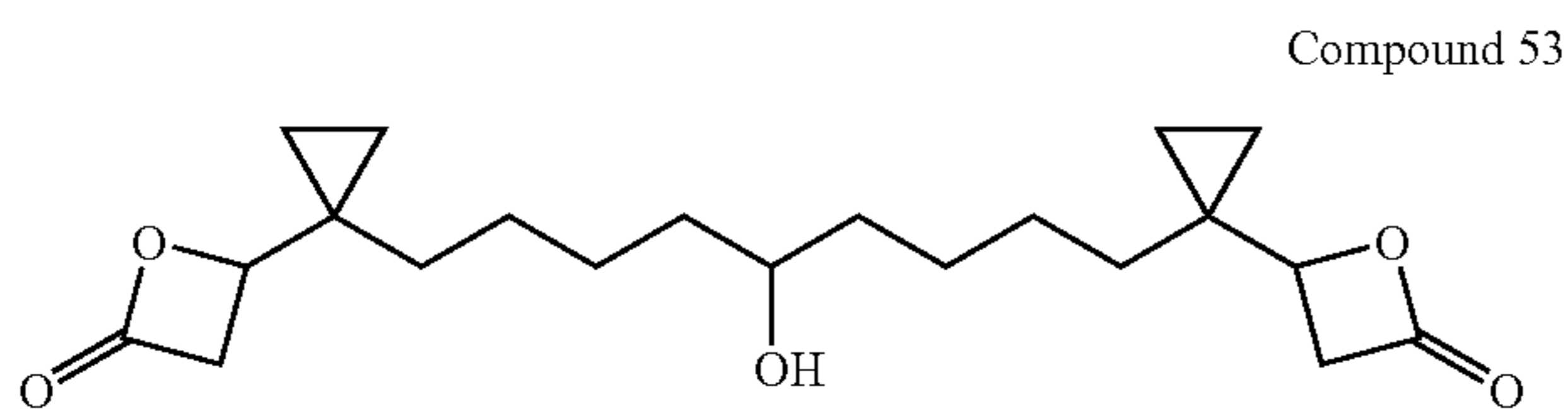
1,9-Bis-[1-(tetrahydro-pyran-2-yloxy)-cyclopropyl]-nonan-5-ol
