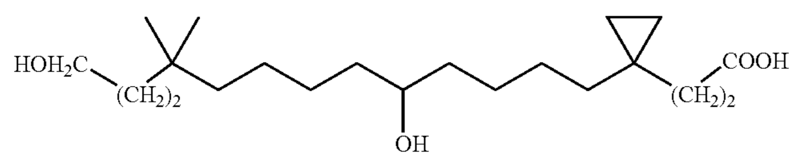
3-[1-(5,13-Dihydroxy-10,10-dimethyl-tridecyl)-cyclopropyl]-propionic acid
