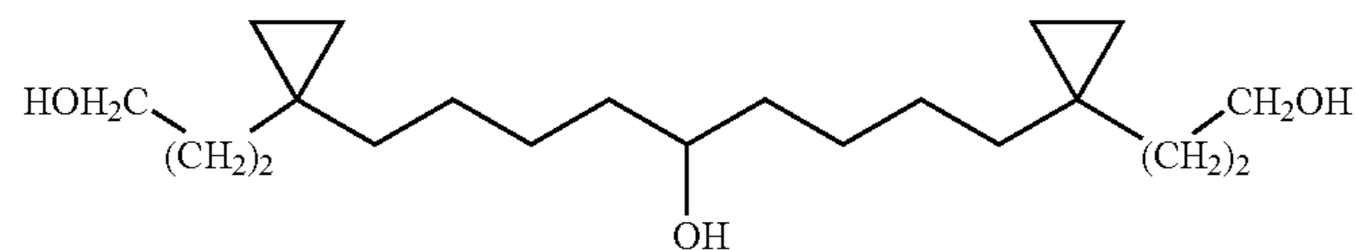
1,9-Bis-[1-(3-hydroxy-propyl)-cyclopropyl]-nonan-5-ol
