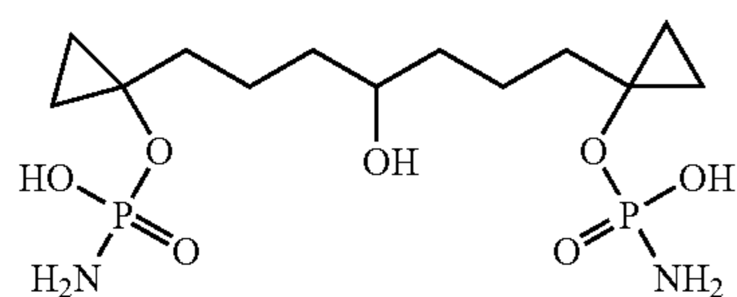
1,7-Bis-(1-phosponamid-cyclopropyl)-4-hydroxy-heptane
