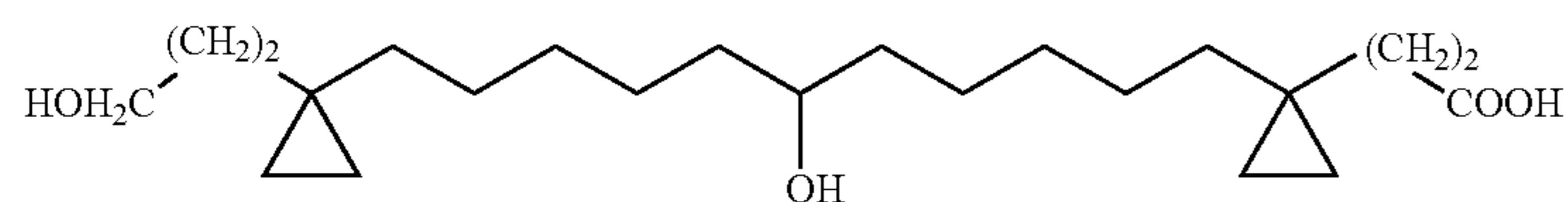
3-(1-{6-Hydroxy-11-[1-(3-hydroxy-propyl)-cyclopropyl]-undecyl}-cyclopropyl)-propionic acid
