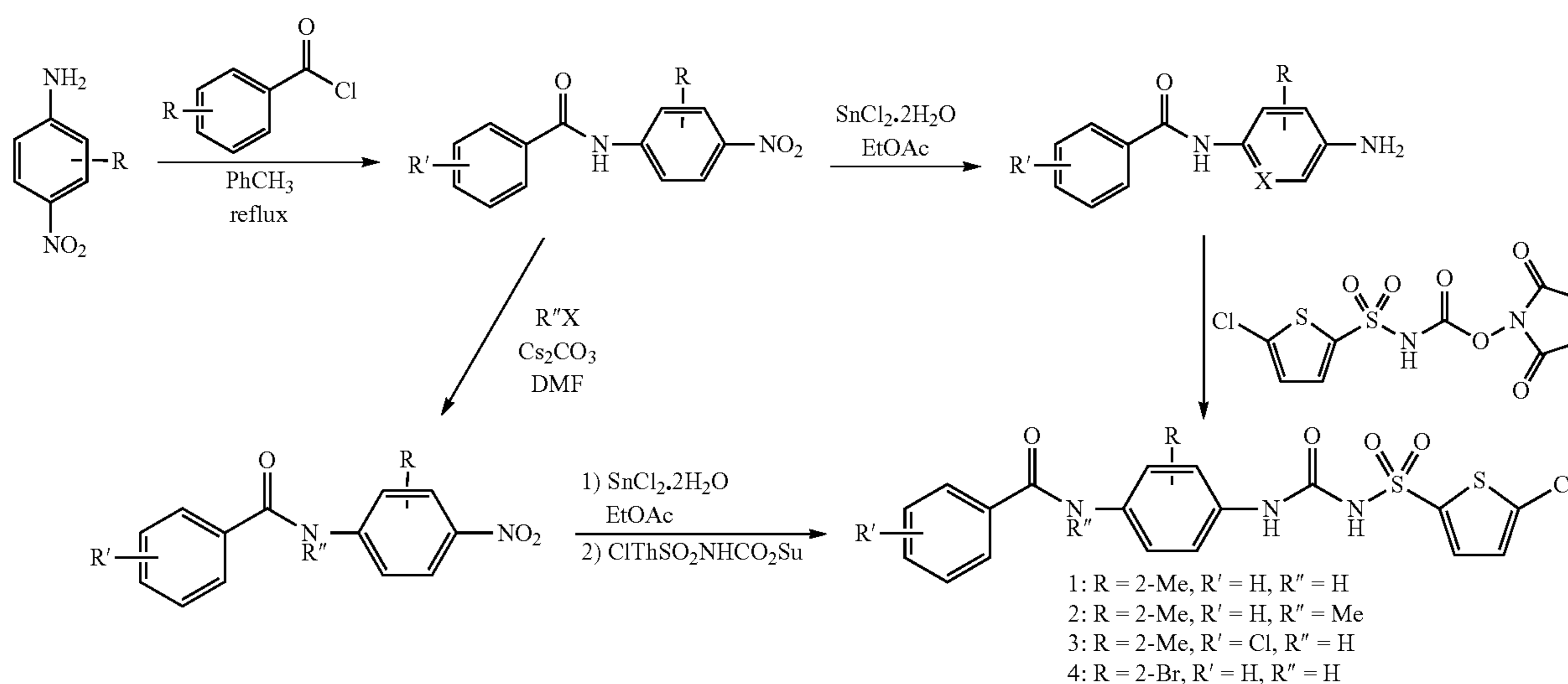
Scheme 3 Benzamide-containing Sulfonylureas
