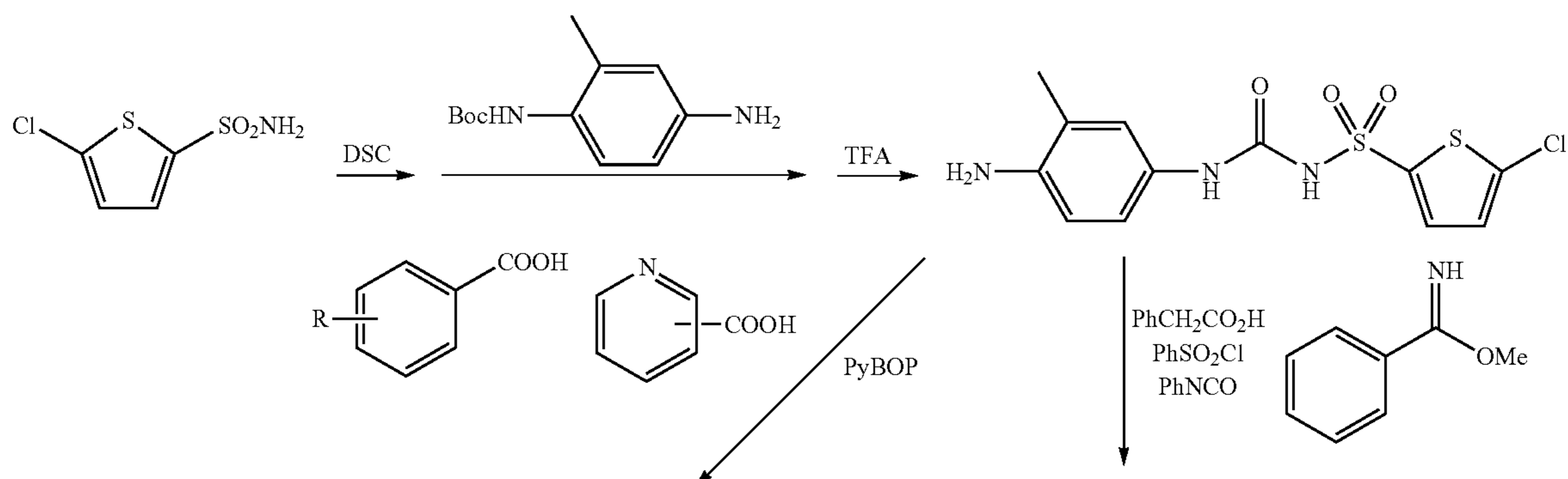
Scheme 4
