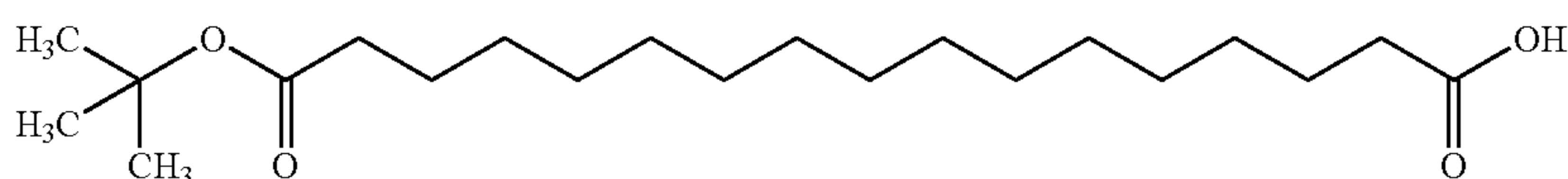
2-Methoxycarbonyl-heptadecanedioic acid 1-methyl ester
