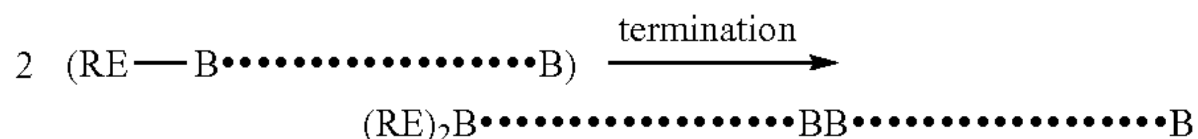
REACTION SCHEME 6:
