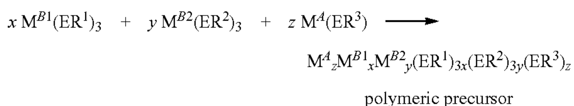
REACTION SCHEME 12:
