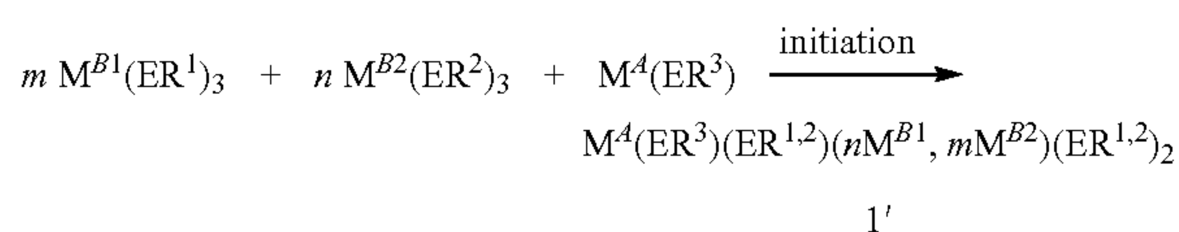
REACTION SCHEME 8:
