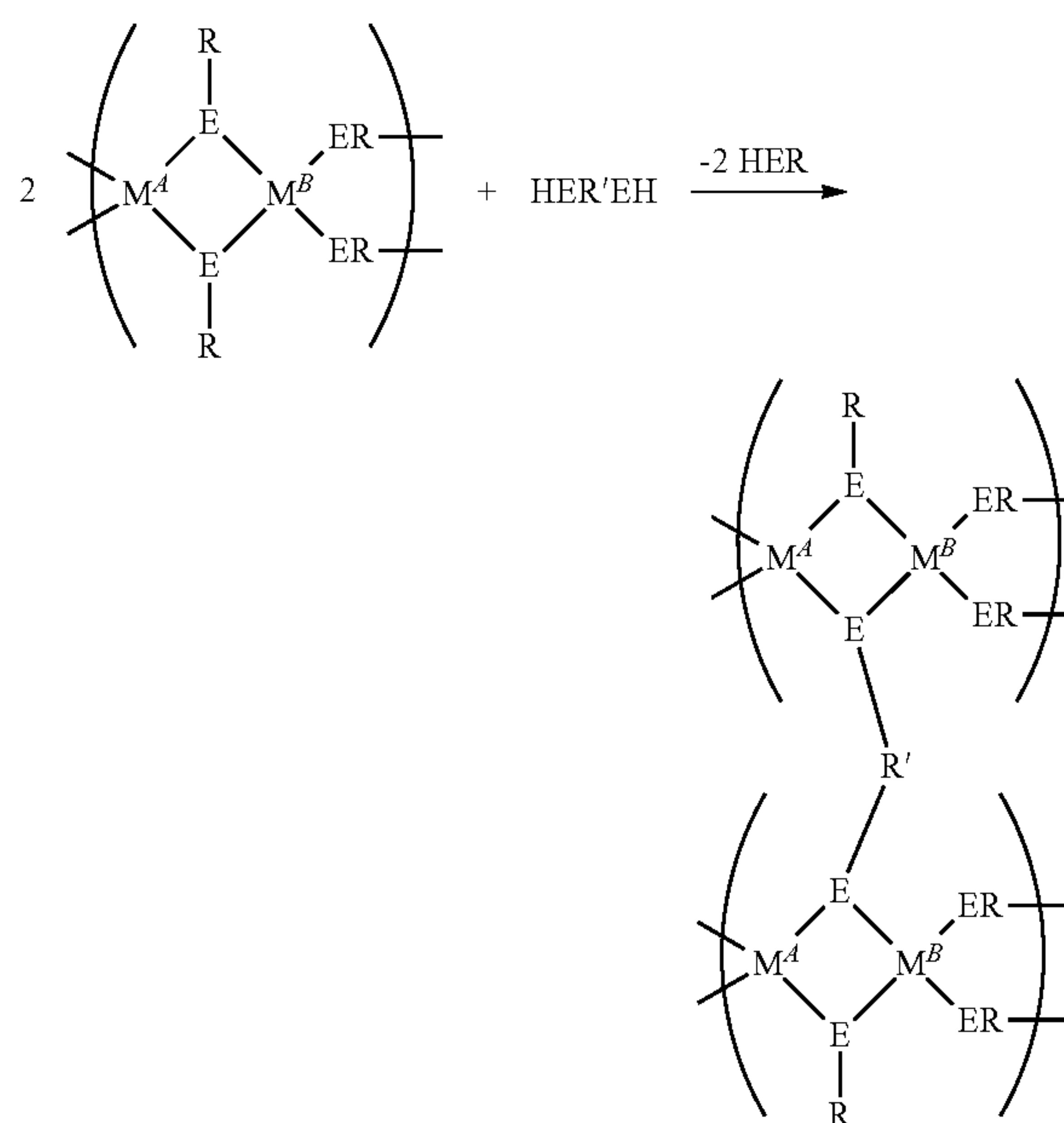
REACTION SCHEME 14
