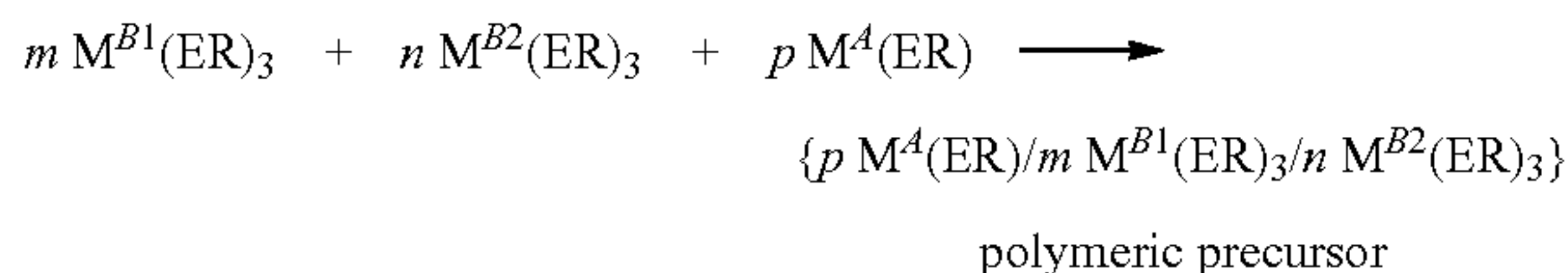
REACTION SCHEME 9:
