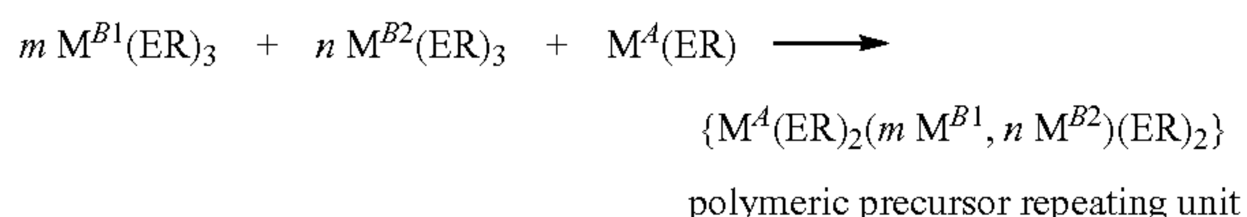
REACTION SCHEME 10:
