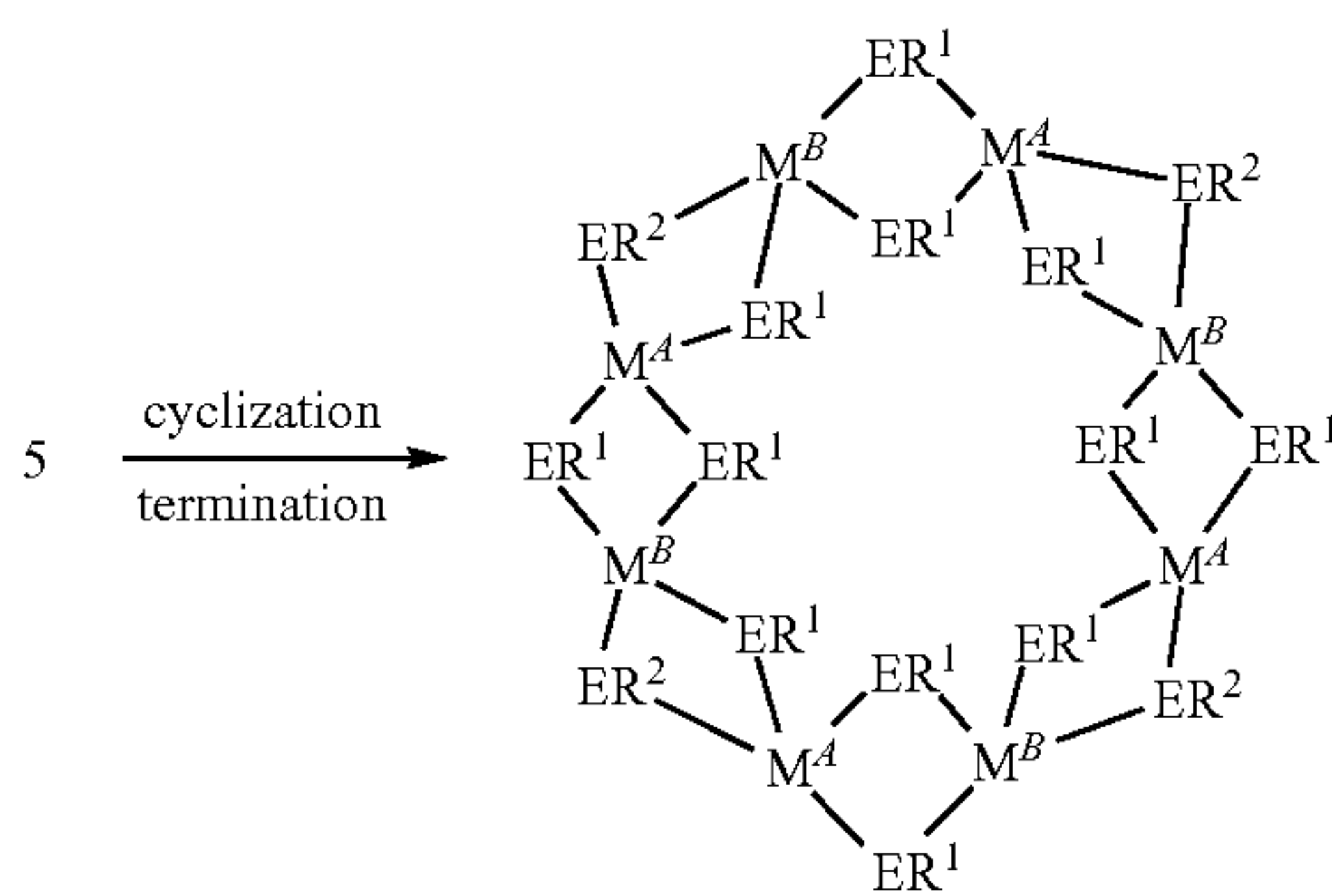
REACTION SCHEME 7:
