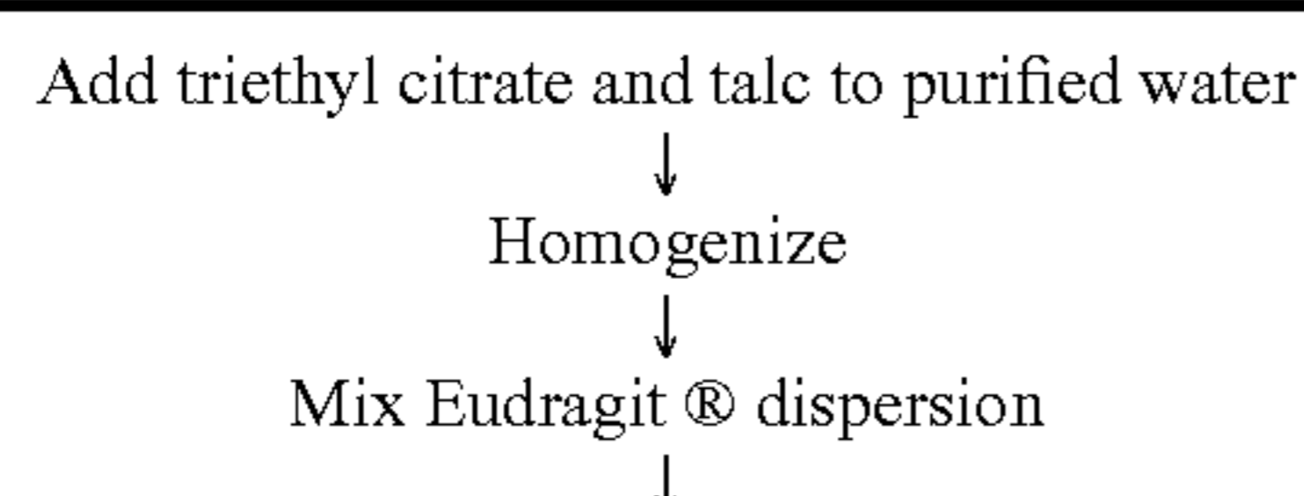
Schematic of Tablet-Core Spray-Coating Process
