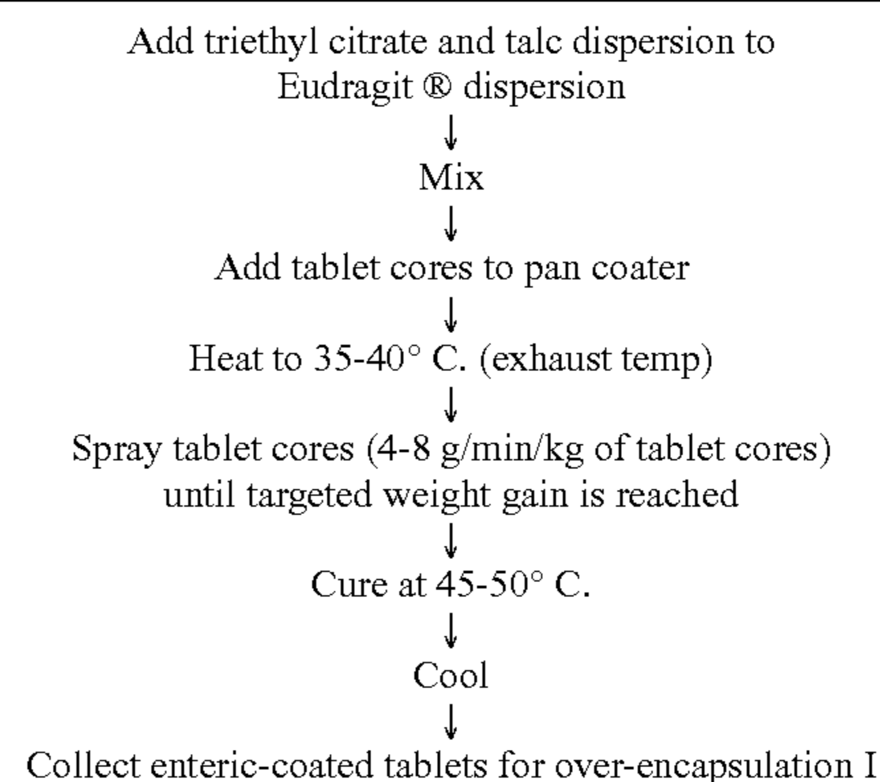
Schematic of Tablet-Core Spray-Coating Process
