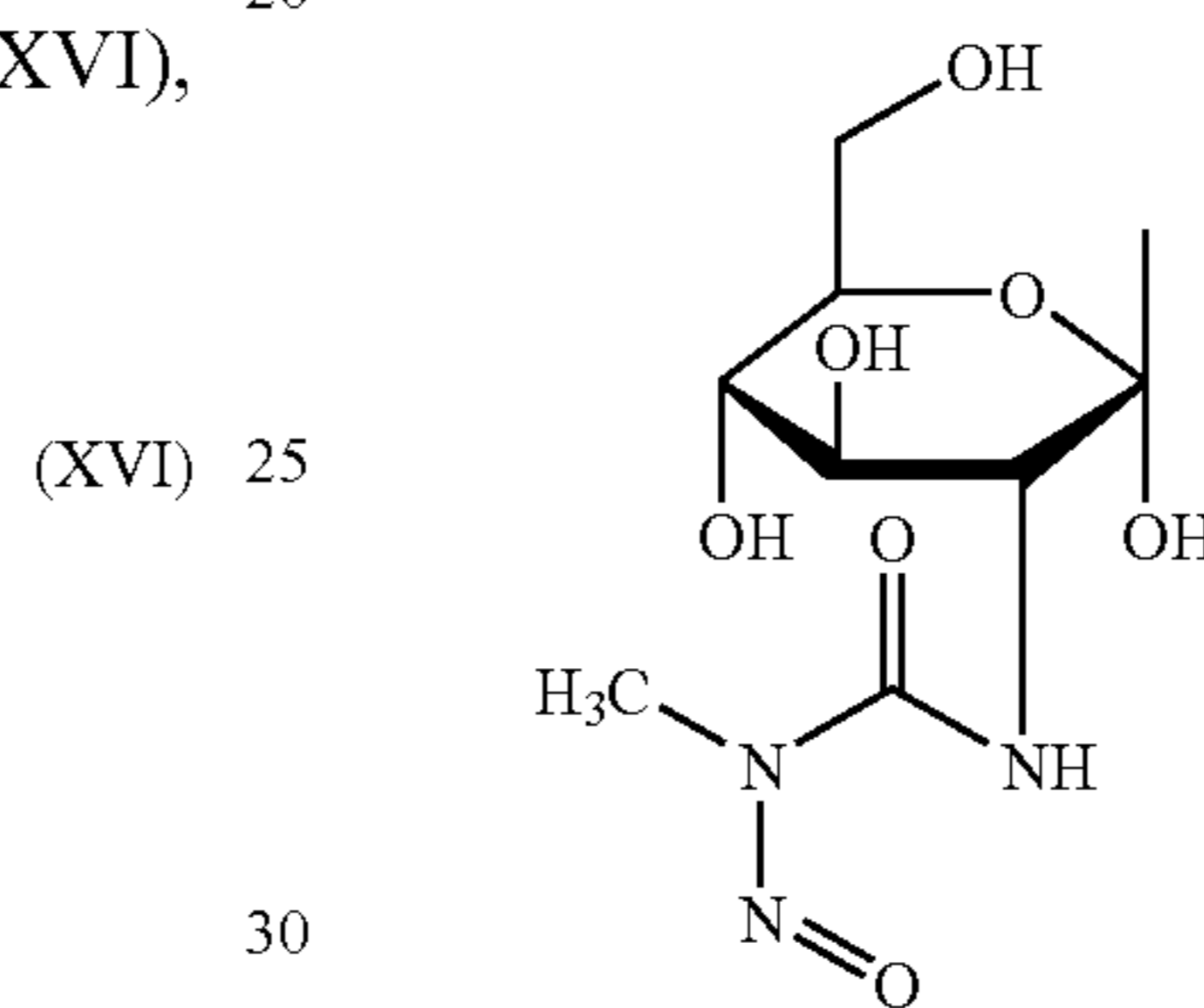
Streptozocin
