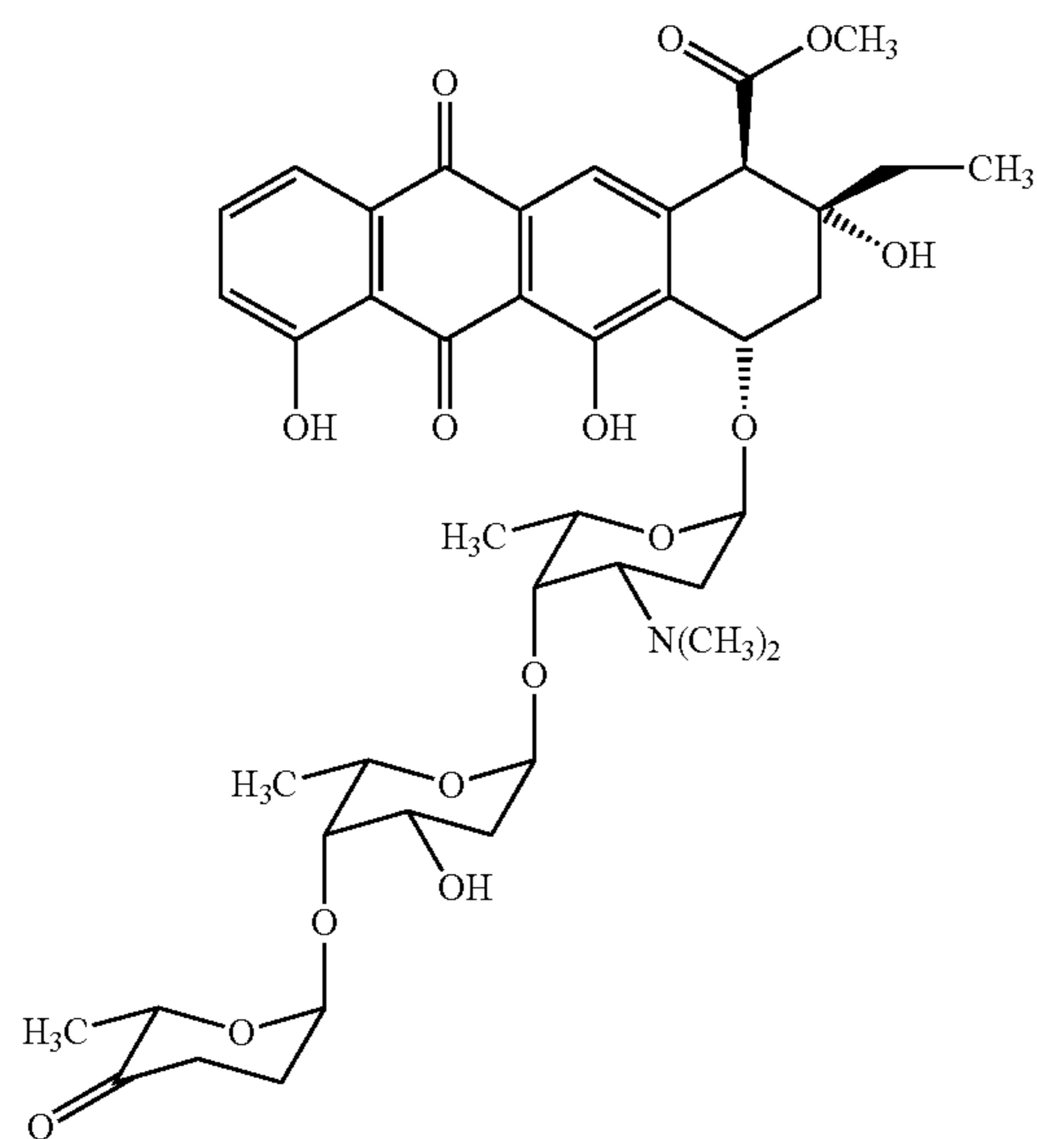
Aclacinomycin A
