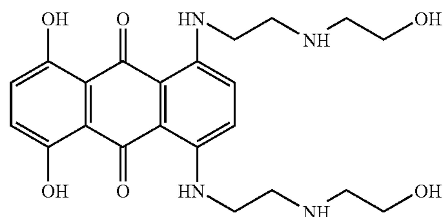
Mitoxantrone
