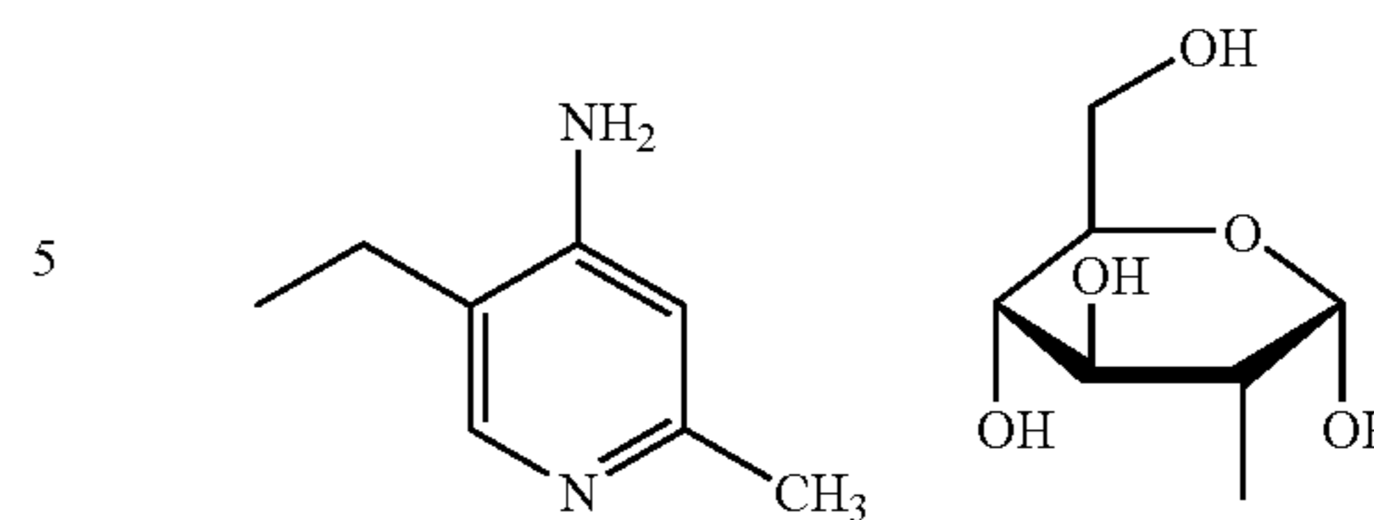
Nimustine
