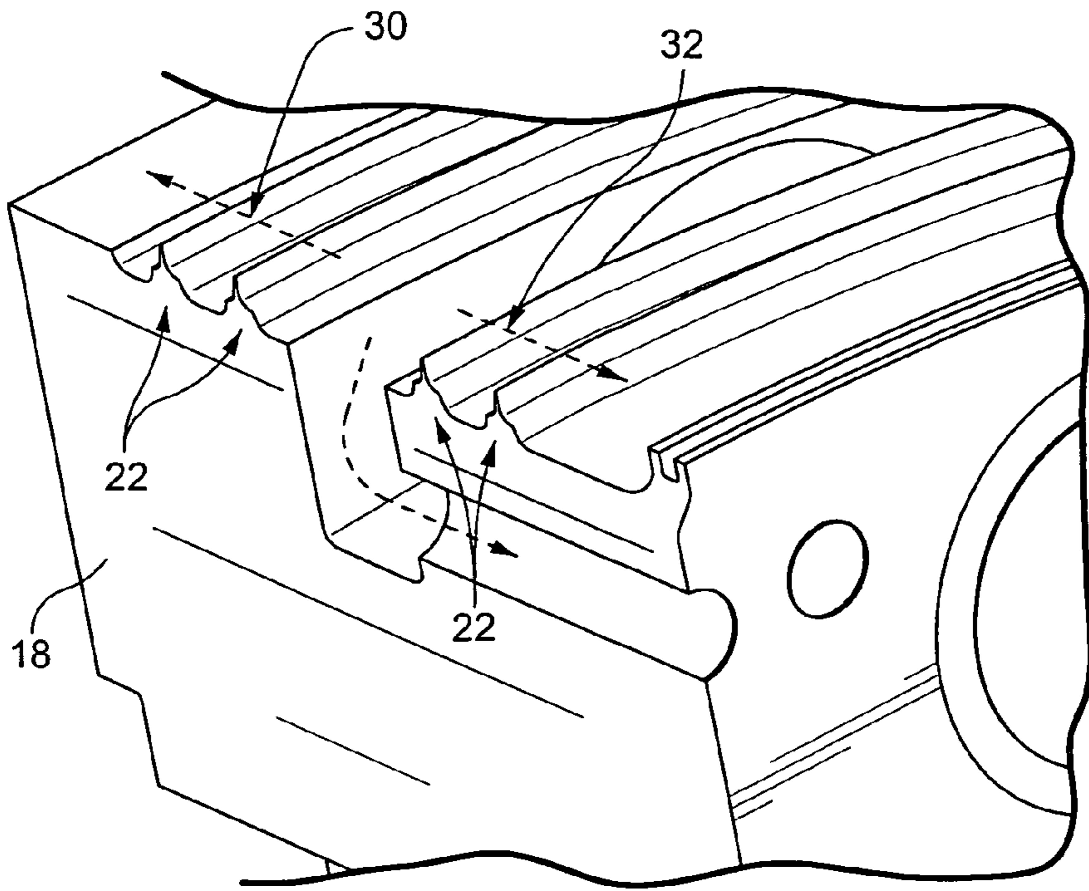
Fig. 2 (PRIOR ART)
