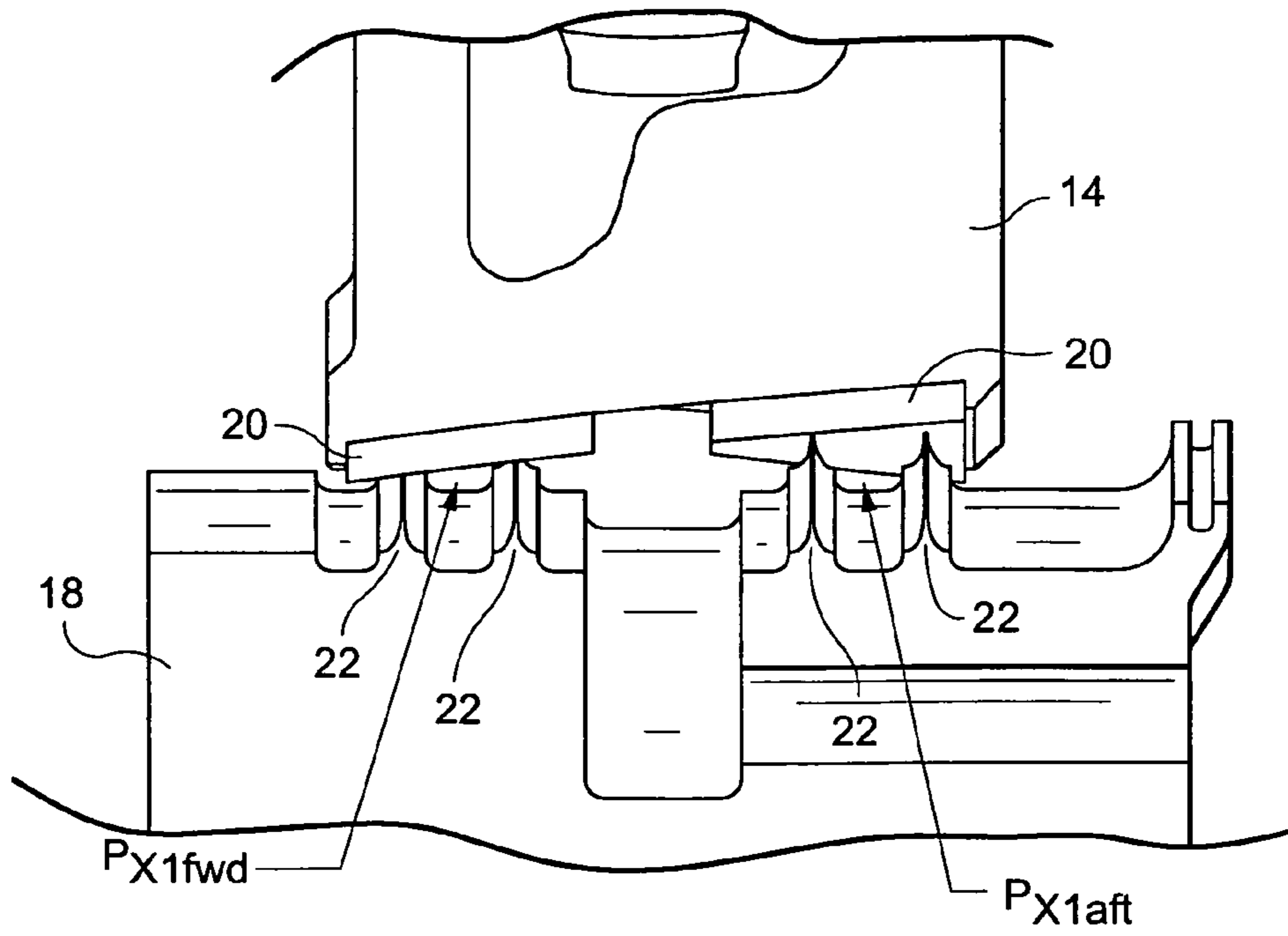
Fig. 4 (PRIOR ART)
