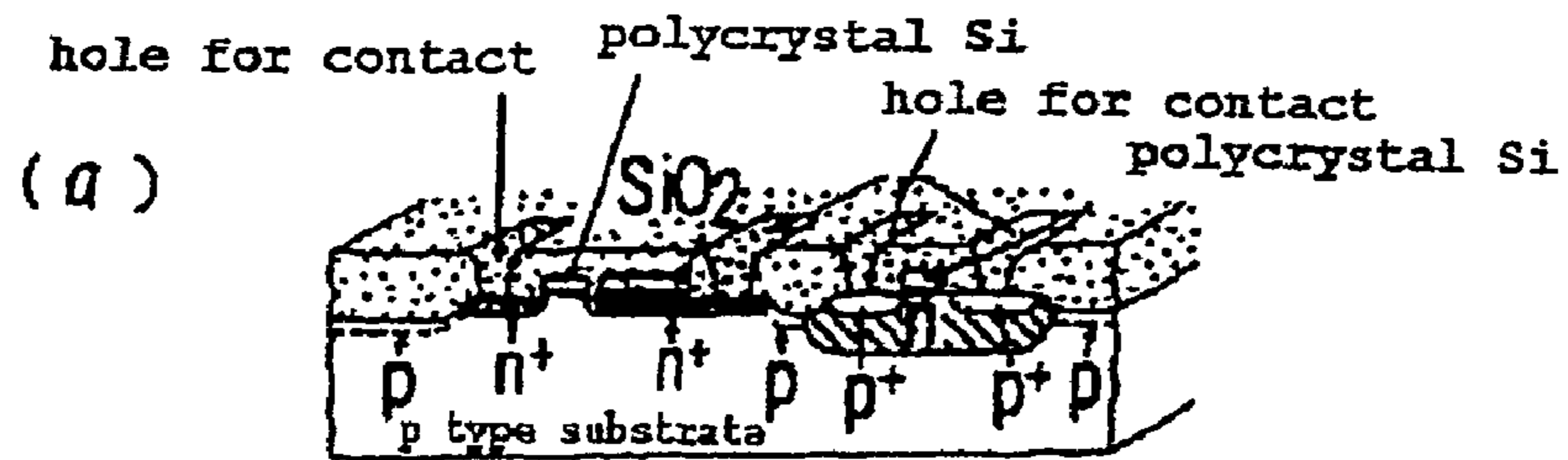
formation of hole for contact
