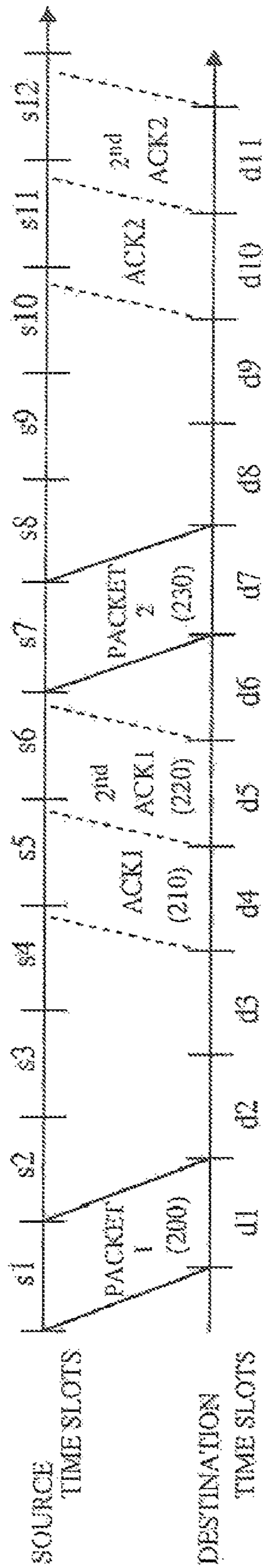
(PRIOR ART) FIG. 2
