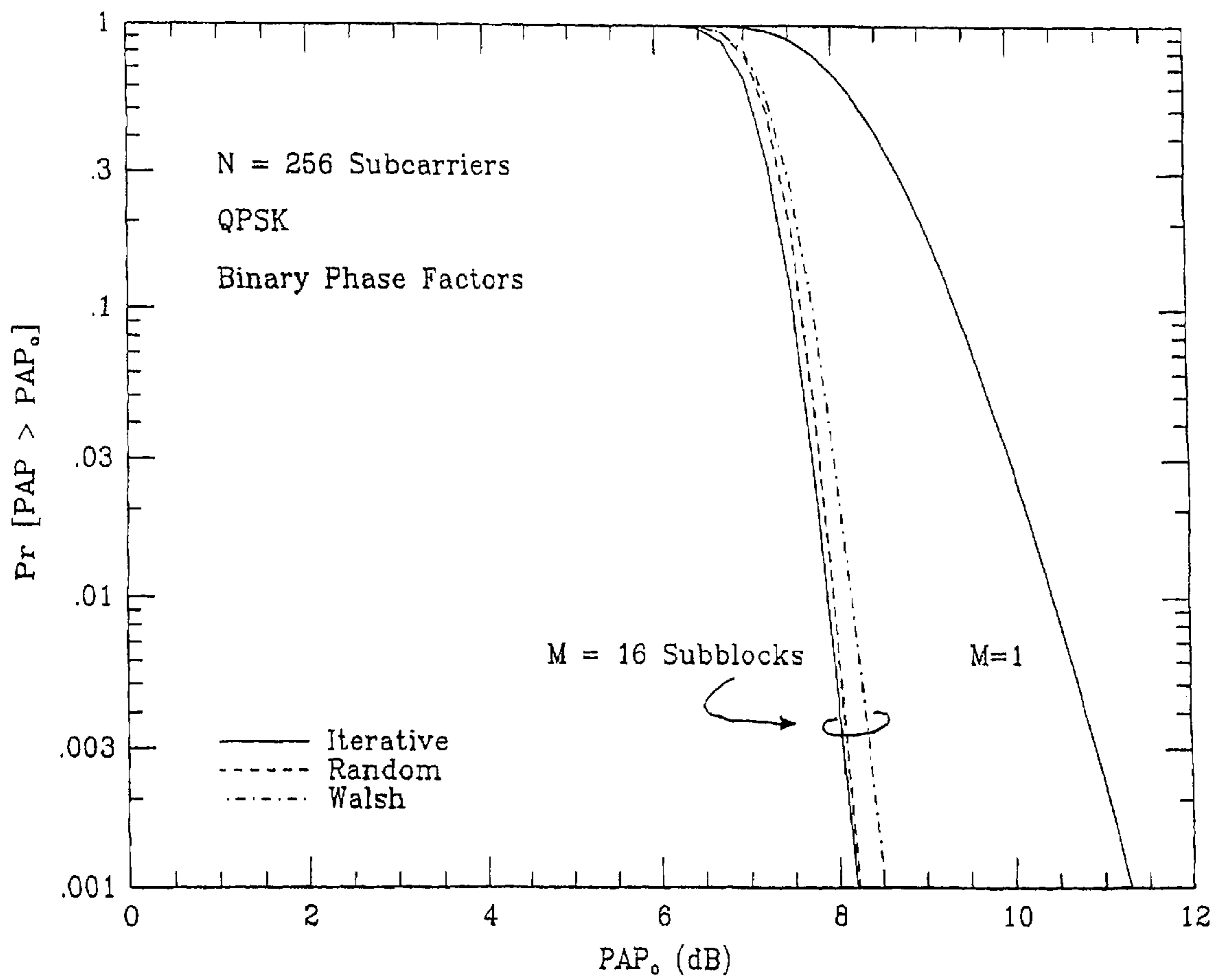
FIG. 14 Performance of Walsh sequences.
