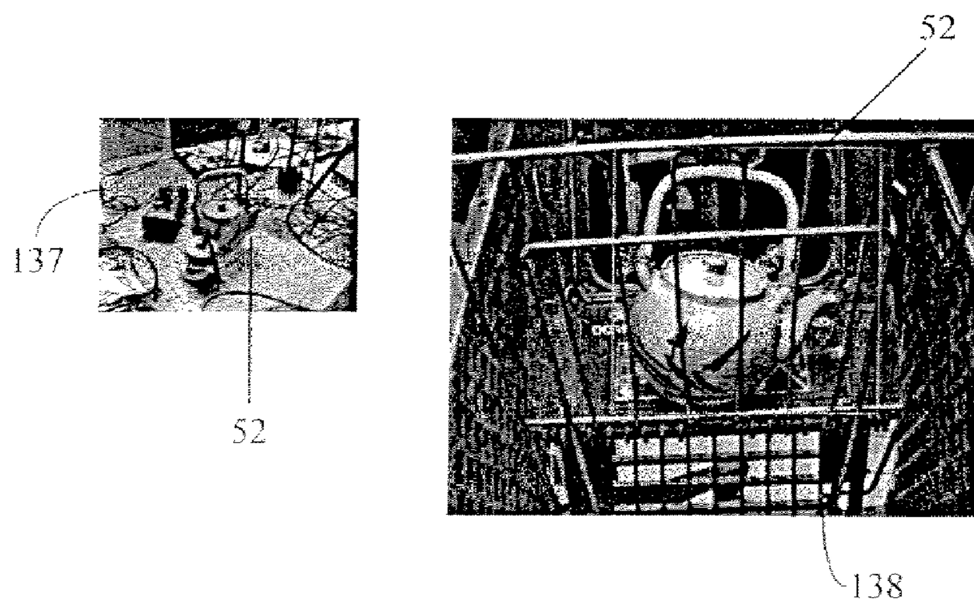
FIG. 32 Teapot Detection
