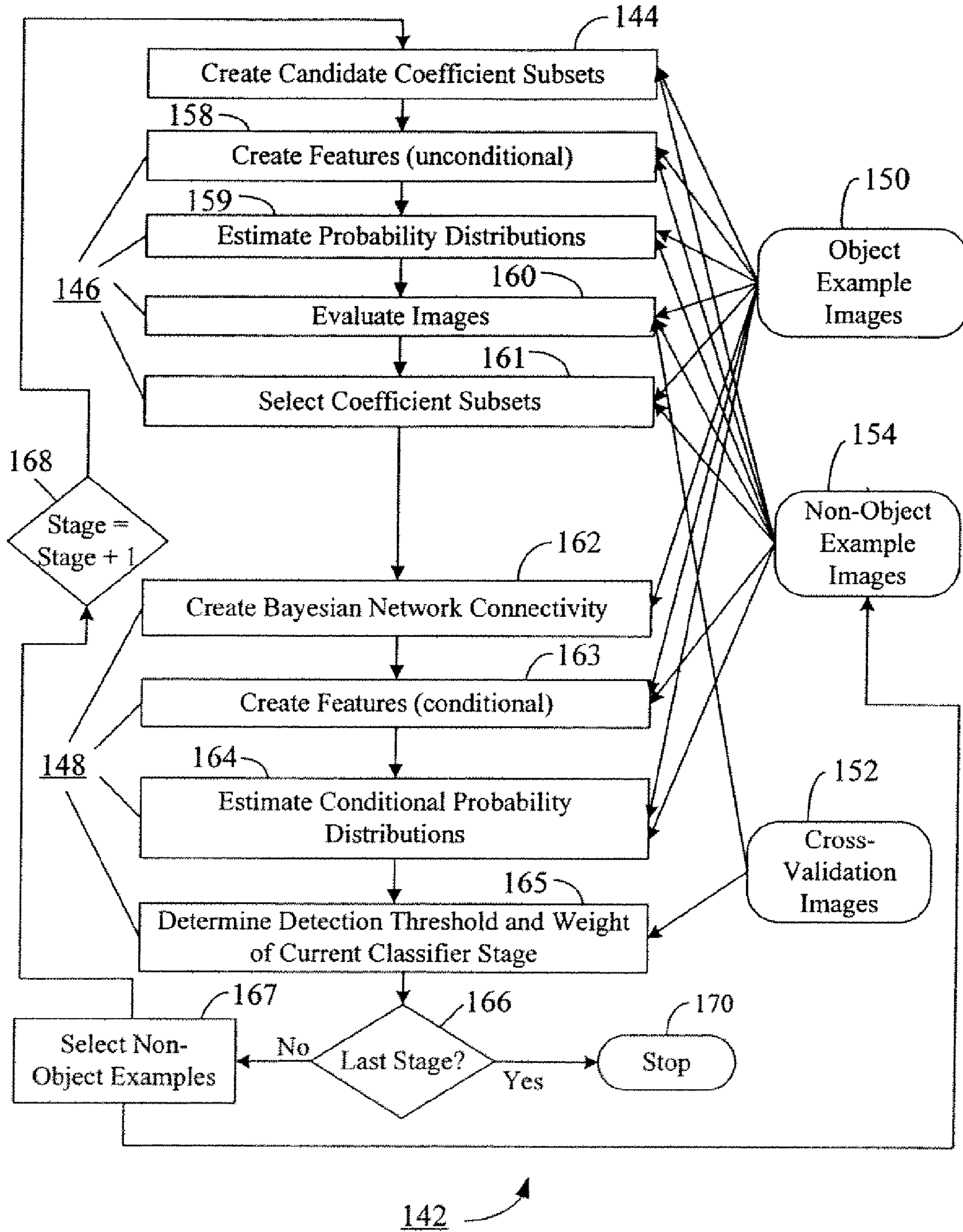
System for building Bayesian Network based classifier
