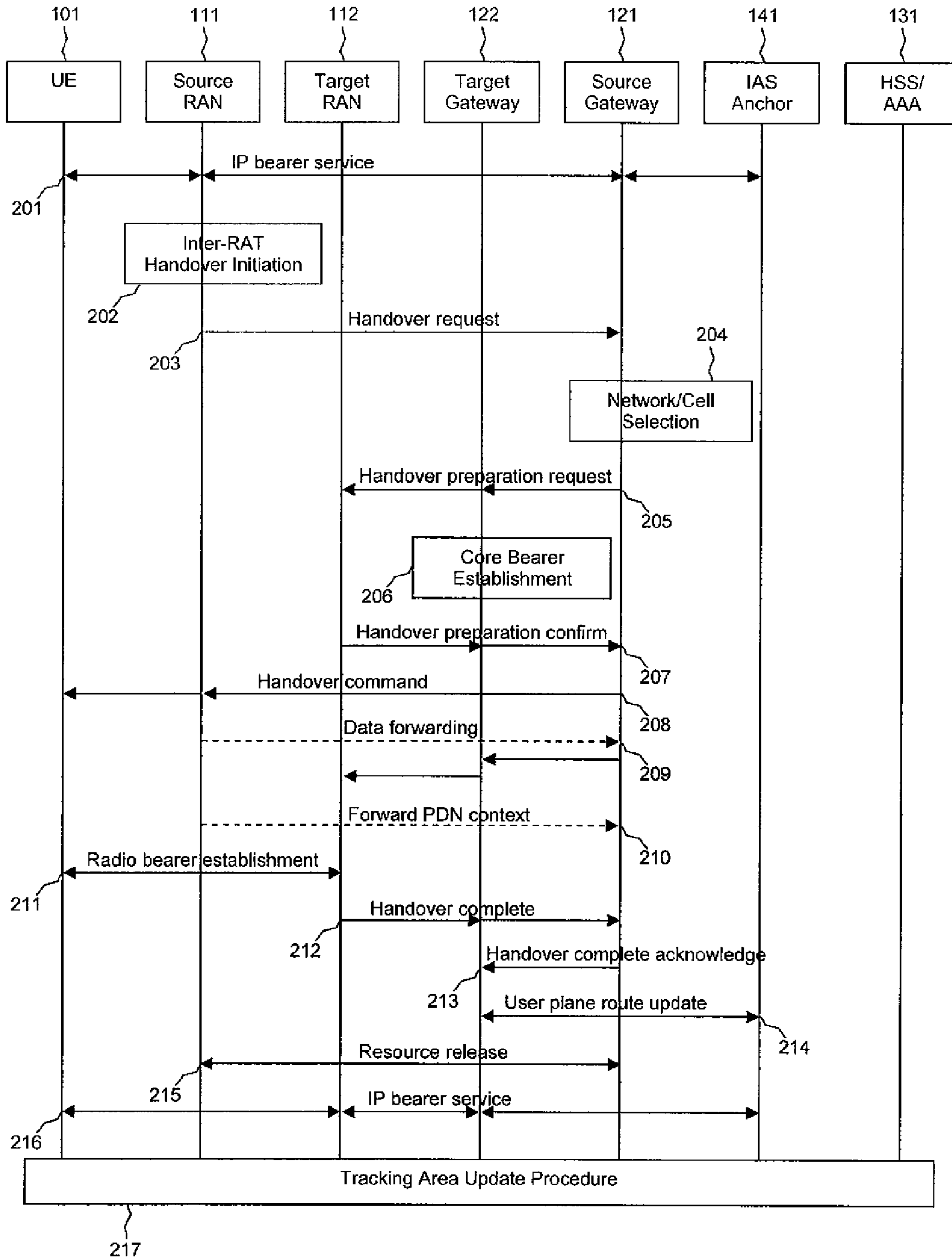
Figure 2 (prior art)
