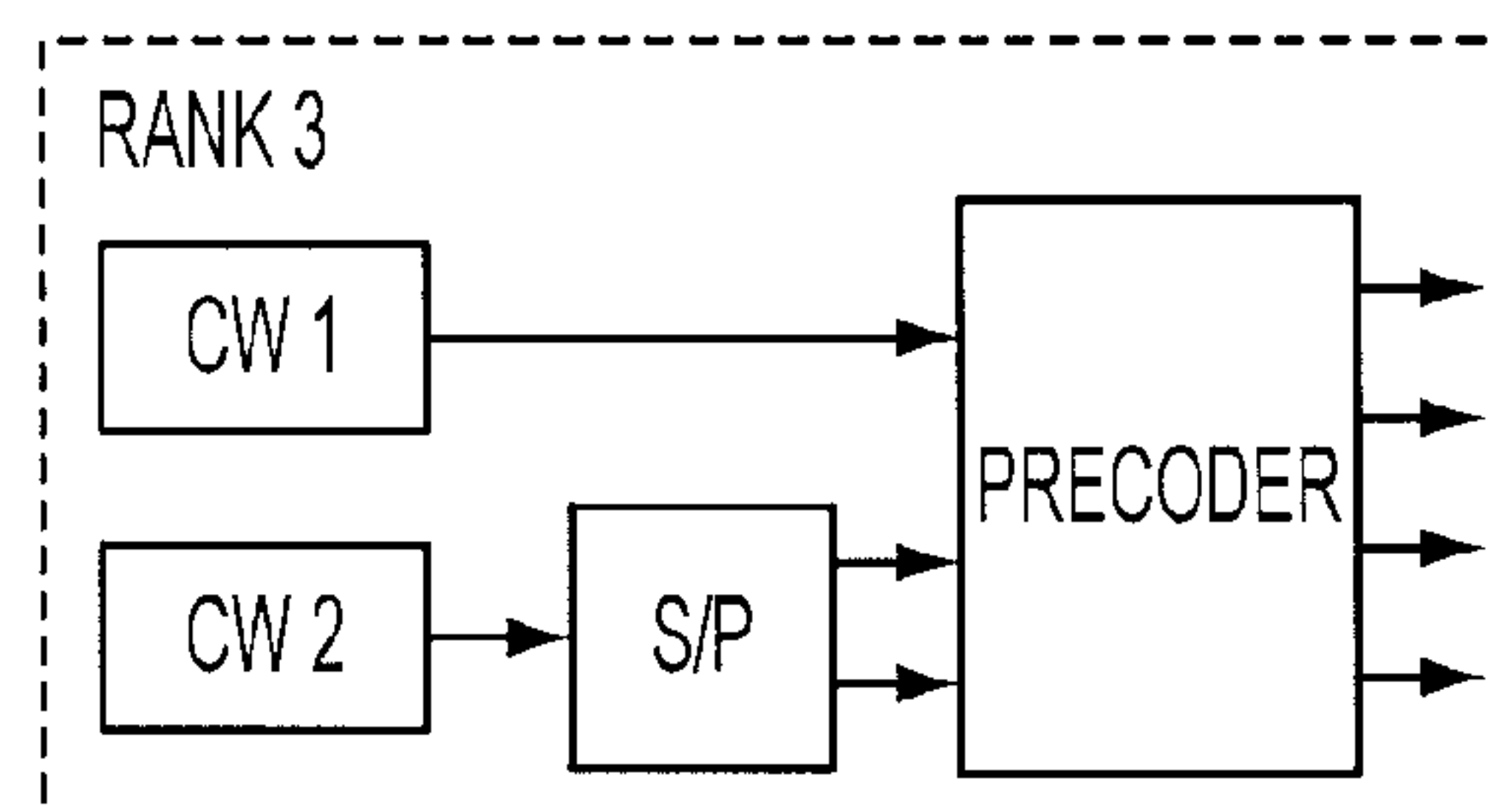
FIG. 5C PRIOR ART
