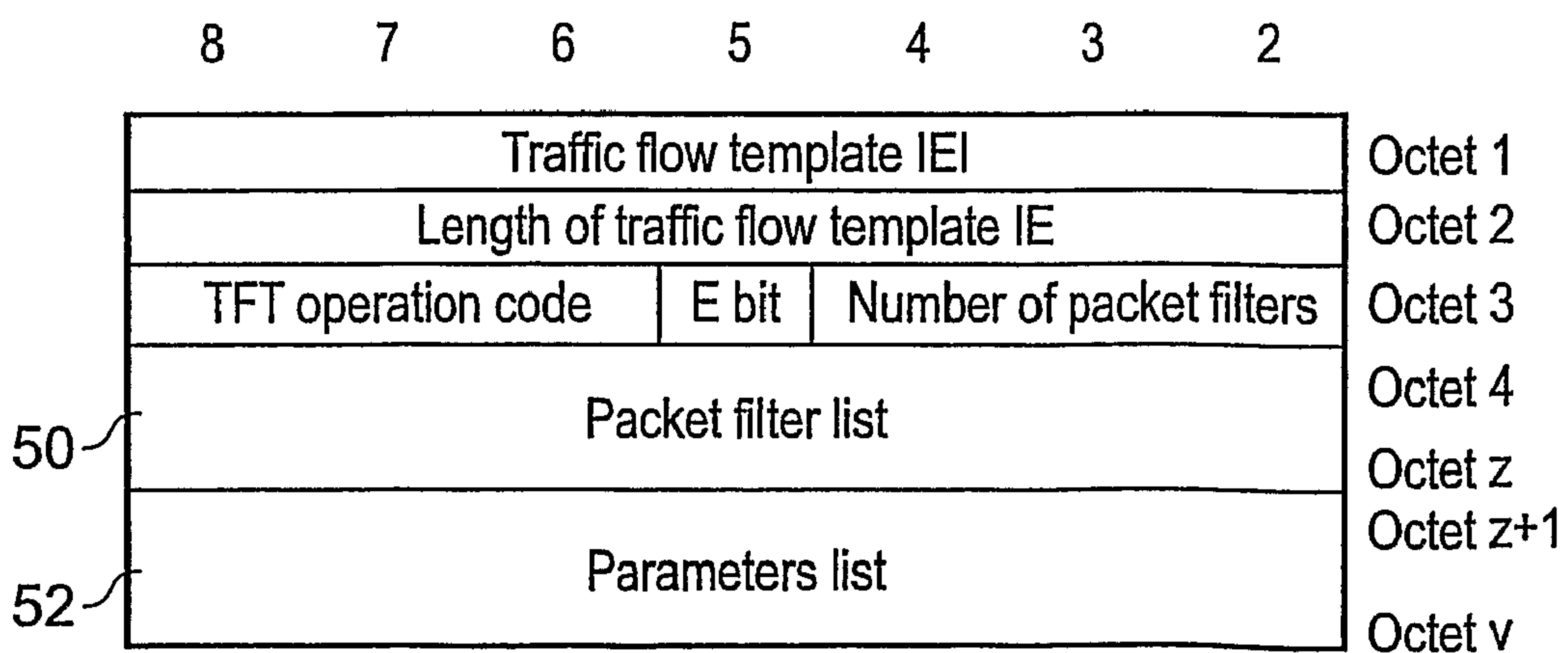
Fig. 12: Traffic Flow Template Information Element
