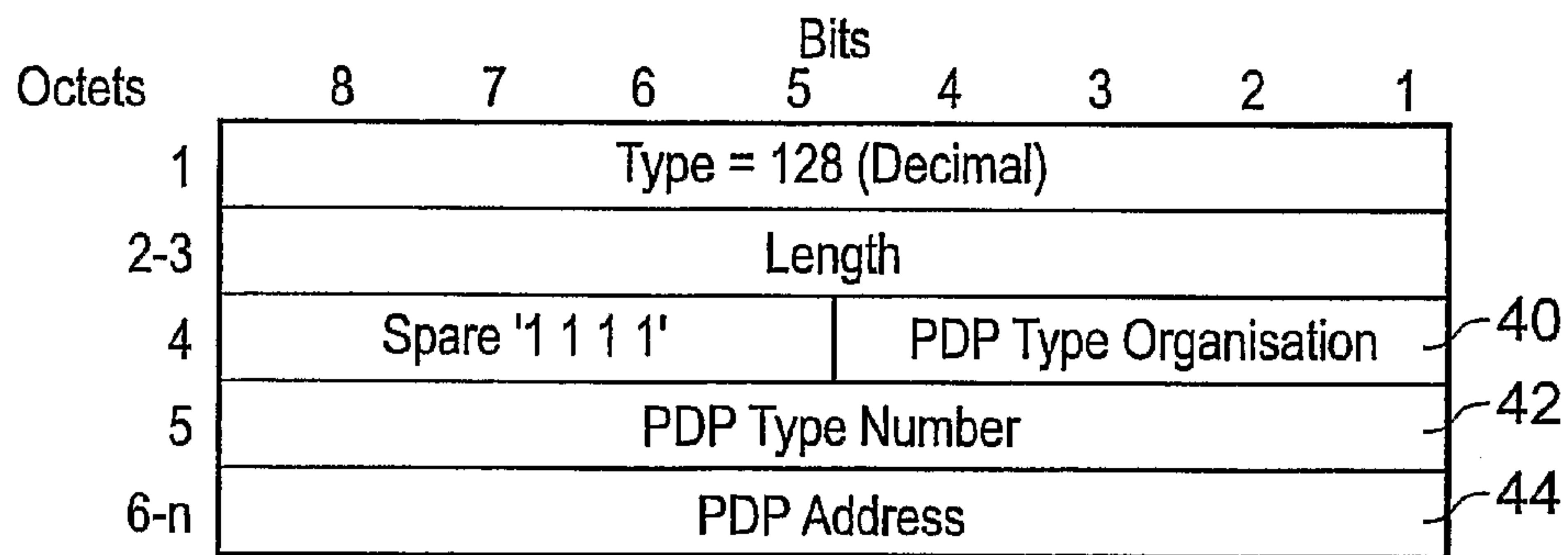
Fig. 6: End User Address Information Element
