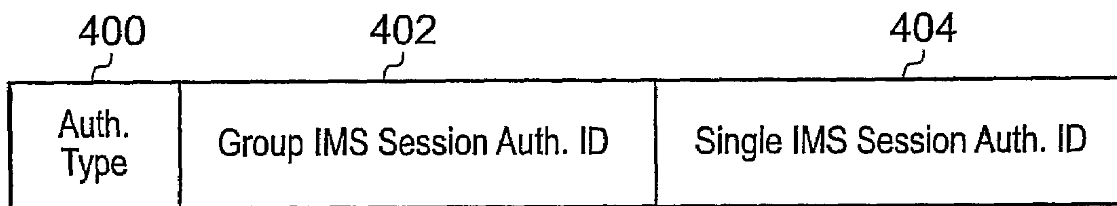
Fig. 19: A Hierarchical Authorisation ID Structure
