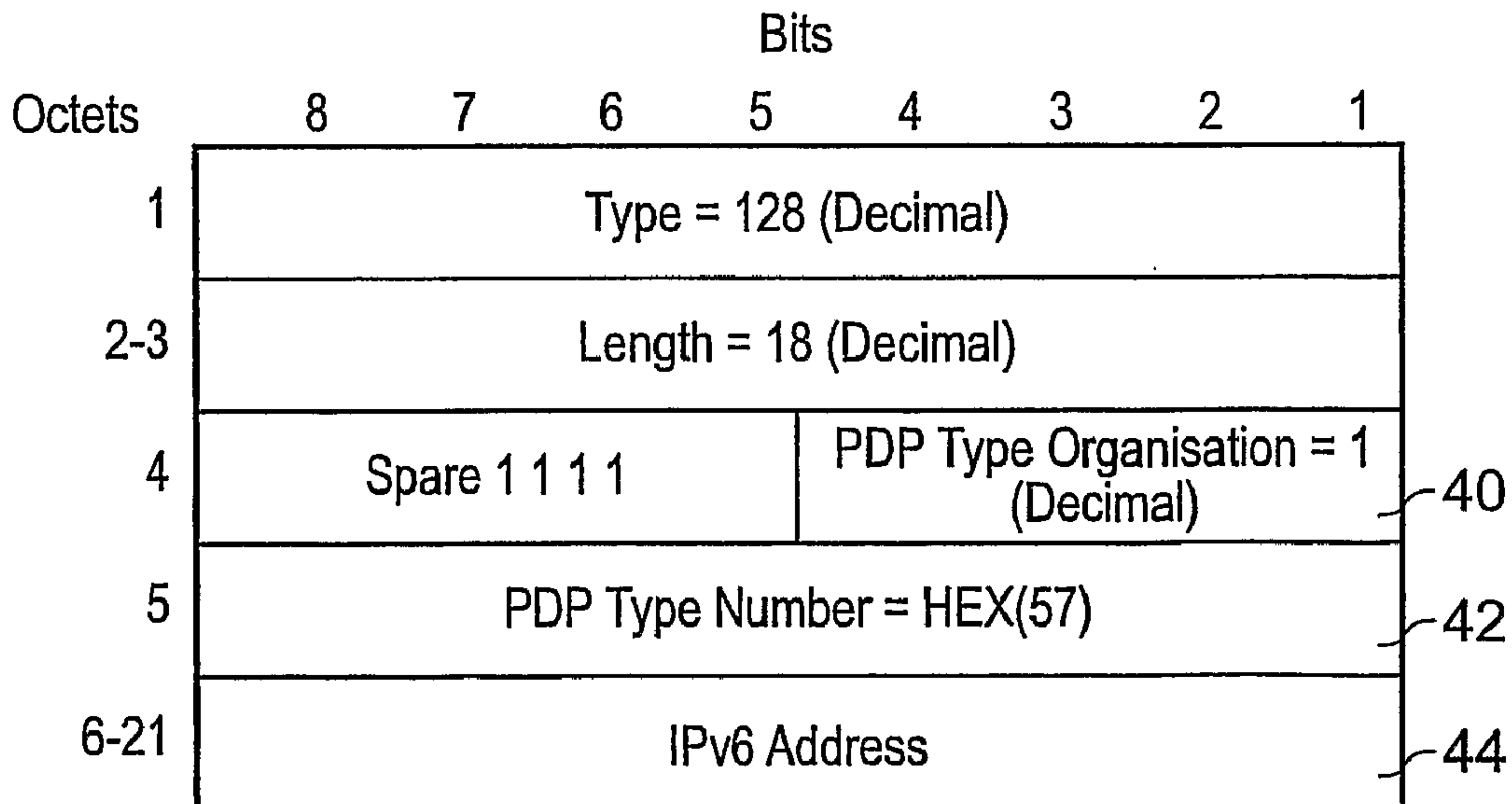
Fig. 9: End User Address Information Element for IPv6
