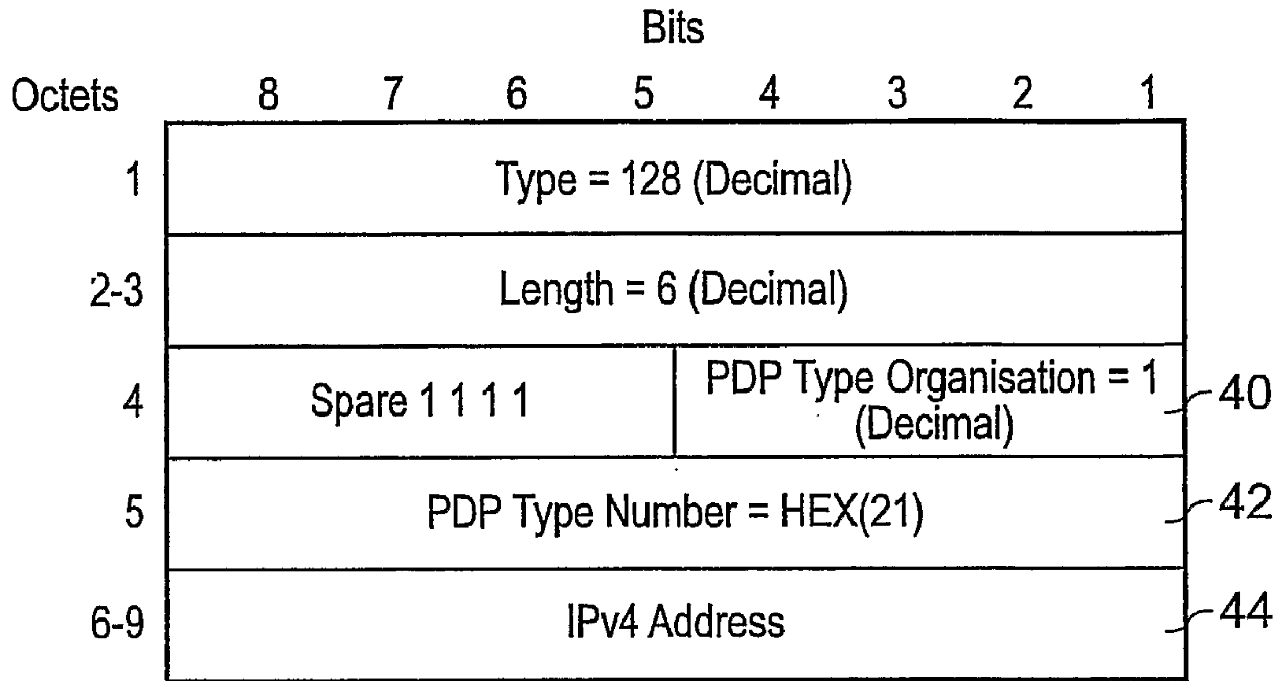
Fig. 8: End User Address Information Element for IPv4
