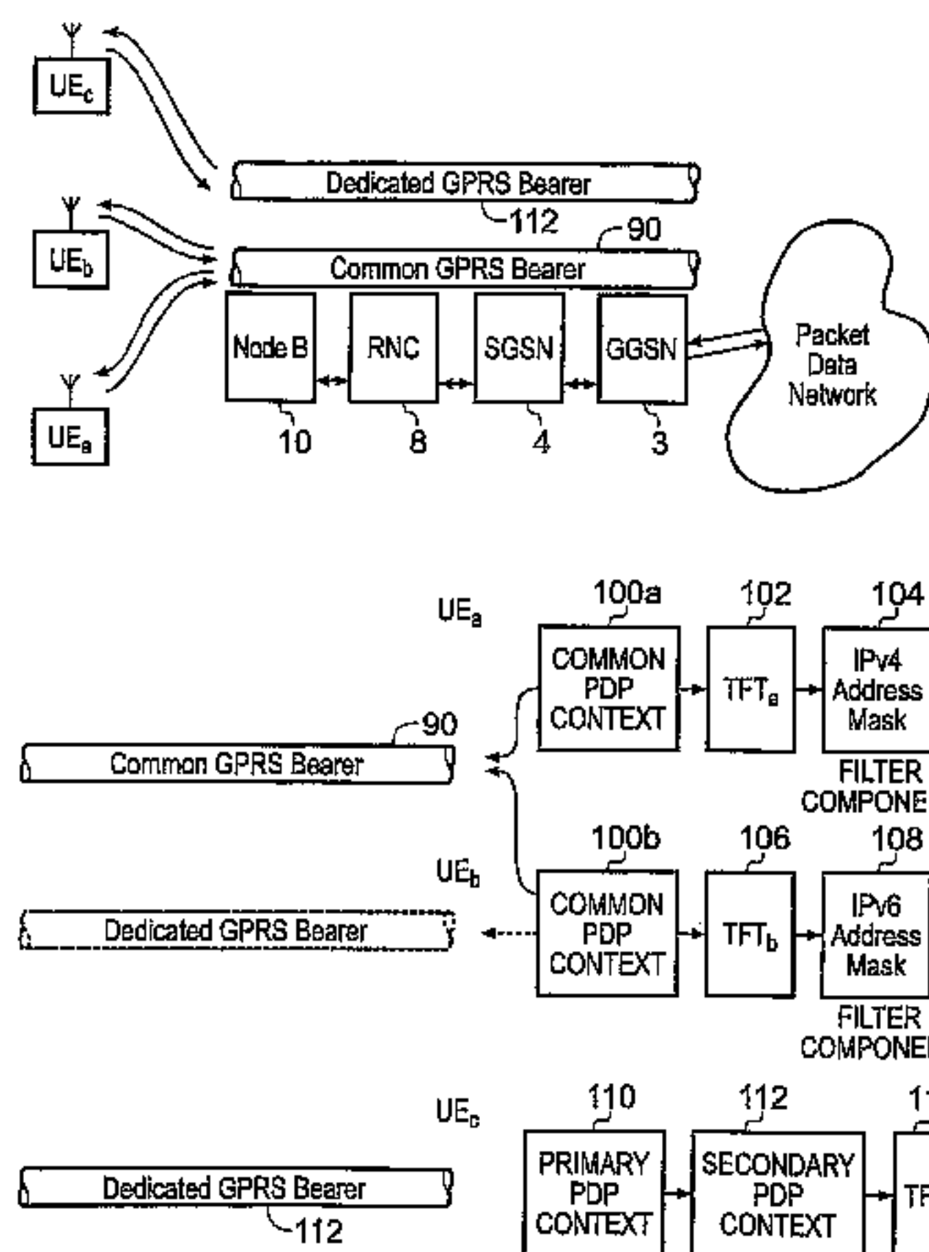
TFT for Common PDP Context
