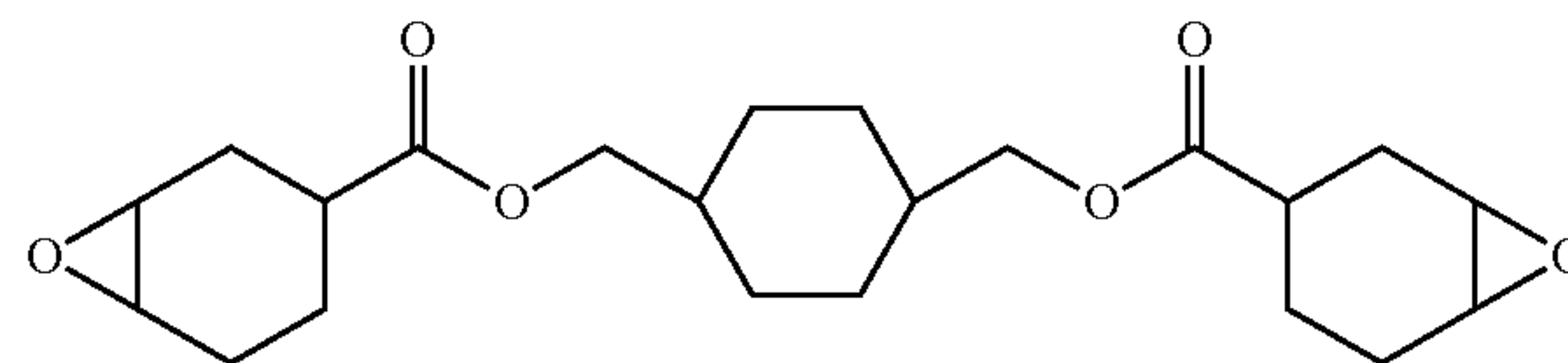
[Chemical Formula 4]
