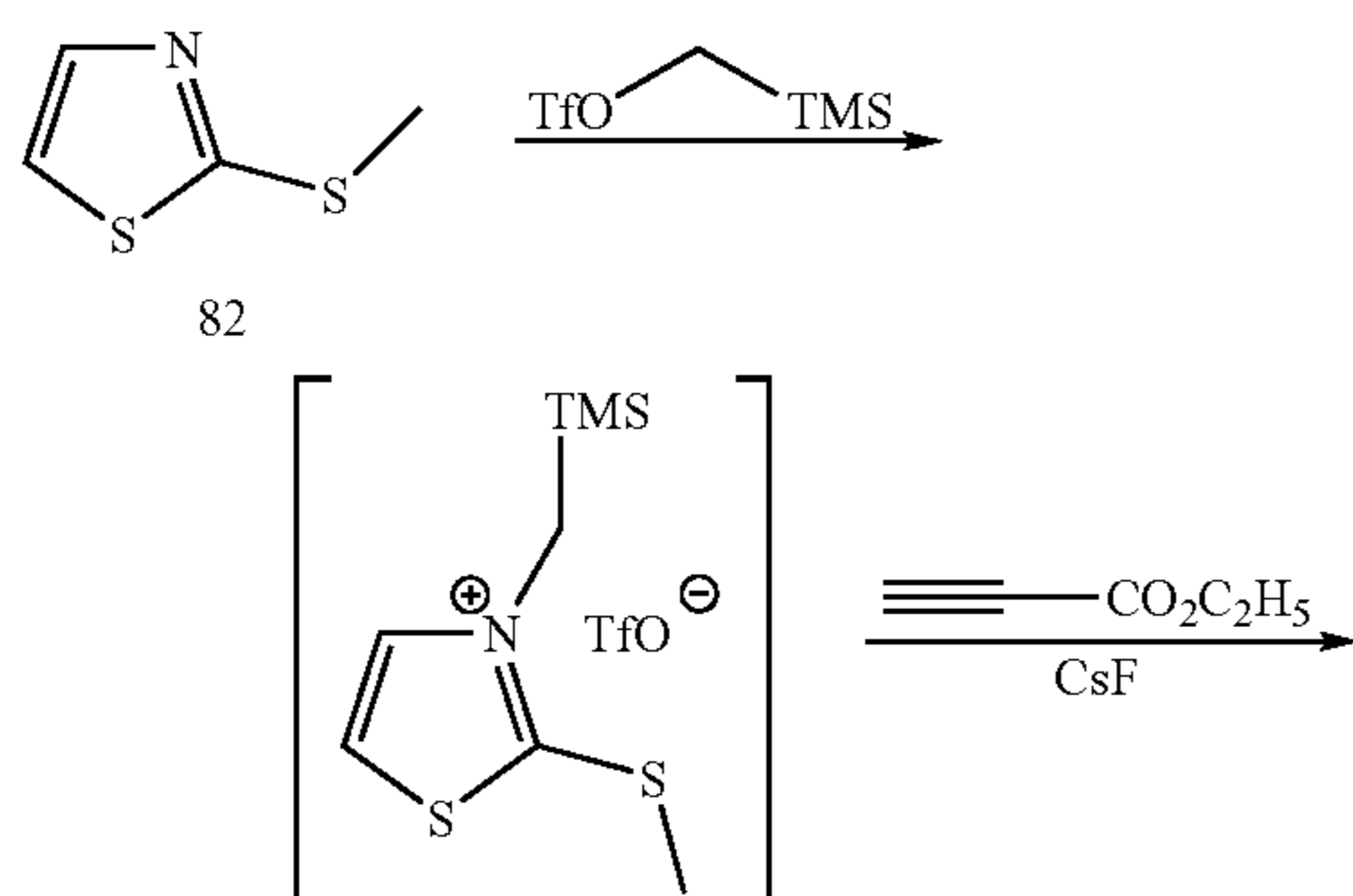
Scheme 11: Synthesis of pyrrolo[2,1-b]thiazole-carboxylic acid derivatives
