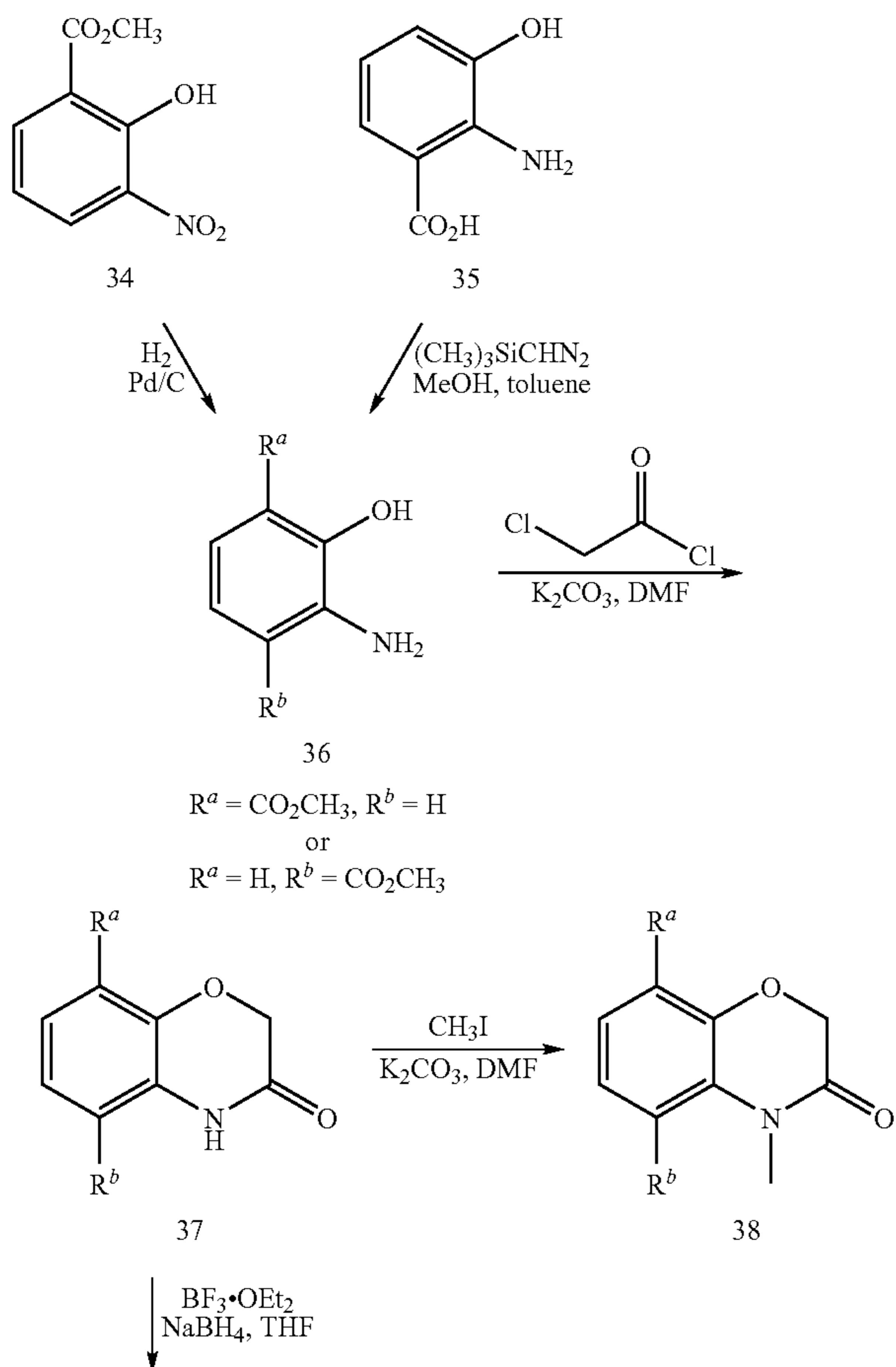
Scheme 8: Synthesis of benzo[1,4]oxazine-carboxylic acid derivatives
