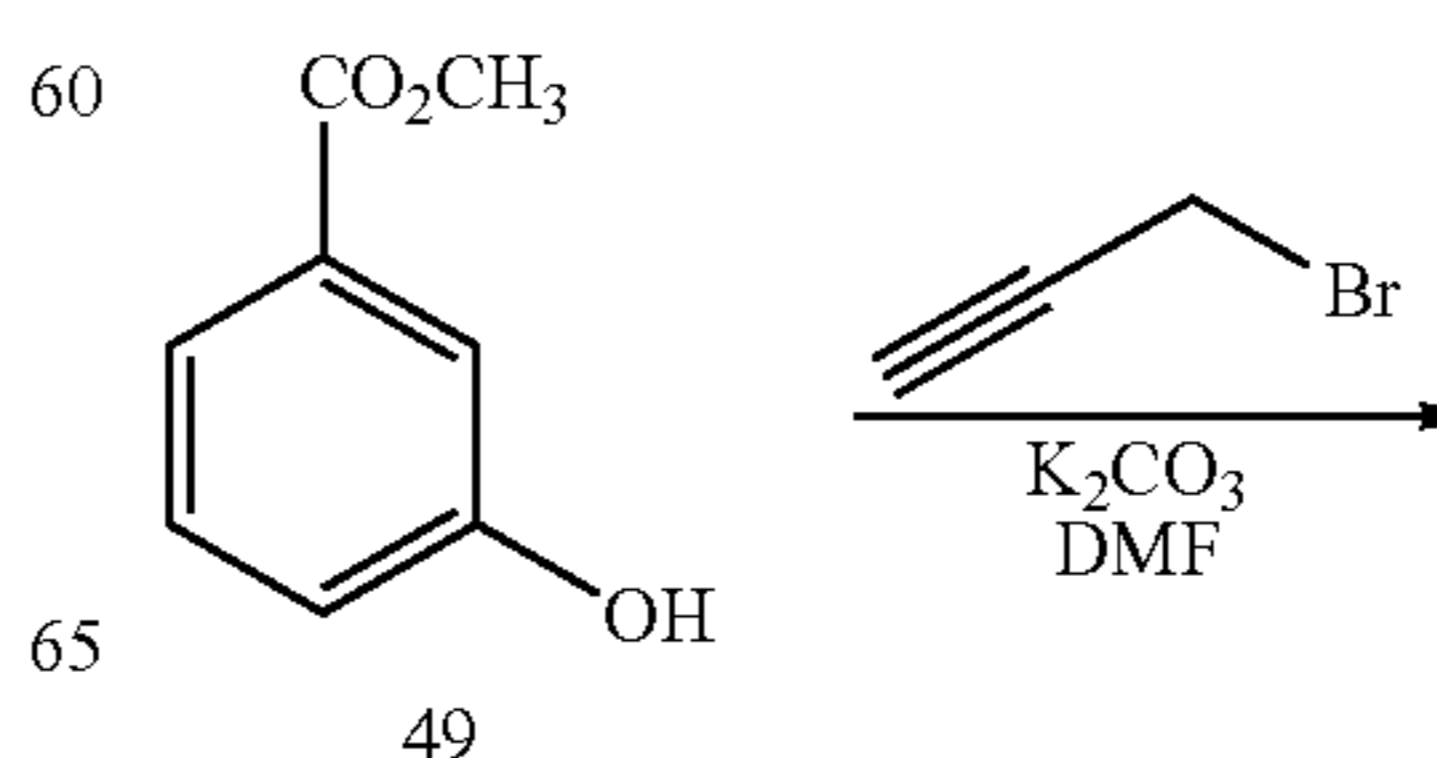
Scheme 9: Synthesis of chroman-carboxylic acid derivatives
