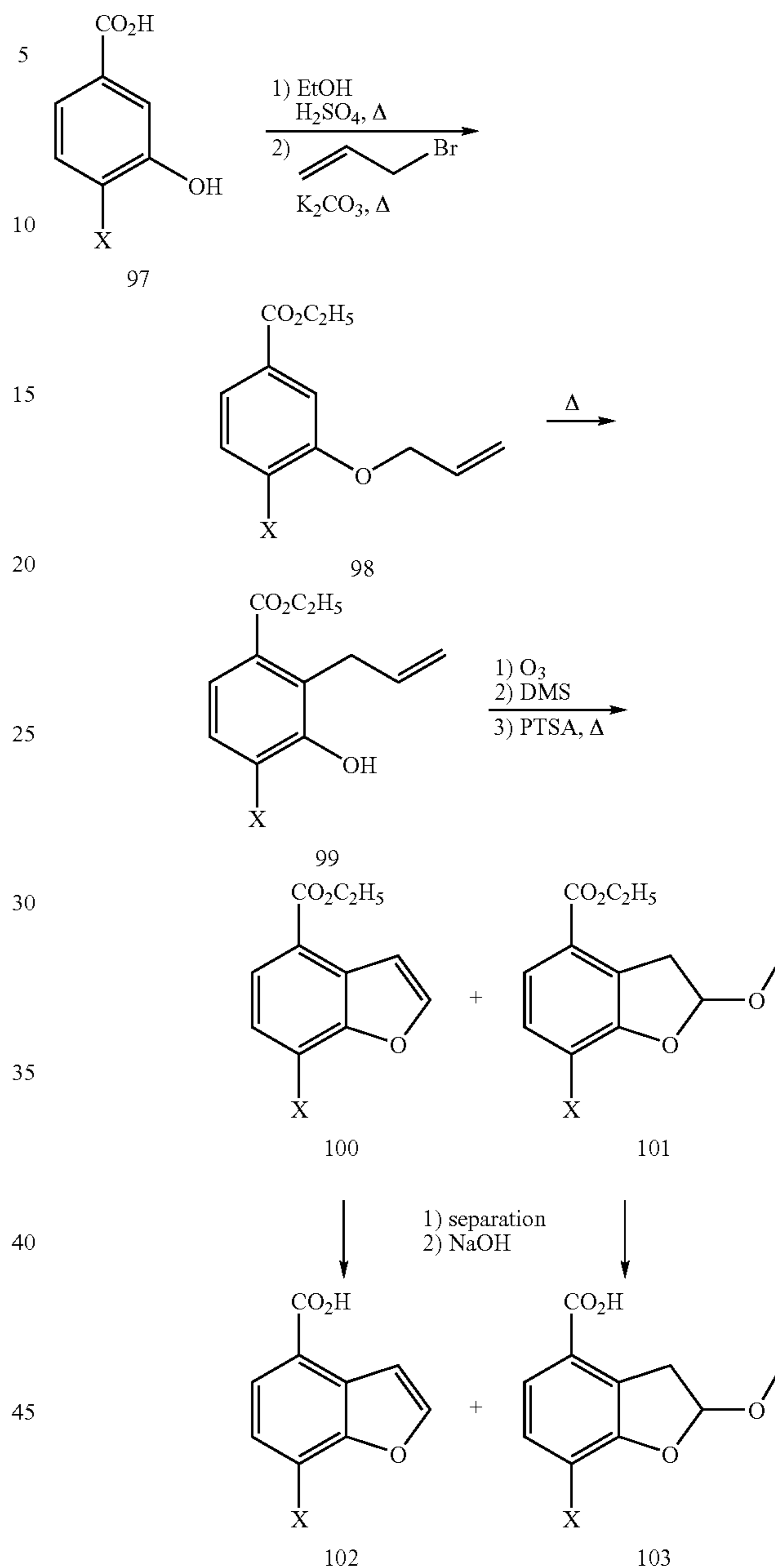
Scheme 14: Synthesis of benzofuran-carboxylic acid derivatives wherein X is fluorine or chlorine
