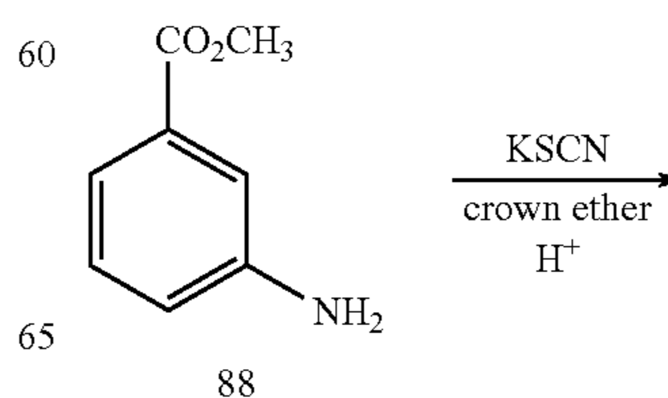
Scheme 12: Synthesis of benzothiazole-carboxylic acid derivatives
