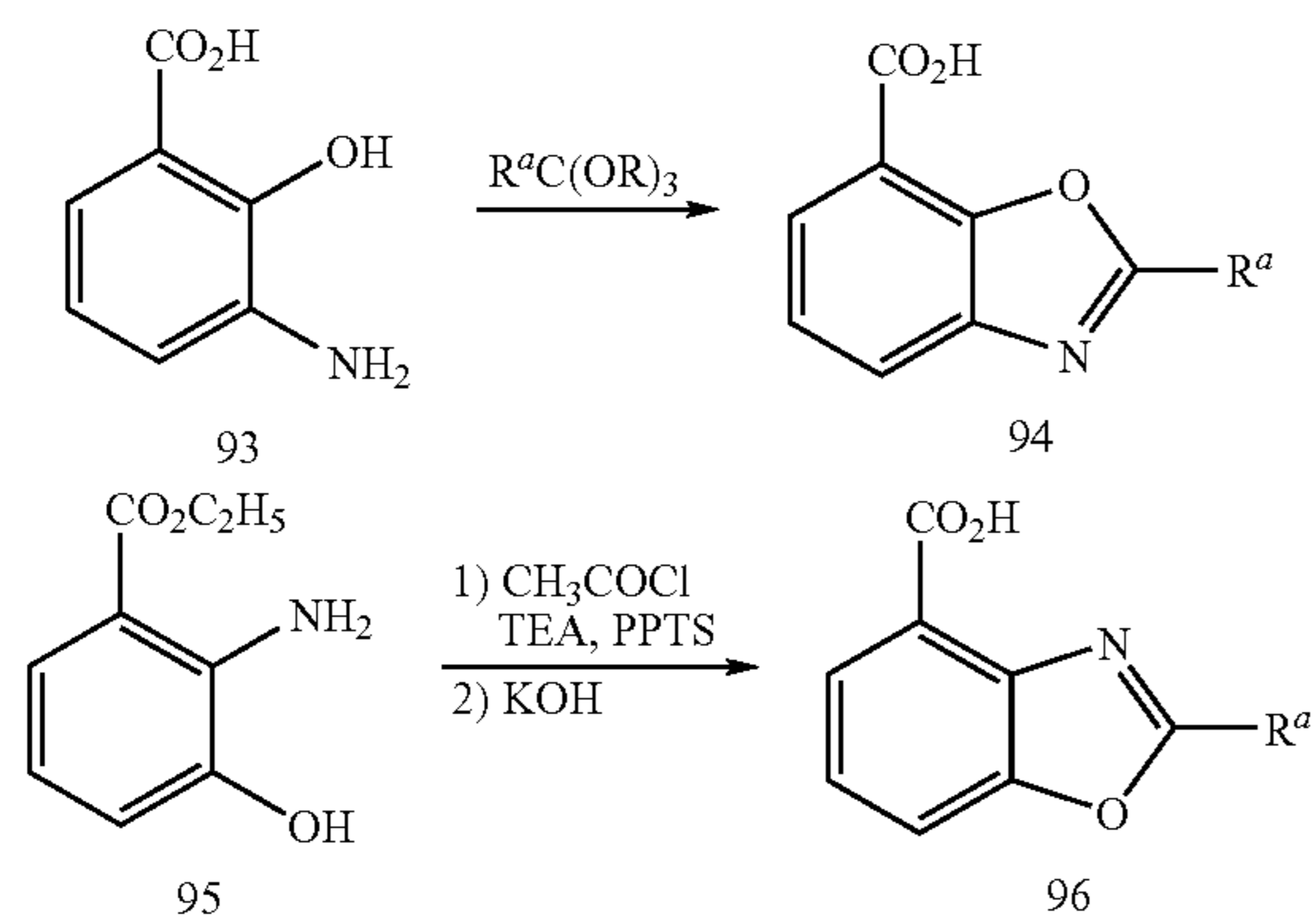
Scheme 13: Synthesis of benzoxazole-carboxylic acid derivatives wherein R is methyl or ethyl and R^a is hydrogen or methyl
