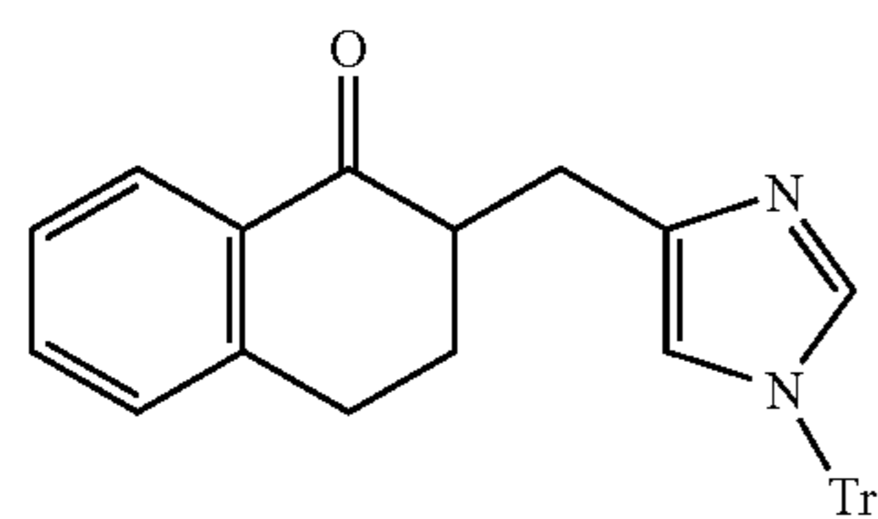
Intermediate TWENTYFIVE-1
