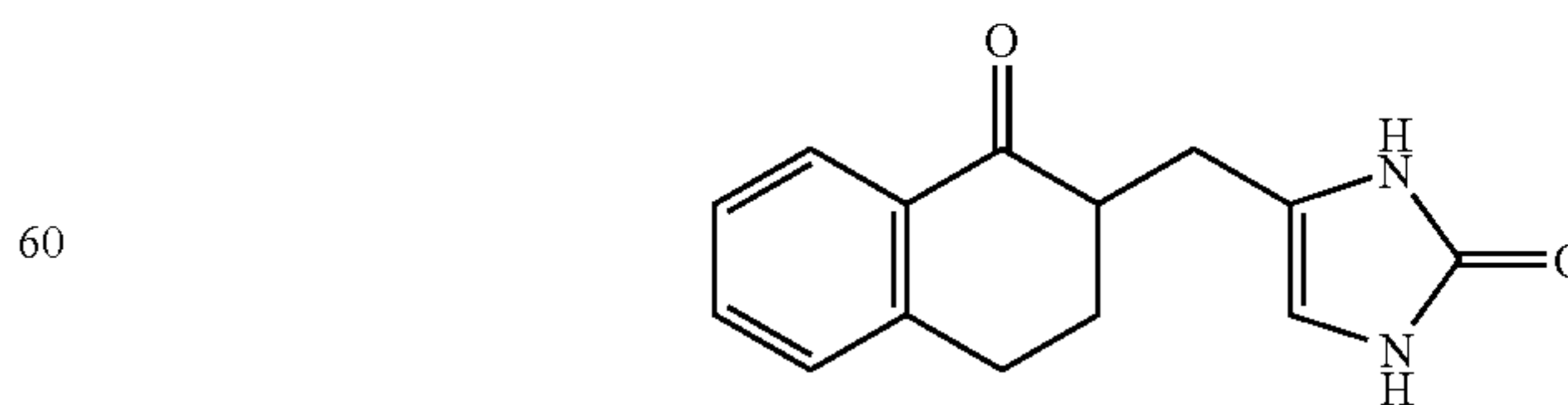
Compound 54
