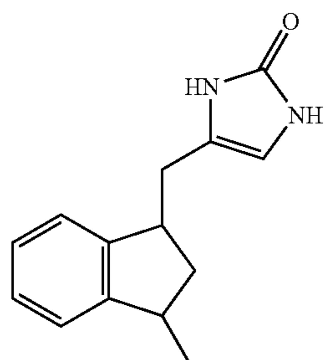
Compound 47
