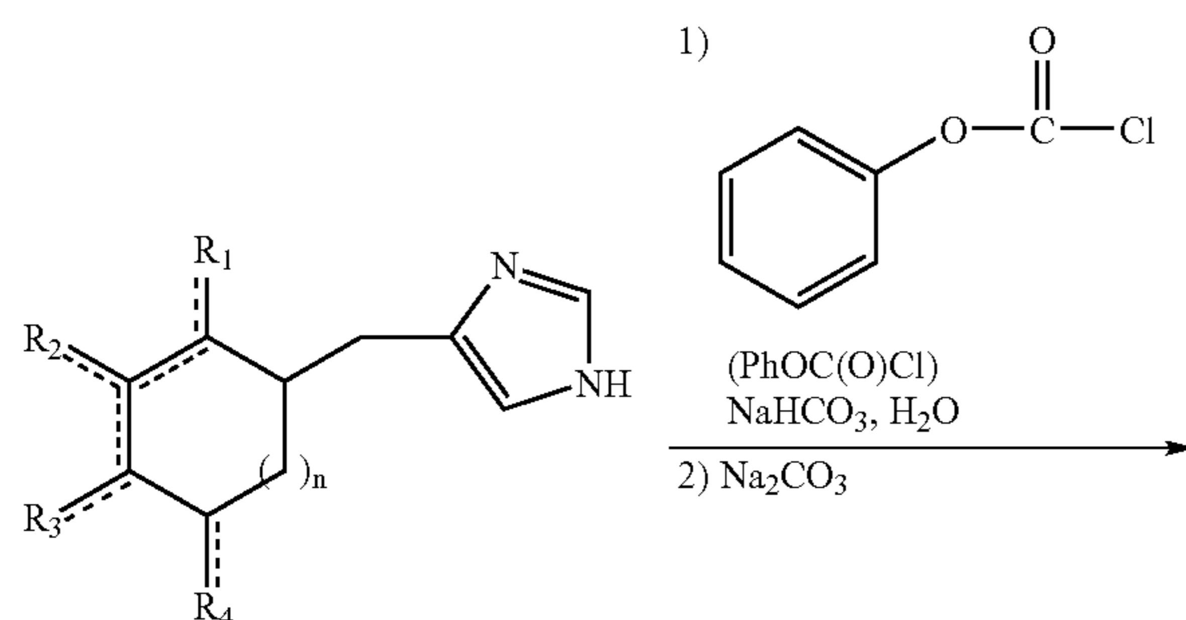
fumarate Formula 5
