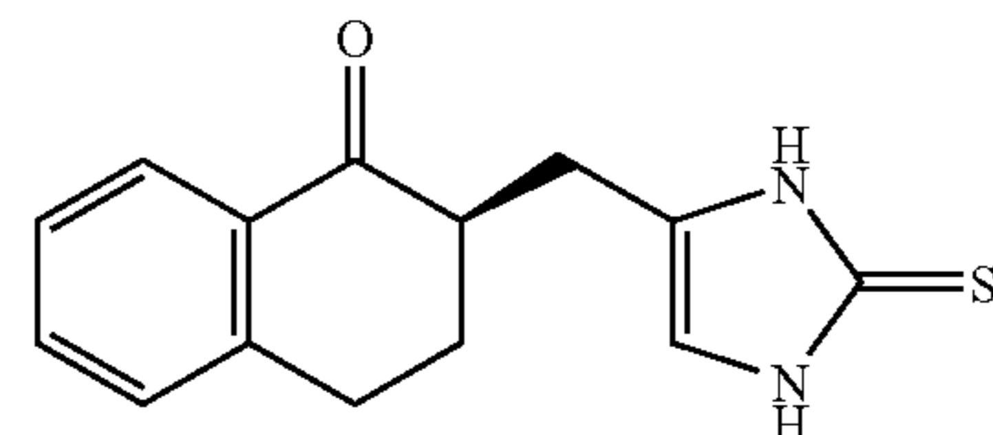
(+) - R Compound 24
