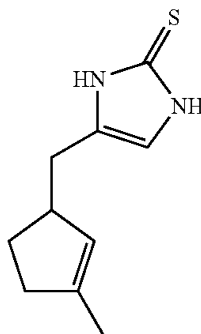
Compound 2
