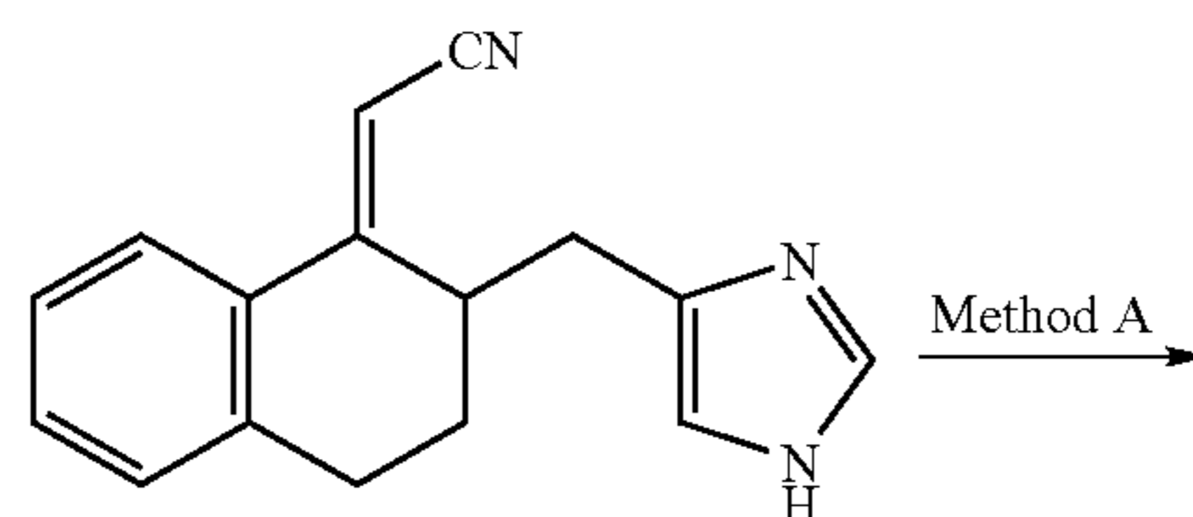
Intermediate TWENTYFIVE-2
