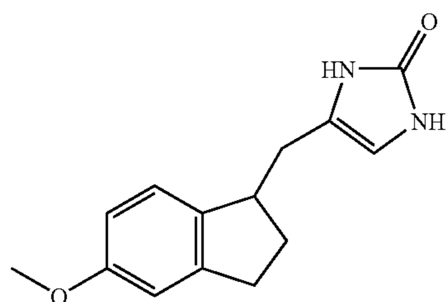
Compound 50
