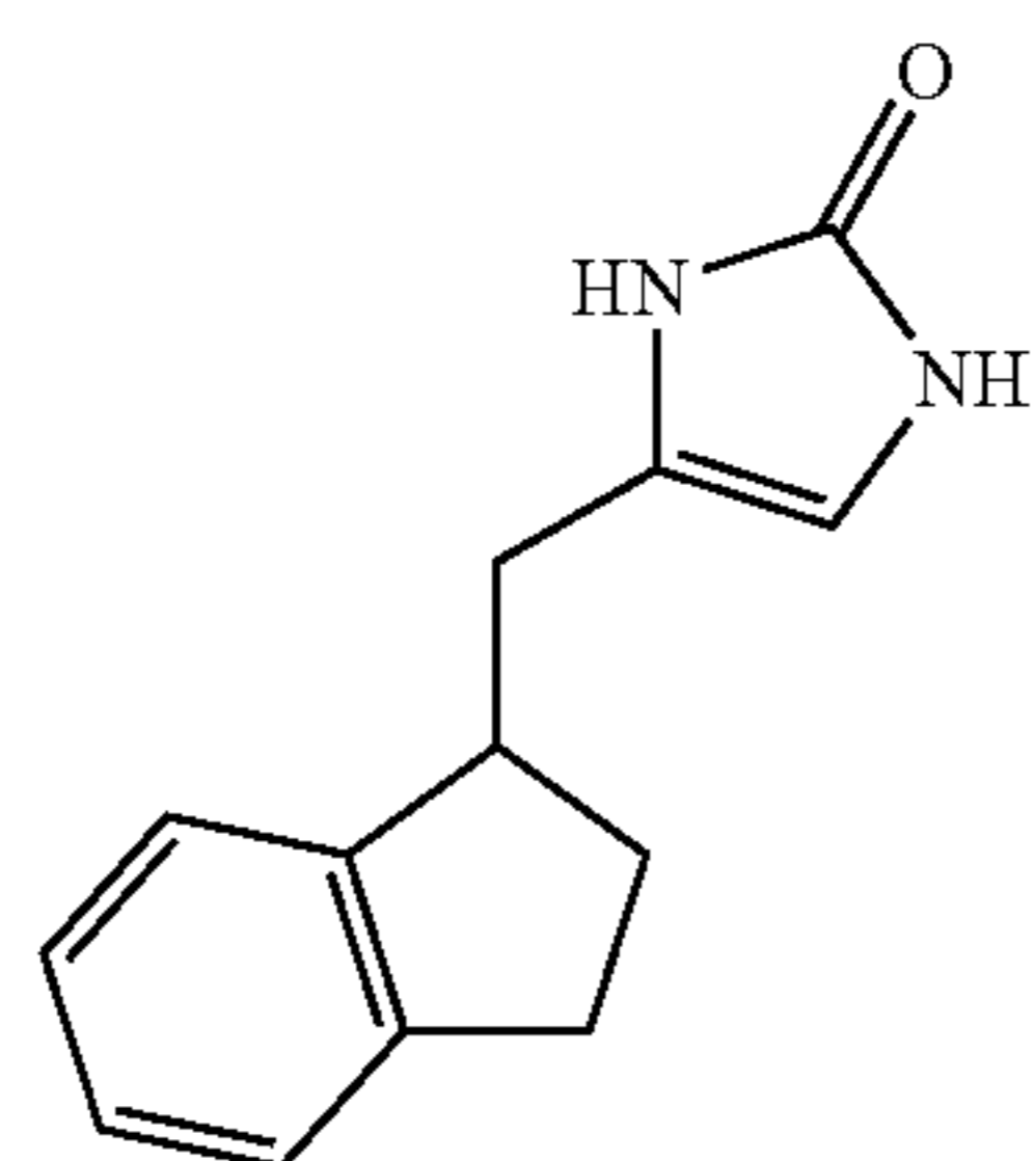
Compound 46
