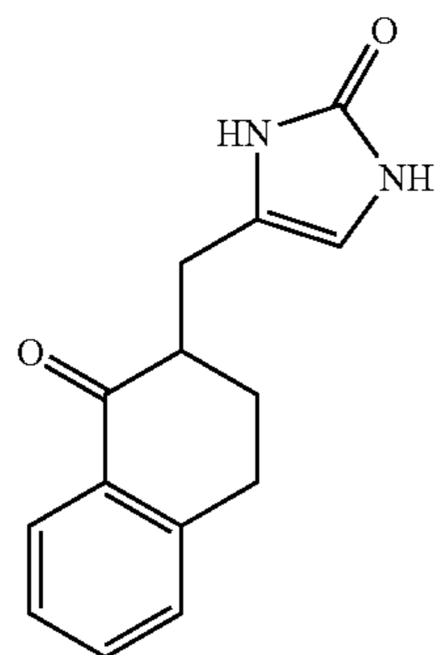
Compound 54
