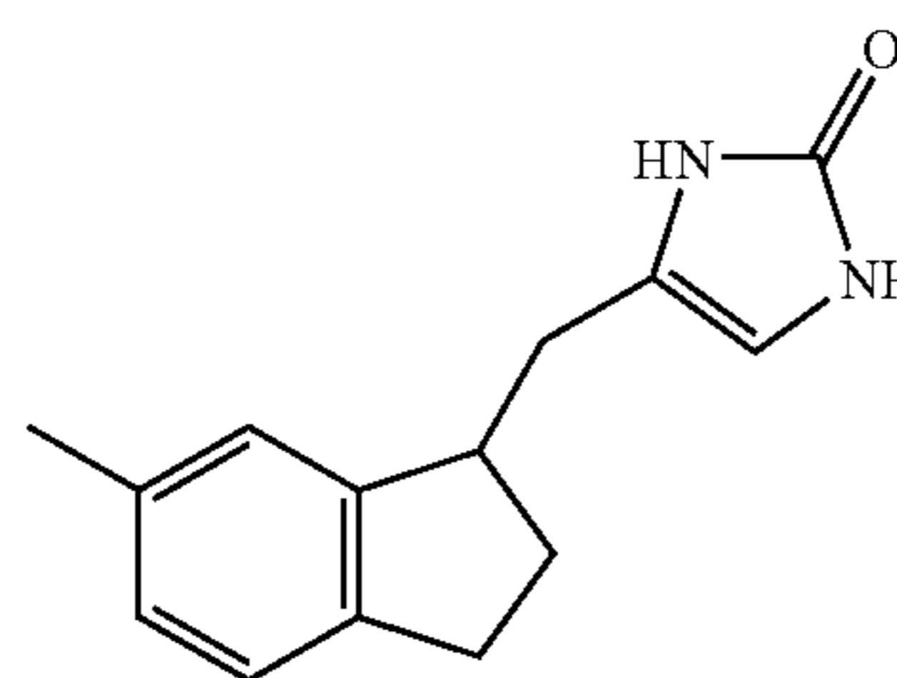
Compound 52
