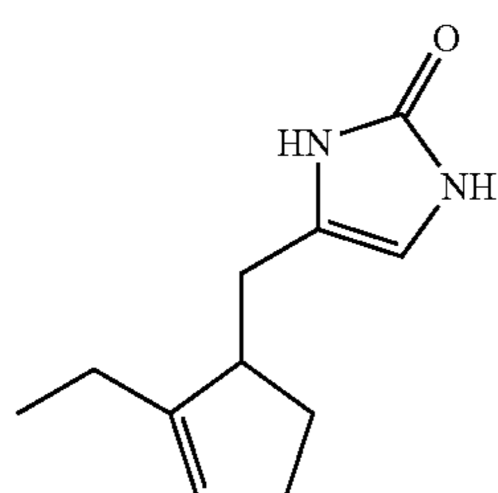
Compound 43
