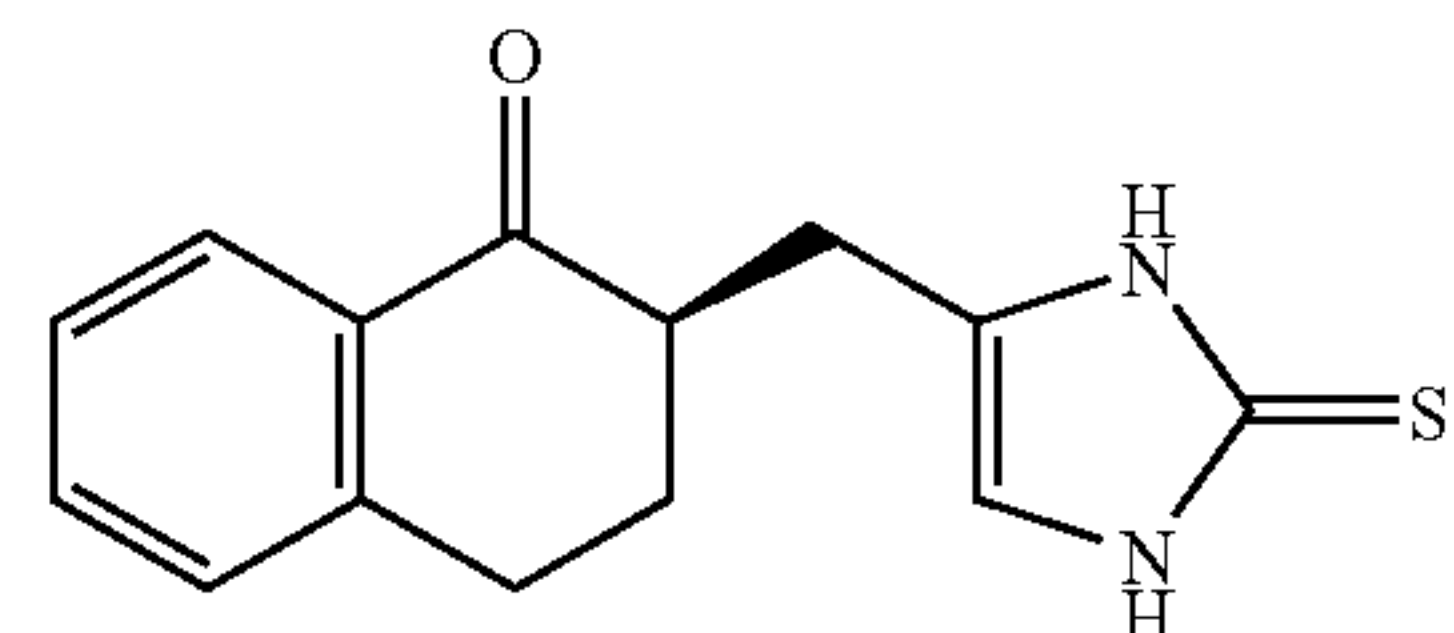
(+) - R Compound 24
