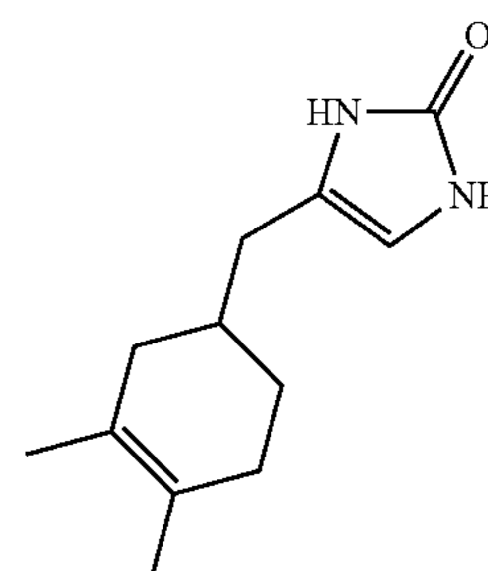
Compound 60
