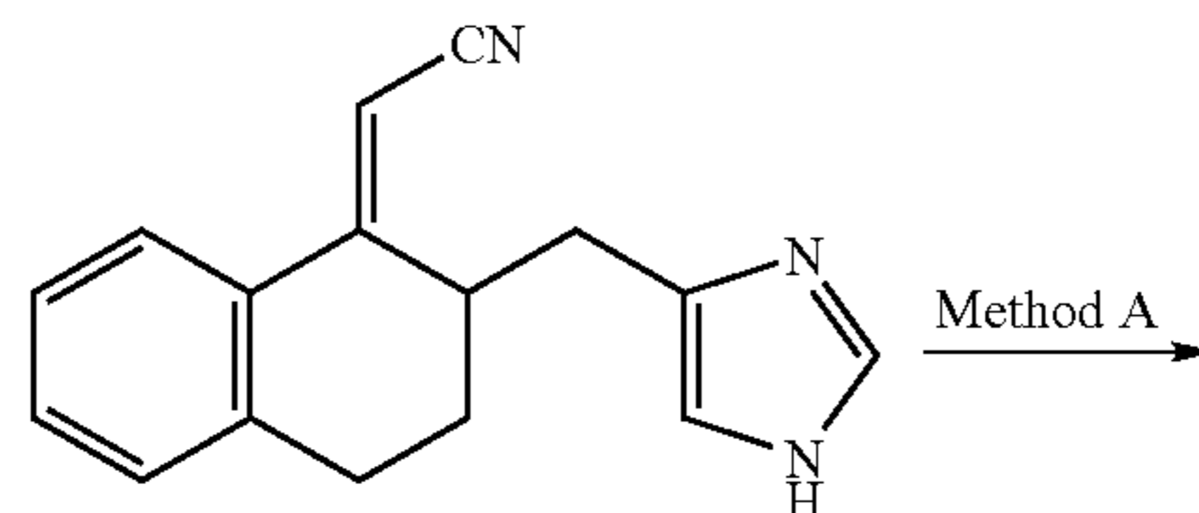
Intermediate TWENTYFIVE-2
