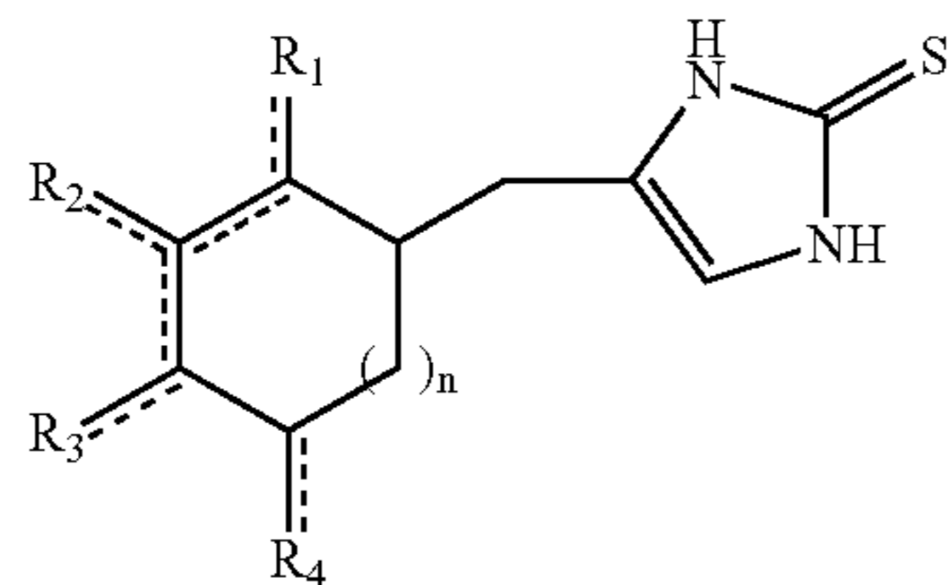
Formula 6
