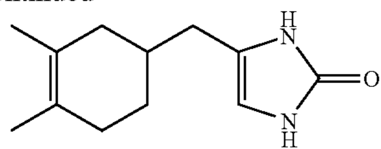
Compound 60
