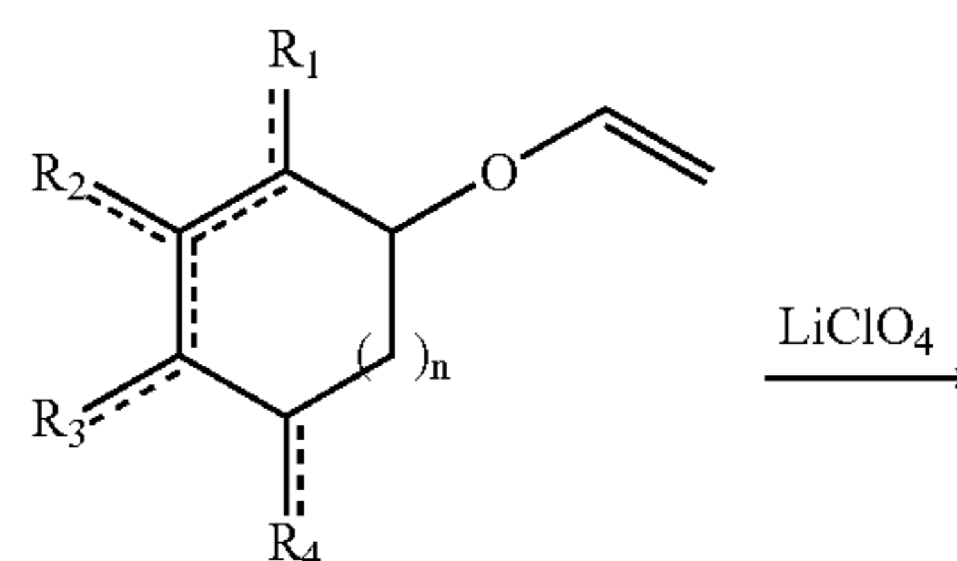
Formula 3
