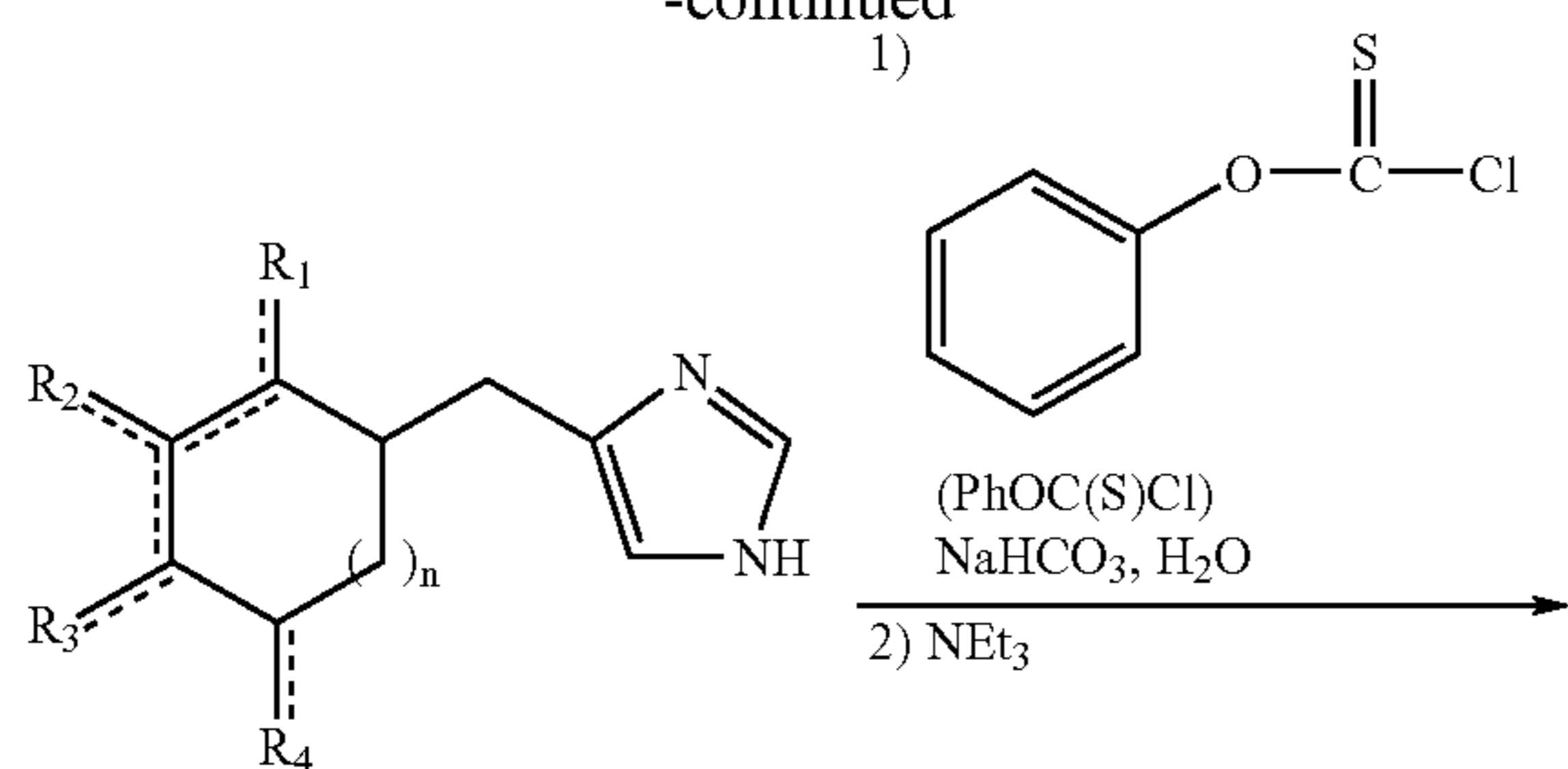
Formula 5
