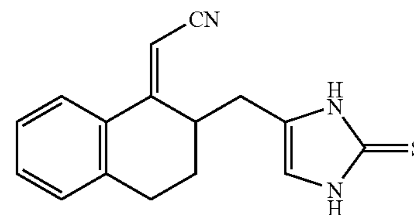
Compound 170
