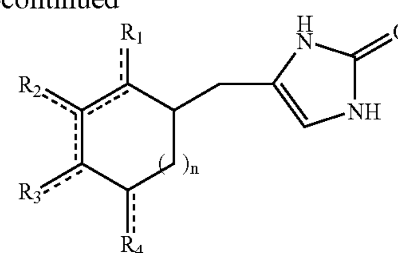
Formula 16
