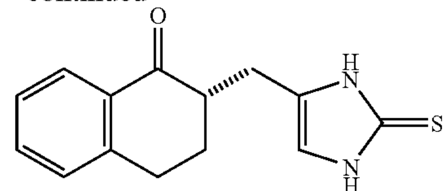
(-) - S Compound 23
