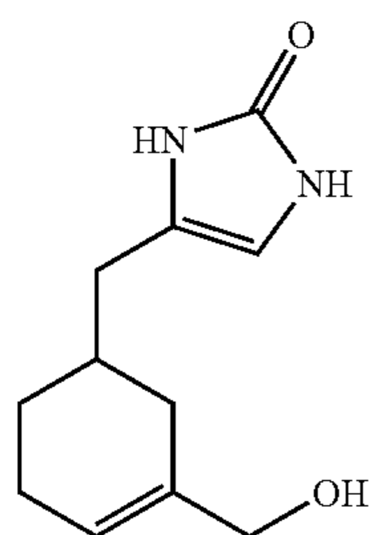
Compound 56
