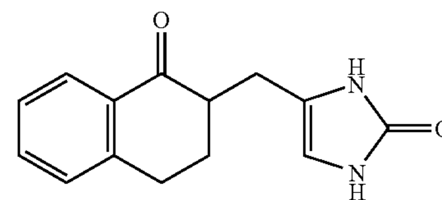
Compound 54
