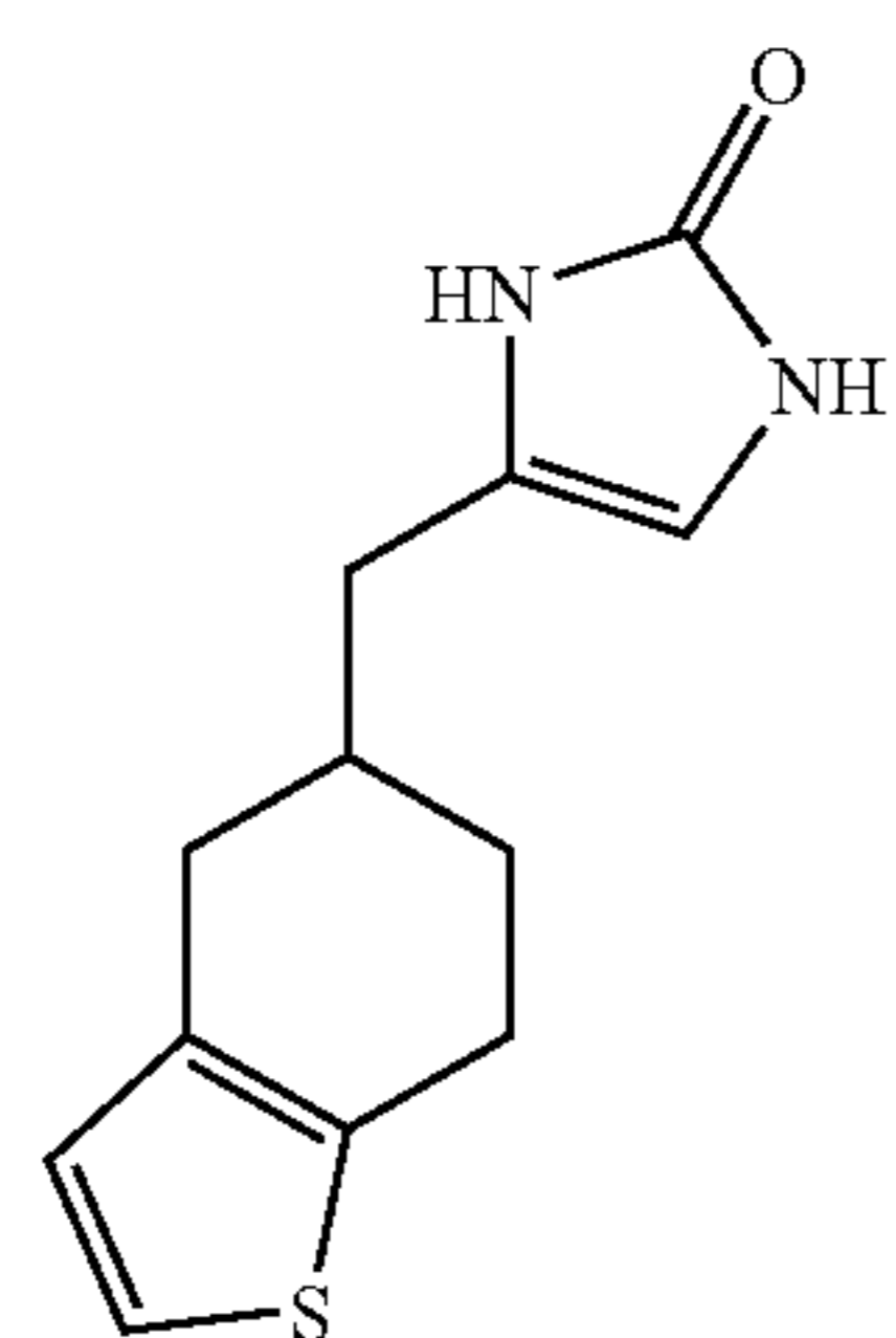
Compound 55
