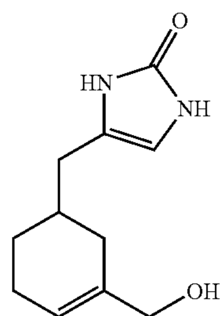
Compound 56
