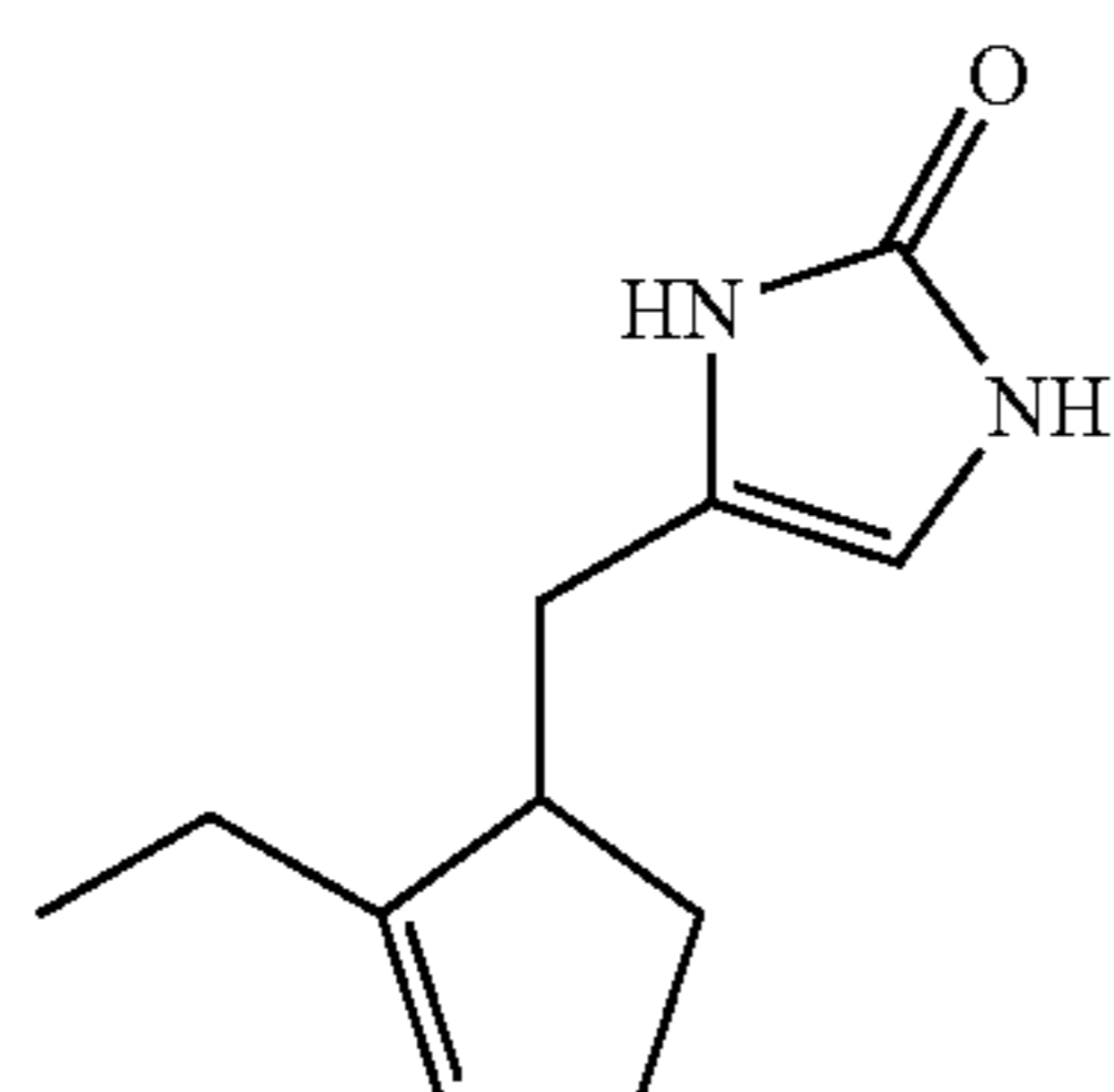
Compound 43
