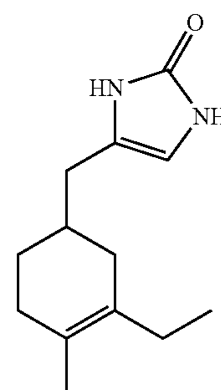
Compound 58
