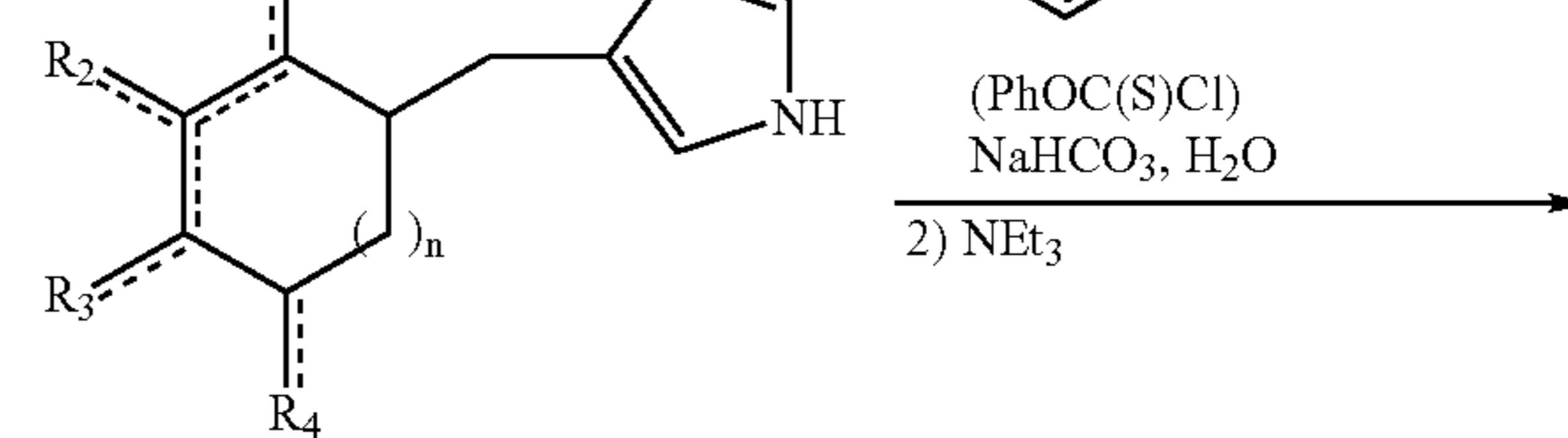
Formula 5
