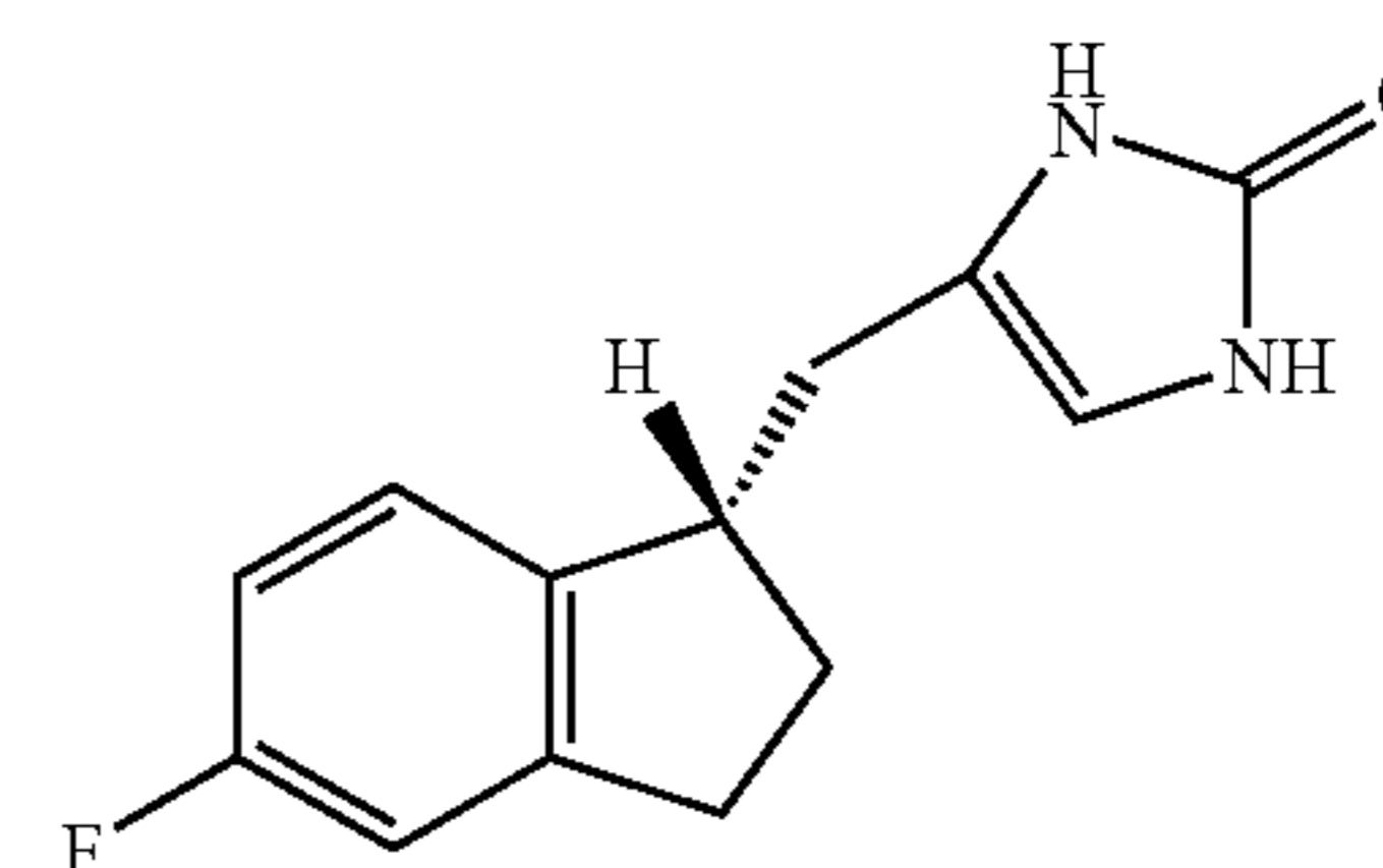
(-) (S) Compound 62
