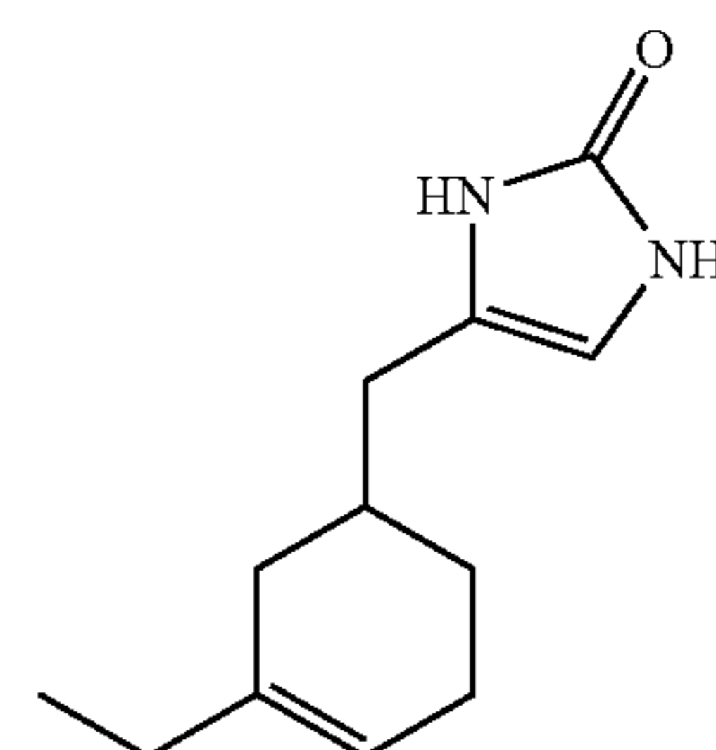
Compound 59
