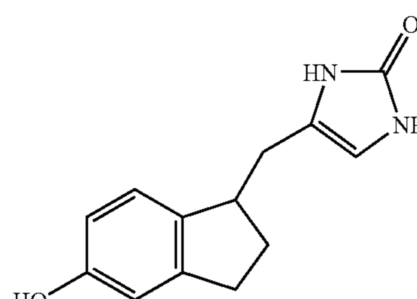
Compound 63
