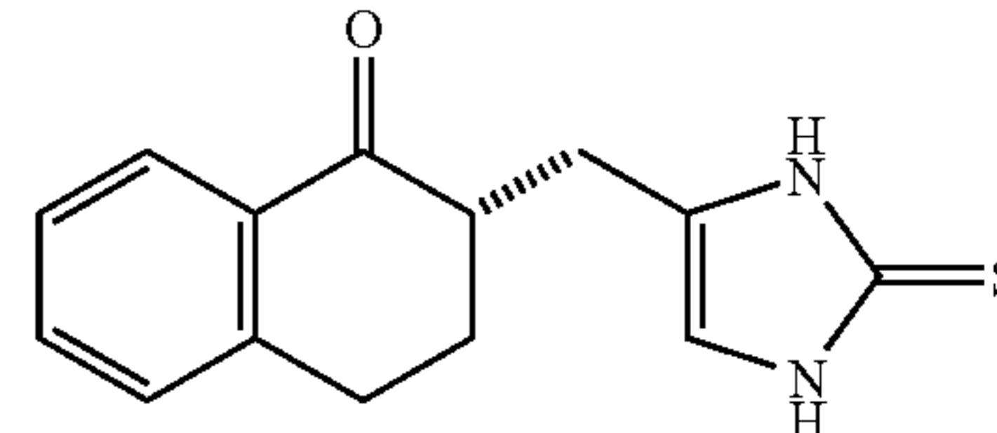
(-) - S Compound 23
