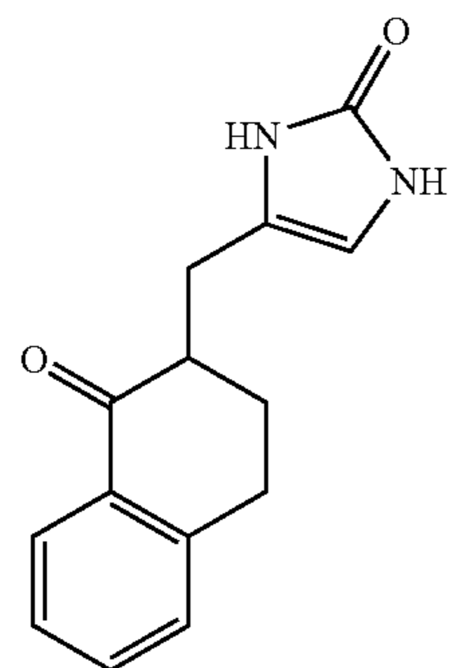
Compound 54
