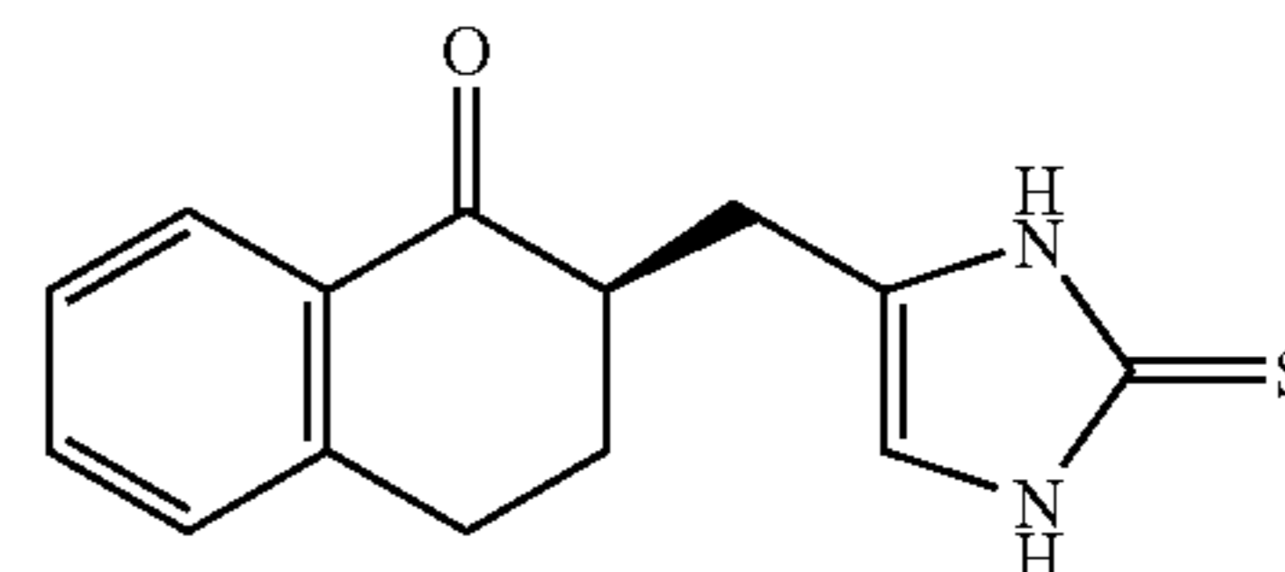
(+) - R Compound 24
