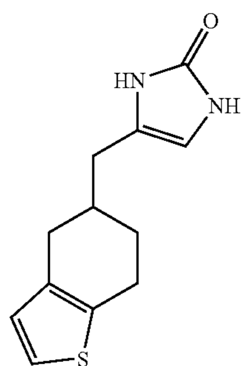
Compound 55
