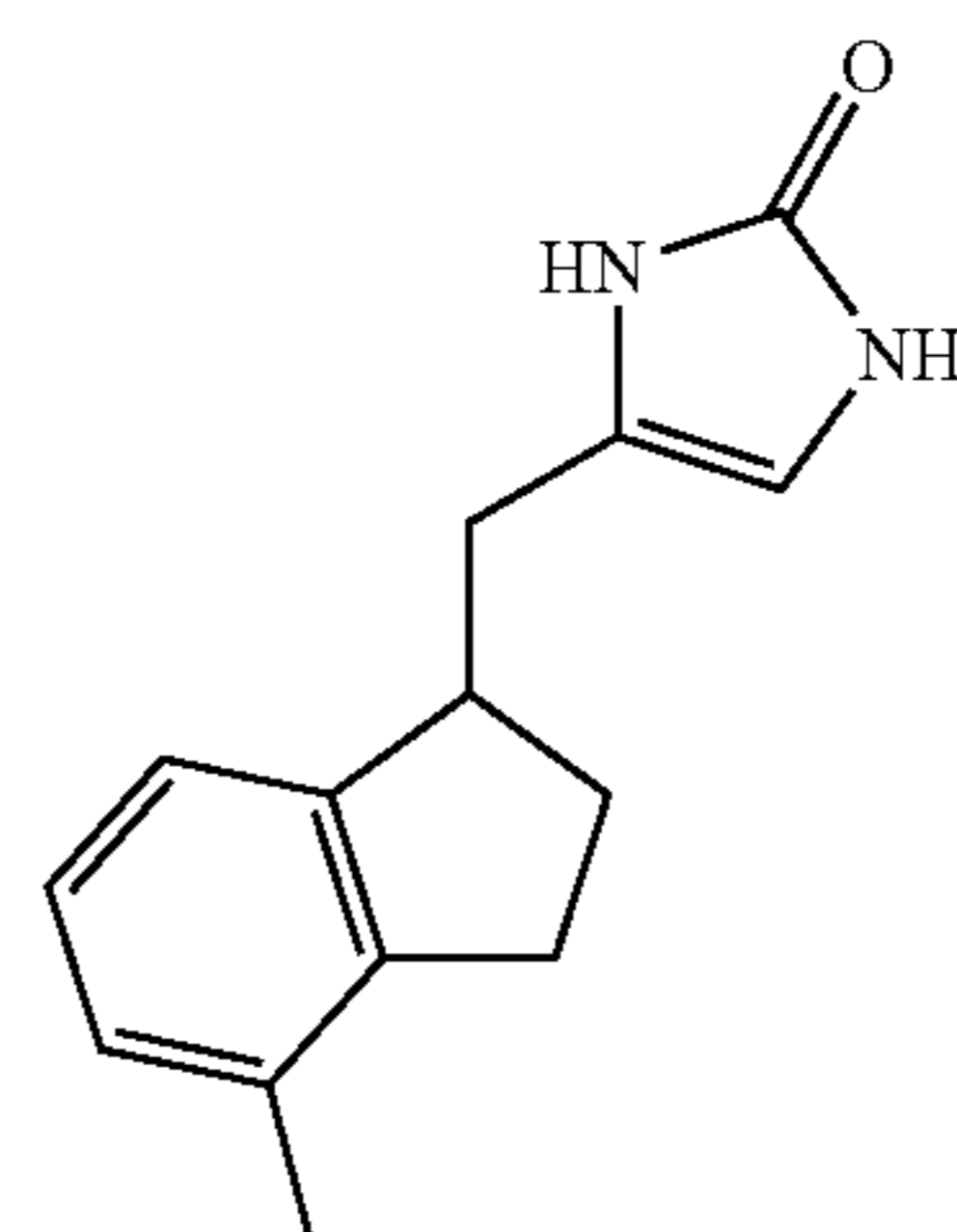
Compound 48
