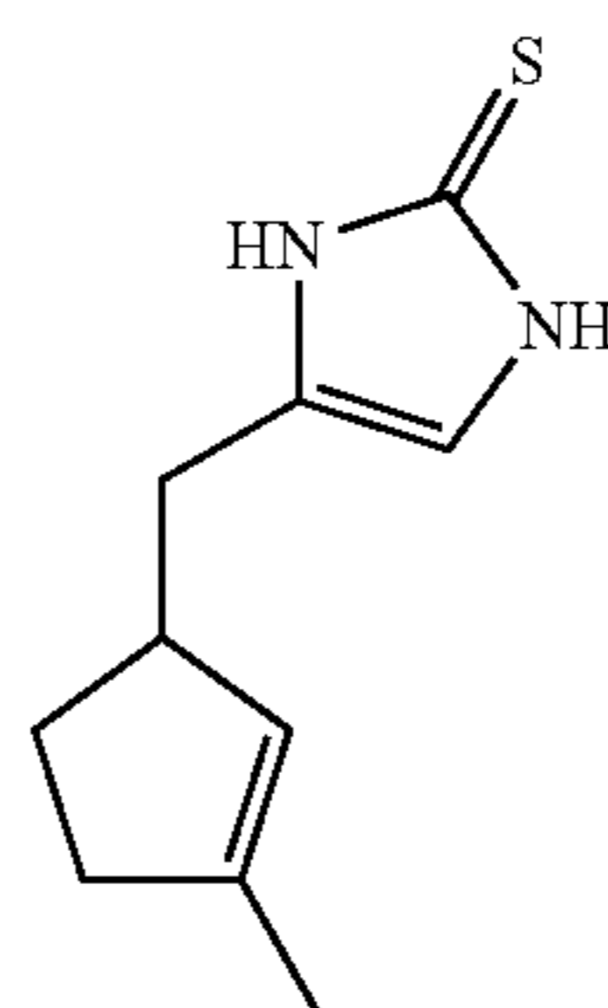
Compound 2
