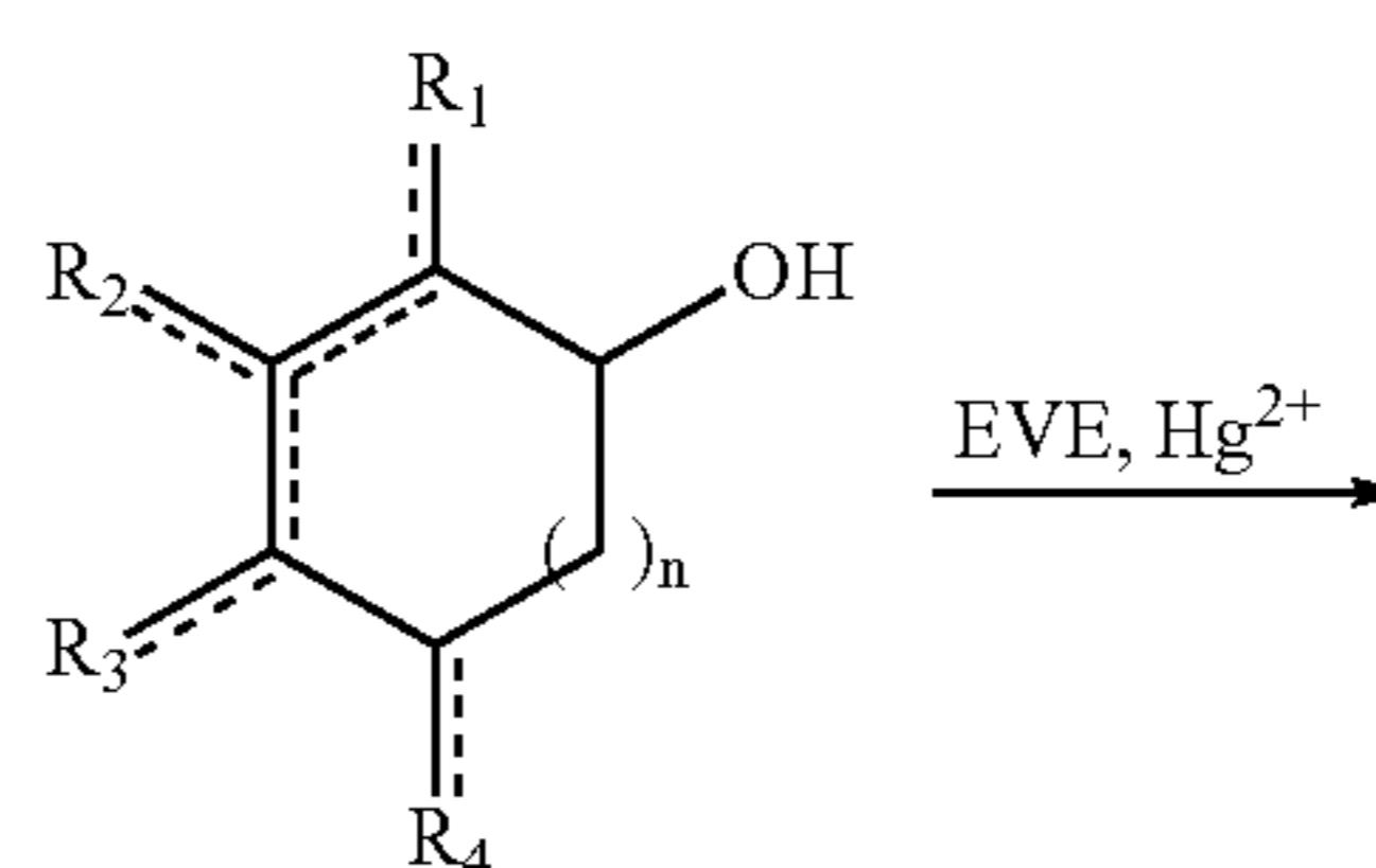
Formula 2A
