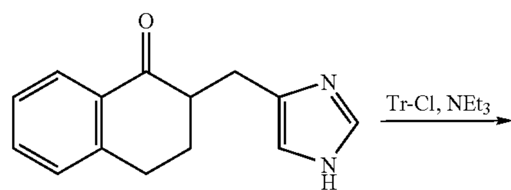
Intermediate E4
