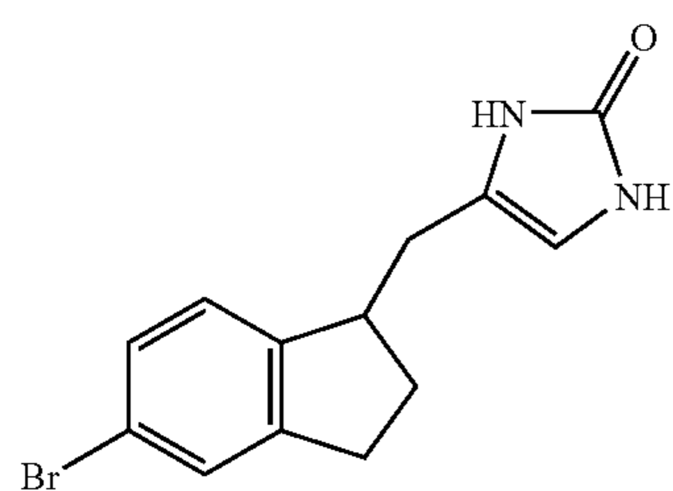
Compound 51
