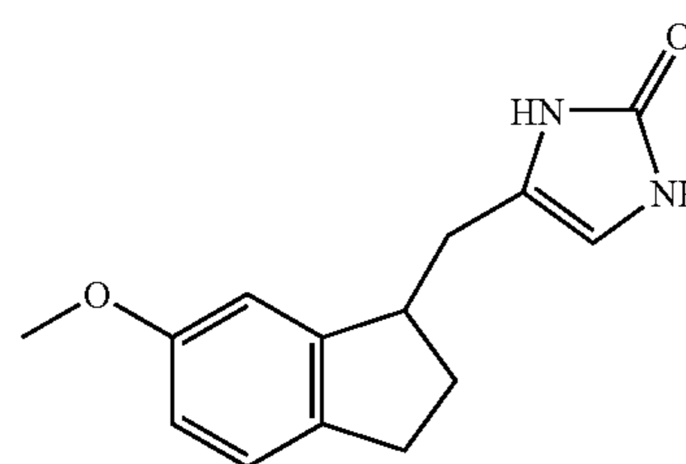
Compound 53
