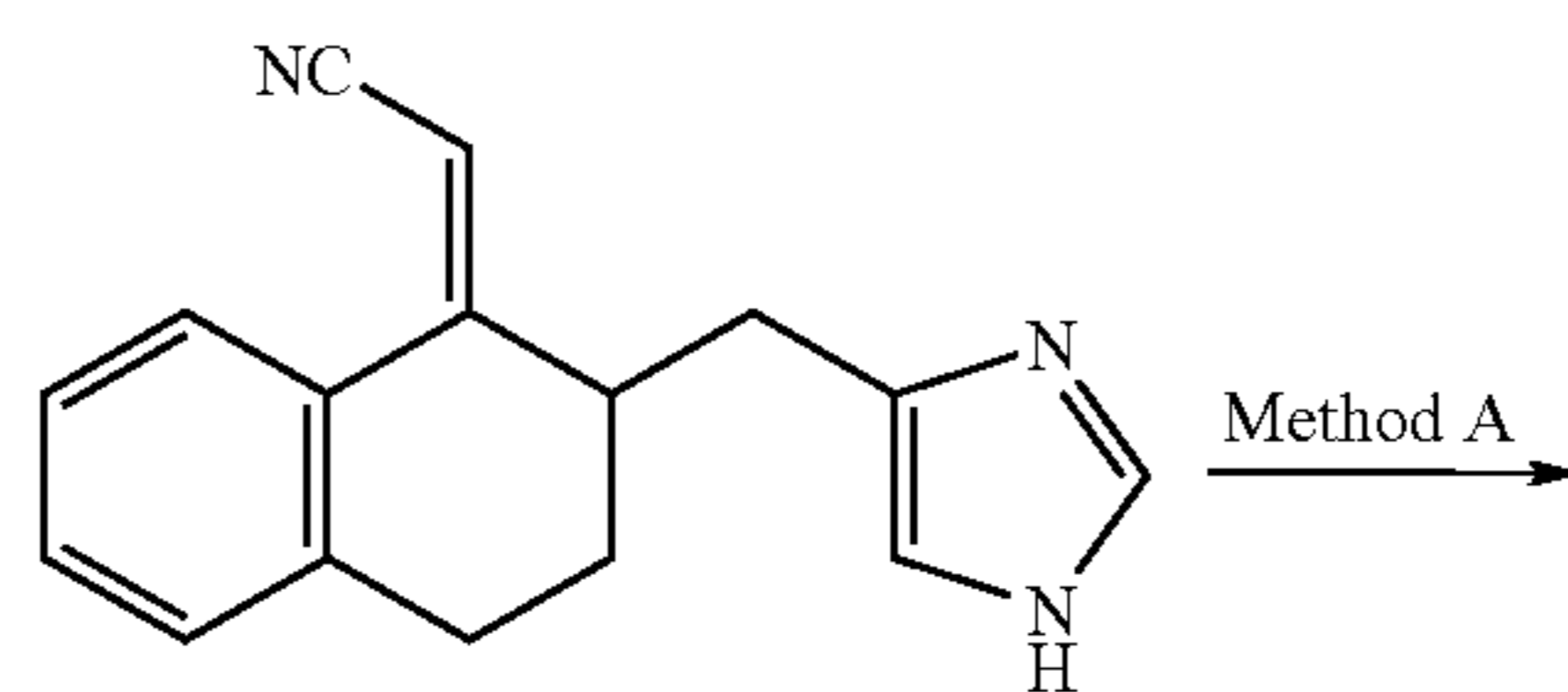
Intermediate TWENTYFIVE-3
