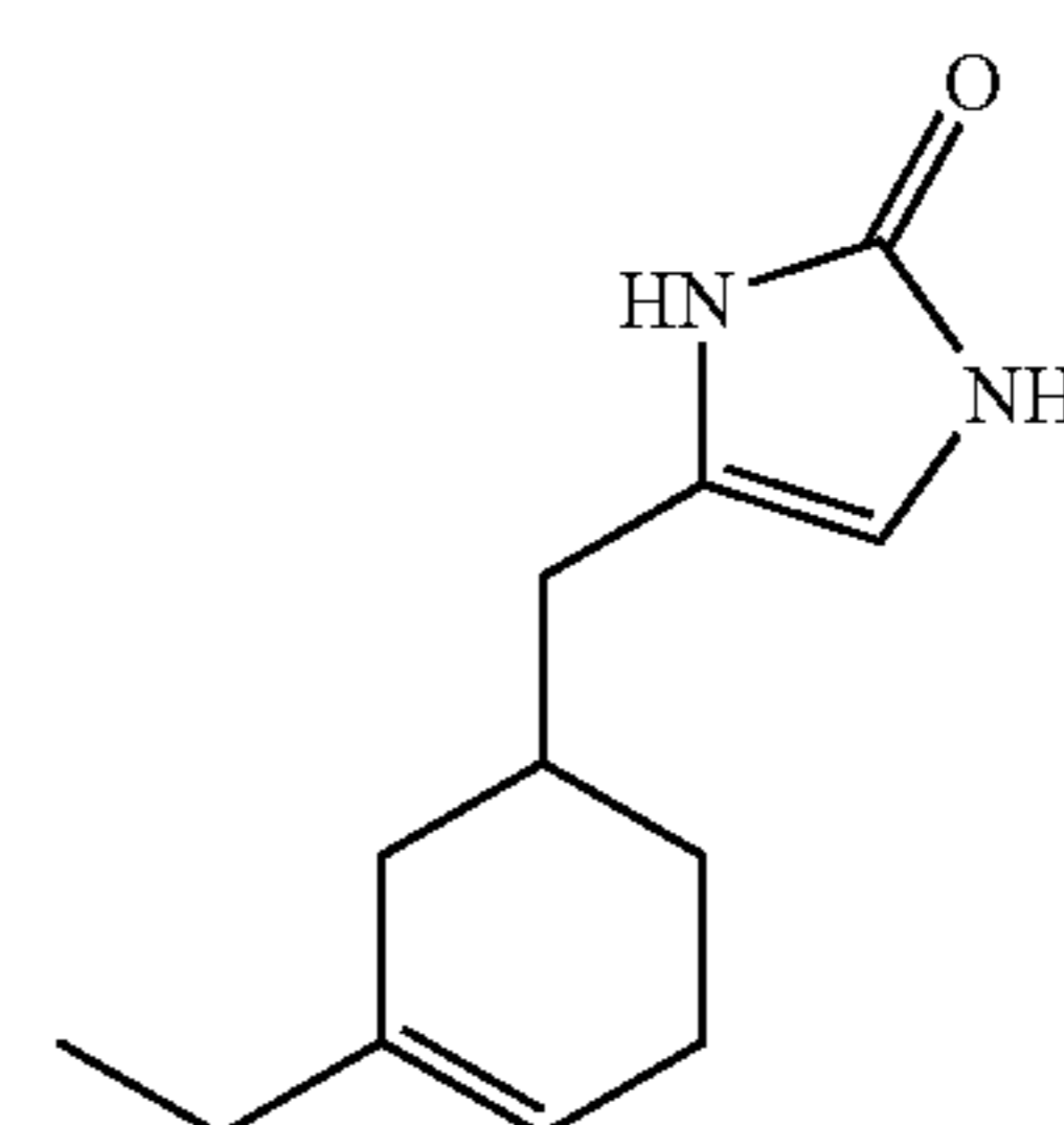
Compound 59
