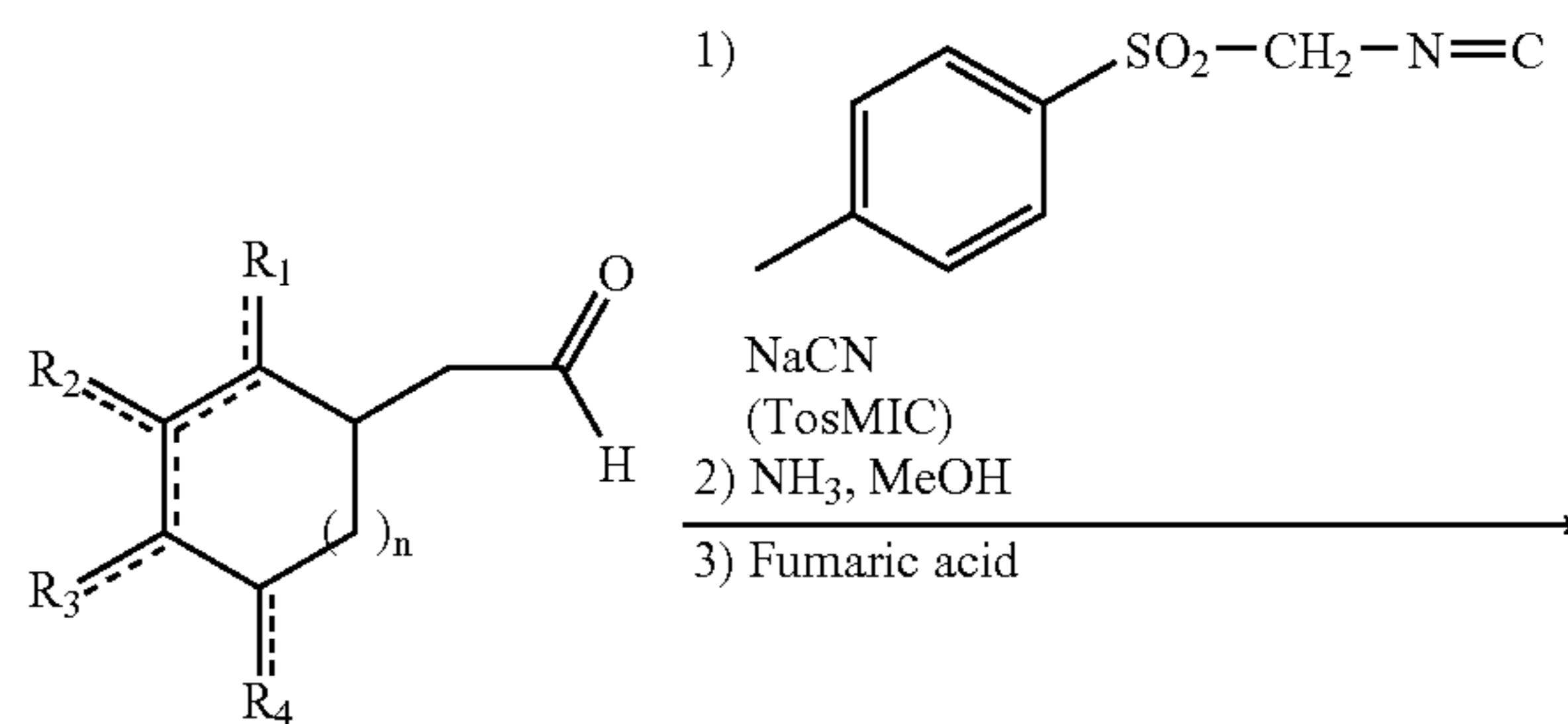
Formula 4
