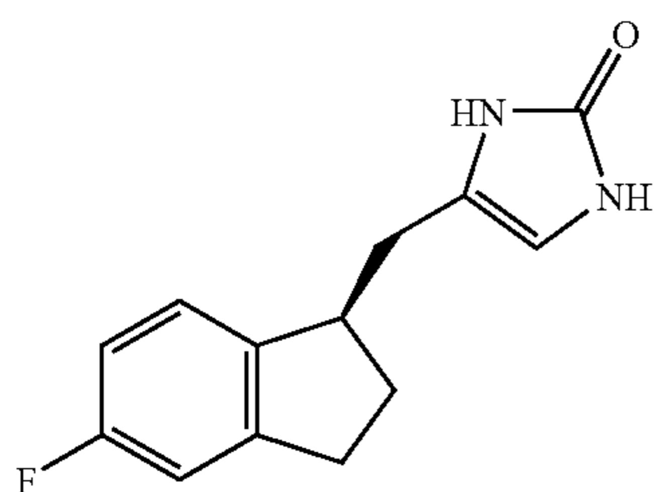
Compound 61
