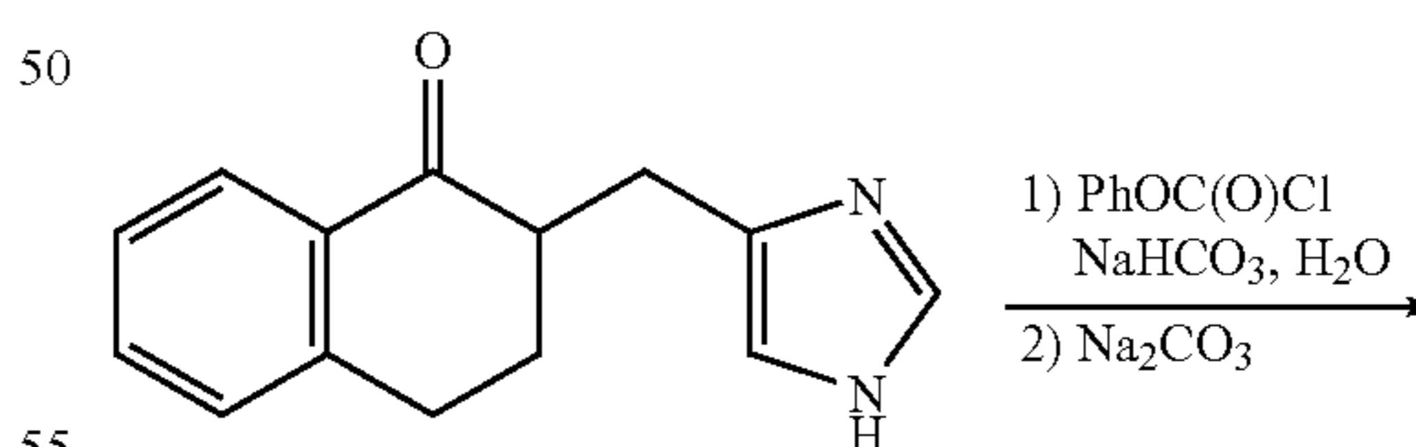
Intermediate E4
