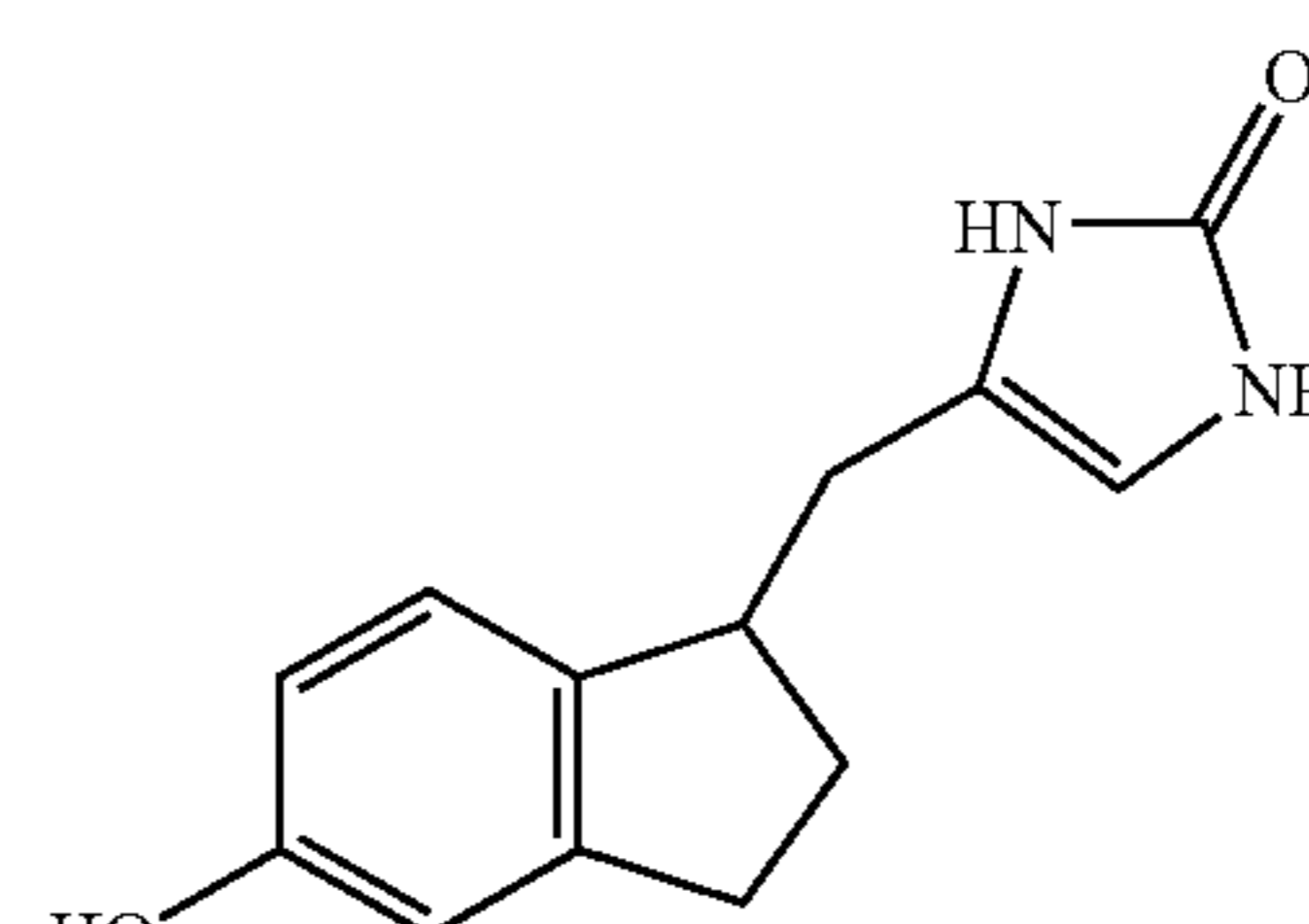
Compound 63
