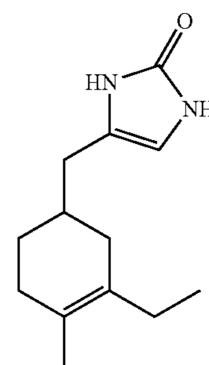
Compound 58
