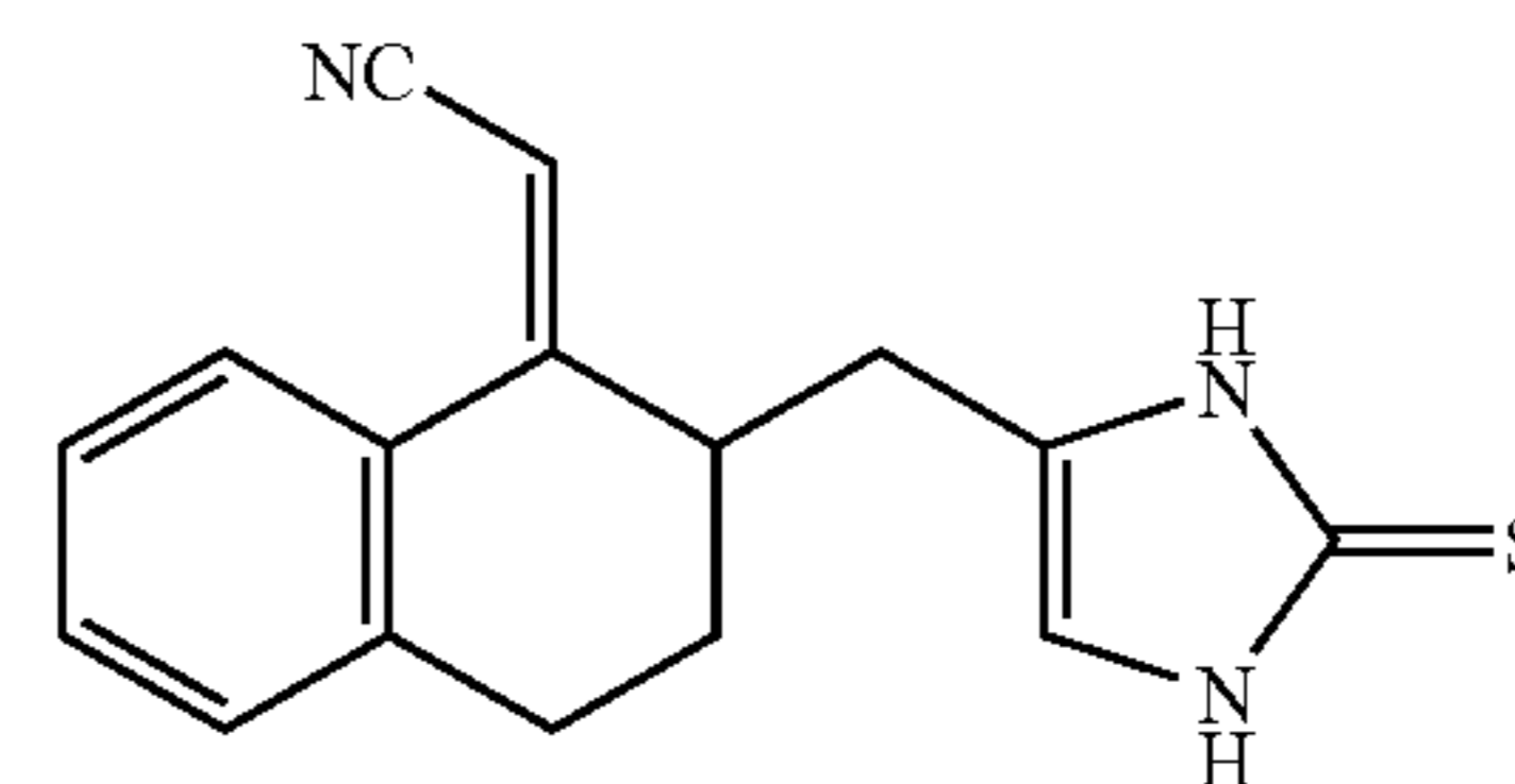
Compound 169
