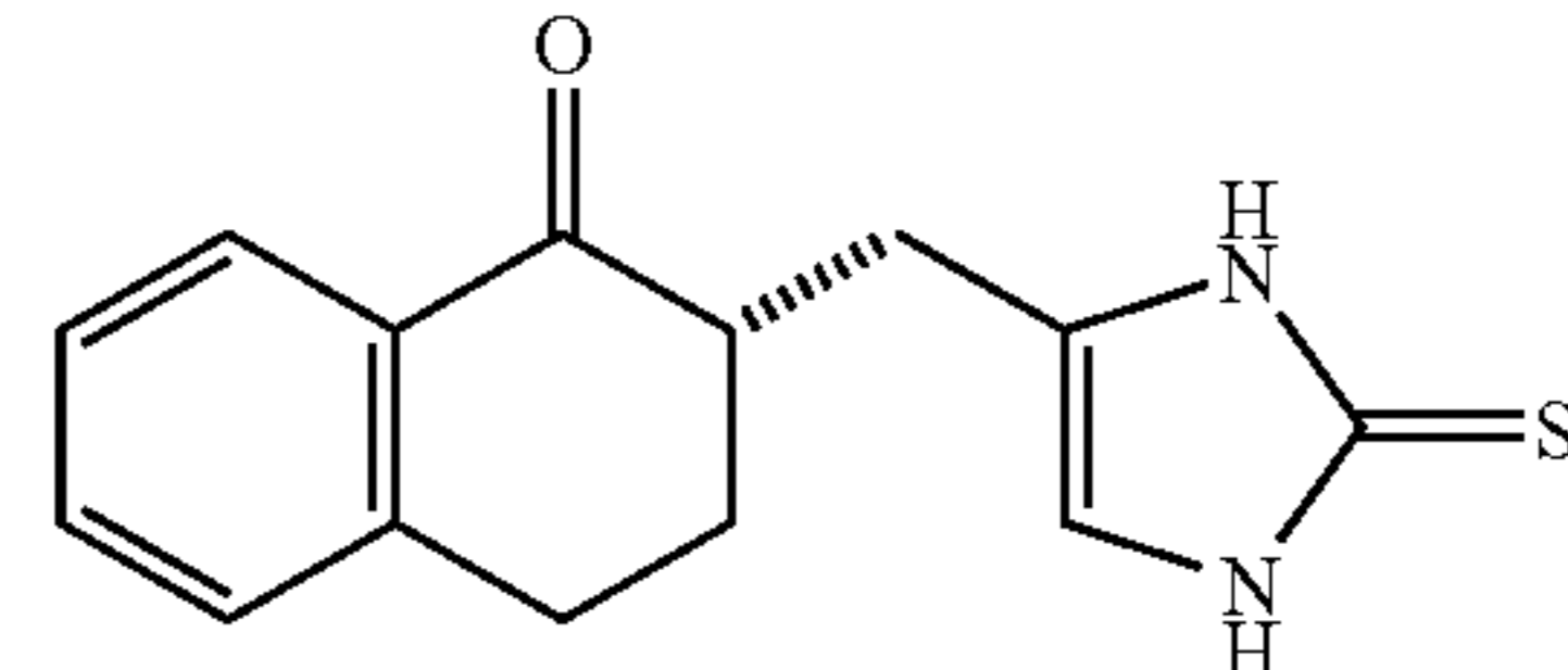
(-) - S Compound 23
