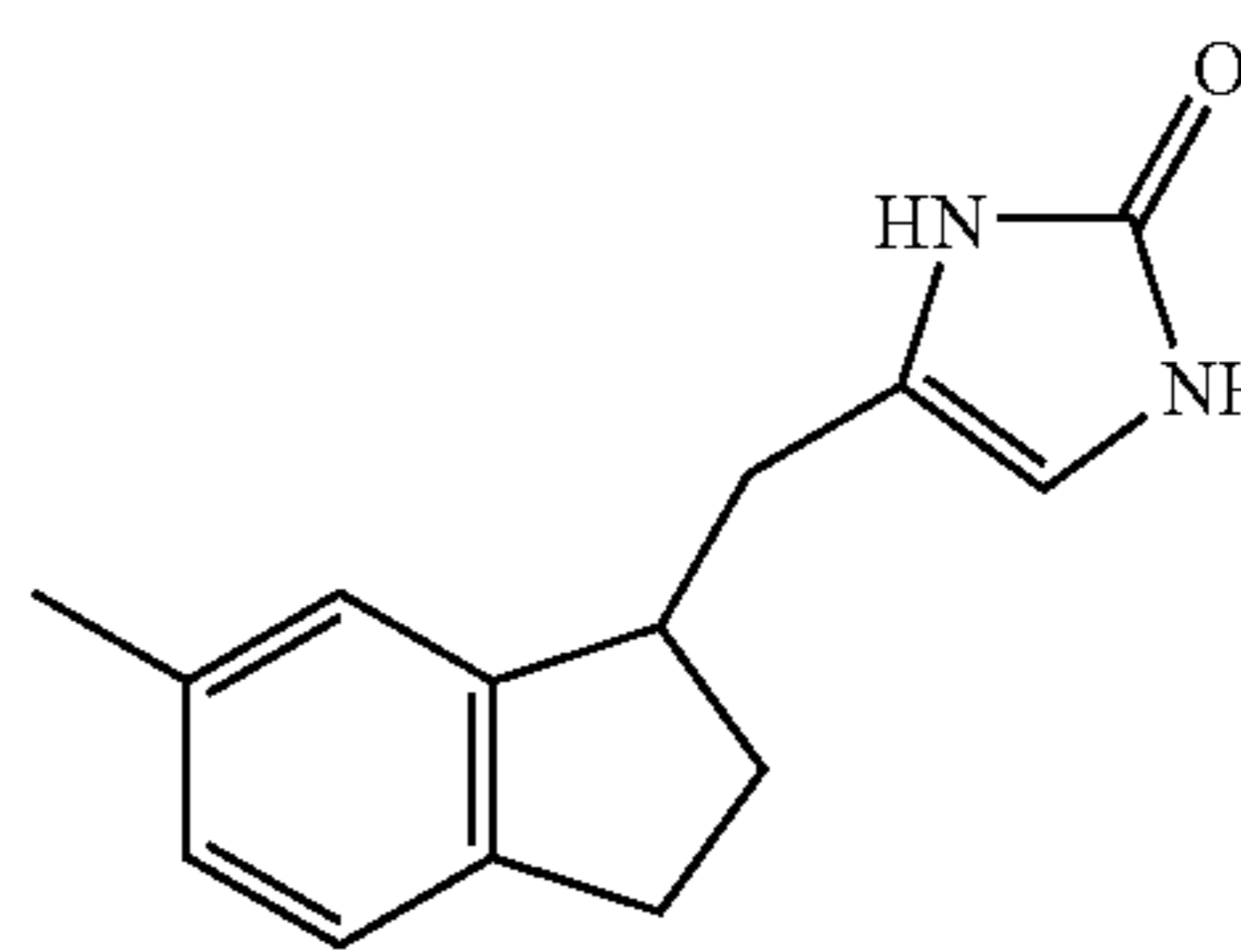
Compound 52
