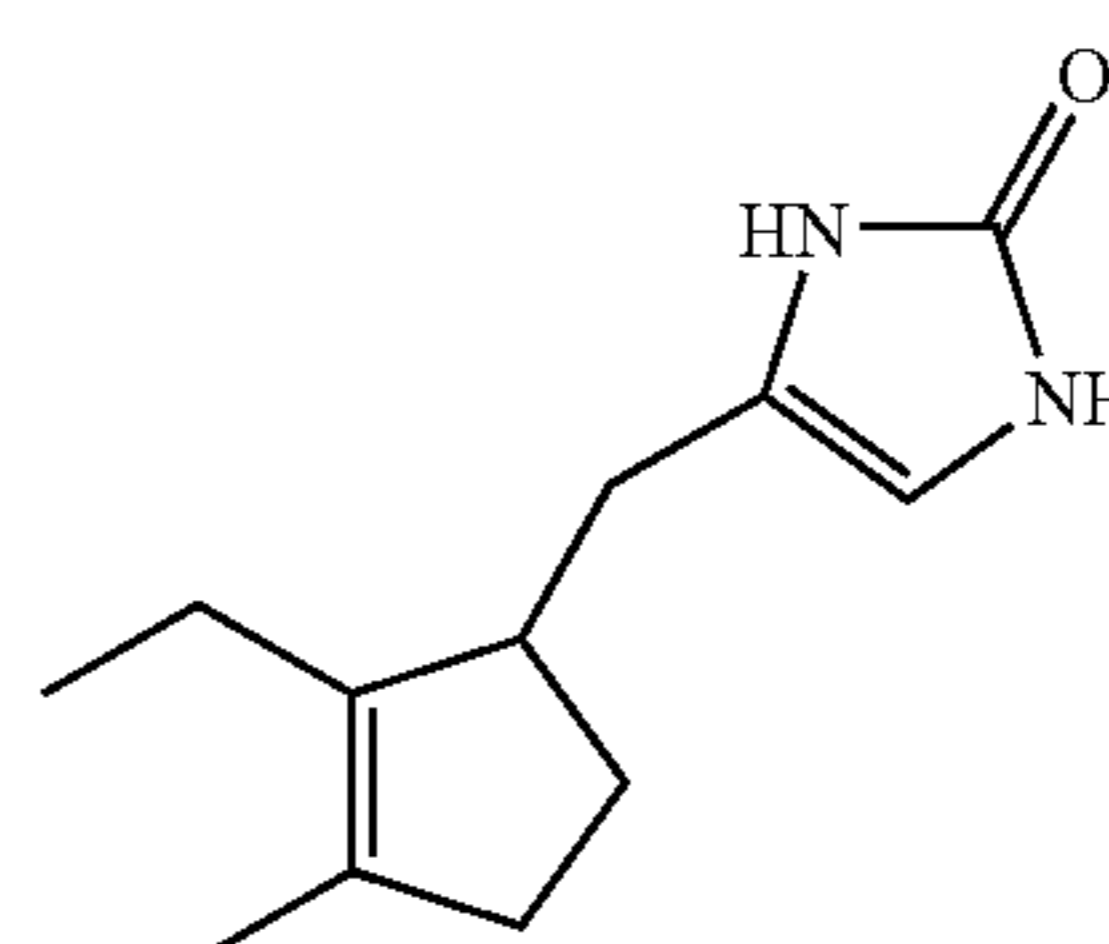
Compound 64
