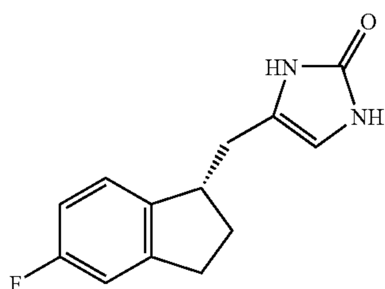
Compound 62
