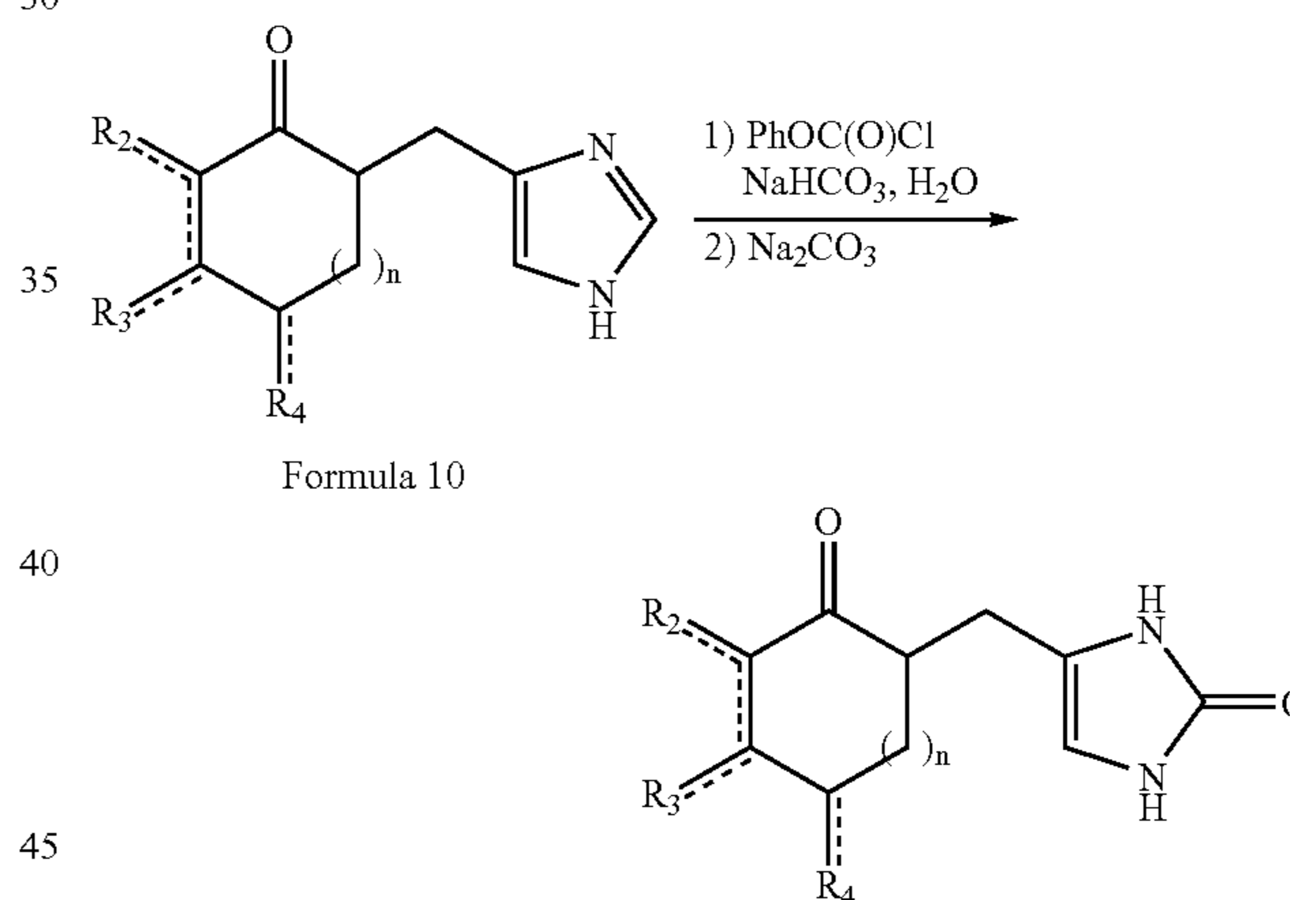
Formula 16
