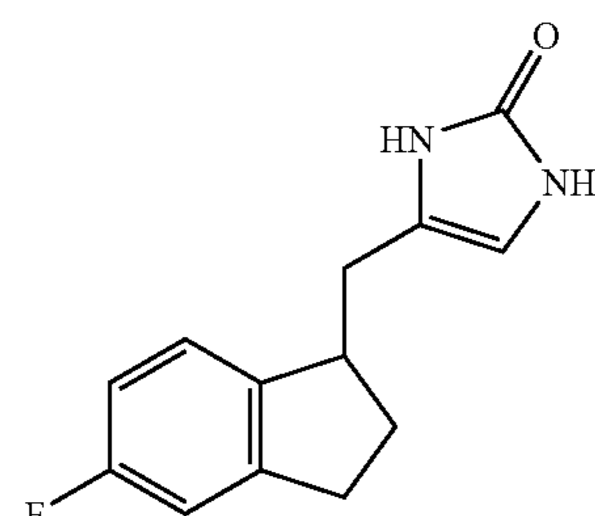
Compound 49
