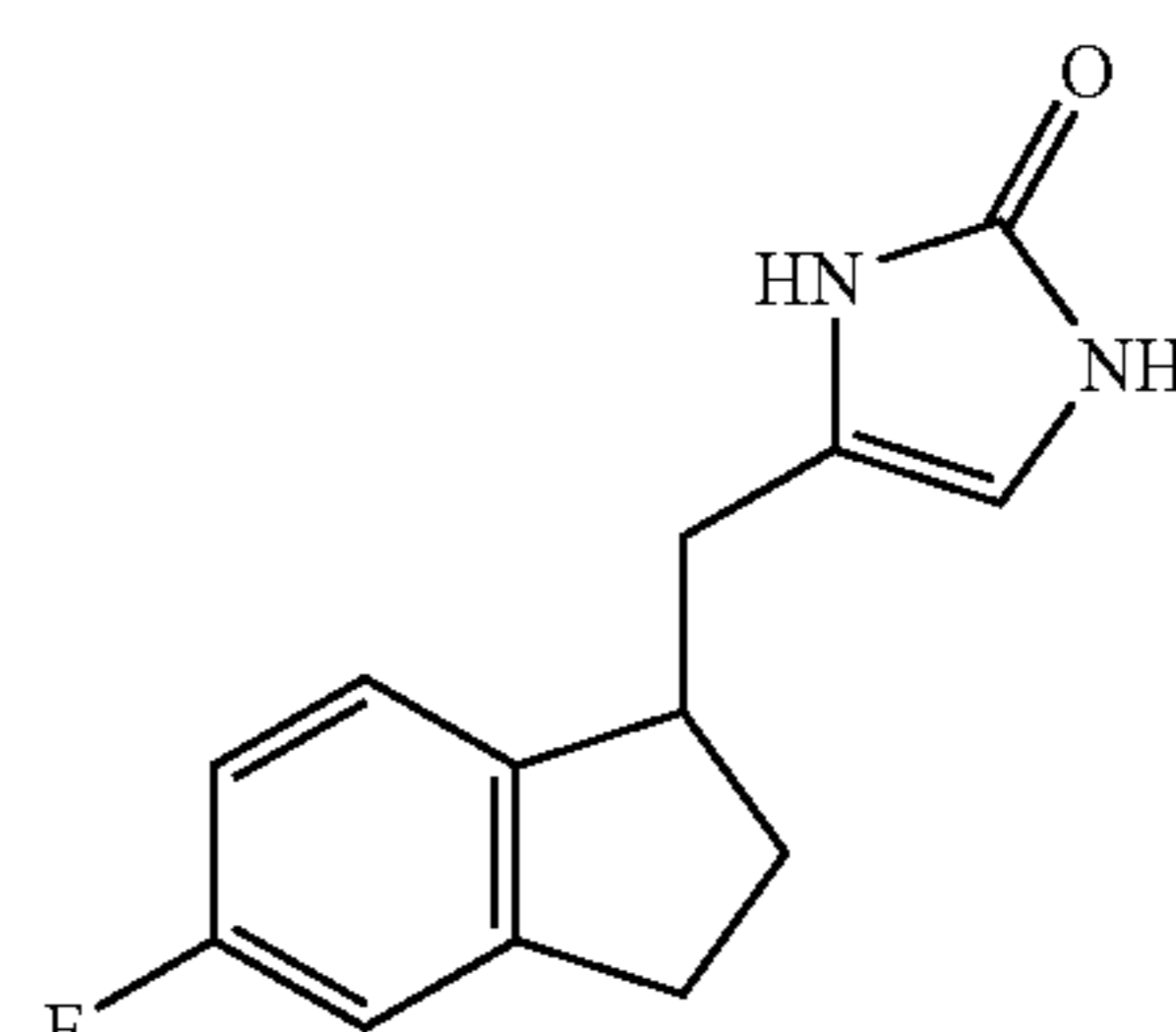
Compound 49
