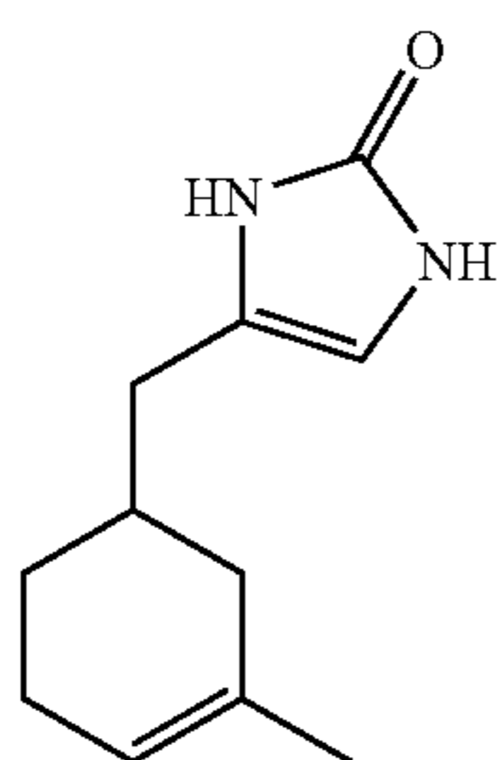
Compound 57
