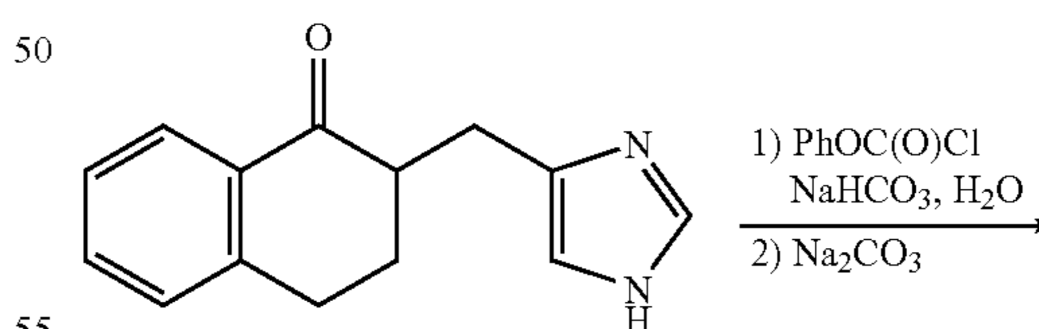
Intermediate E4
