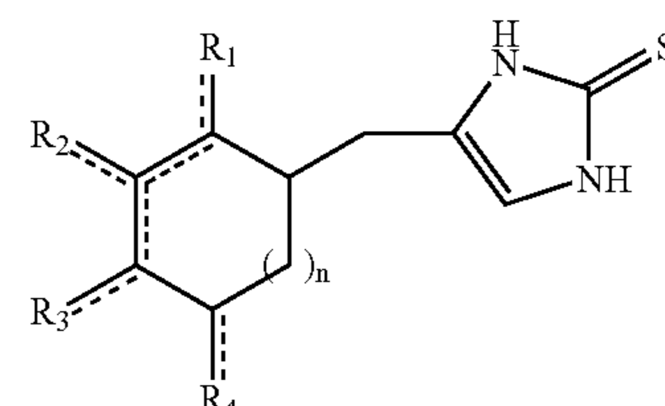
Formula 6
