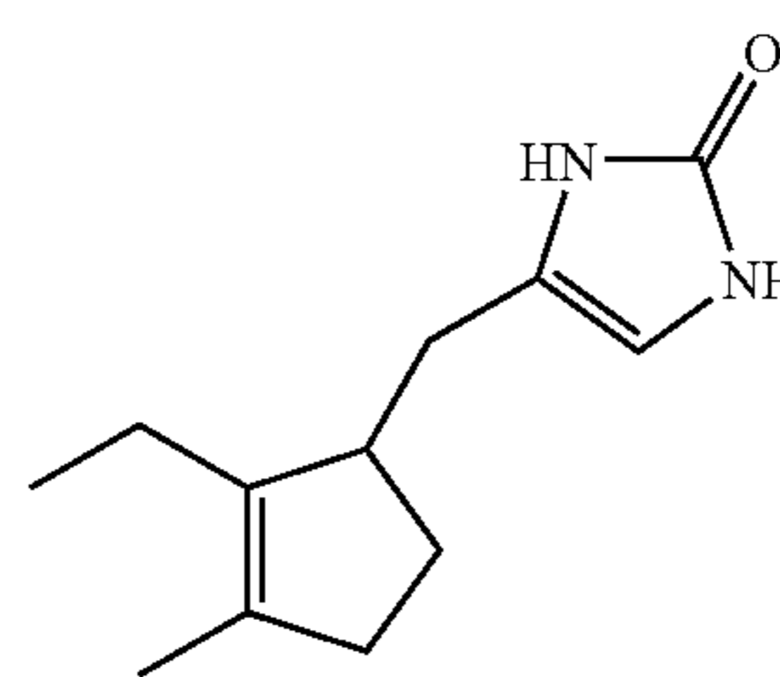
Compound 64
