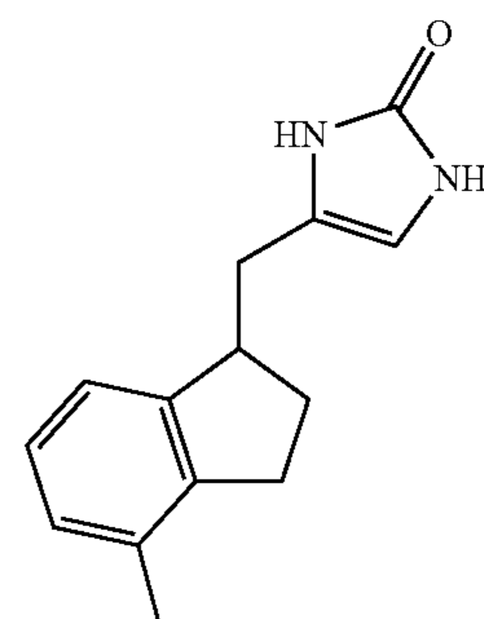
Compound 48
