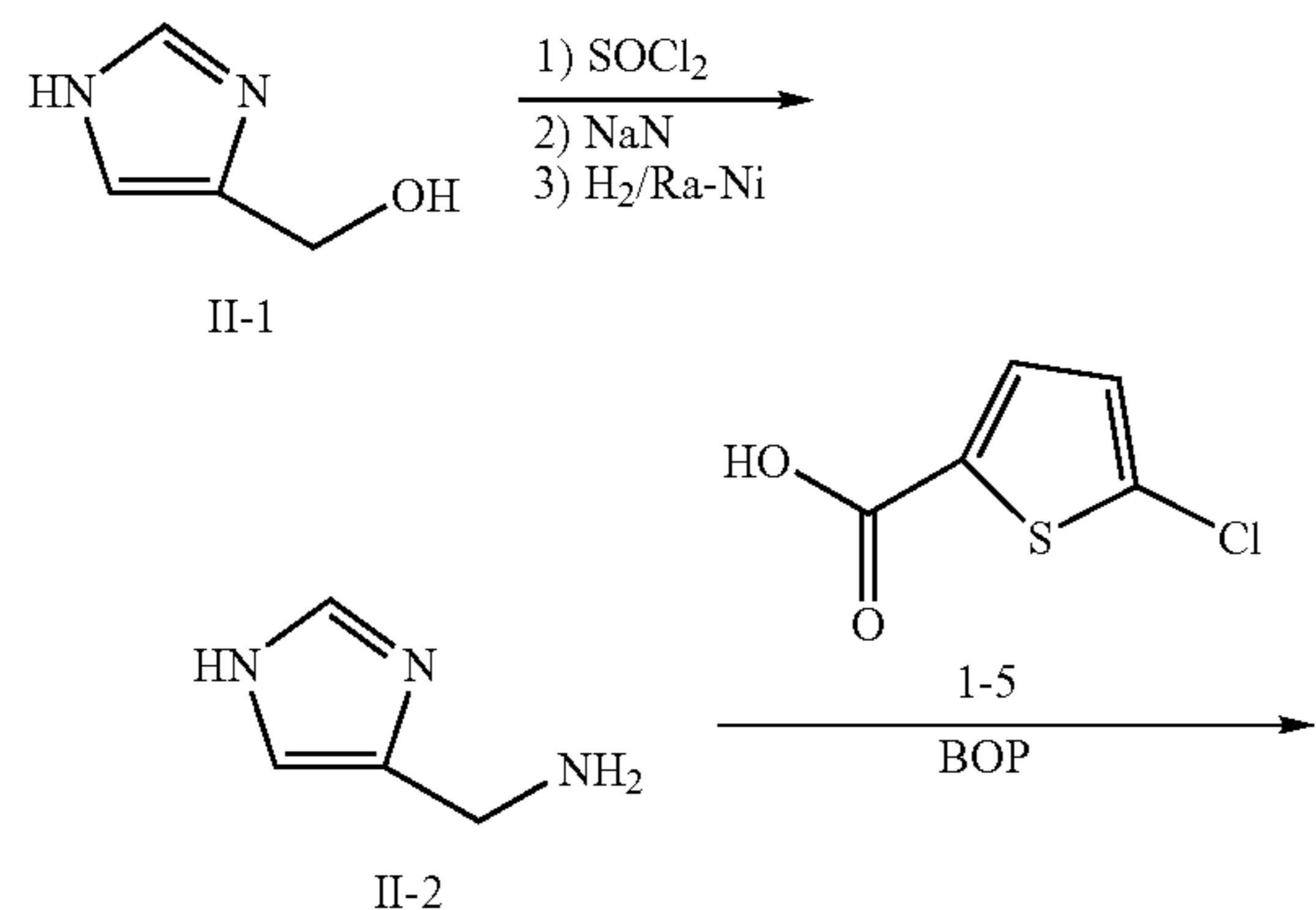
SCHEME 3
