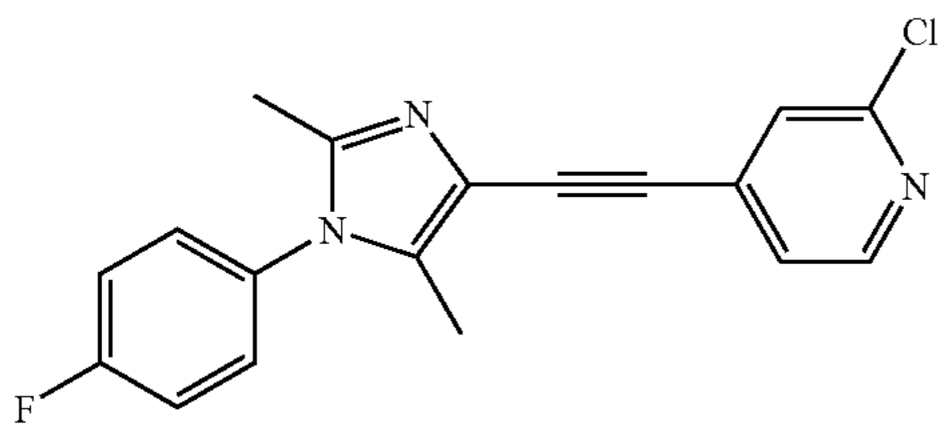
2-Chloro-4-[1-(4-fluoro-phenyl)-2,5-dimethyl-1H-imidazol-4-ylethynyl]-pyridine
