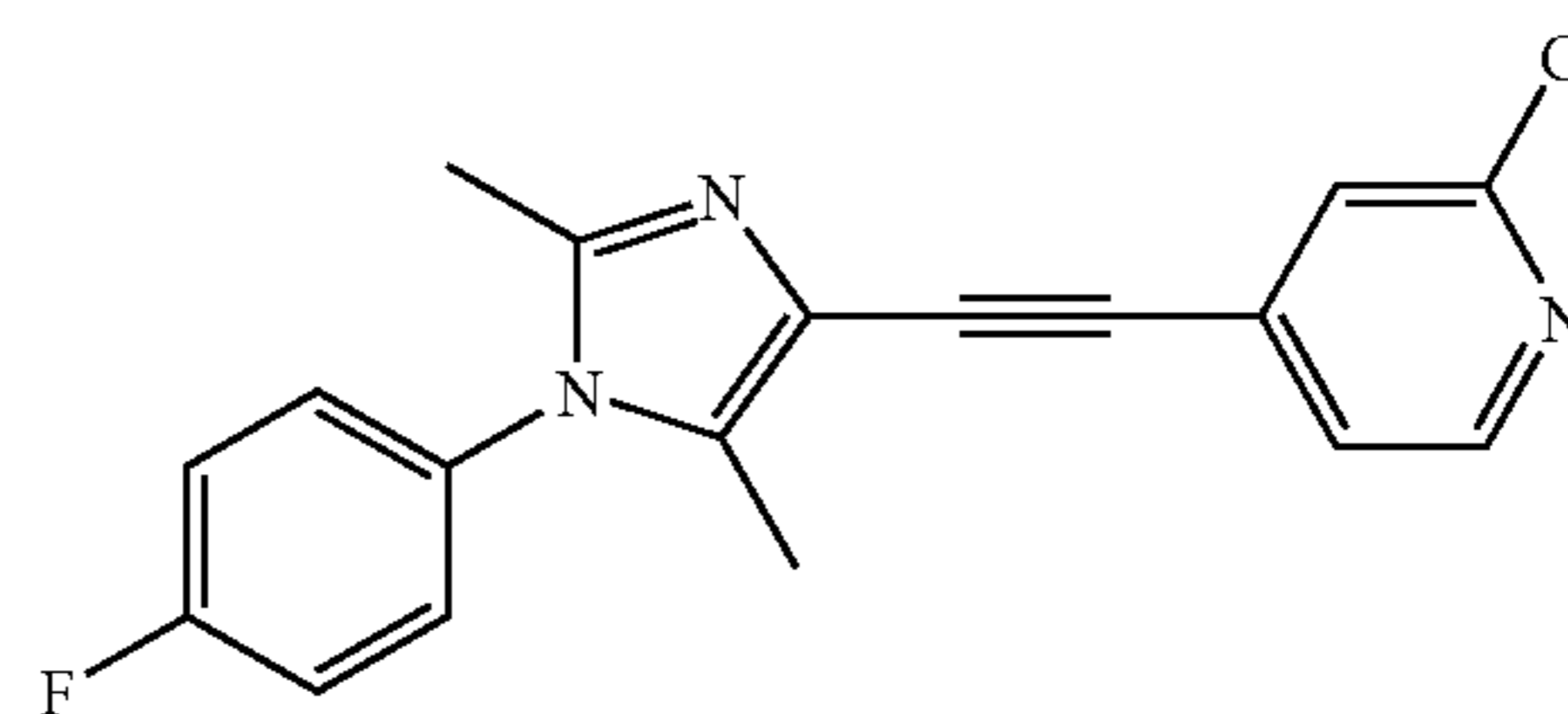
2-Chloro-4-[1-(4-fluoro-phenyl)-2,5-dimethyl-1H-imidazol-4-ylethynyl]-pyridine
