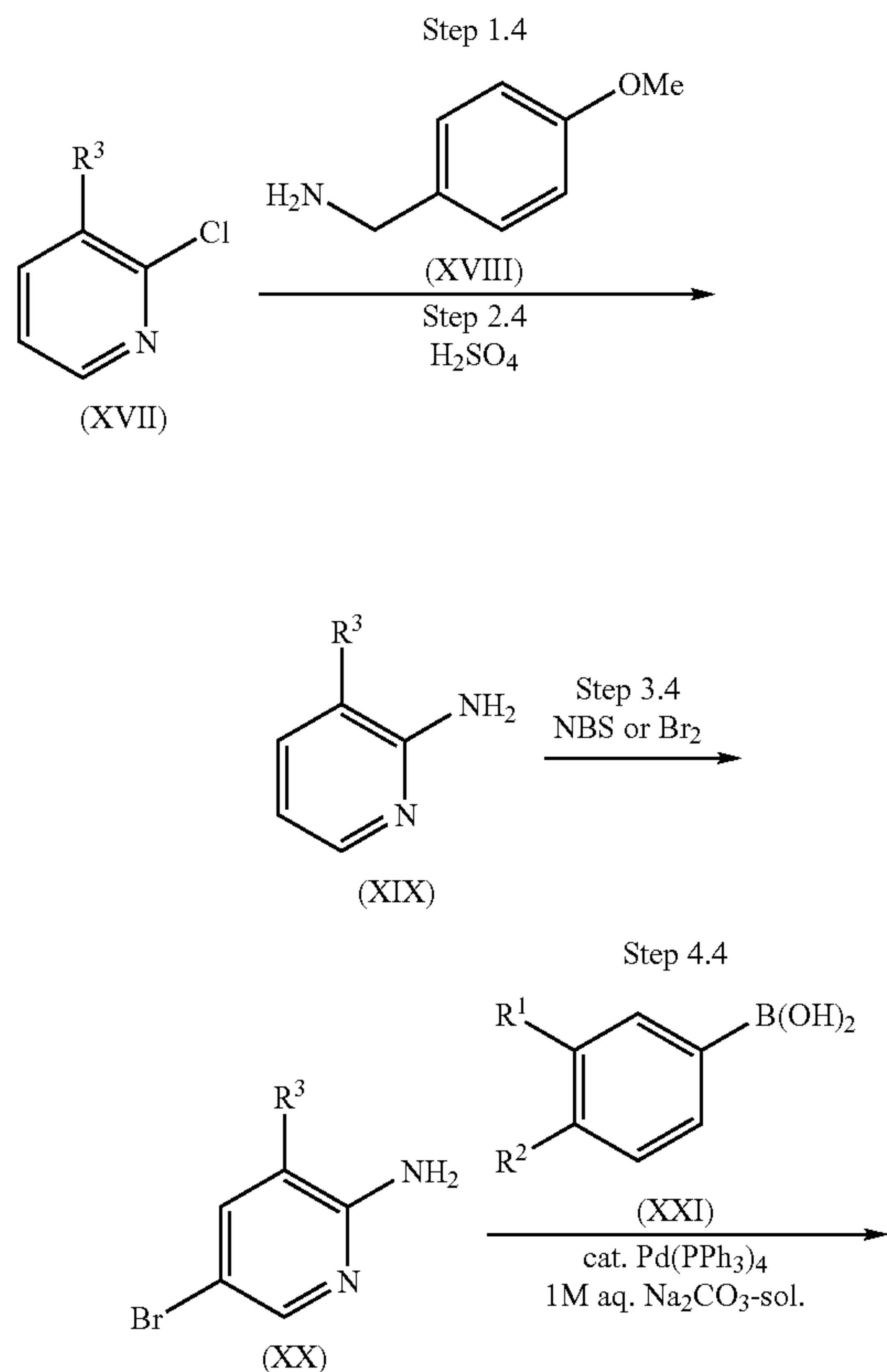
Scheme 4
