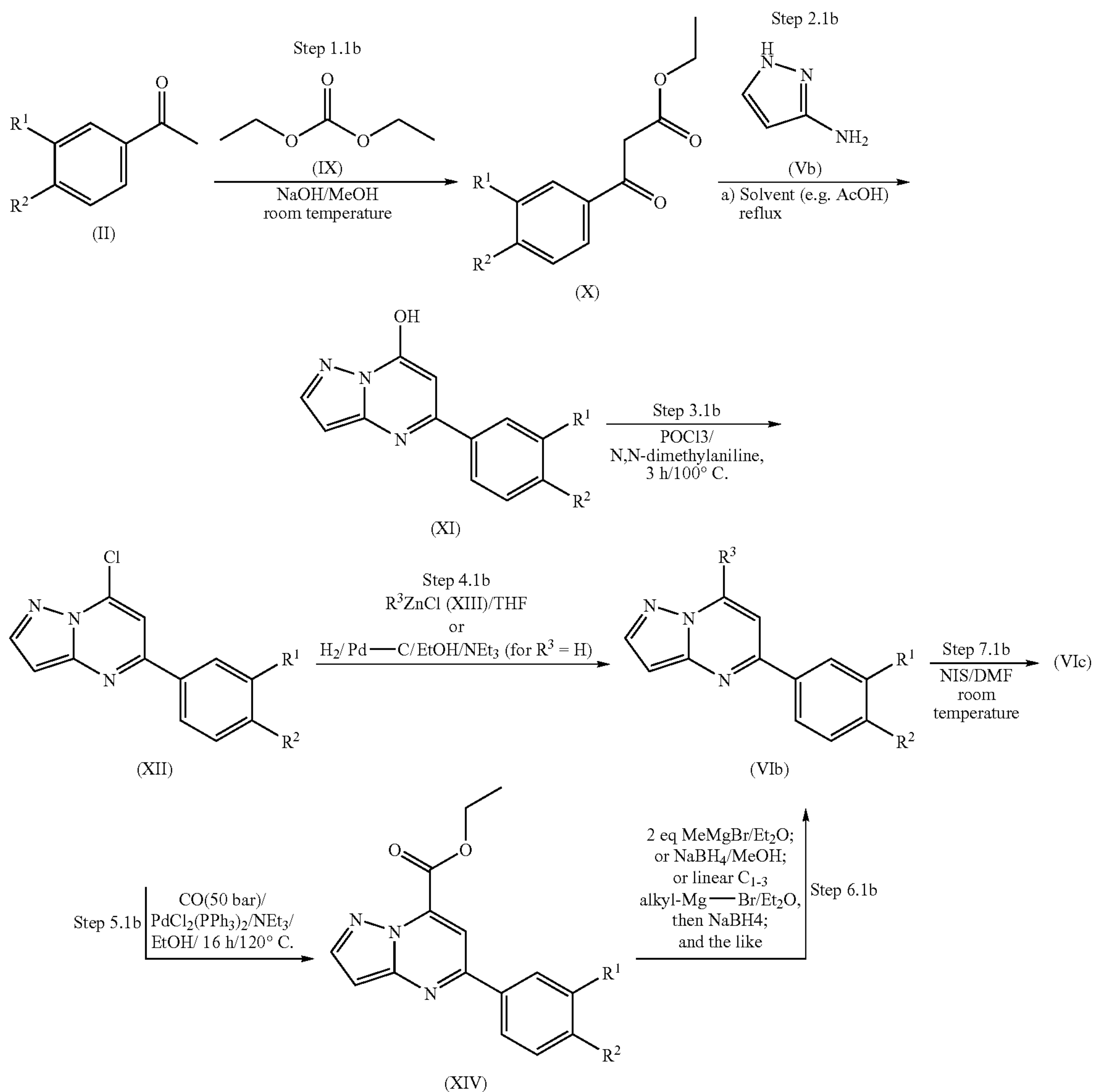
Scheme 1b
