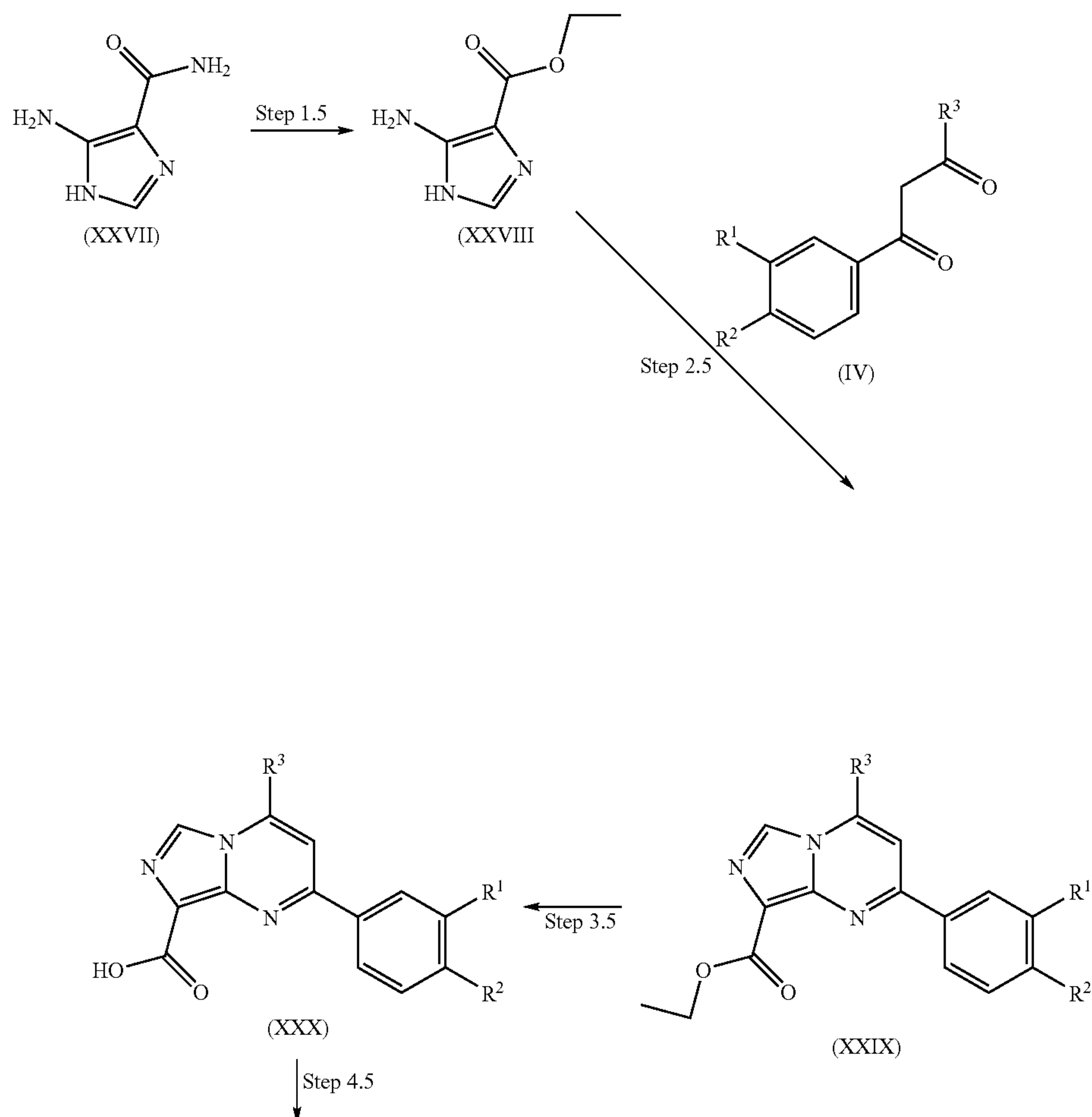
Scheme 5
