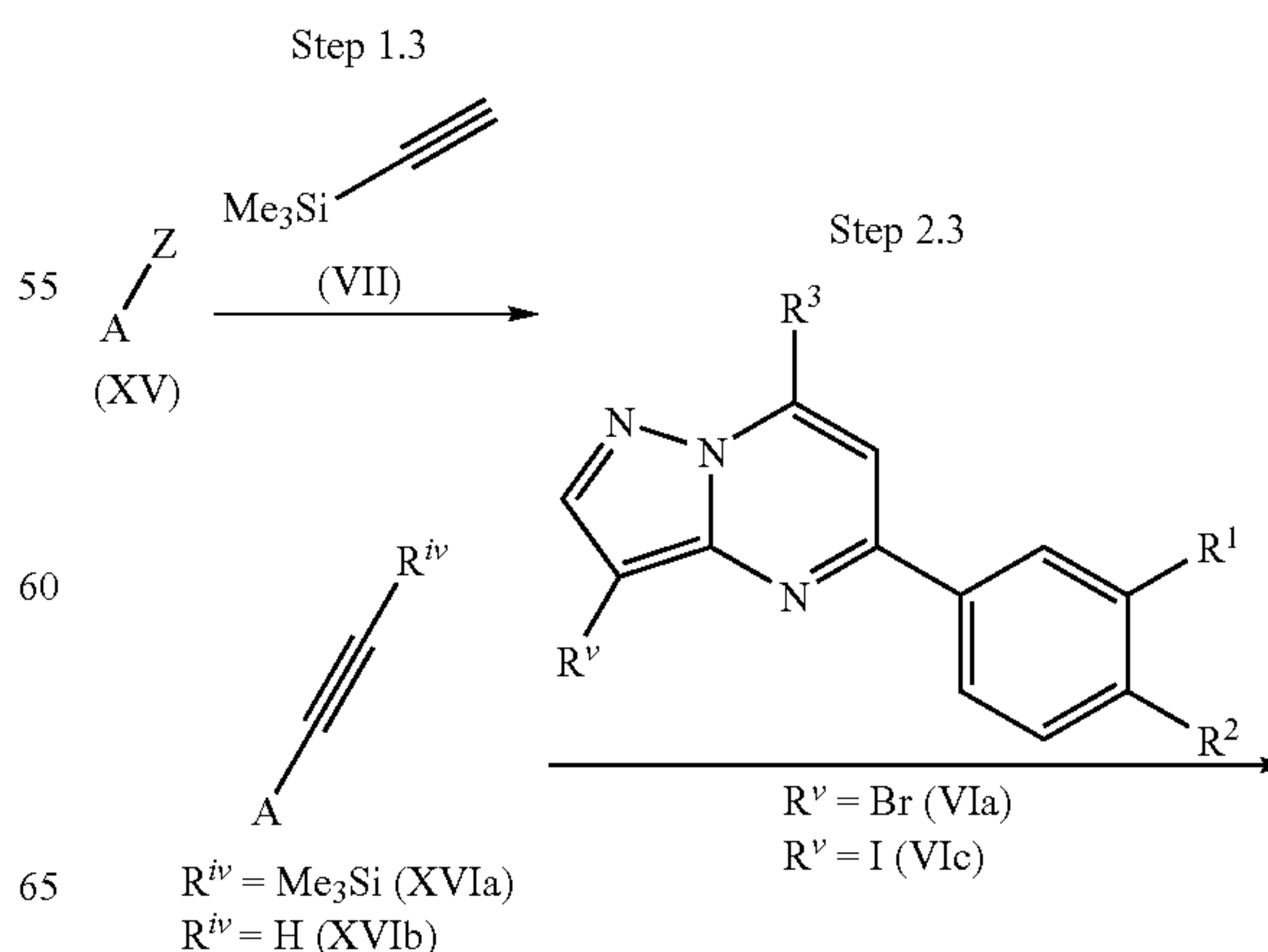
Scheme 3
