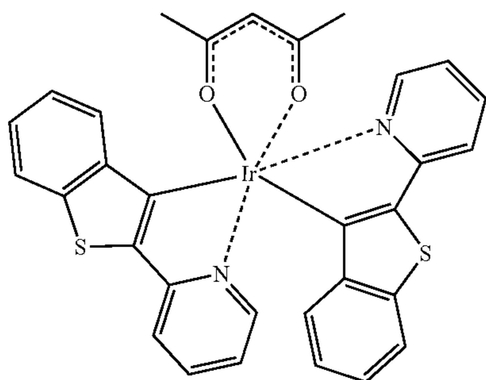
Ir(btp) 2 (acac) 1
