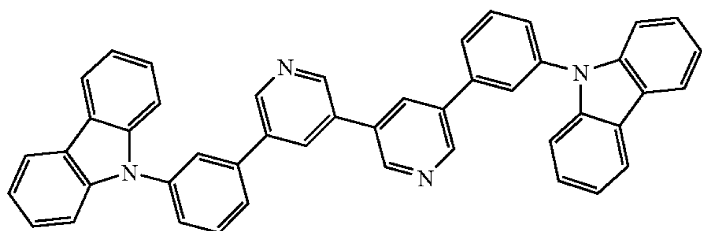
5,5'-bis(3-(carbazol-9-yl)phenyl)-3,3'-bipyridine
