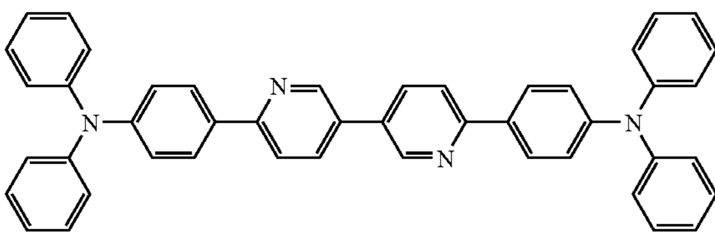
4,4'-(3,3'-bipyridine-6,6'-diyl)bis(N,N-diphenylaniline)
