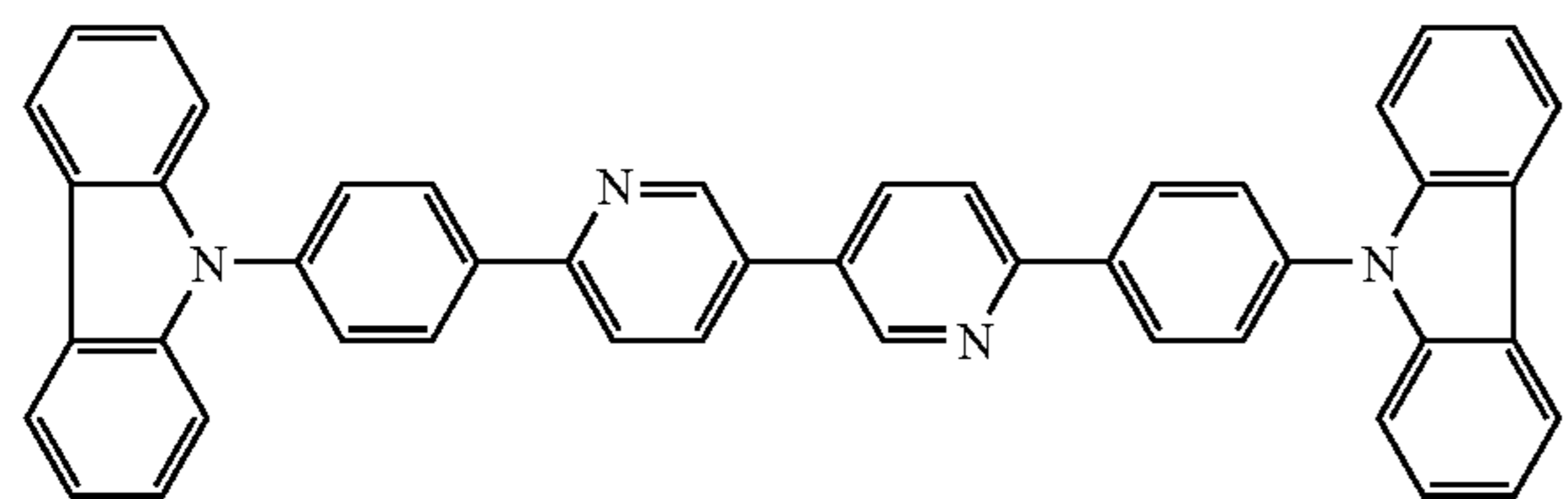
6,6'-bis(4-(carbazol-9-yl)phenyl)-3,3'-bipyridine
