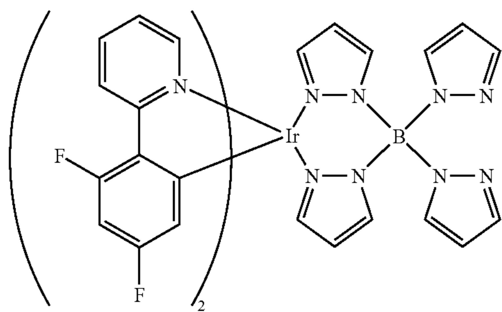
bis[2-(4,6-difluorophenyl)pyridinato-N,C 2' ]iridium(III)tetra(1-pyrazolyl)borate (Fir6)
