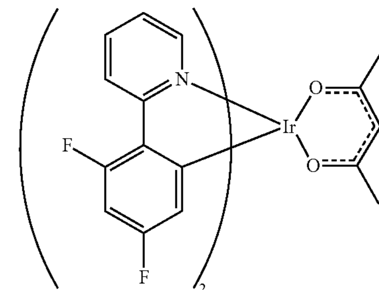
bis(2-[4,6-difluorophenyl]pyridinato-N,C2')iridium(acetylacetonate) [FIr(acac)]
