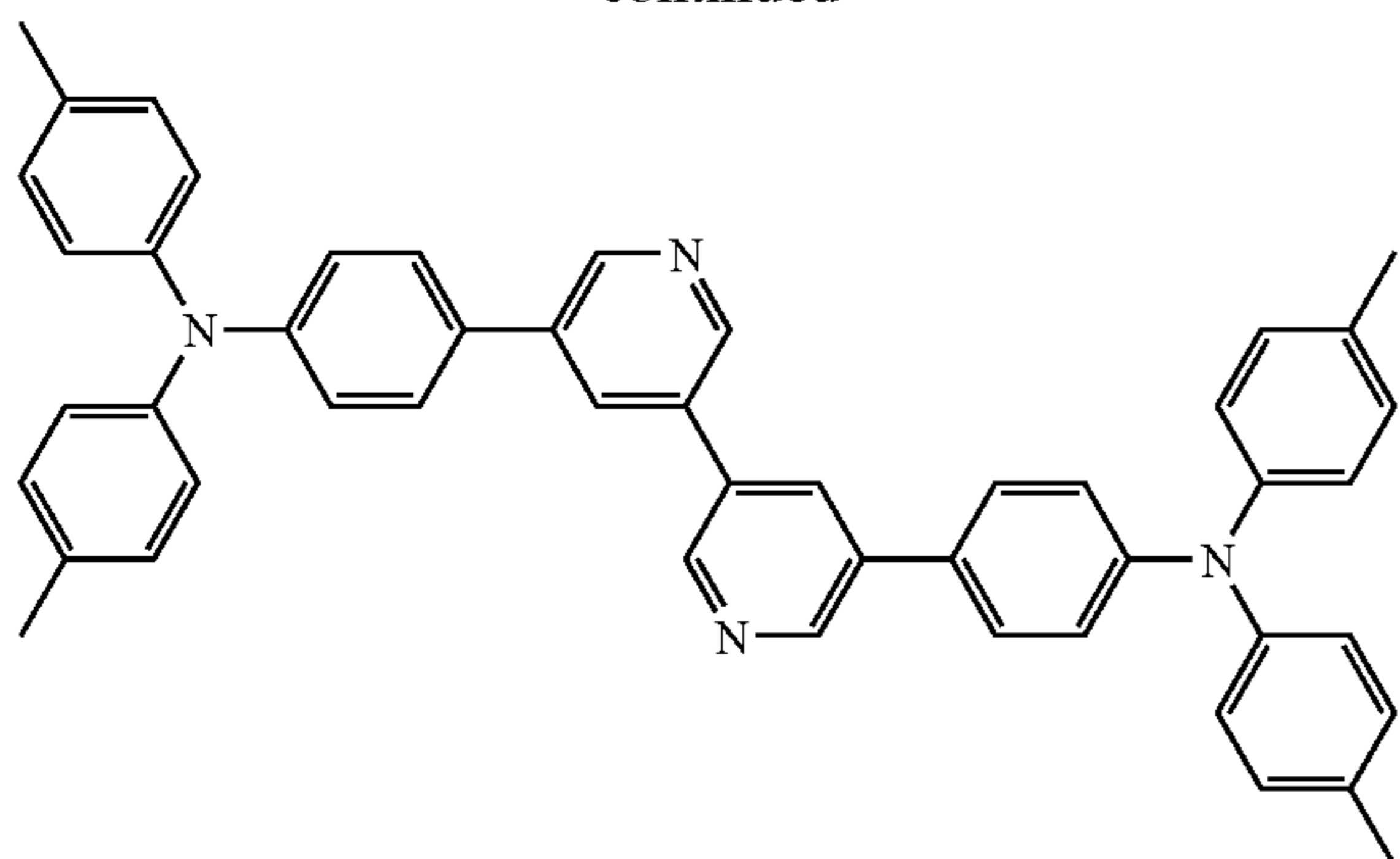
5,5'-bis(4-di(4-methylphenyl)aminophenyl)-3,3'-bipyridine
