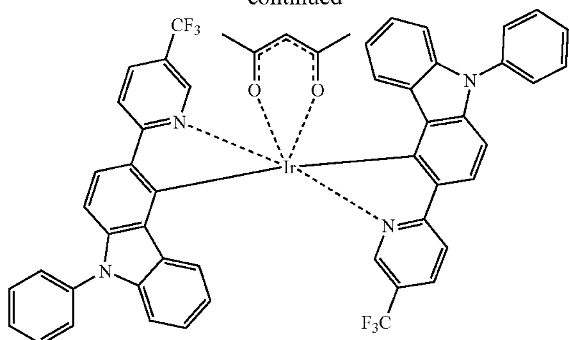
(Cz-CF 3 )Ir(III)(acac) Bis[5-trifluoromethyl-2-[3-(N-phenylcarbazolyl)pyridinato-N,C2']iridium(III)(acetylacetonate)
