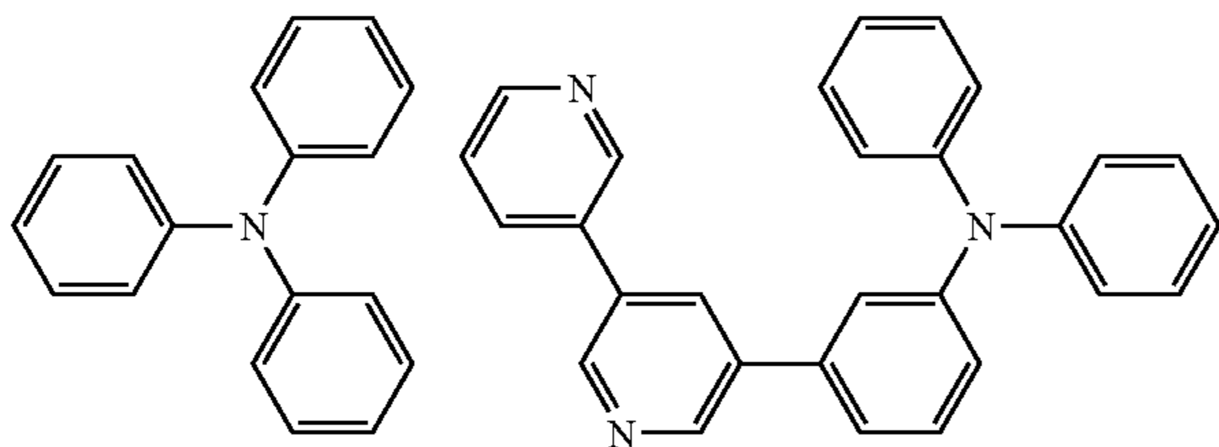
5,5'-bis(3-diphenylaminophenyl)-3,3'-bipyridine
