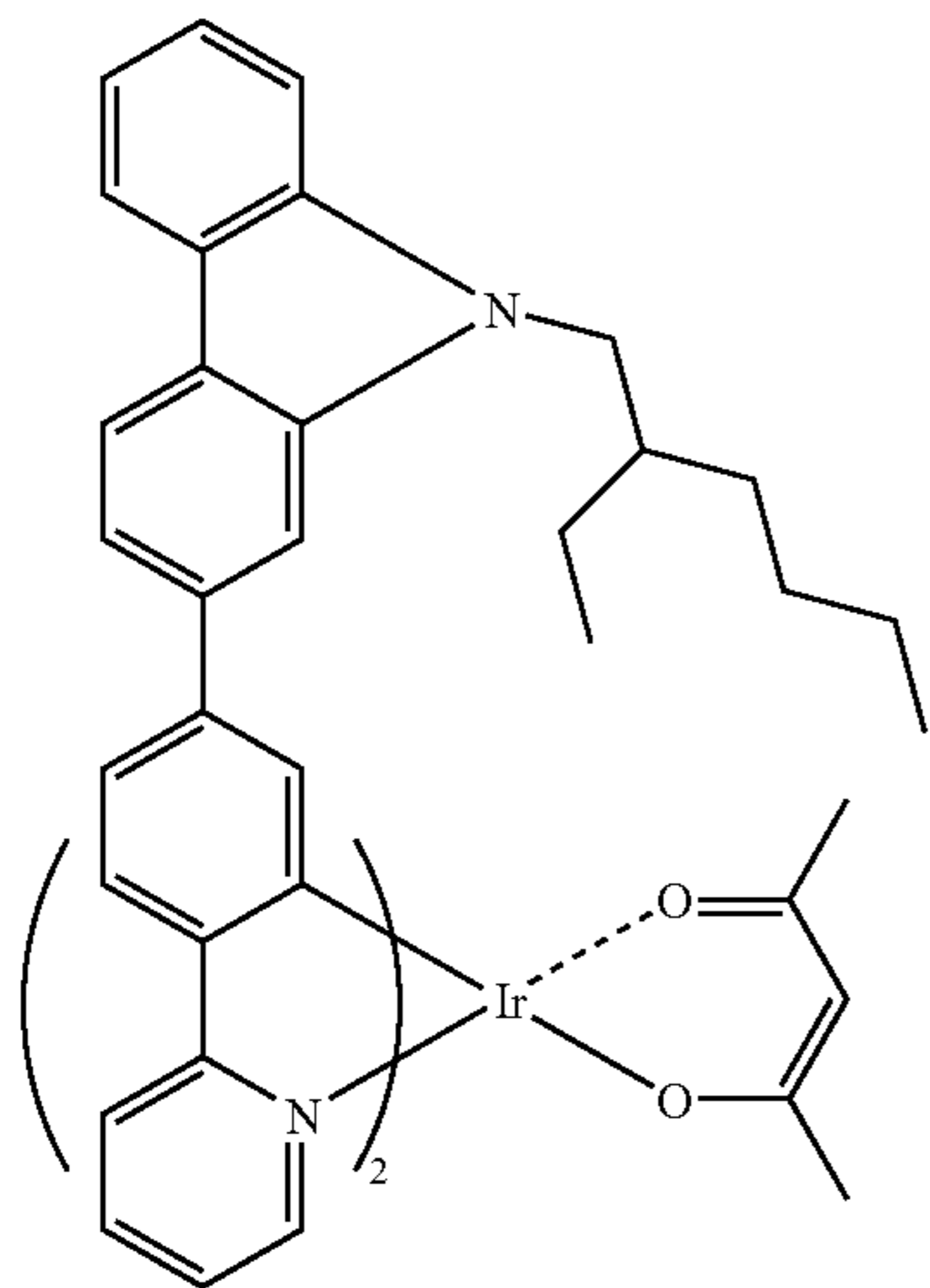
(2-PhPyCz) 2 Ir(III)(acac)
