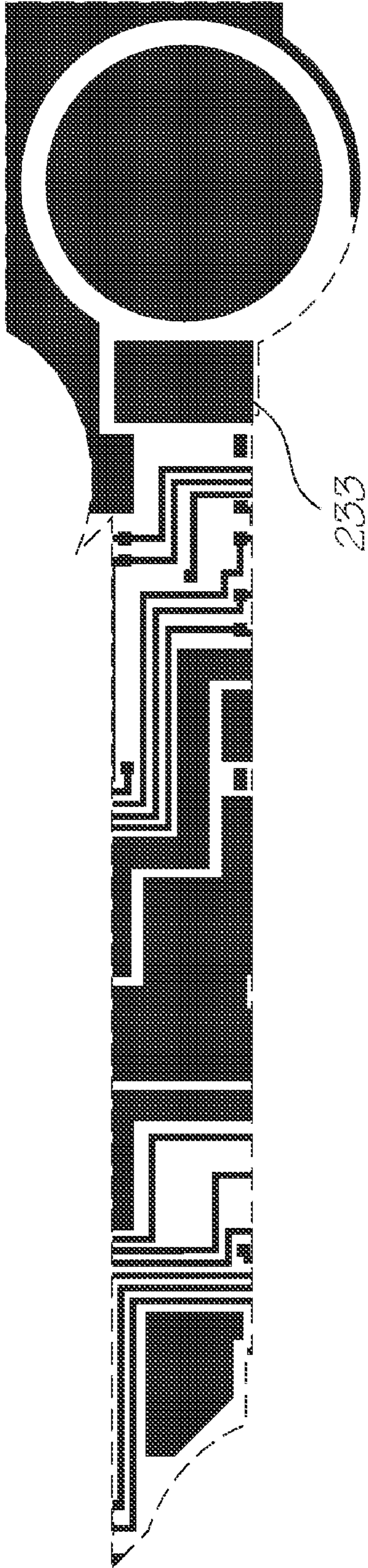
Metal 2 mask
