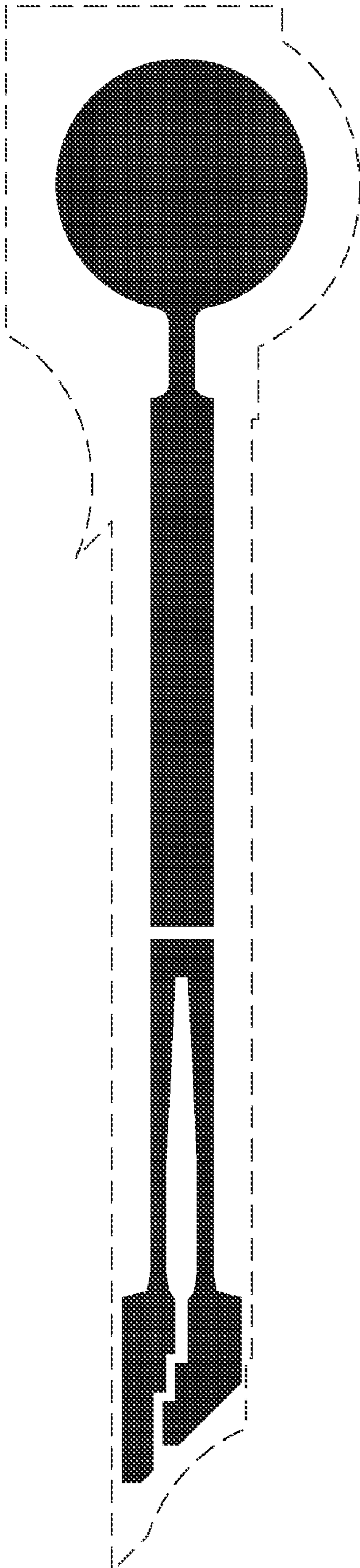
Heater mask
