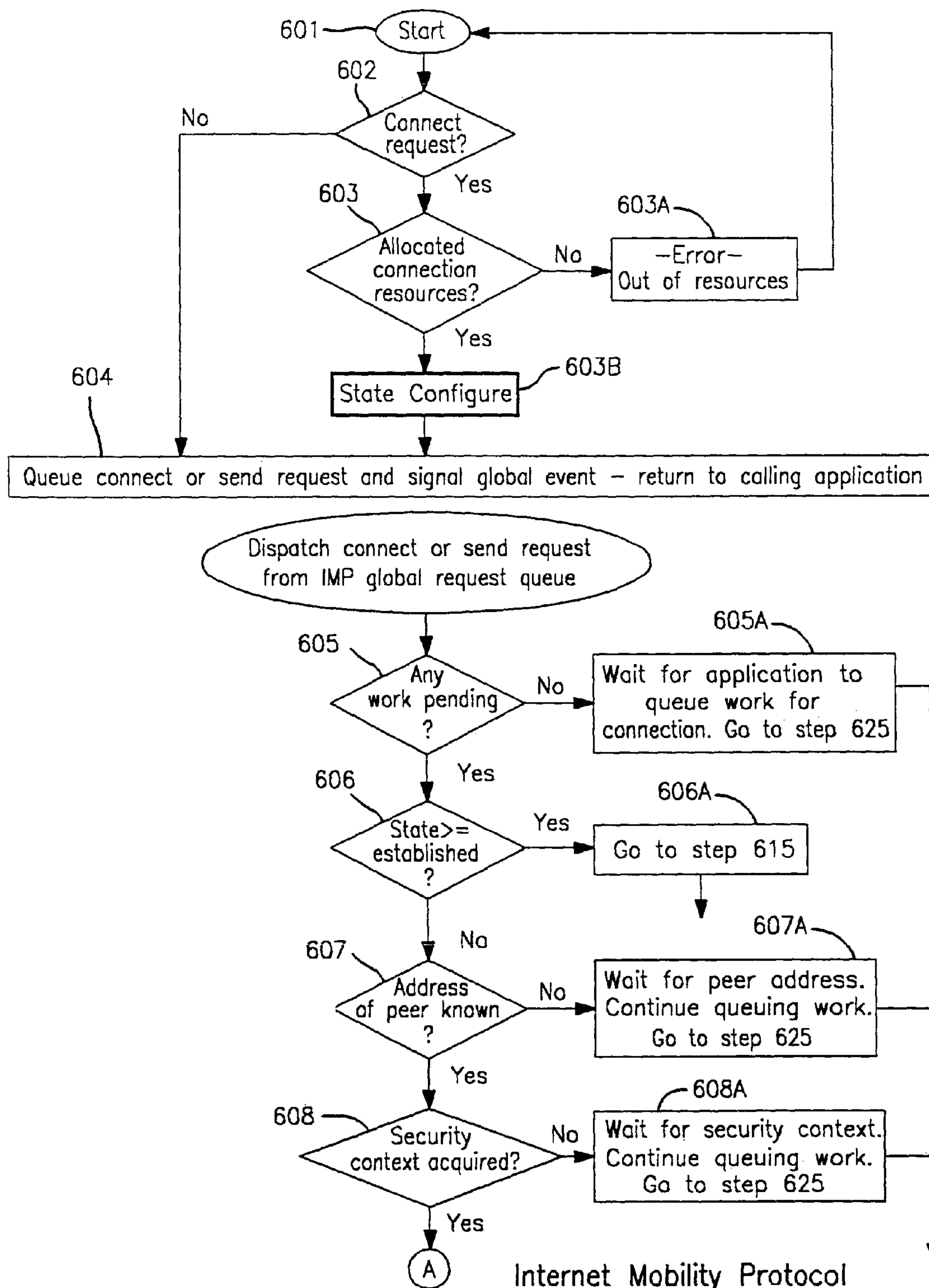
FIG. 10A Connect and Send request logic
