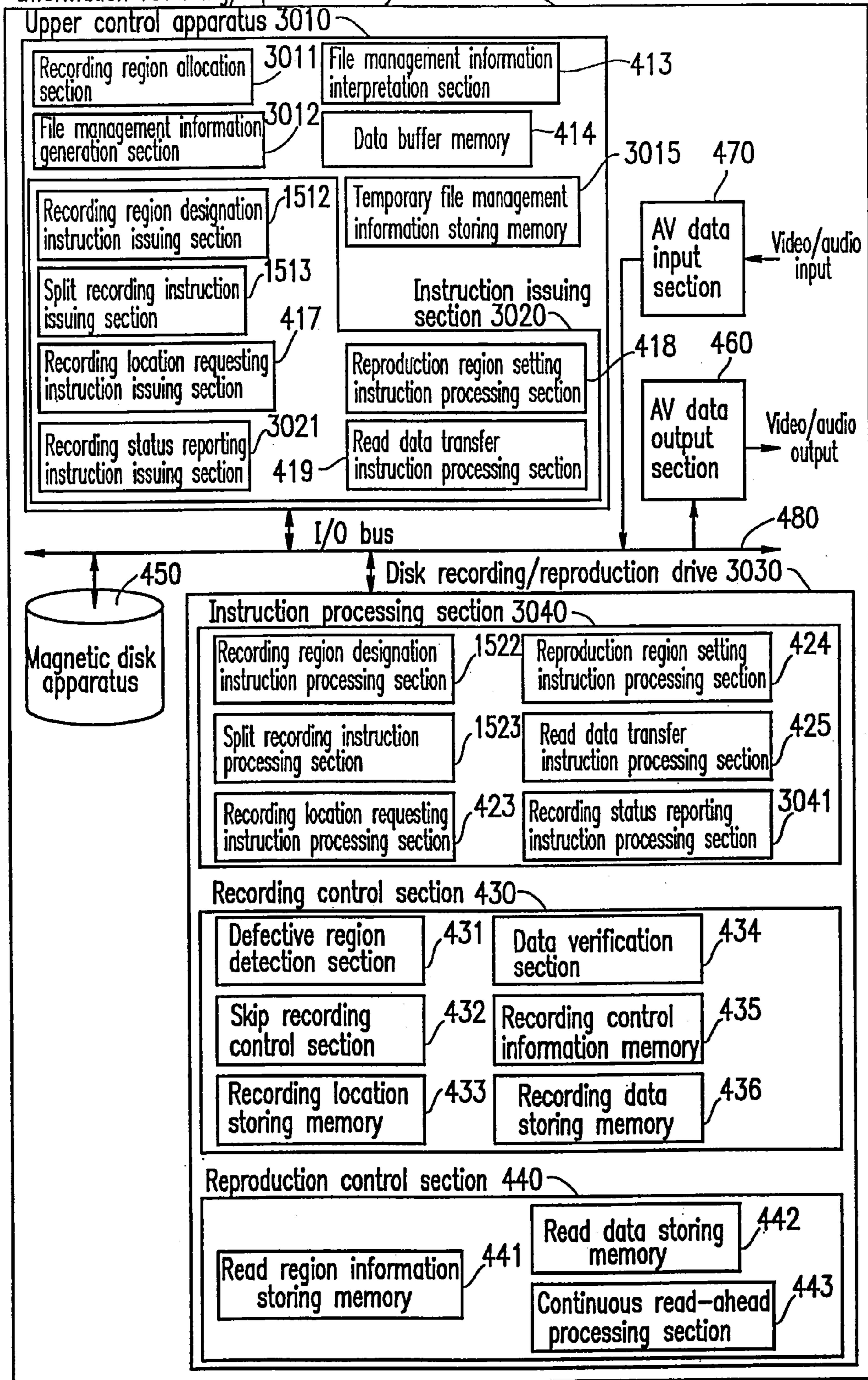
Information recording/reproduction system 3000
