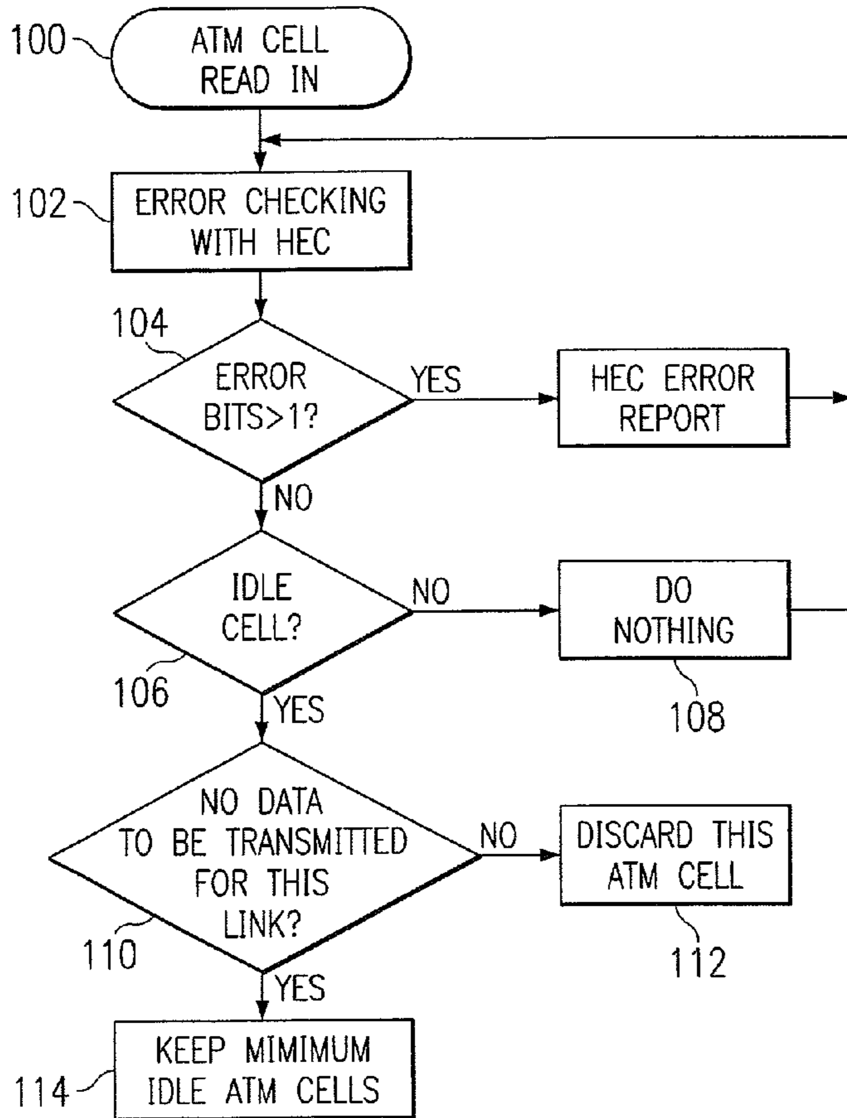
FIG. 6 (PRIOR ART)
