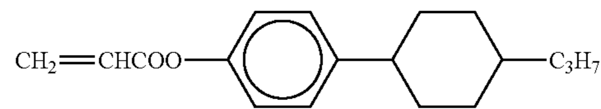
Chemical formula 2
