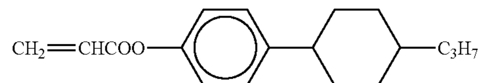
Chemical formula 2
