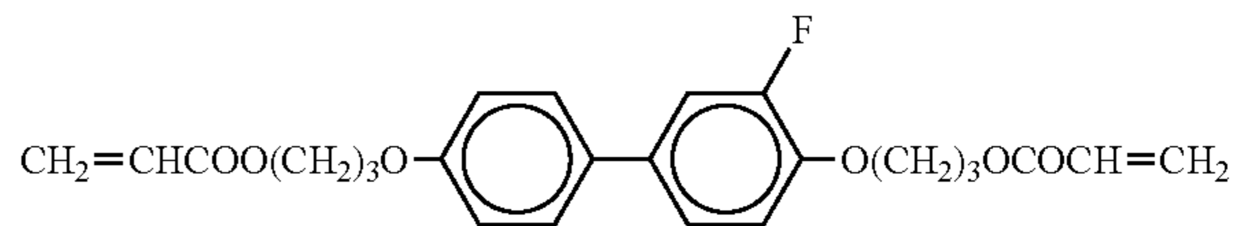
Chemical formula 2
