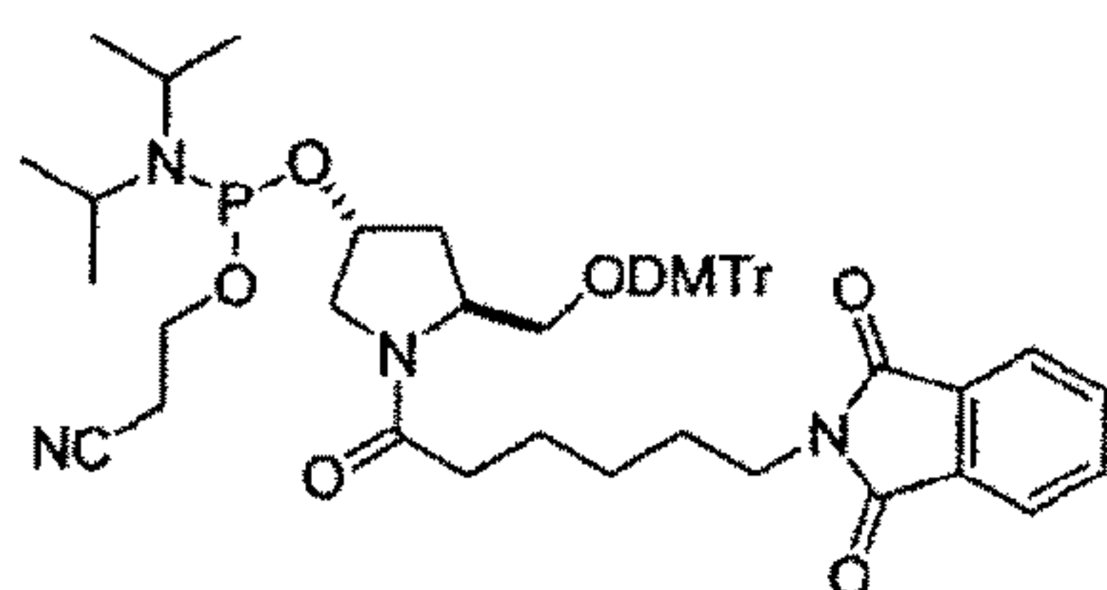
III. Hydroxyproline-Amine Amidite
