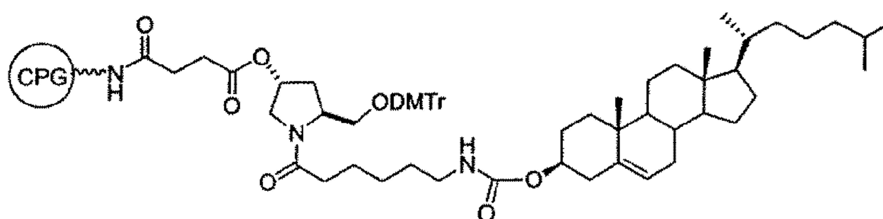
II. Cholesterol-Hyp Icaa CPG
