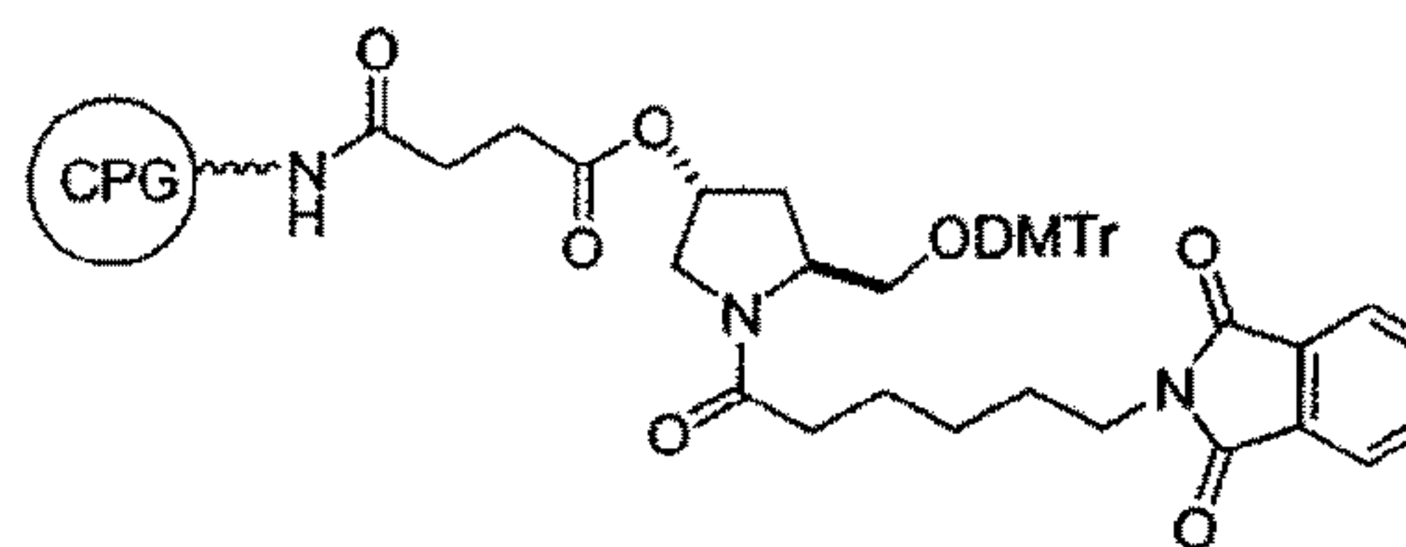
IV. Hydroxyproline-Amine Icaa CPG
