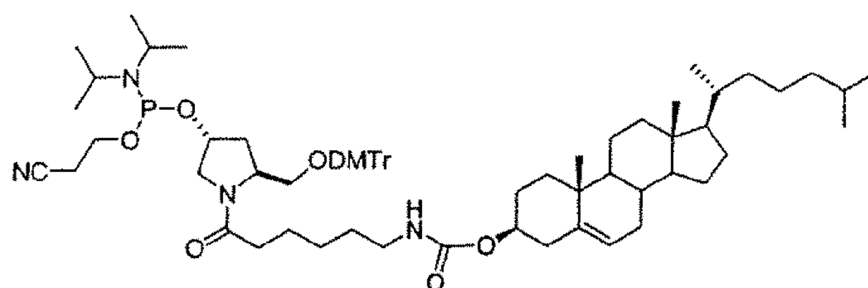
I. Cholesterol-Hyp Amidite
