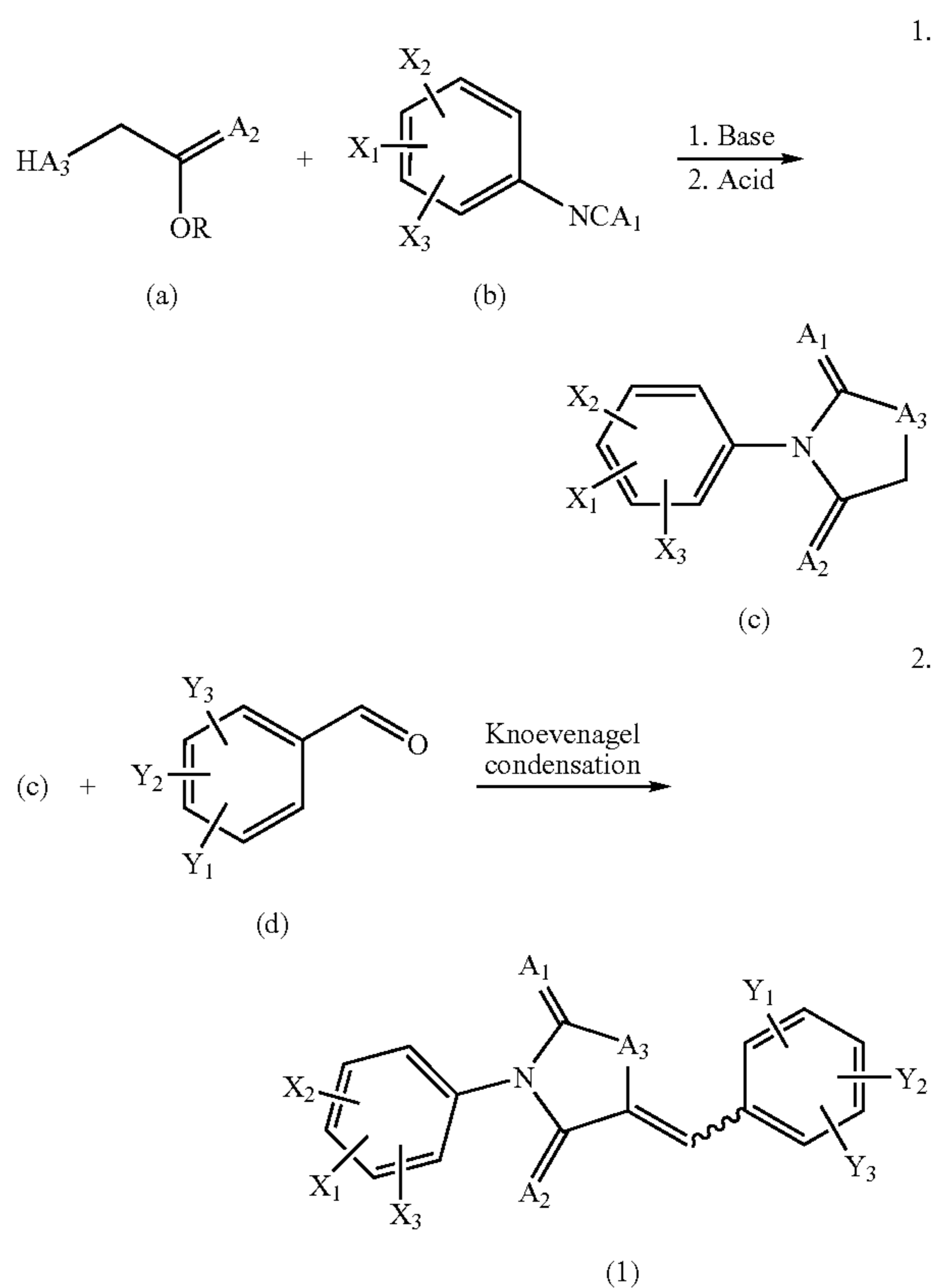
REACTION SCHEME 1
