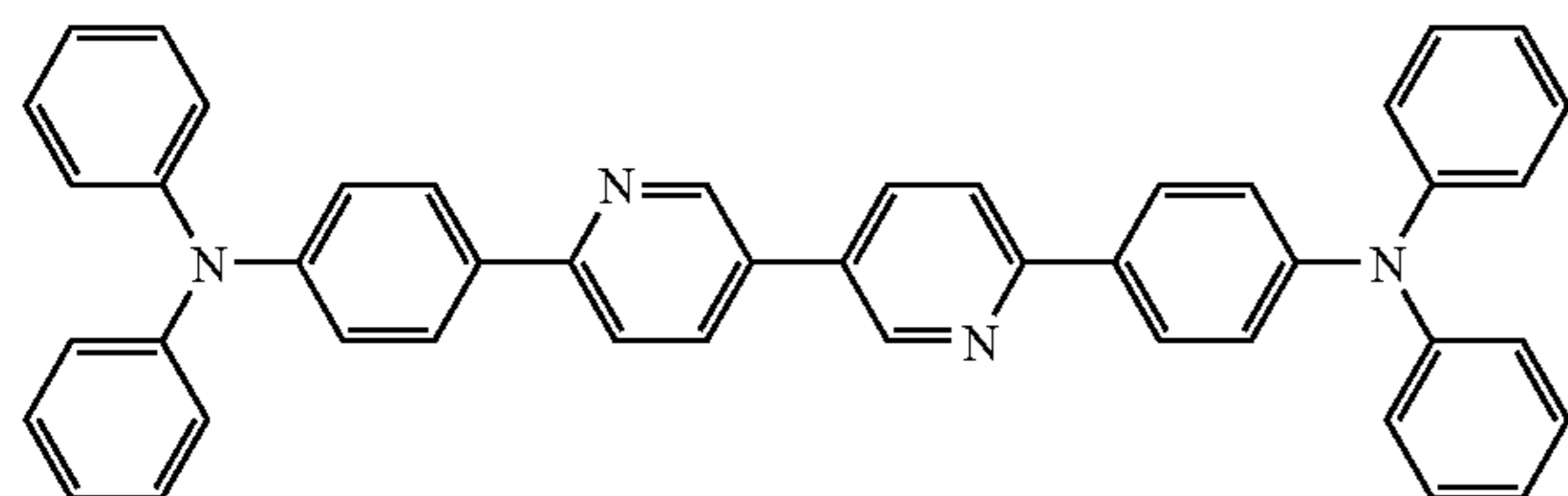
4,4'-(3,3'-bipyridine-6,6'-diyl)bis(N,N-diphenylaniline)
