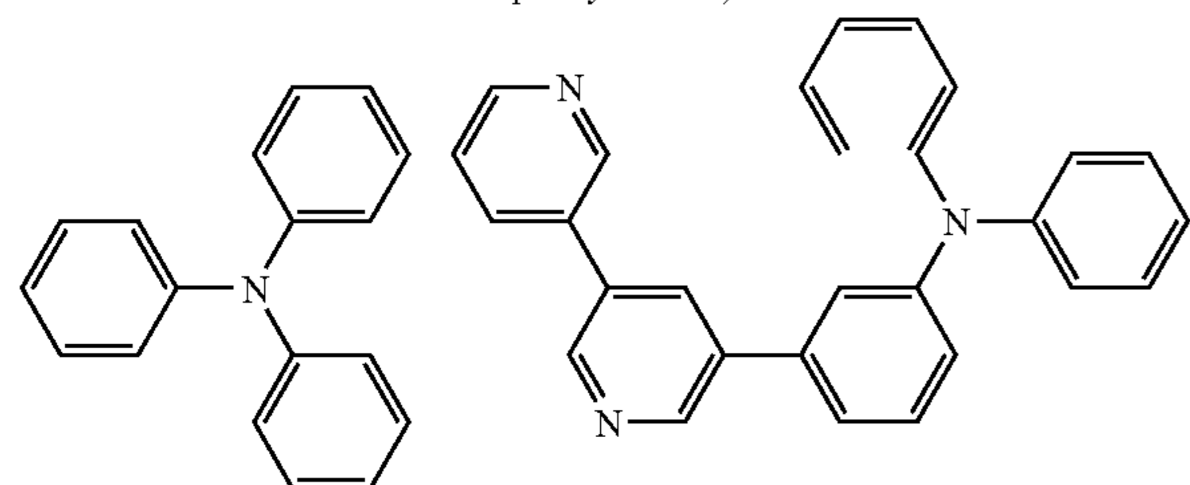
5,5'-bis(3-diphenylaminophenyl)-3,3'-bipyridine
