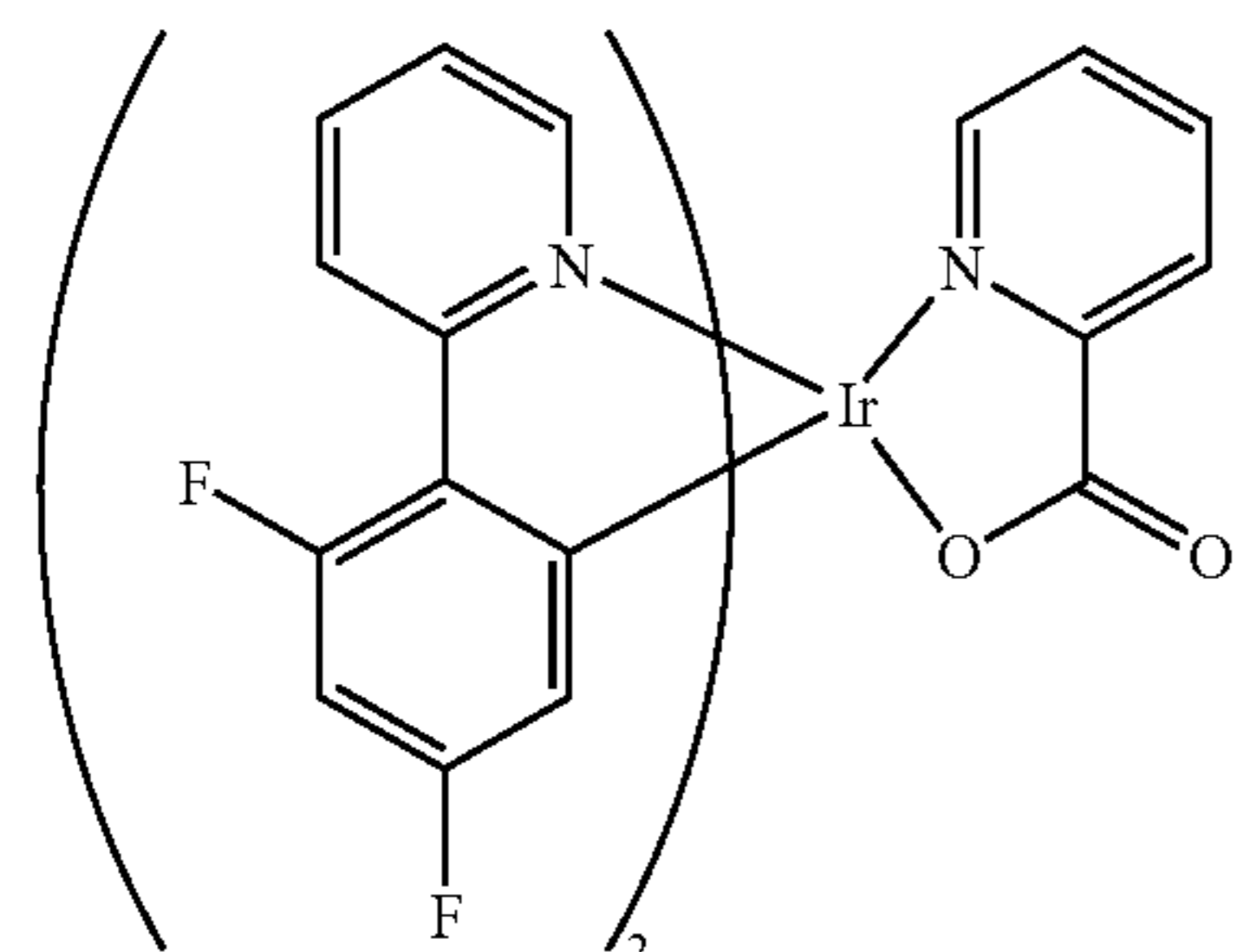
bis(2-[4,6-difluorophenyl]pyridinato-N,C2')iridium(III) picolinate [FIrPic]
