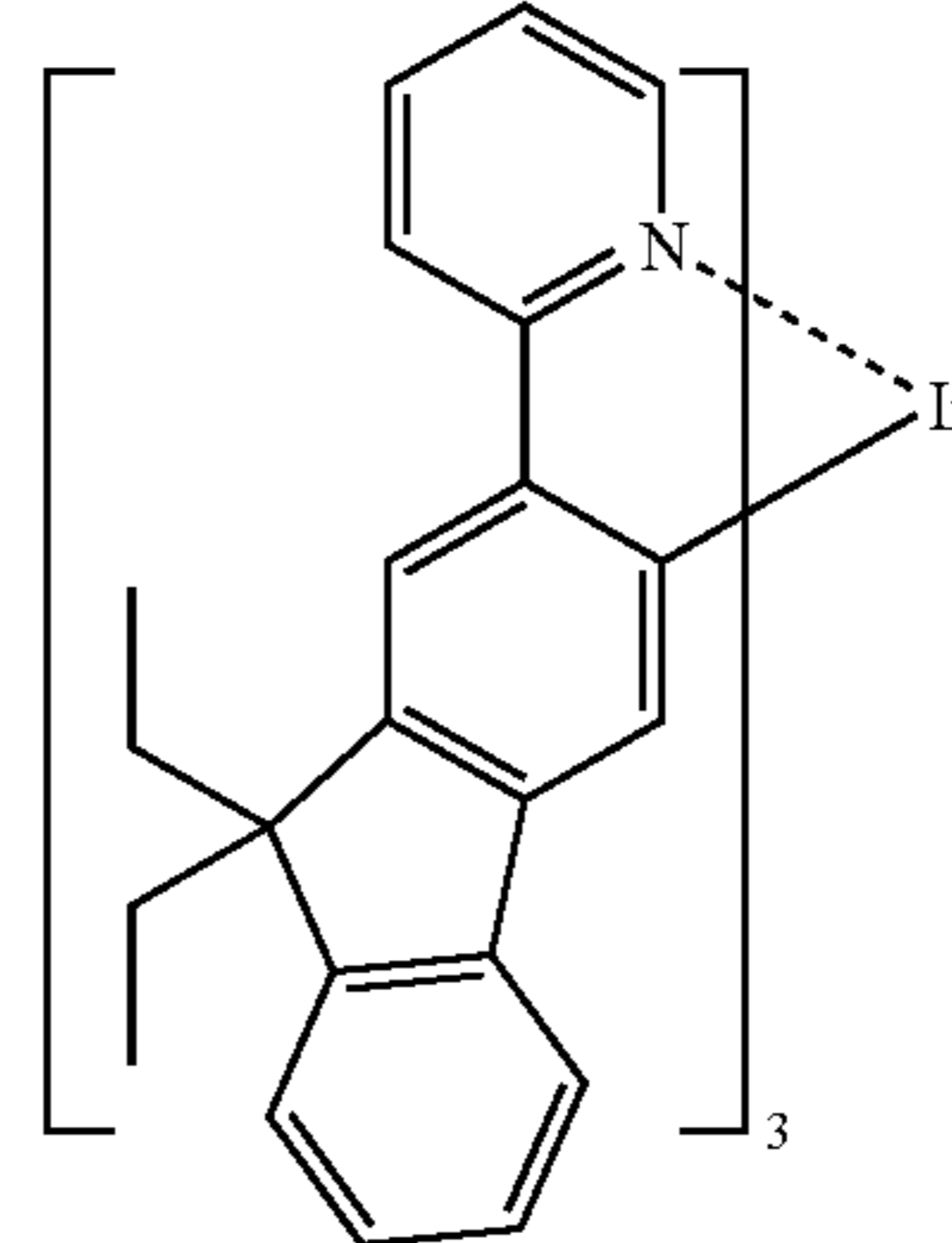
[Ir(Flpy) 3 ] Tris[2-(9,9-dimethylfluoren-2-yl)pyridinato-(N,C3')]iridium(III)
