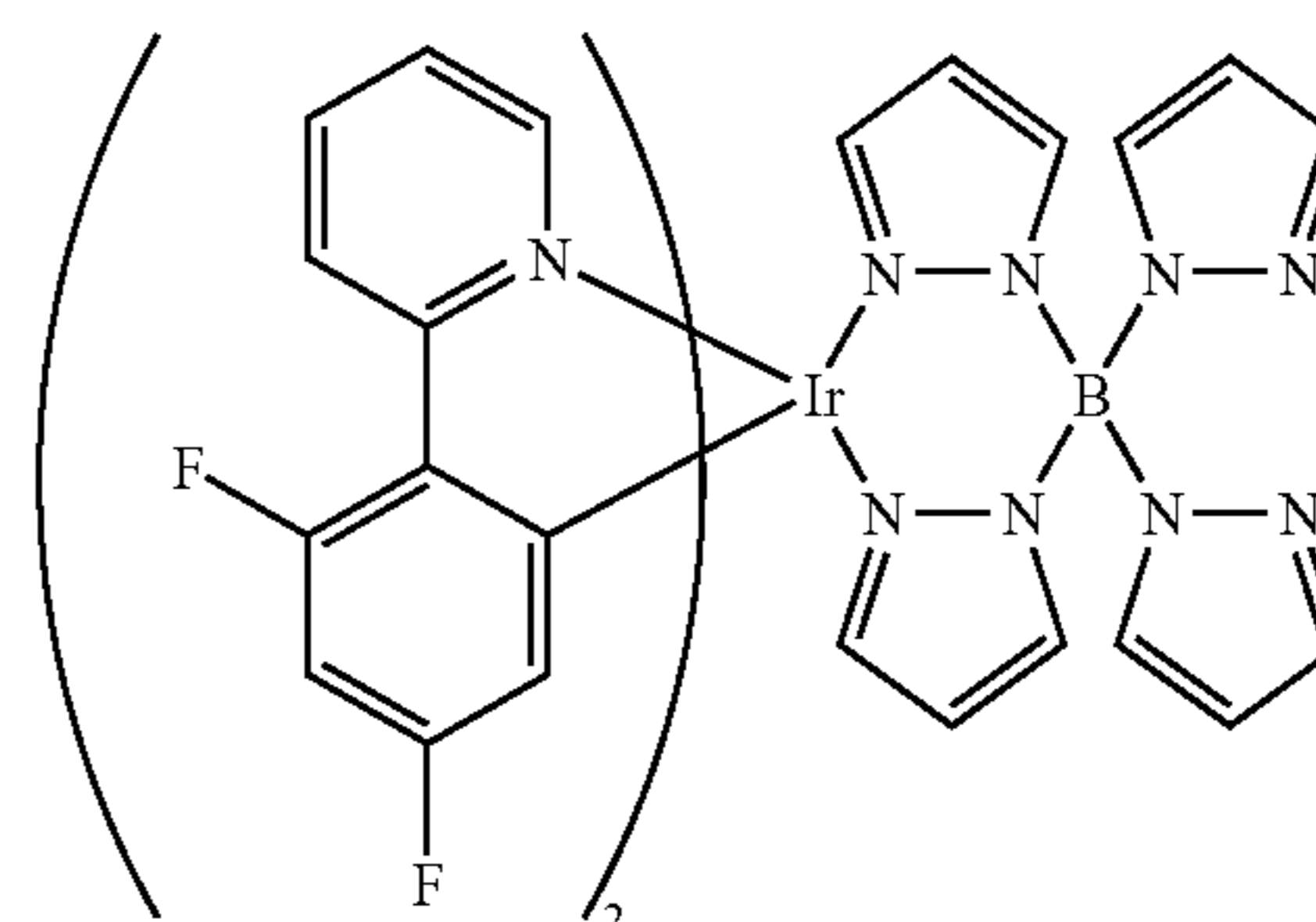
bis[2-(4,6-difluorophenyl)pyridinato-N,C2']iridium(III)tetra(1-pyrazolyl)borate (FIR6)
