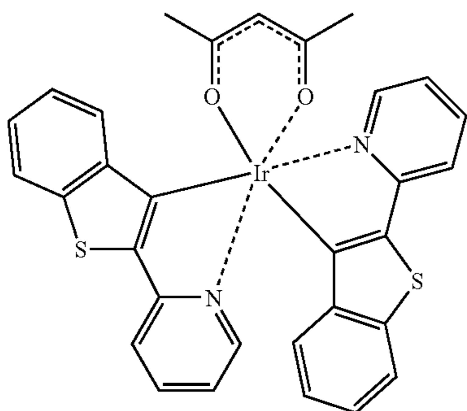
Ir(btp) 2 (acac)
