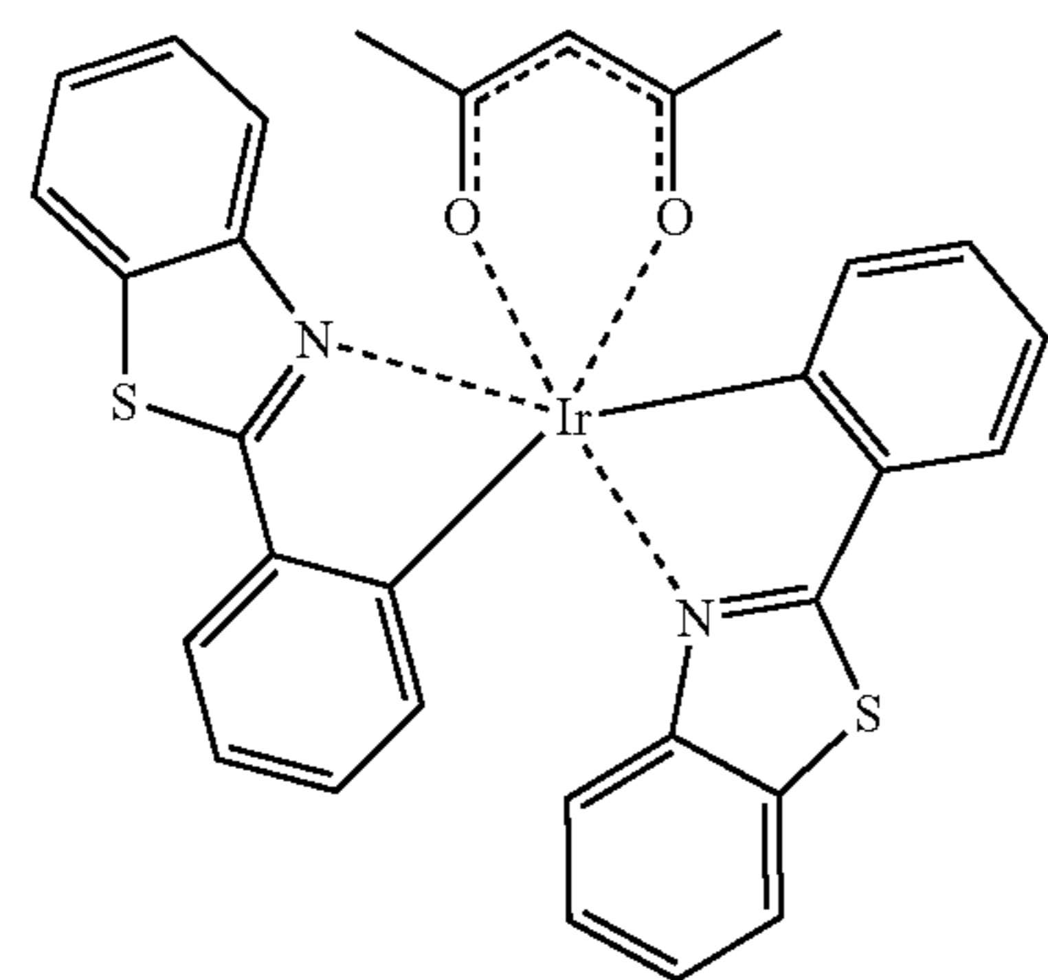
(bt) 2 Ir(III)(acac) Bis[2-phenylbenzothiazolato-N,C2'] iridium(III)(acetylacetonate)
