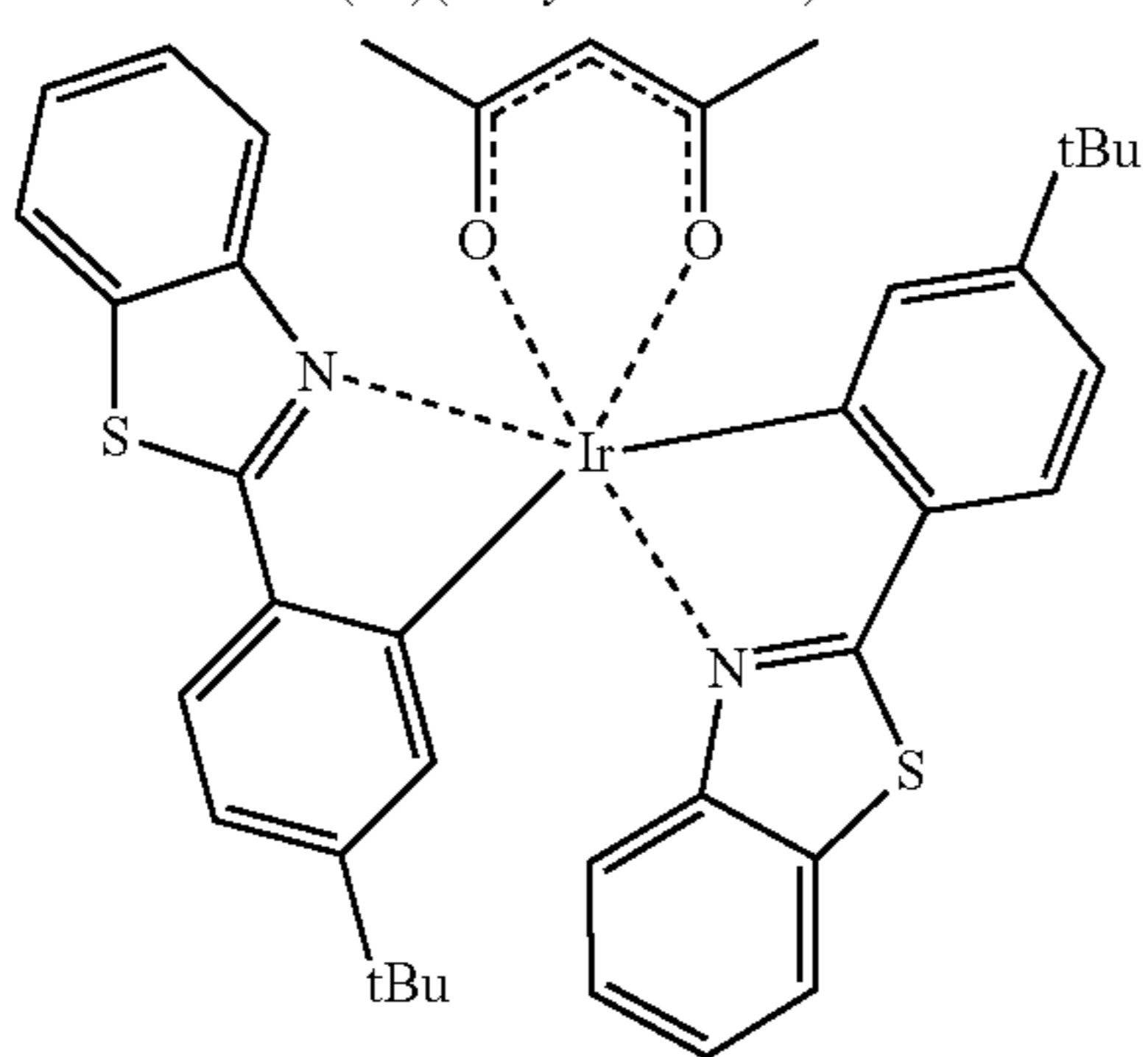
(t-bt) 2 Ir(III)(acac) Bis[2-(4-tert-butylphenyl)benzothiazolato-N,C2'] iridium(III)(acetylacetonate)
