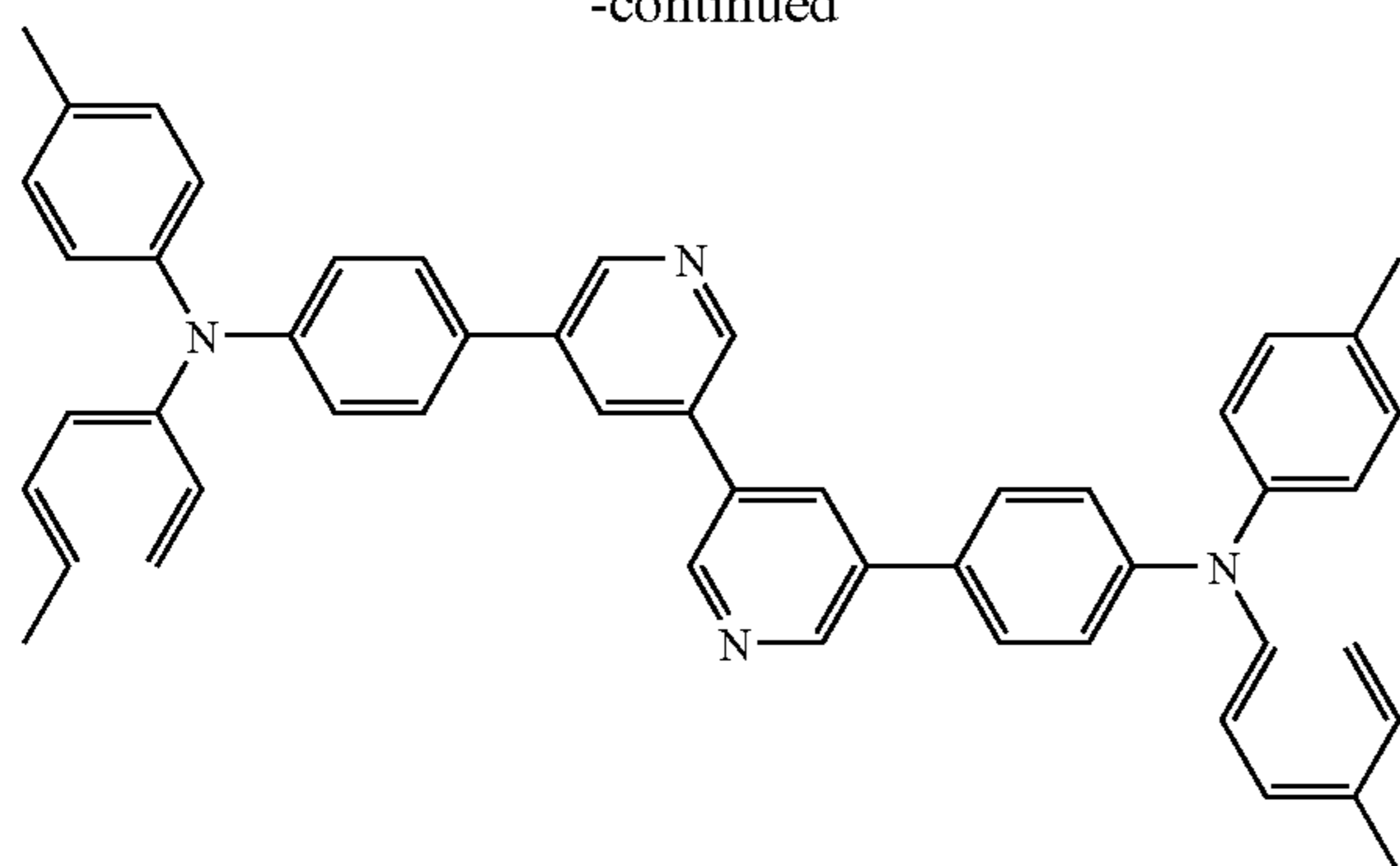
5,5'-bis(4-di(4-methylphenyl)aminophenyl)-3,3'-bipyridine
