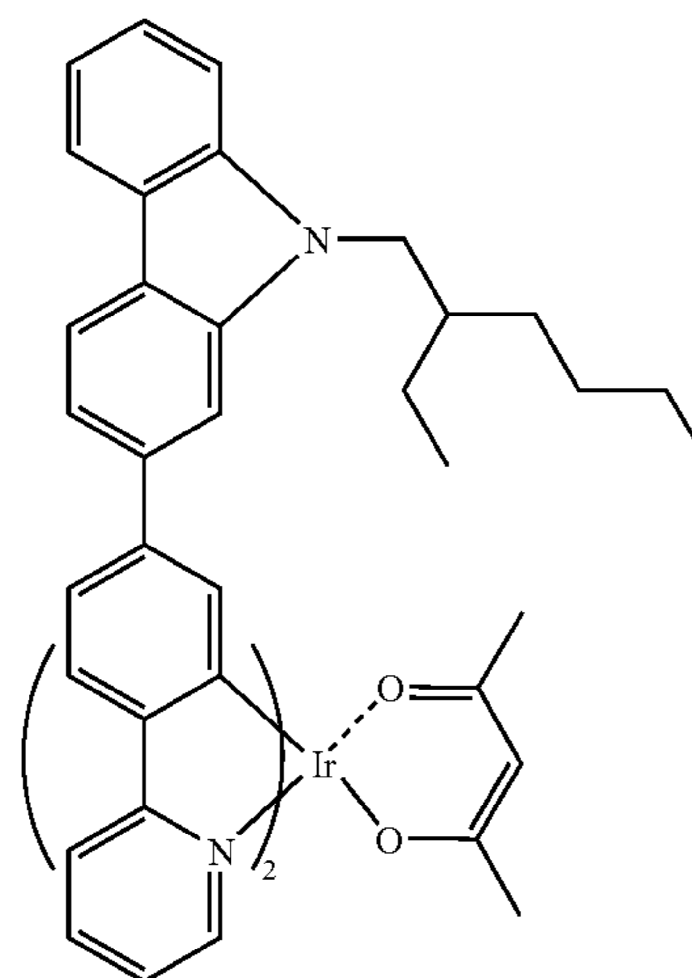
(2-PhPyCz) 2 Ir(III)(acac)
