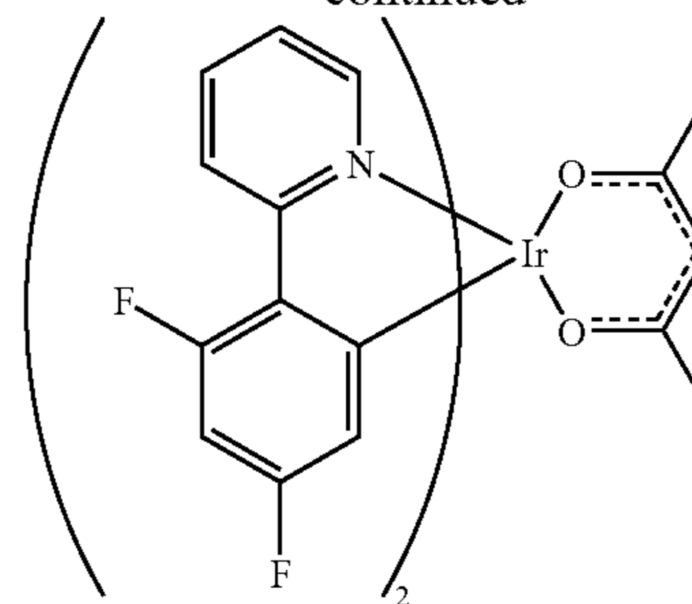
bis(2-[4,6-difluorophenyl]pyridinato-N,C2')iridium(acetylacetonate) [FIr(acac)]
