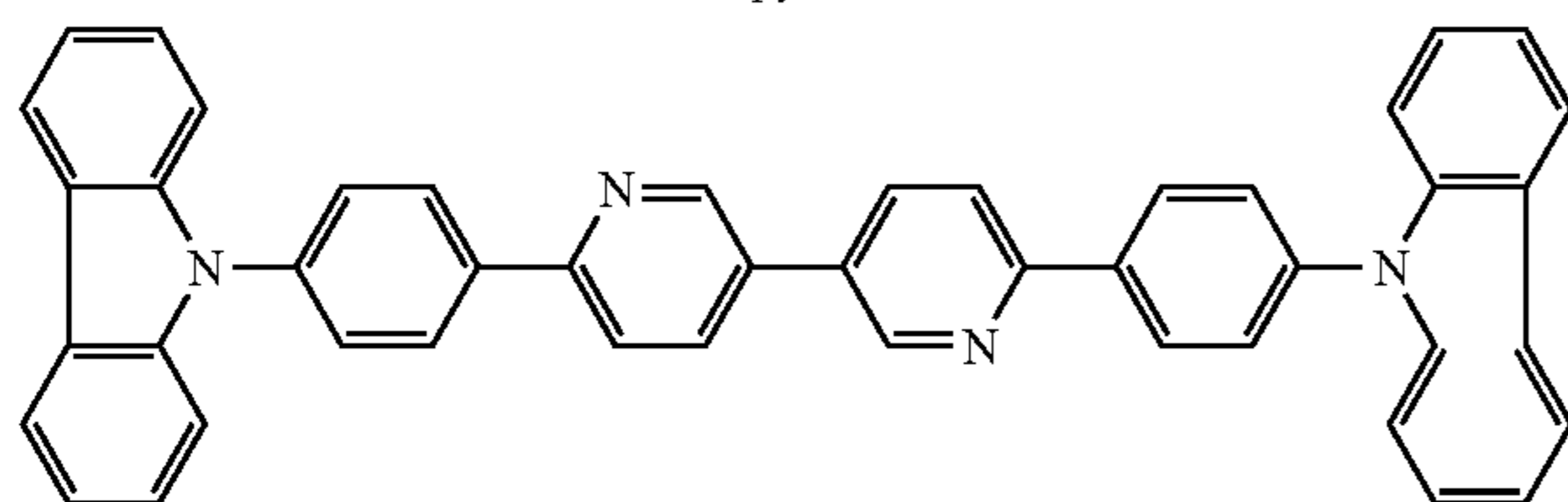
6,6'-bis(4-(carbazol-9-yl)phenyl)-3,3'-bipyridine
