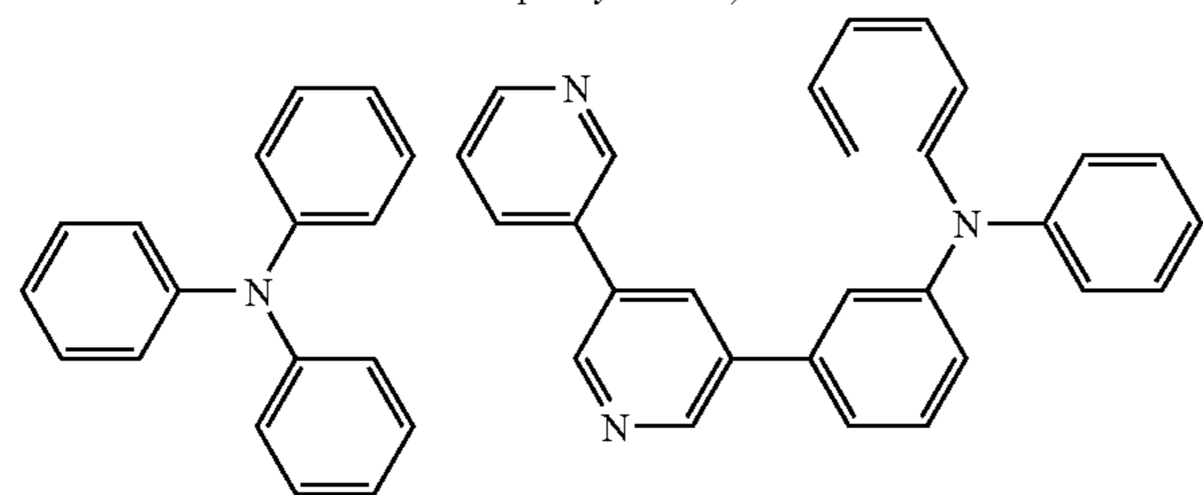
5,5'-bis(3-diphenylaminophenyl)-3,3'-bipyridine
