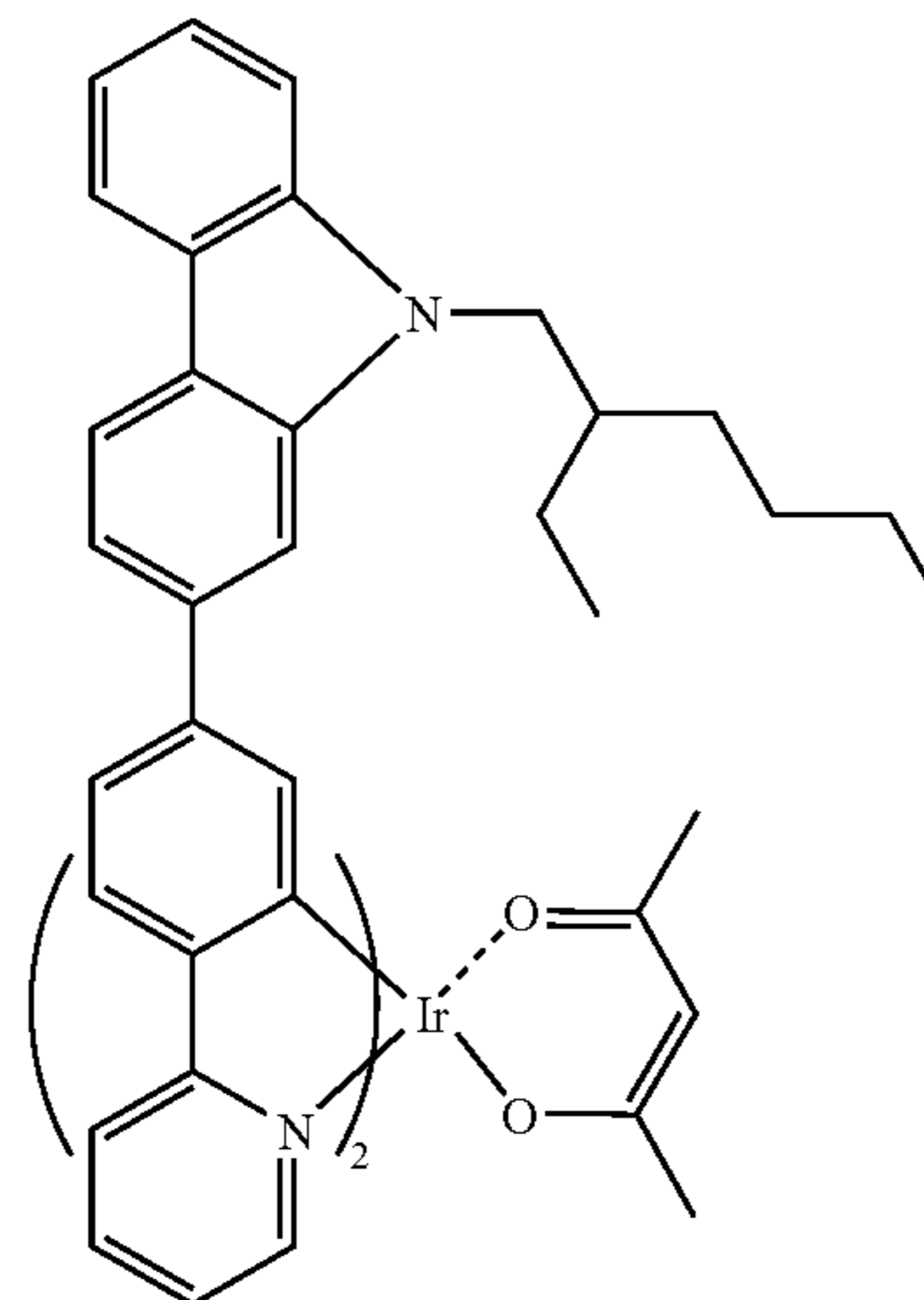
(2-PhPyCz) 2 Ir(III)(acac)
