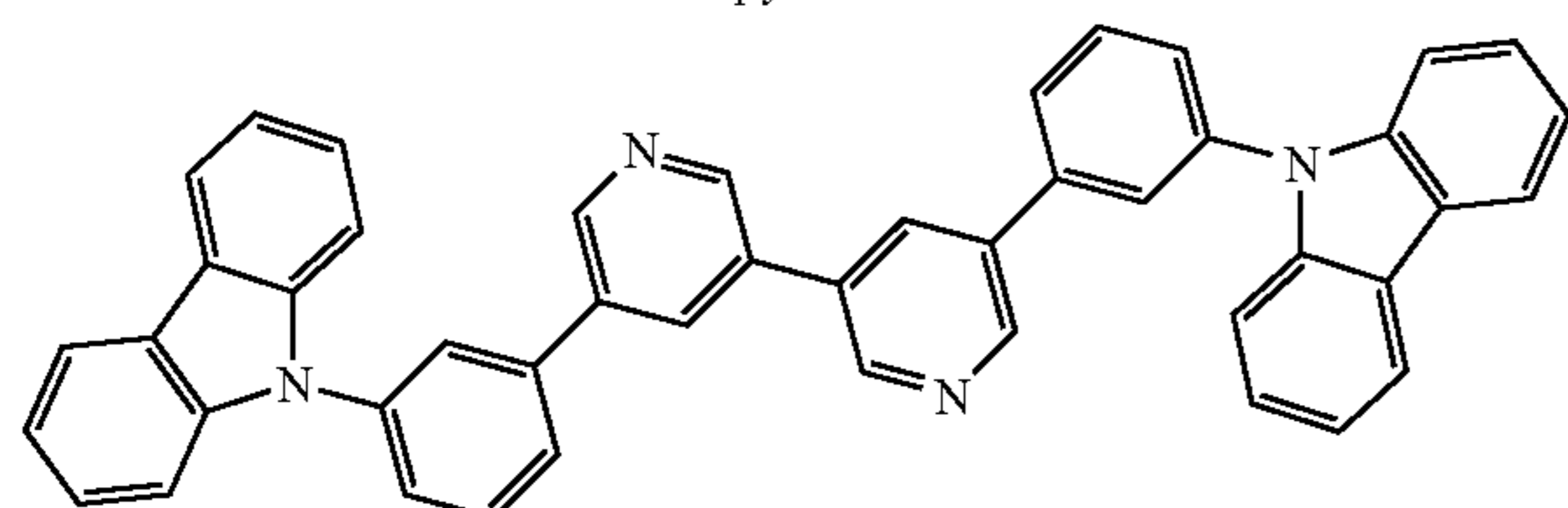
5,5'-bis(3-(carbazol-9-yl)phenyl)-3,3'-bipyridine
