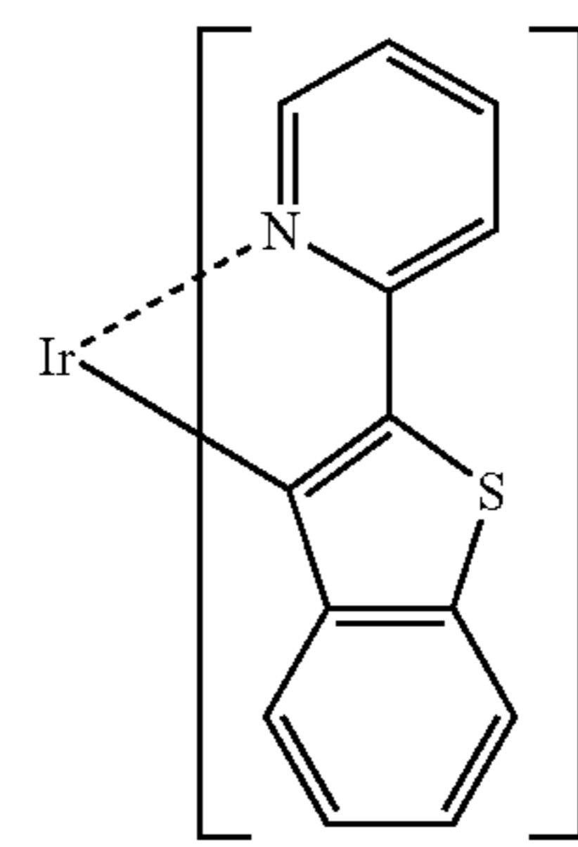
Ir(btp) 3
