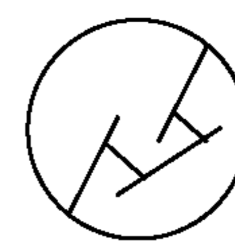
Moderately branched molecule of 3 units
