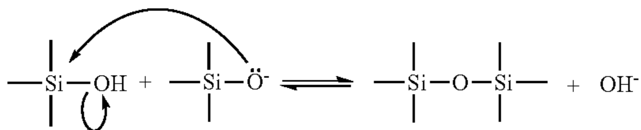
FIG 10: Nucleophilic Attack to Form Siloxane Bond
