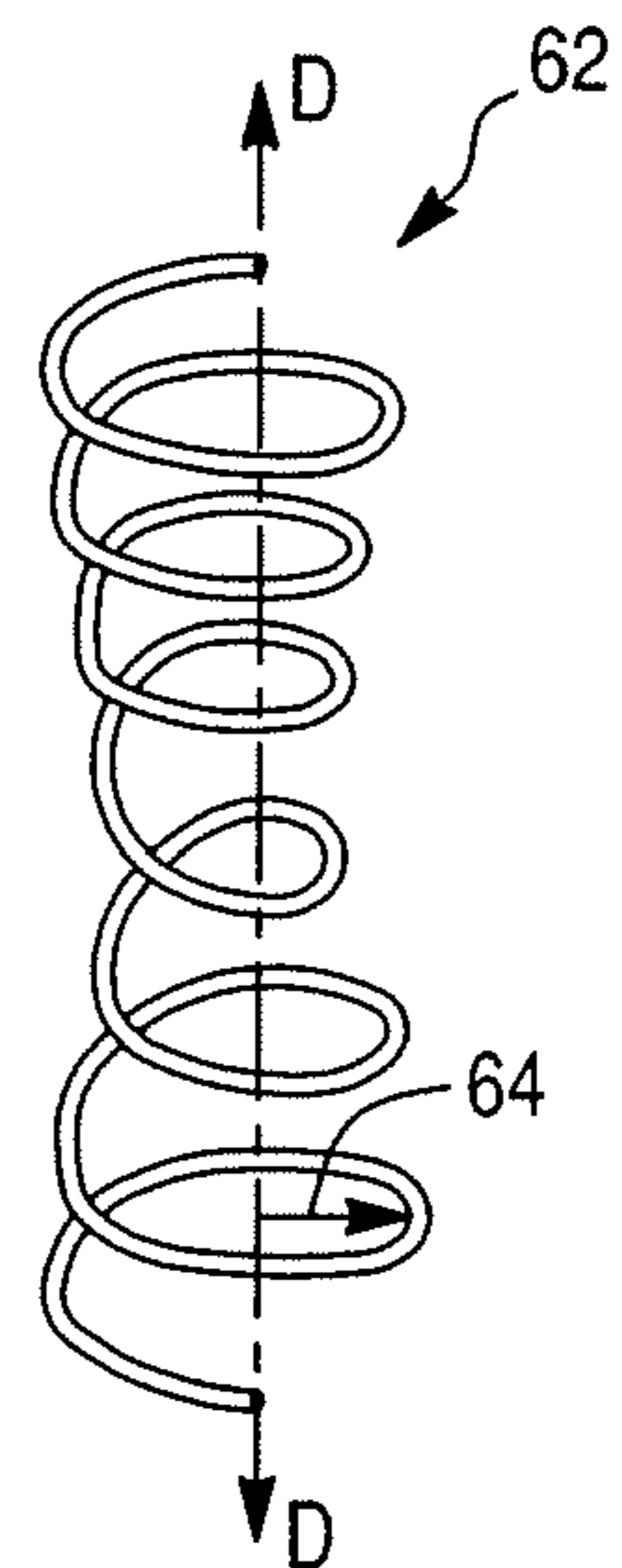
Fig. 3C Prior Art
