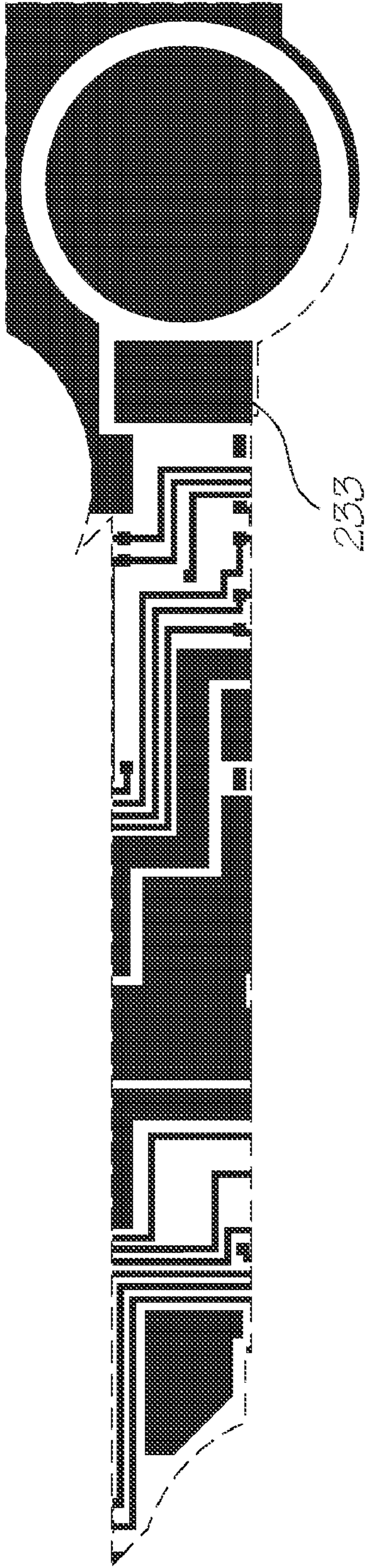
Metal 2 mask
