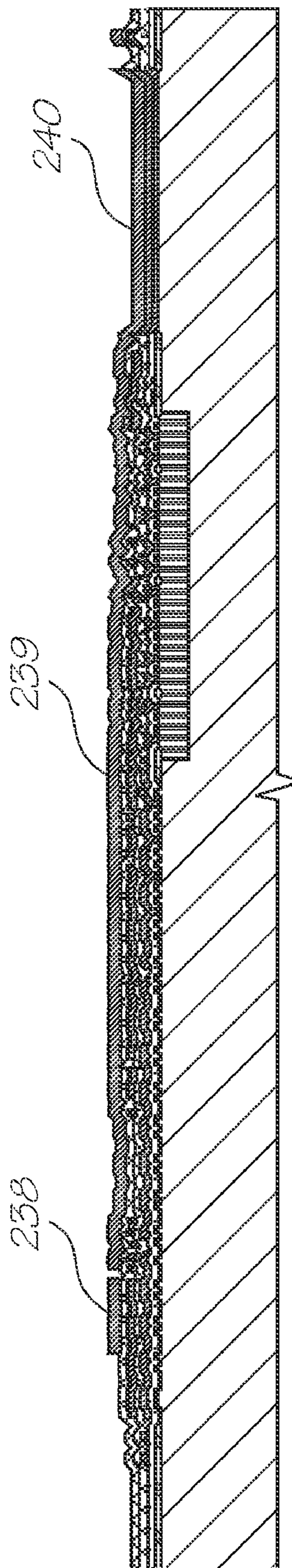
Deposit metal 3
