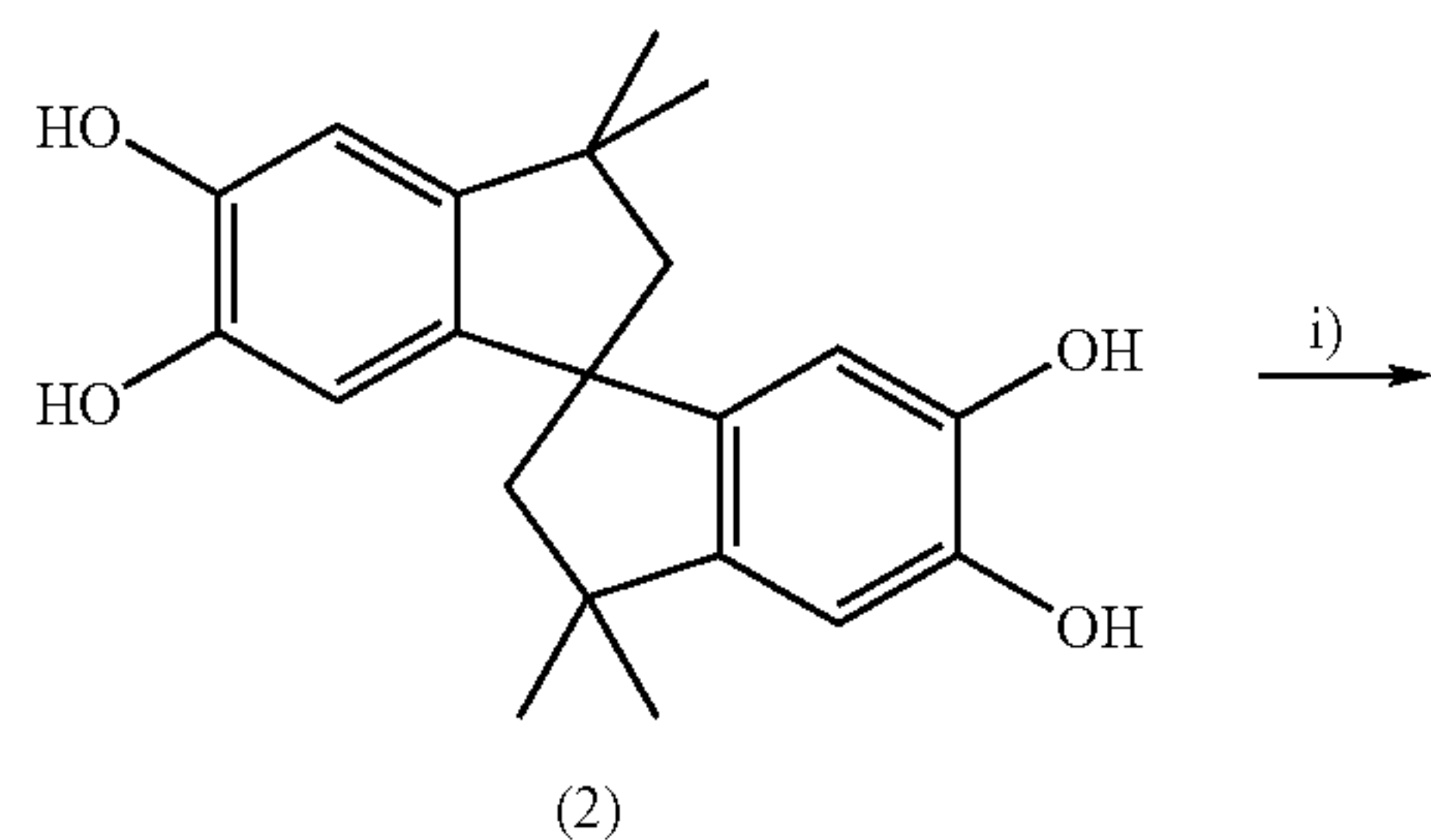
Reaction scheme C:
