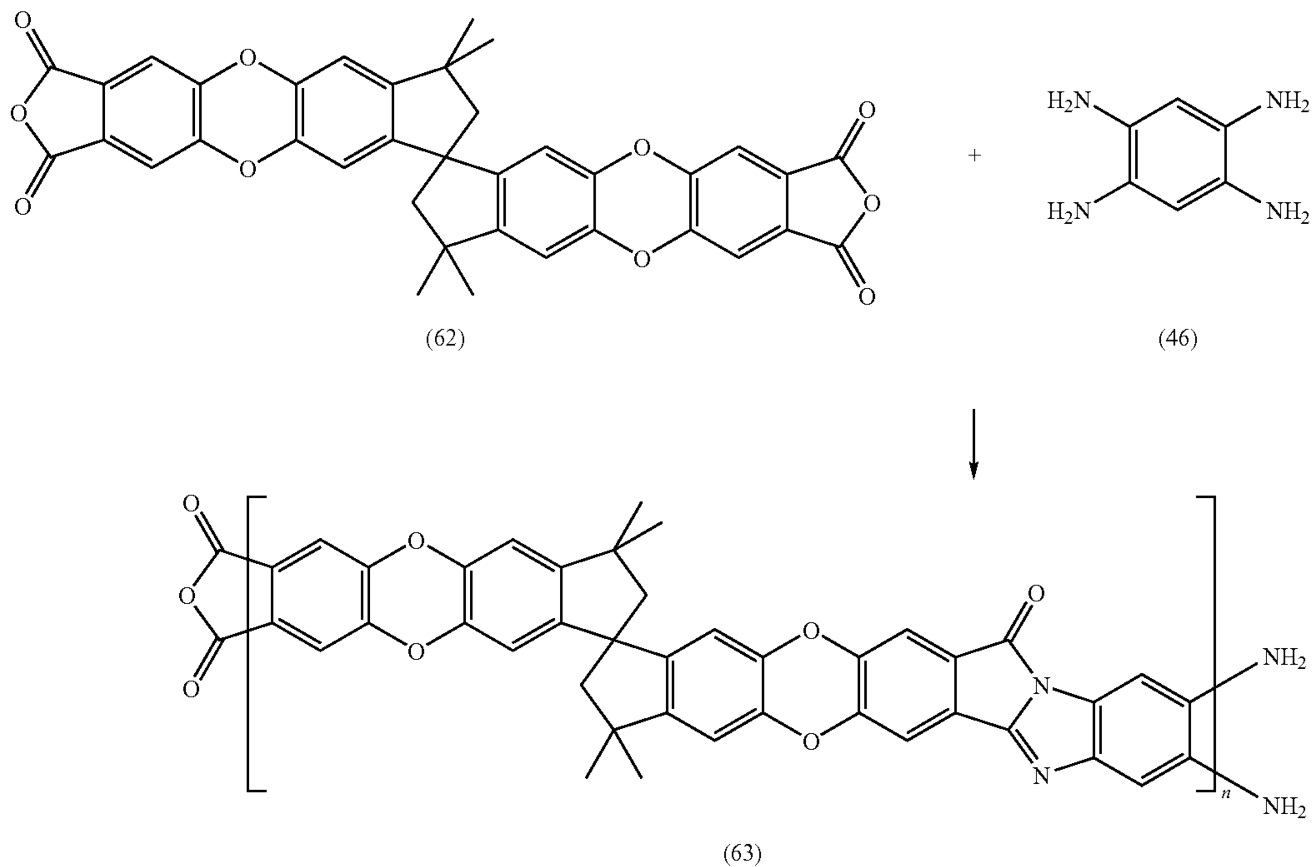
Reaction scheme F
