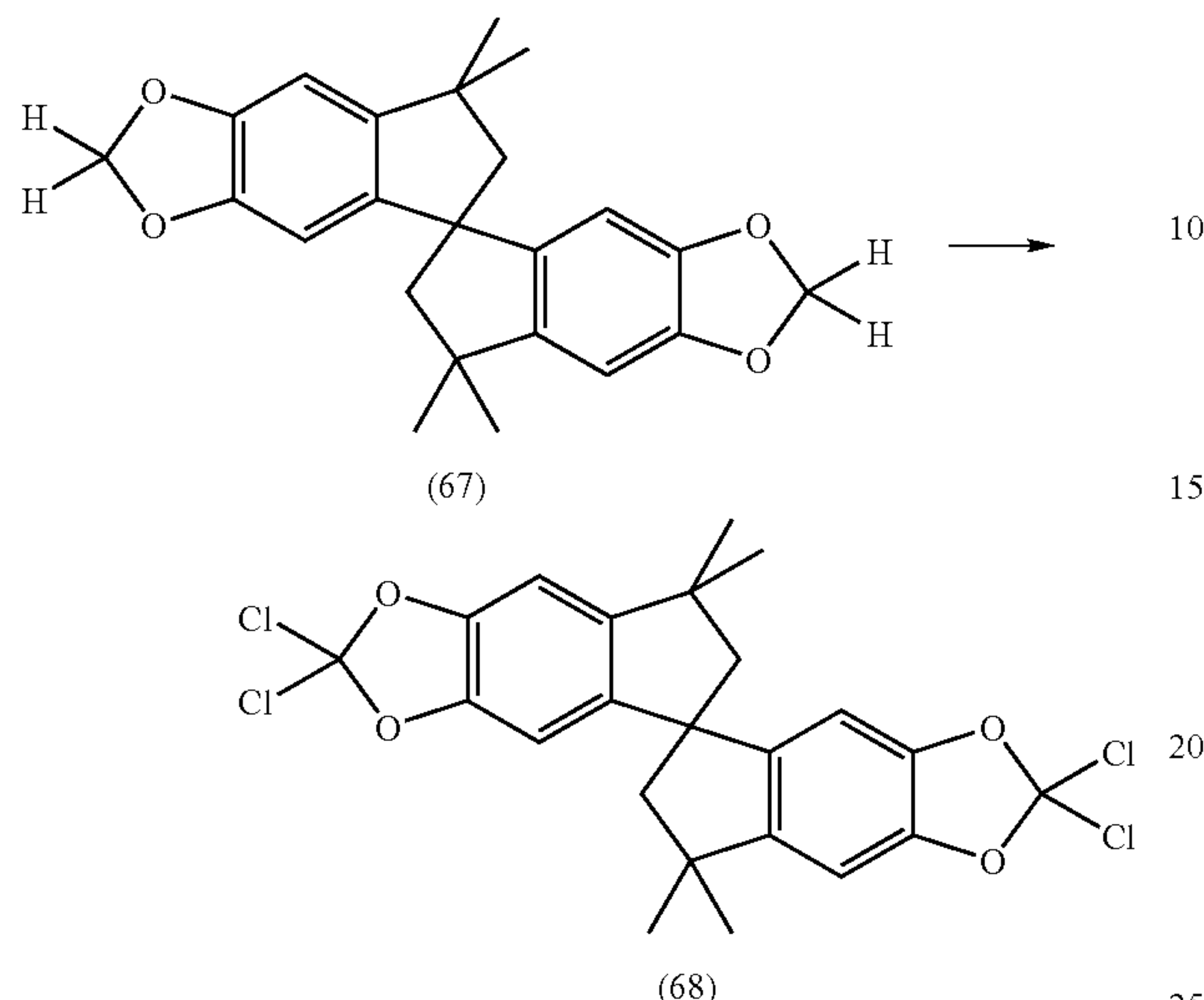
Reaction scheme H
