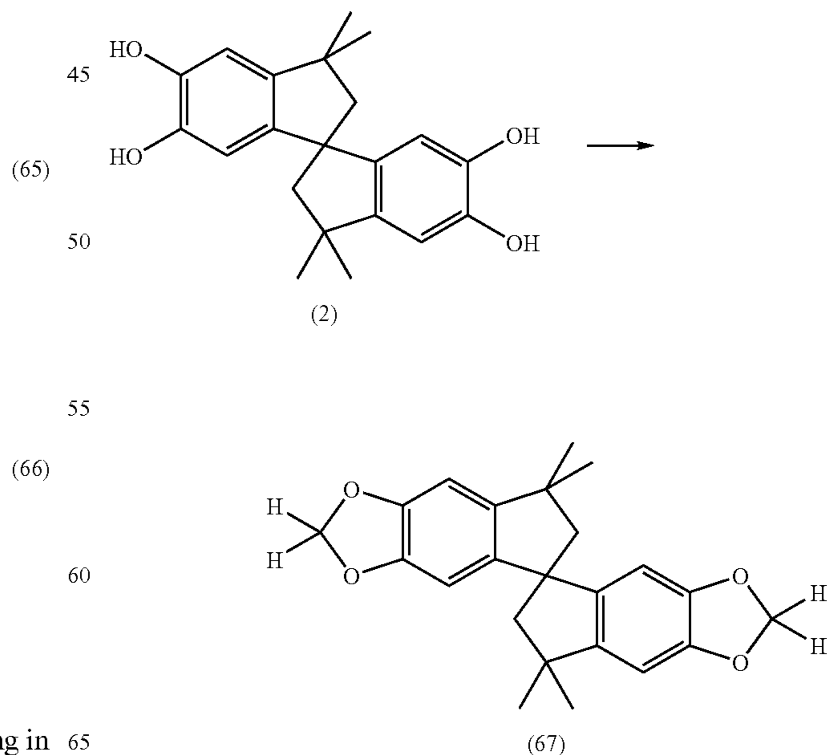
Reaction scheme G
