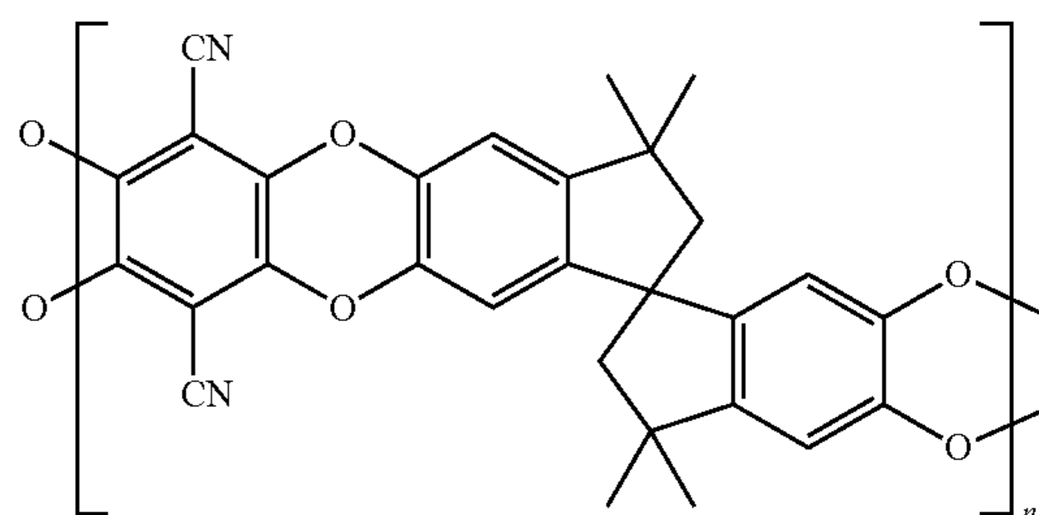
Polydioxane A (1)
