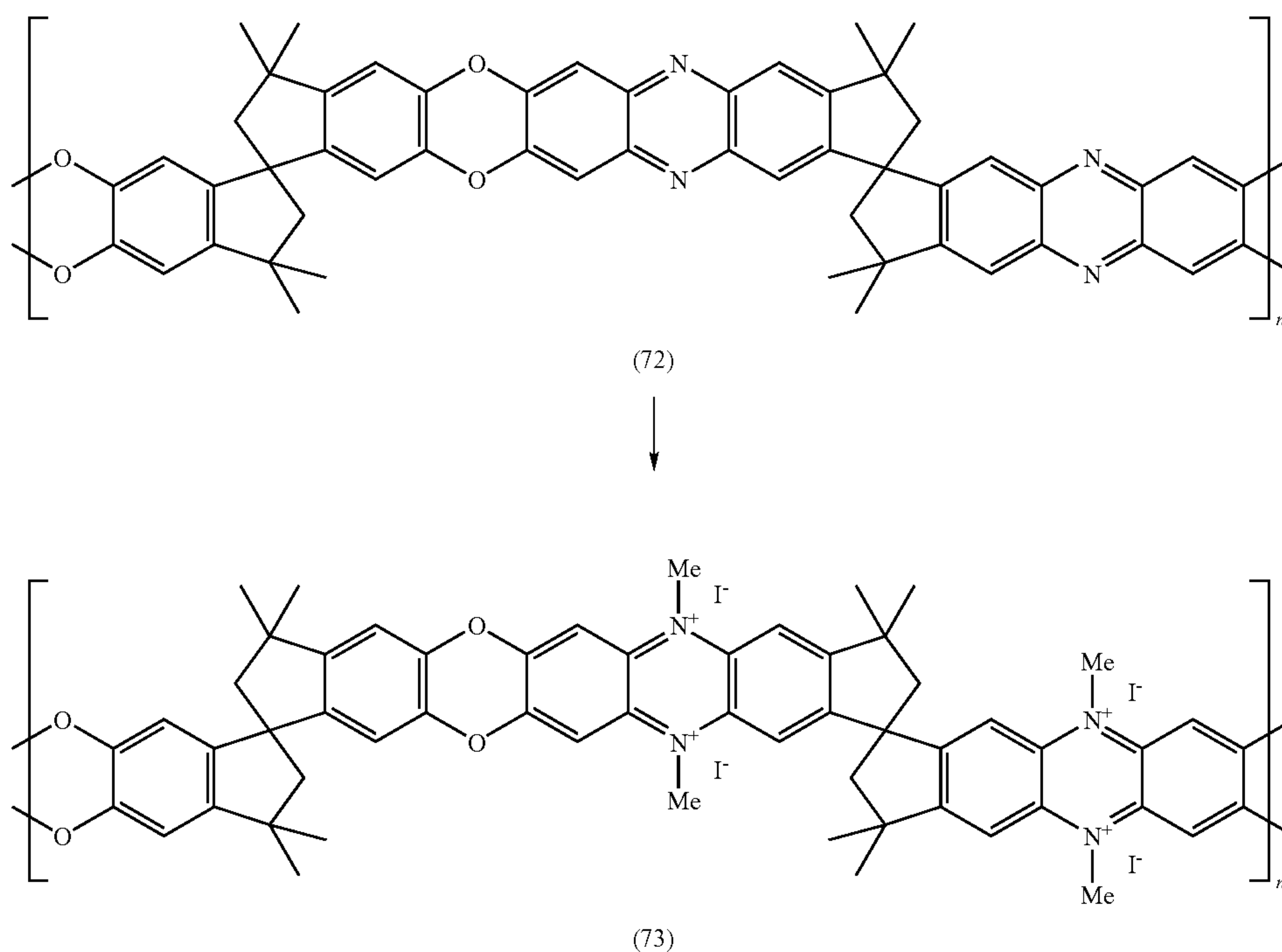
Reaction scheme L
