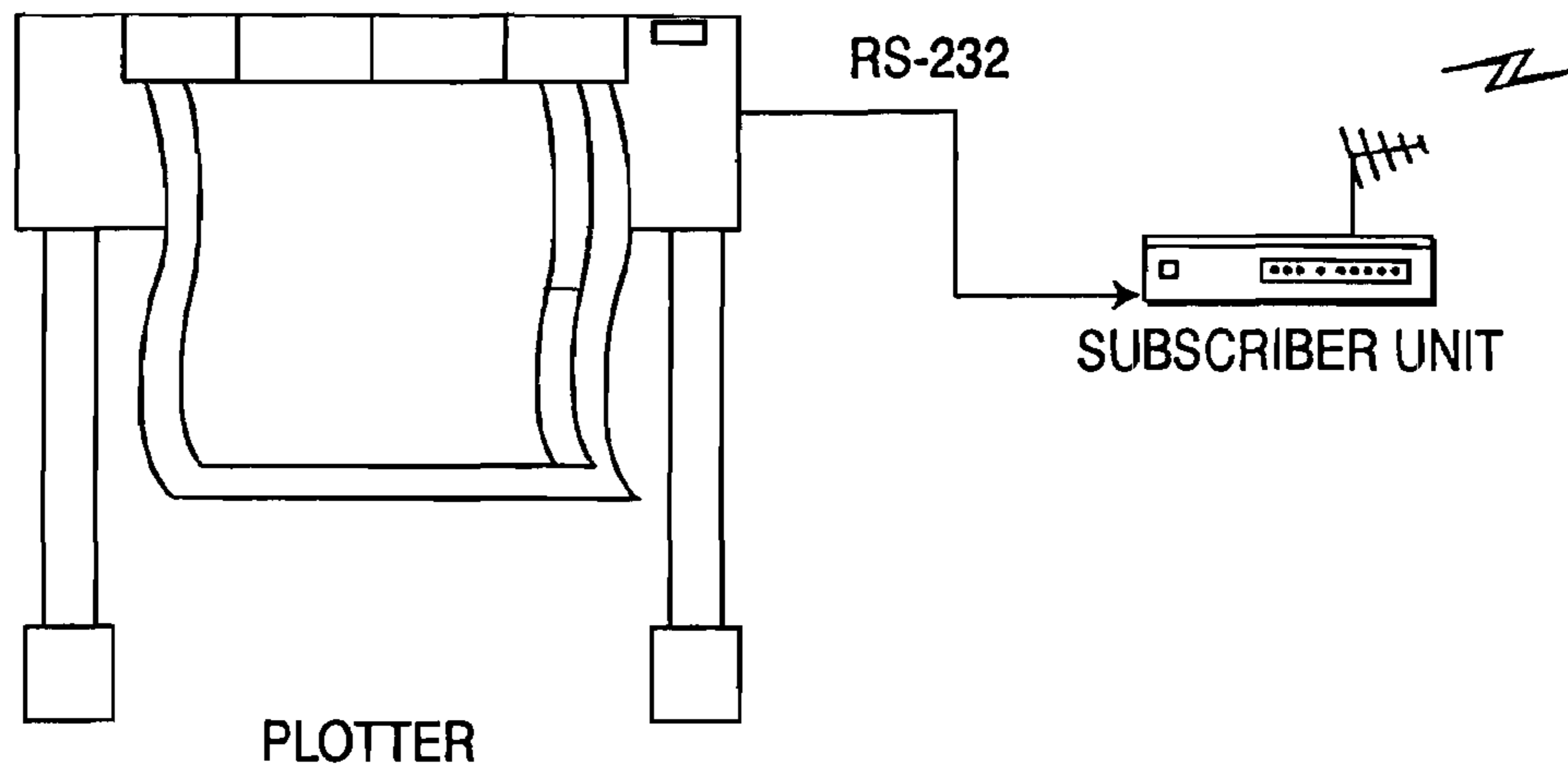
WIDEBAND CONNECTION FIG. 2D
