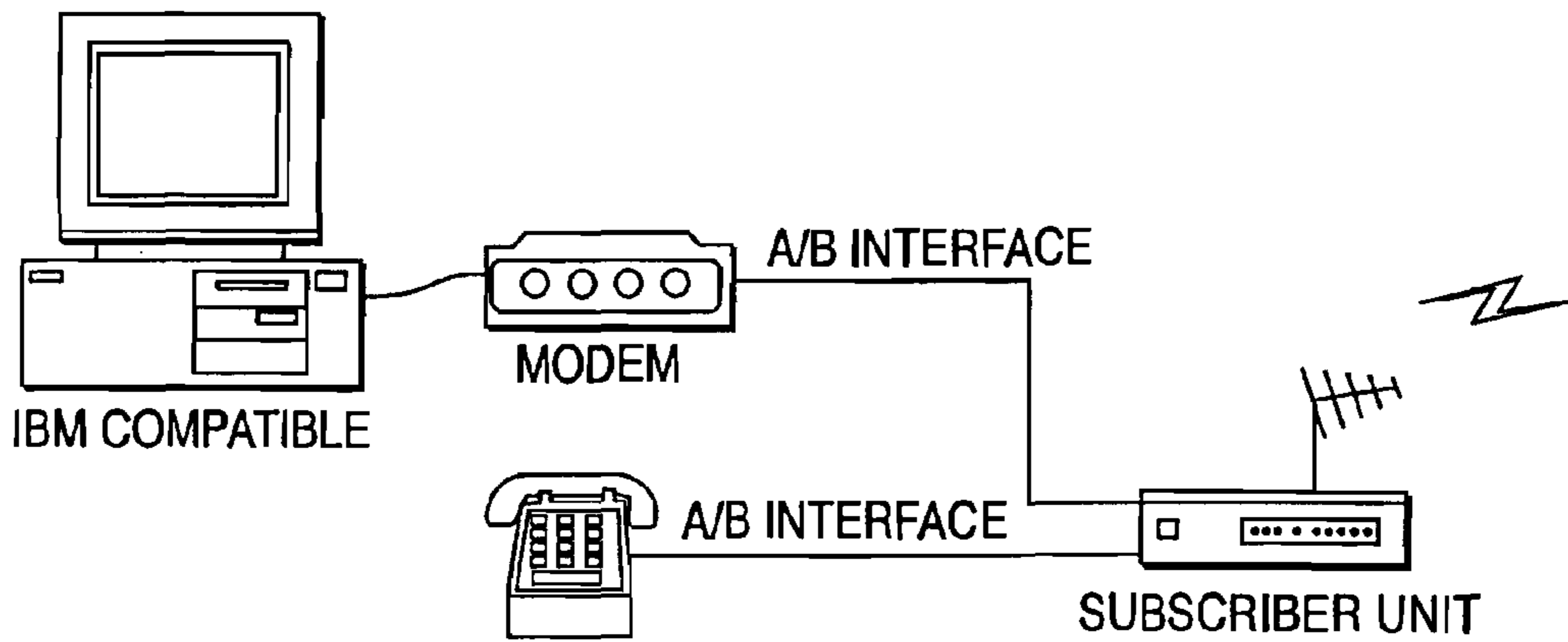
POTS TERMINAL INTERFACE FIG. 2B
