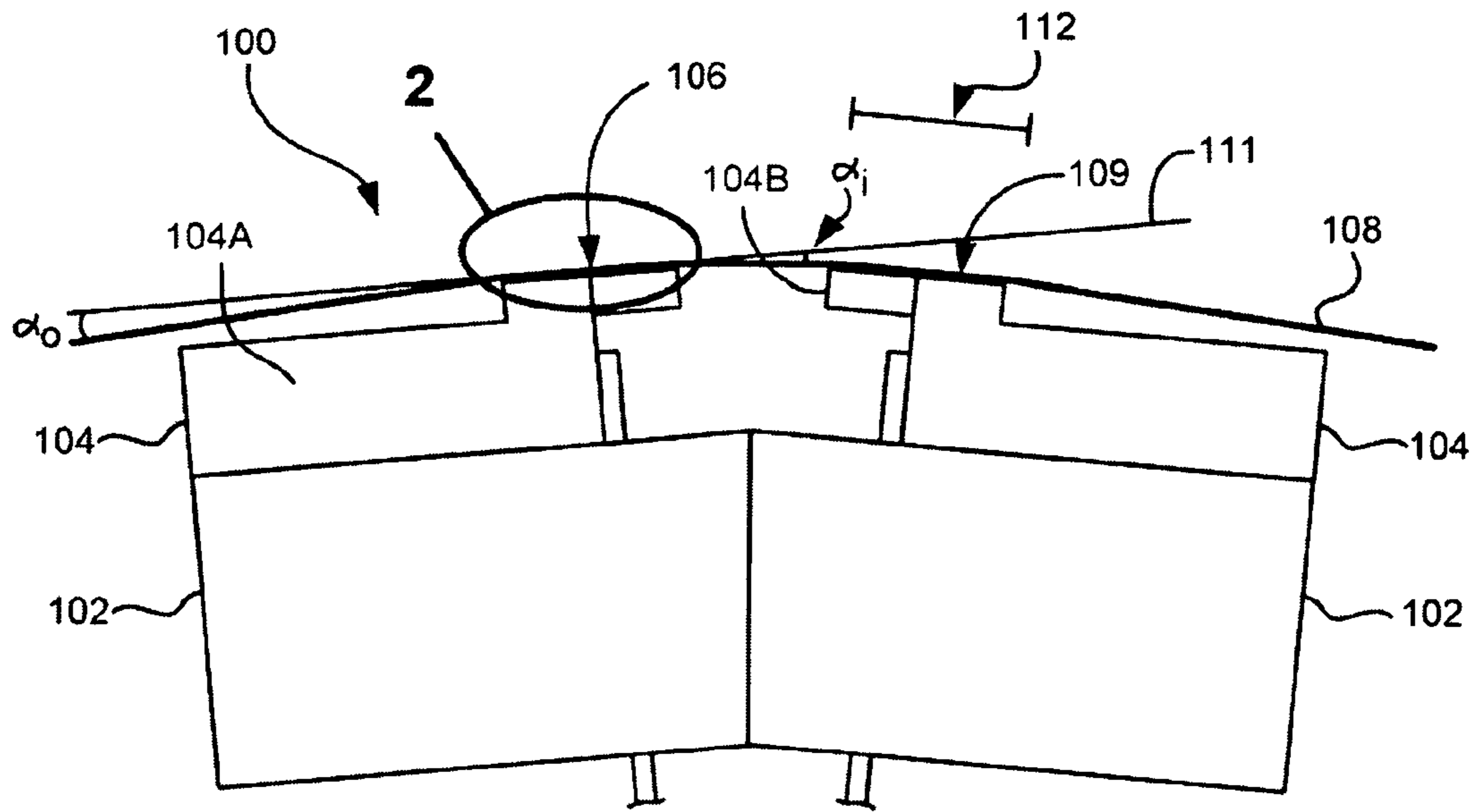
FIG. 1 (prior art)
