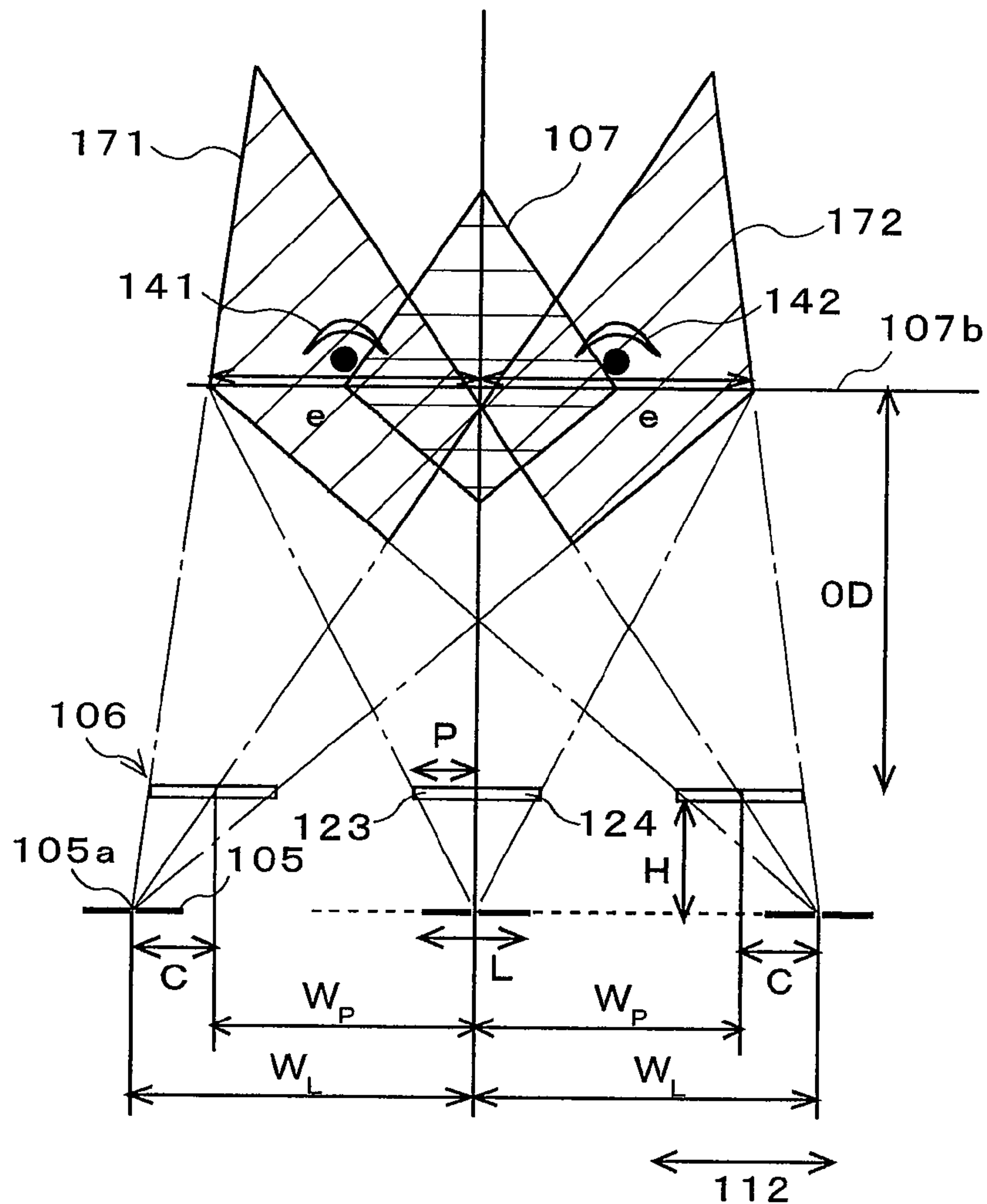
FIG. 7 (PRIOR ART)
