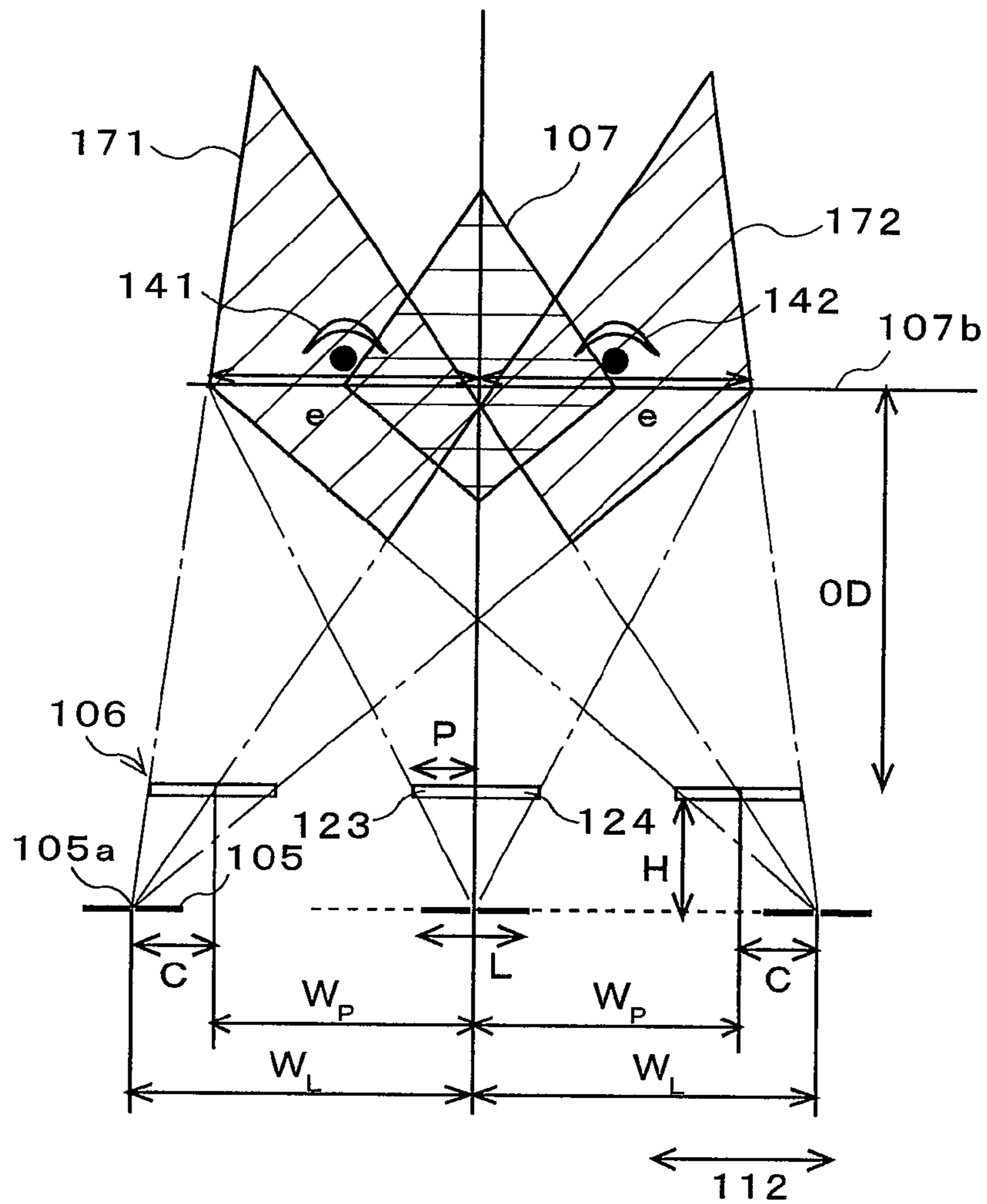
FIG. 7 (PRIOR ART)
