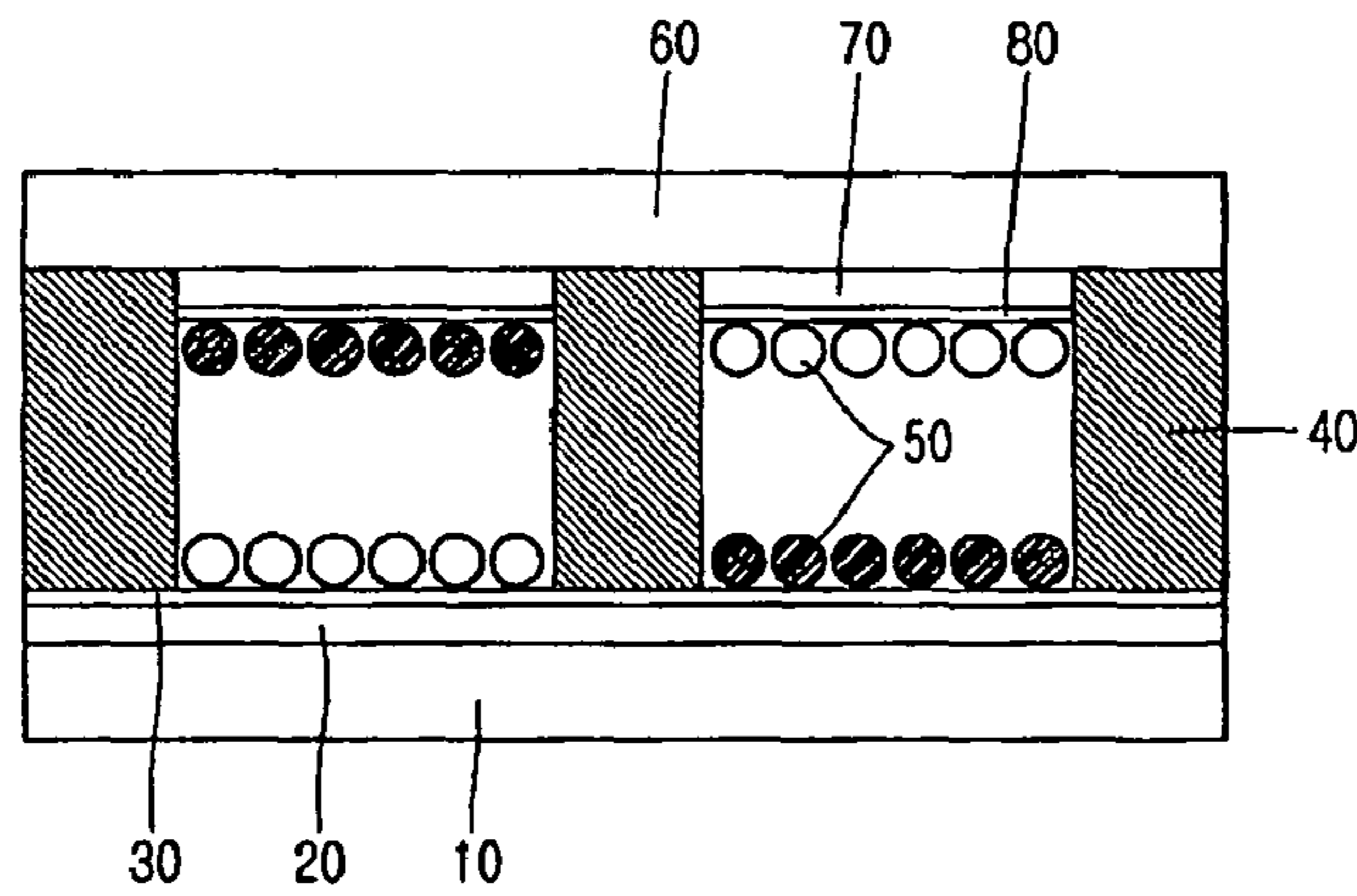
FIG. 1 PIROR ART
