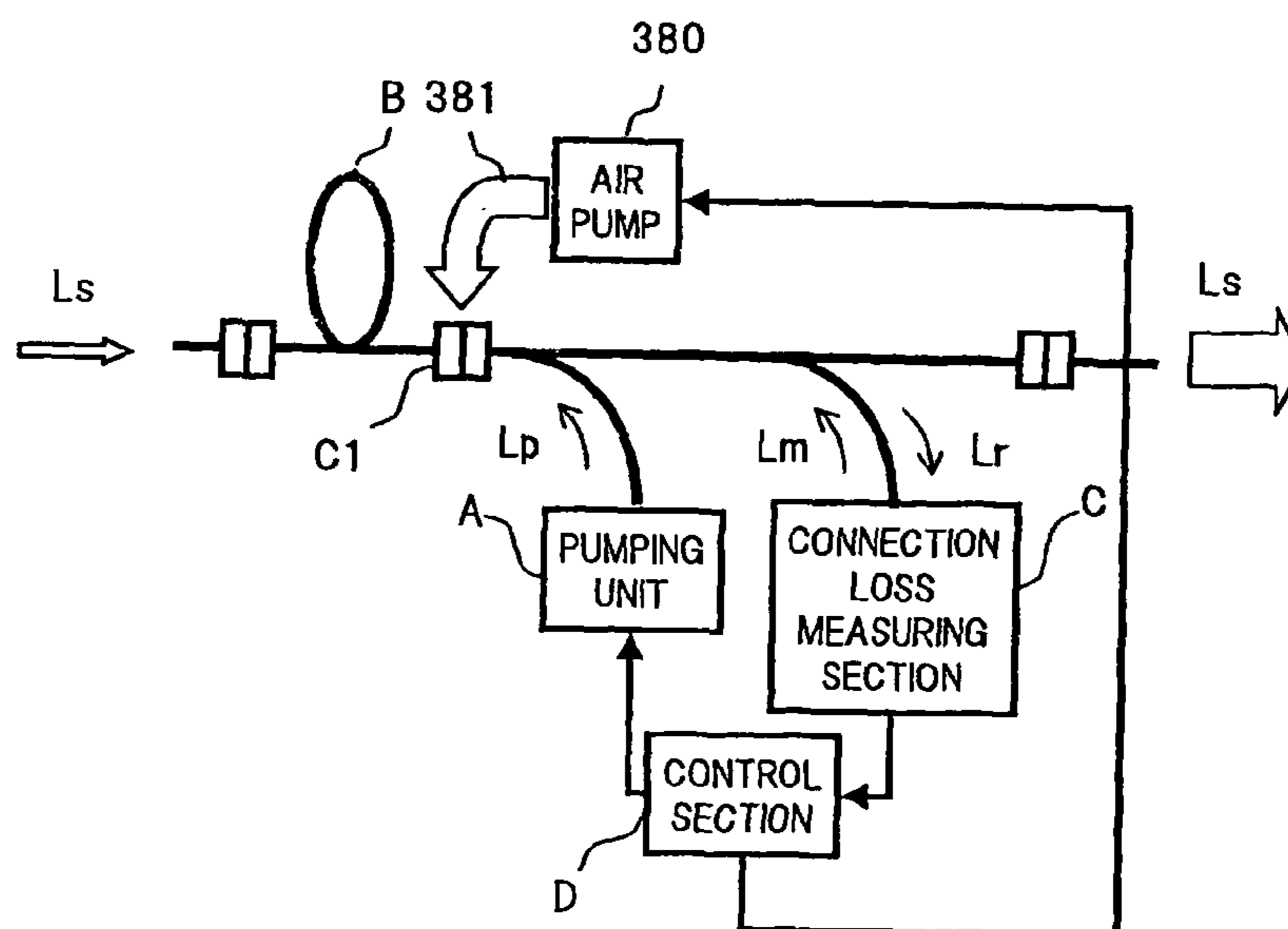
CONFIGURATION OF EMBODIMENT 3-5 OF PRESENT INVENTION
