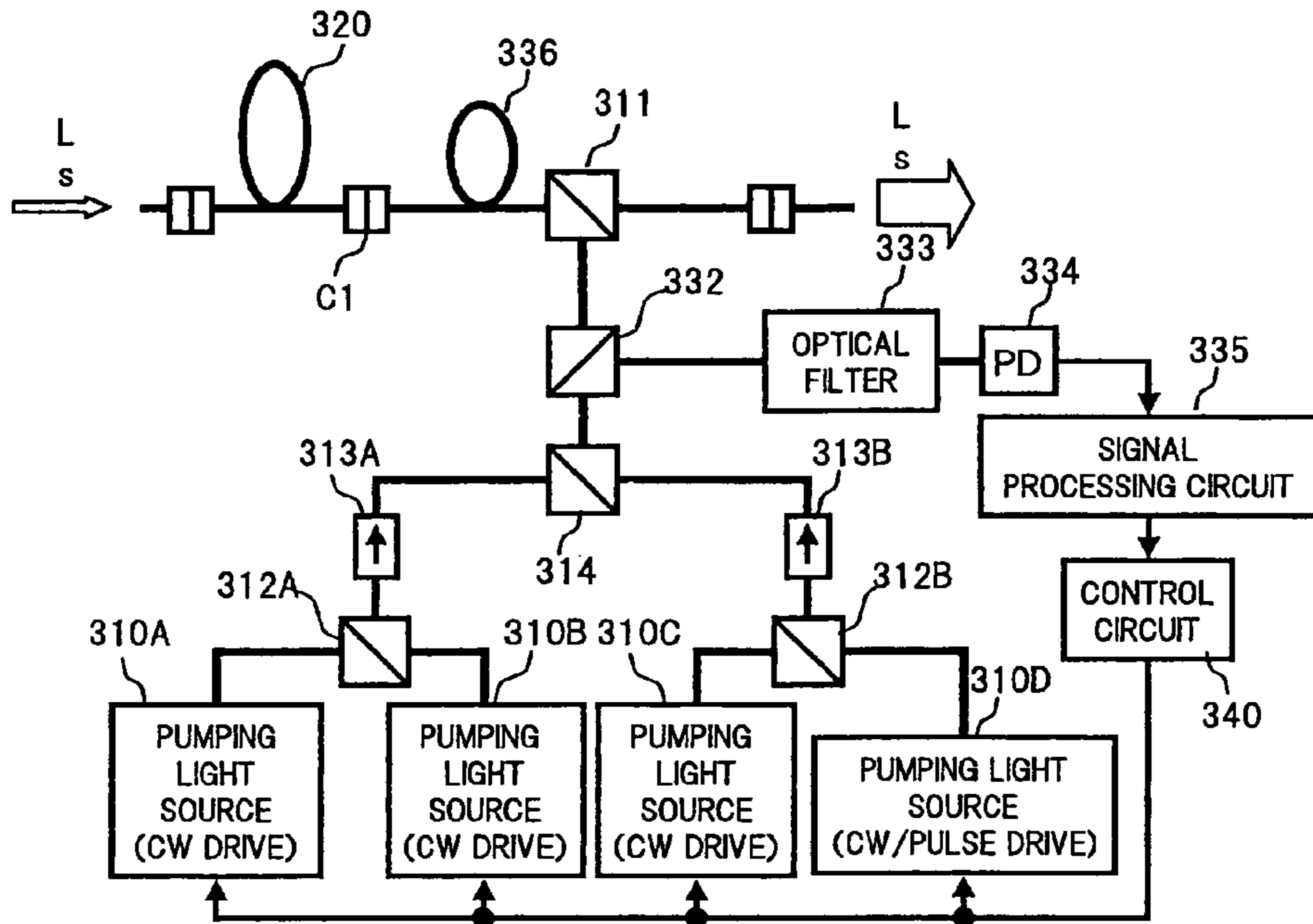
CONFIGURATION OF EMBODIMENT 3-3 OF PRESENT INVENTION
