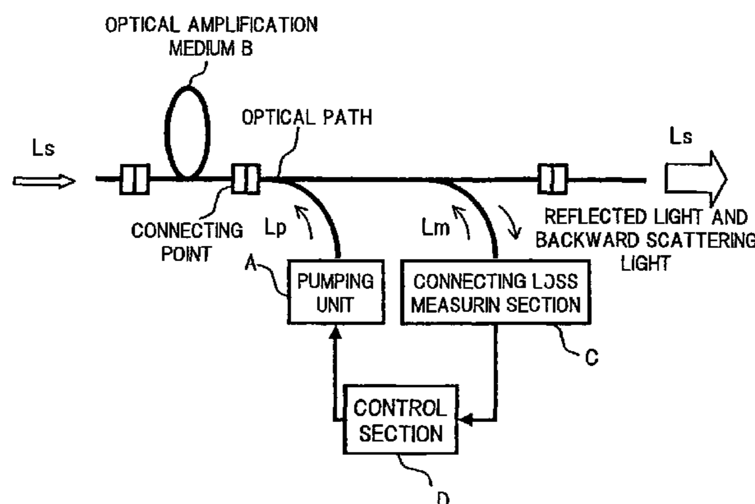
BASIC CONFIGURATION OF EMBODIMENT 3 OF PRESENT INVENTION
