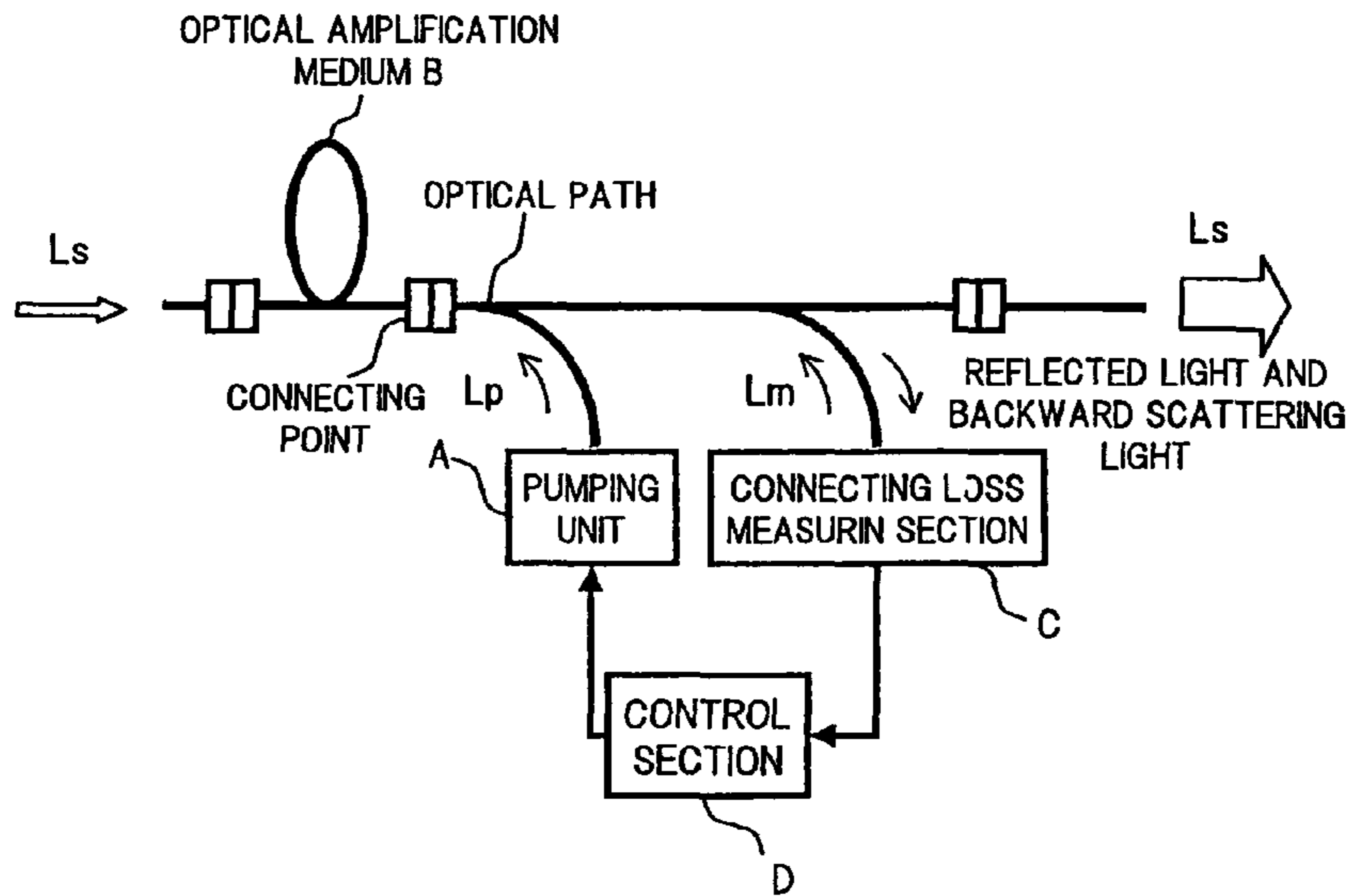
BASIC CONFIGURATION OF EMBODIMENT 3 OF PRESENT INVENTION
