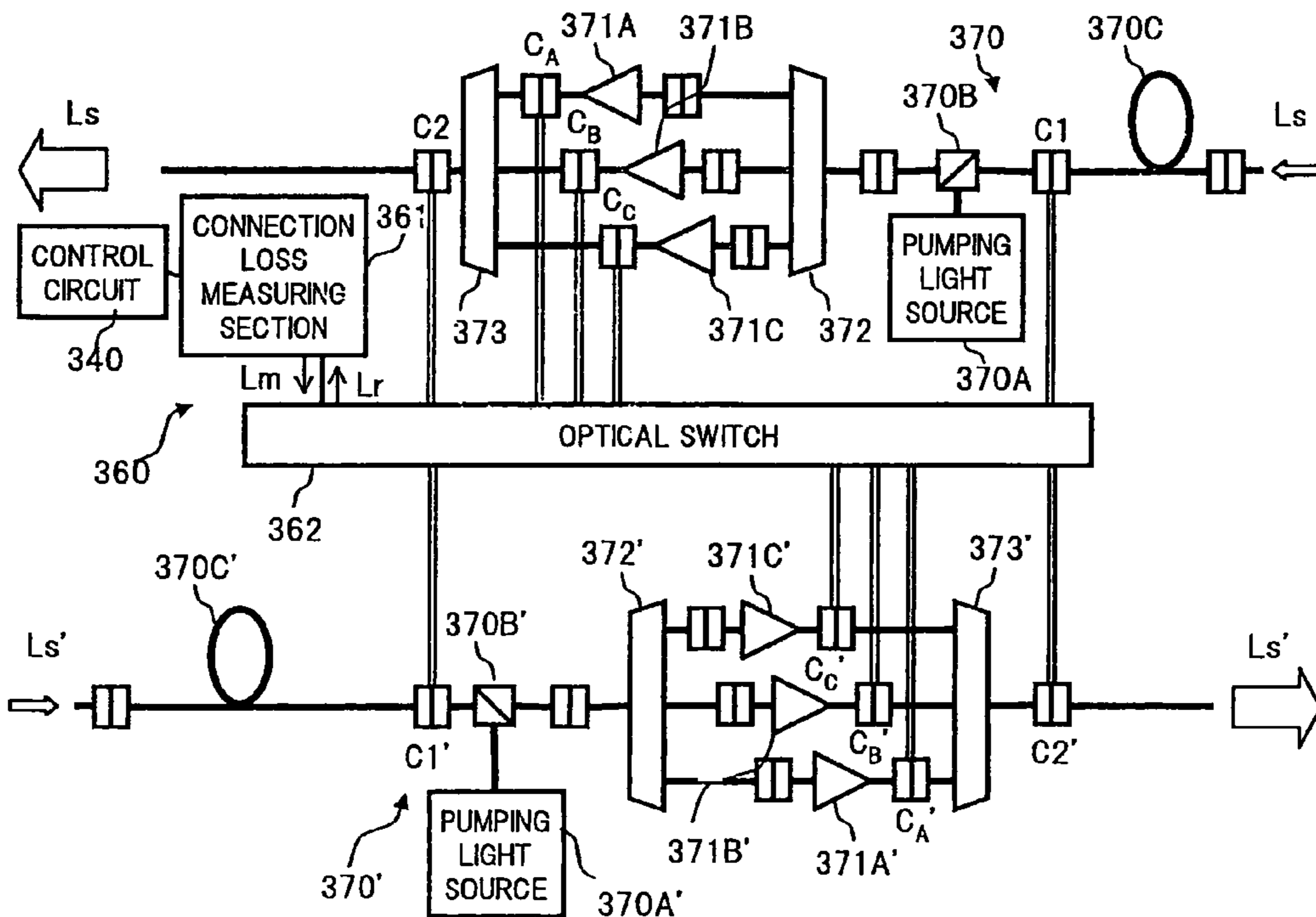
CONFIGURATION OF EMBODIMENT 3-4 OF PRESENT INVENTION
