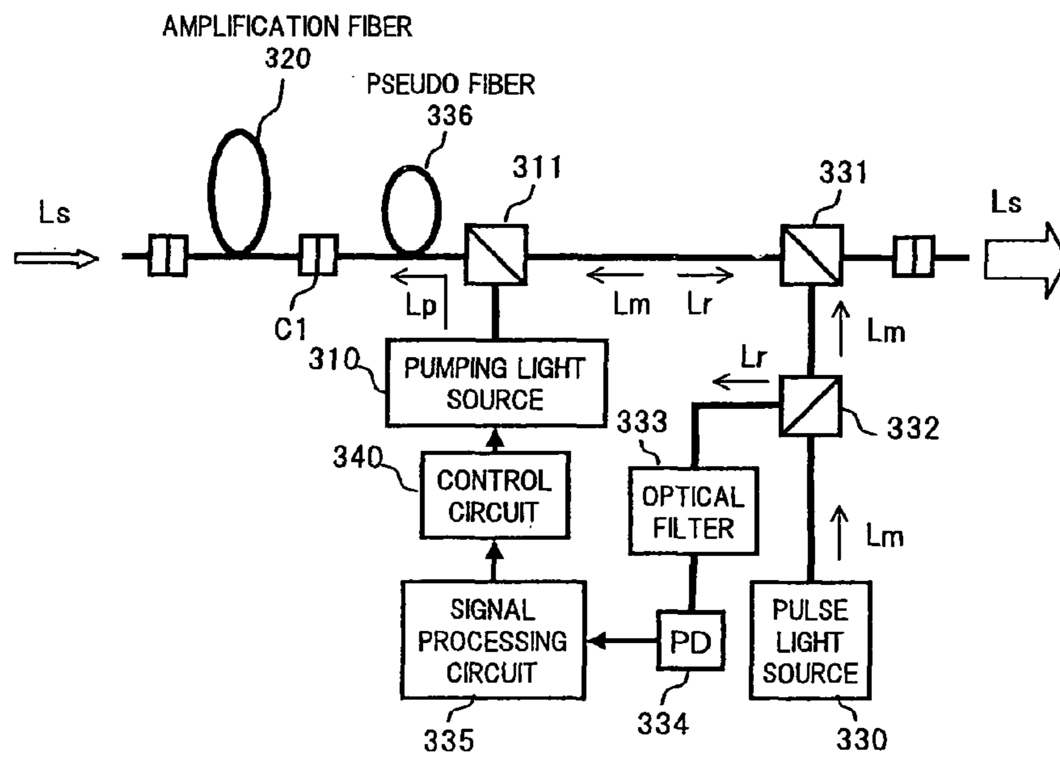
CONFIGURATION OF EMBODIMENT 3-1 OF PRESENT INVENTION
