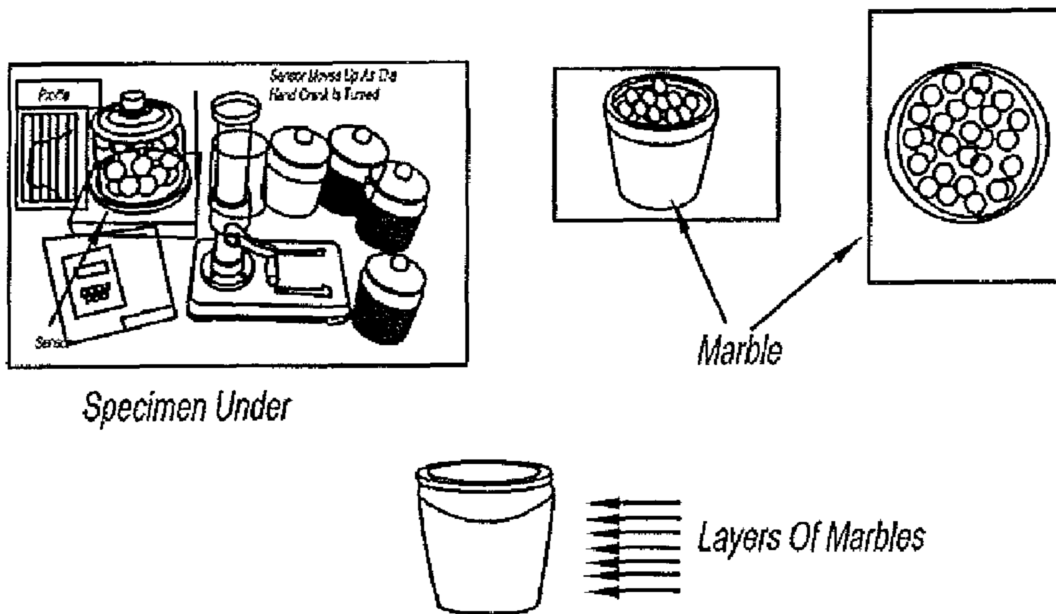
The laboratory equipment used to inspect the gelatin specimens. Each specimen is filled with a marble + gelatin + tagged material.
