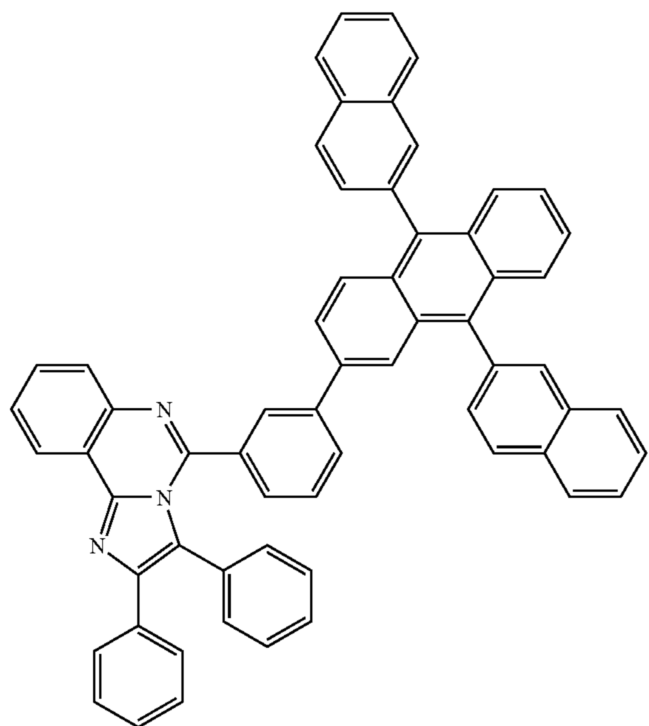
[compound 1-4-12]
