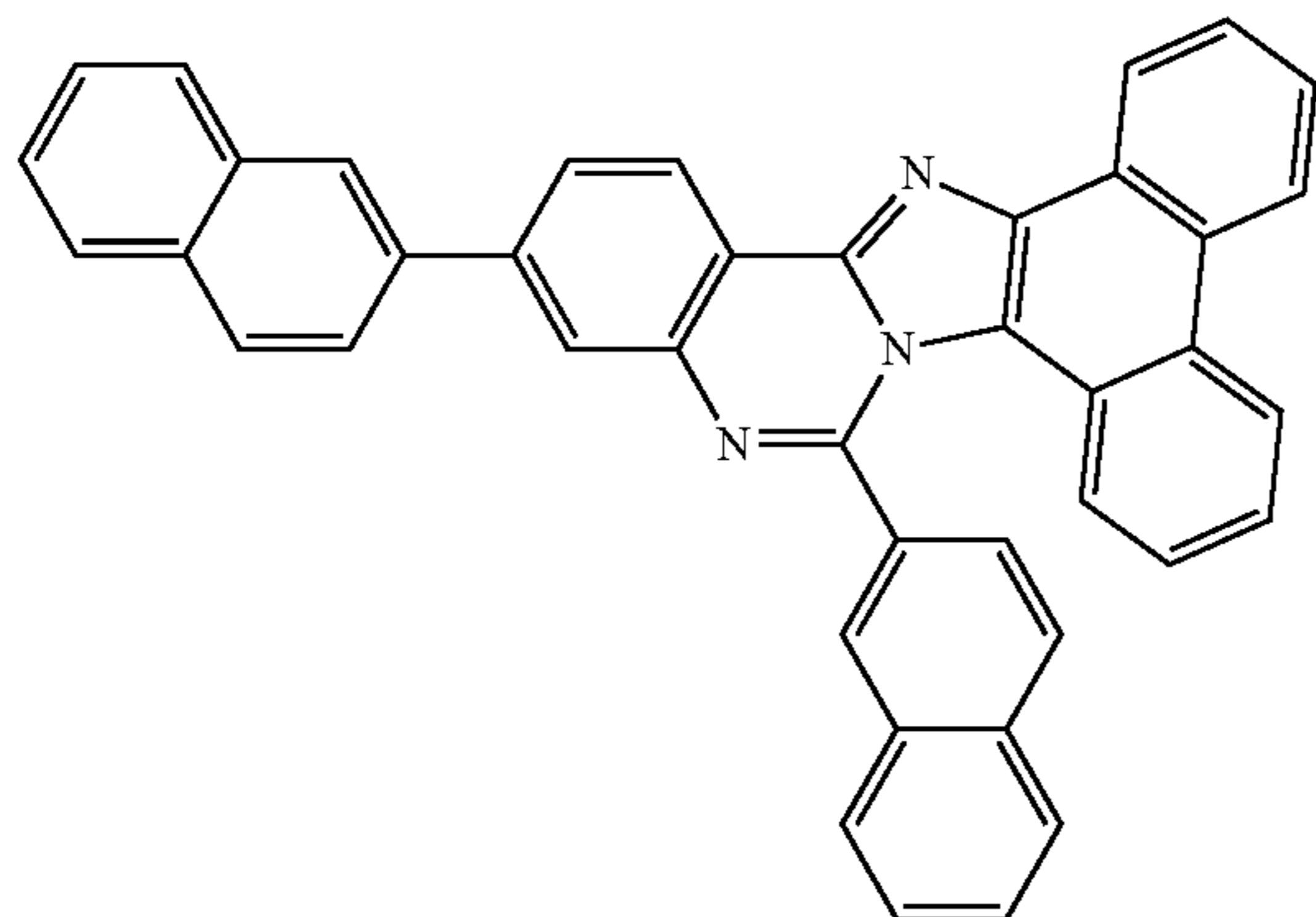
[compound 1-4-34]
