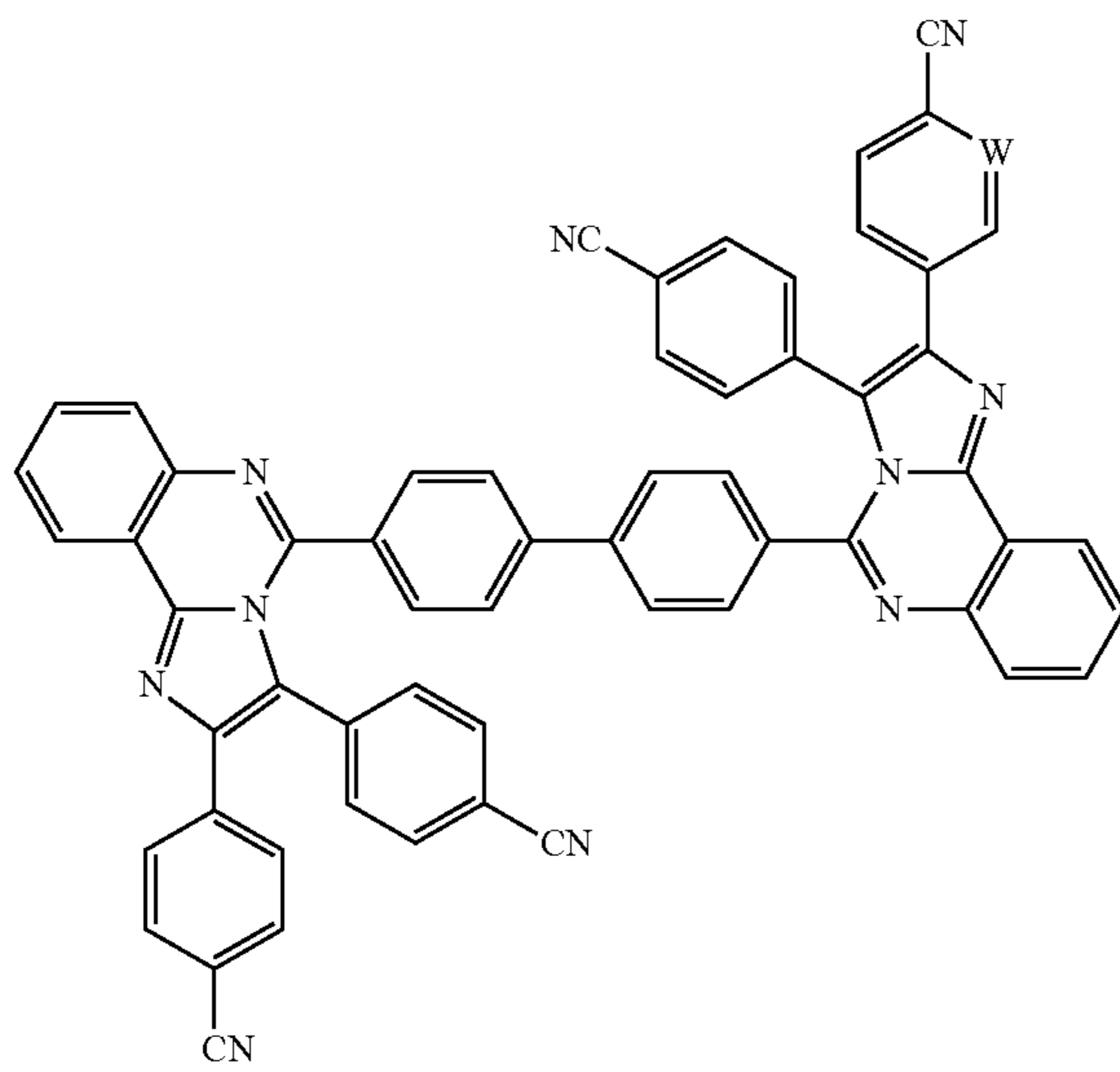
[compound 1-4-22]
