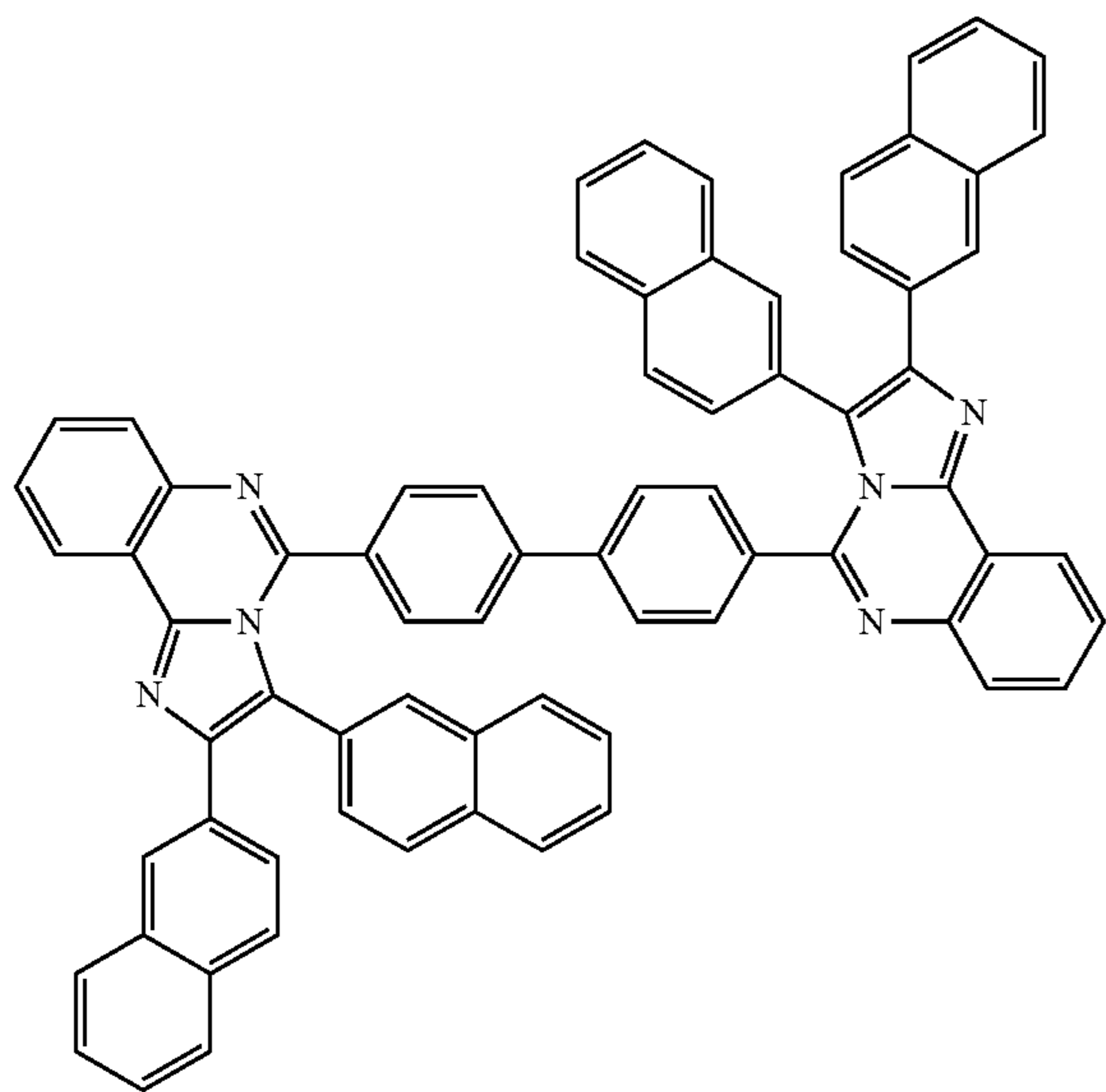
[compound 1-4-24]
