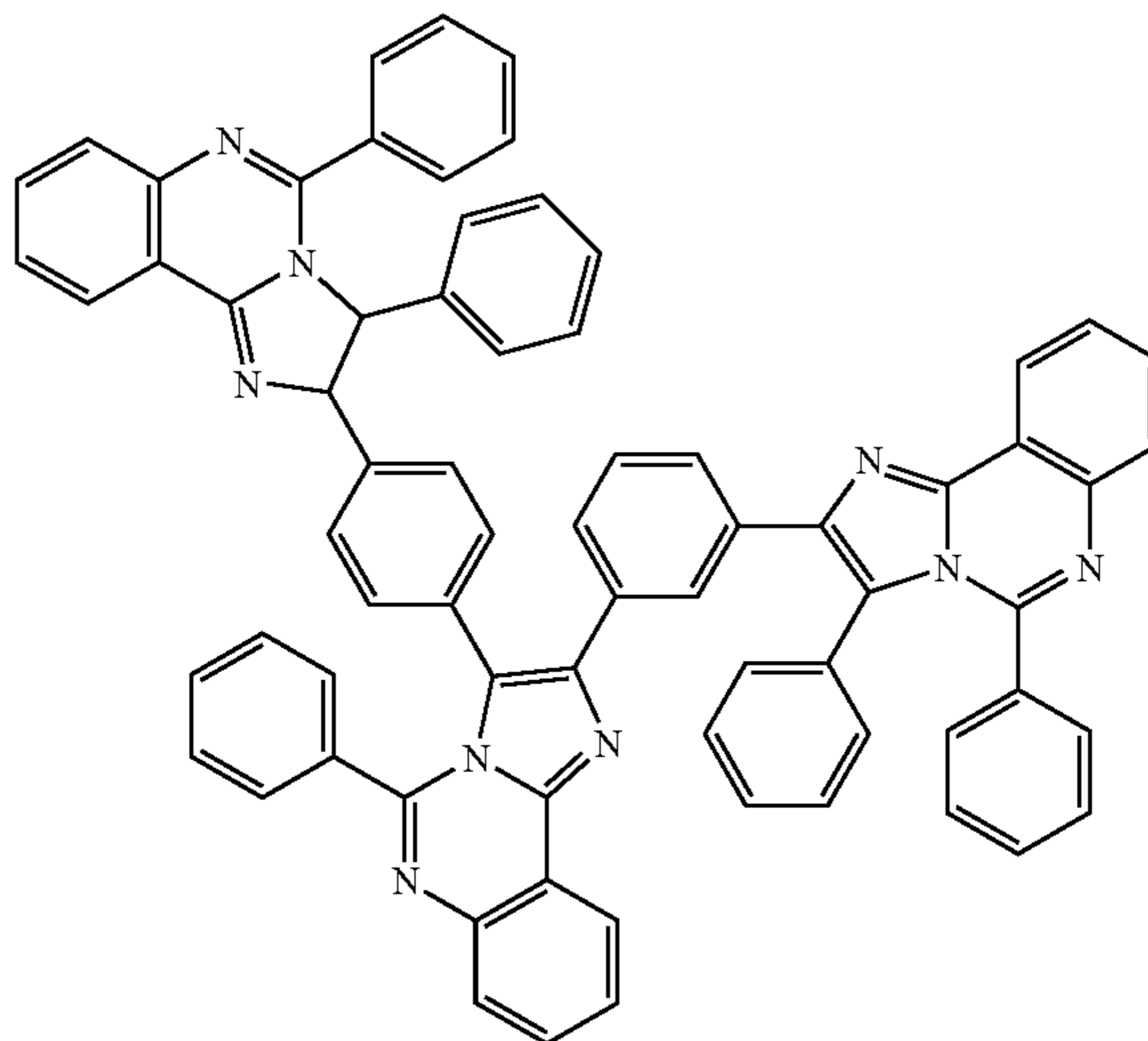
[compound 1-4-25]
