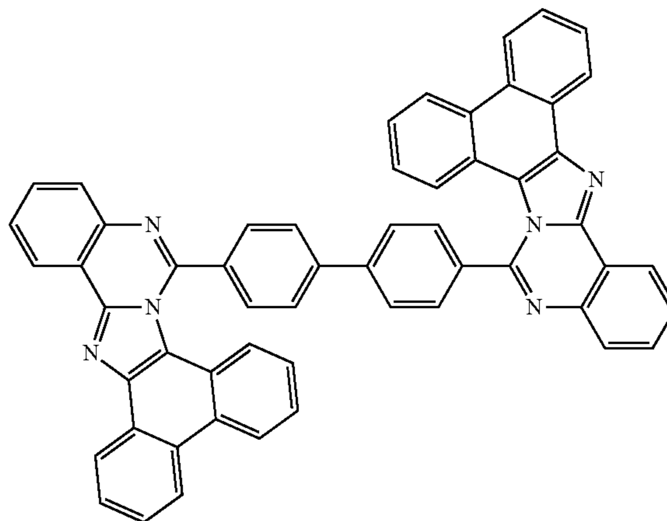
[compound 1-4-31]
