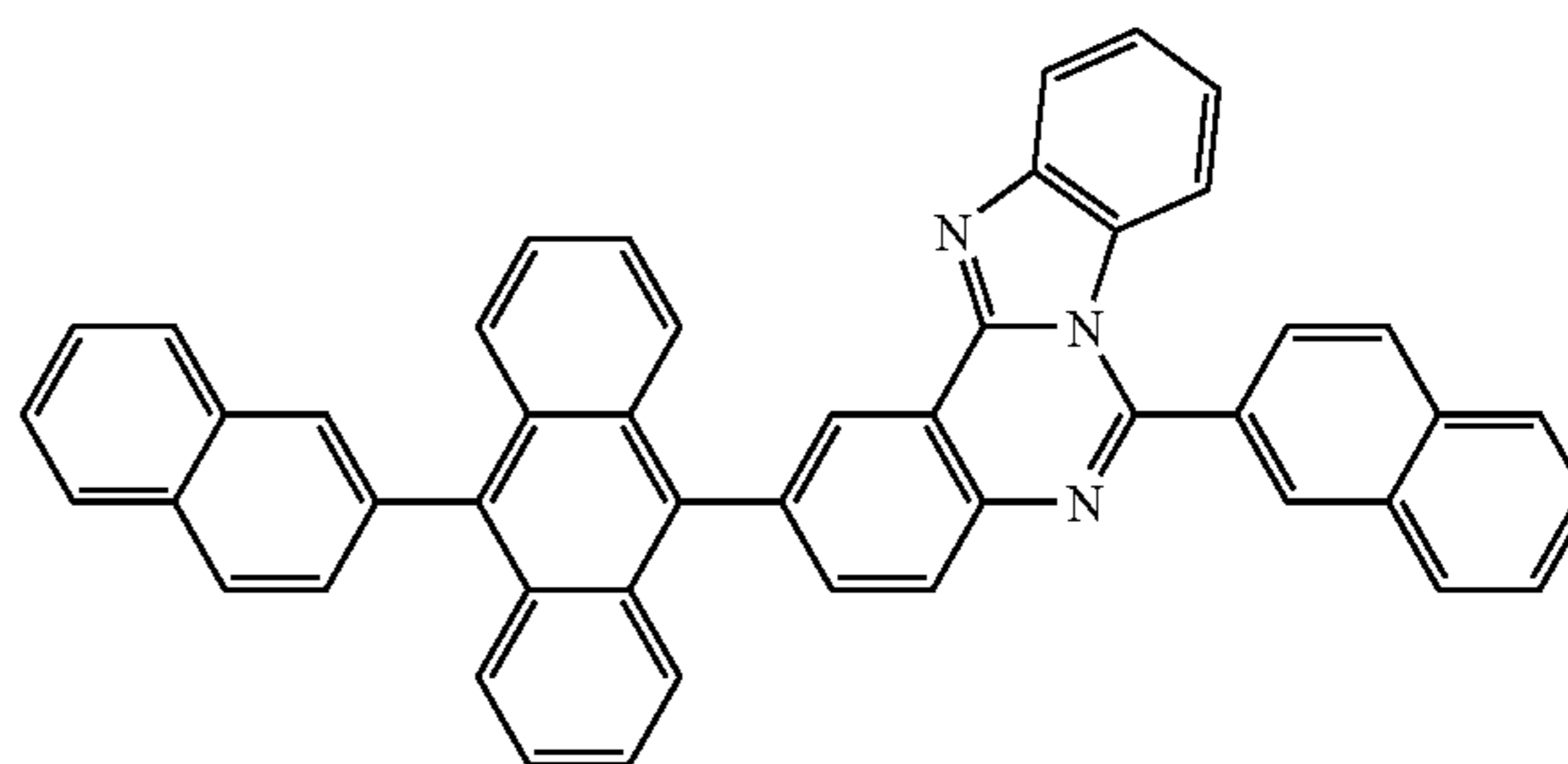
[compound 1-4-43]
