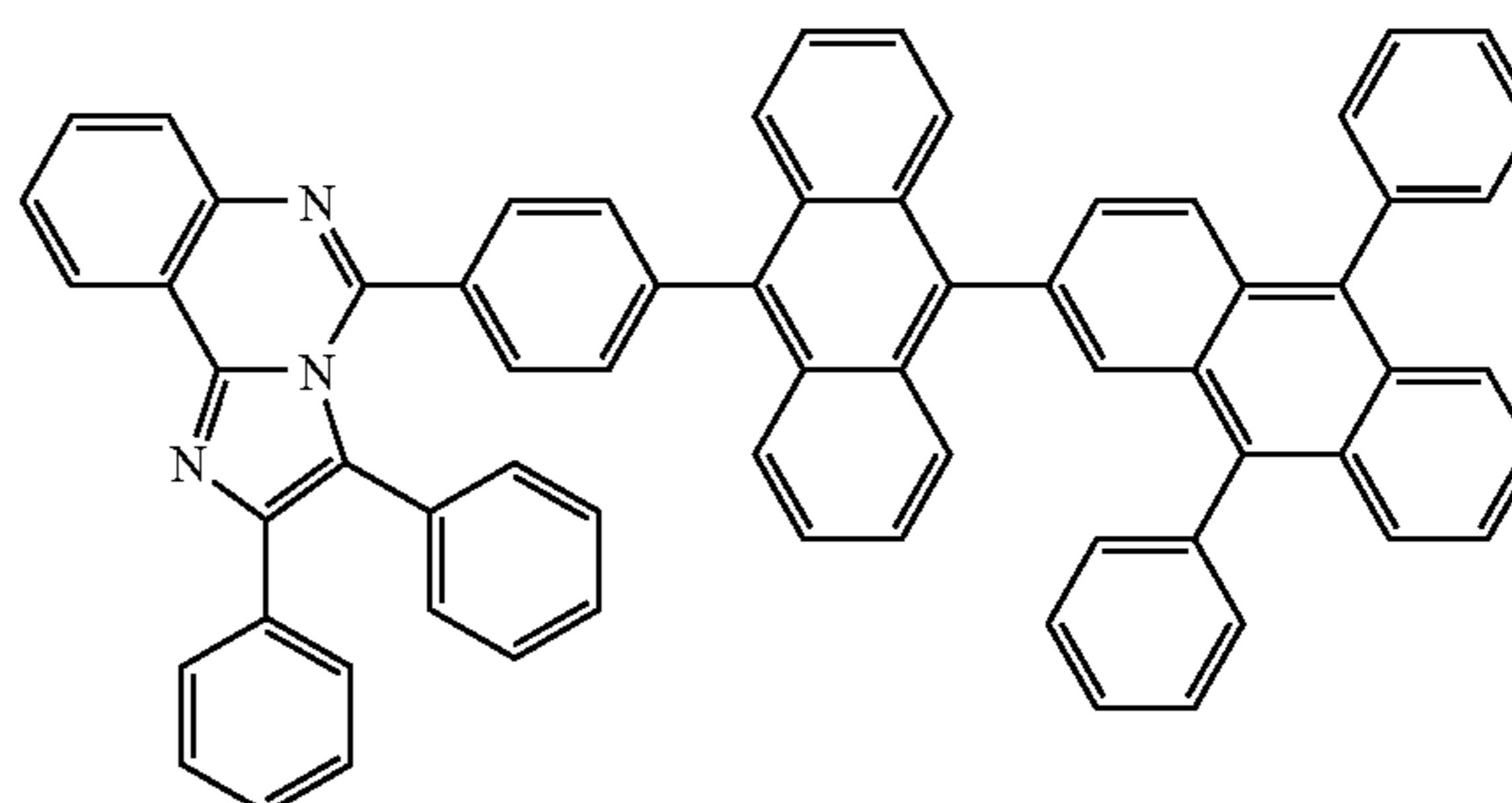
[compound 1-4-13]
