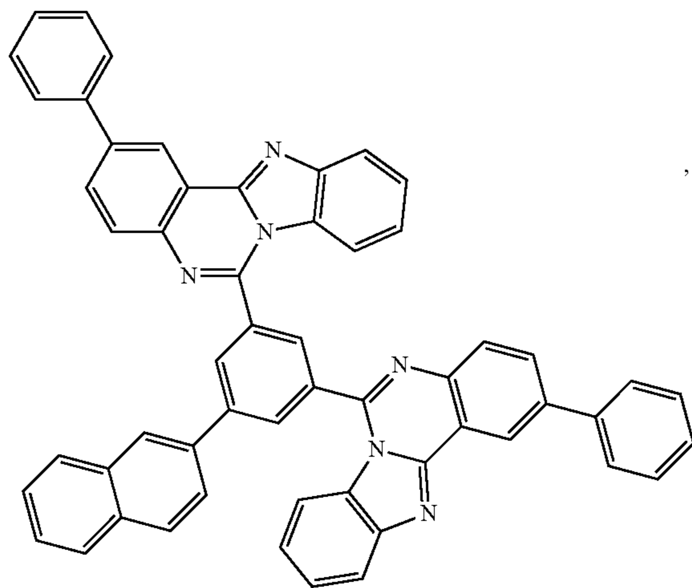
[compound 1-4-42]
