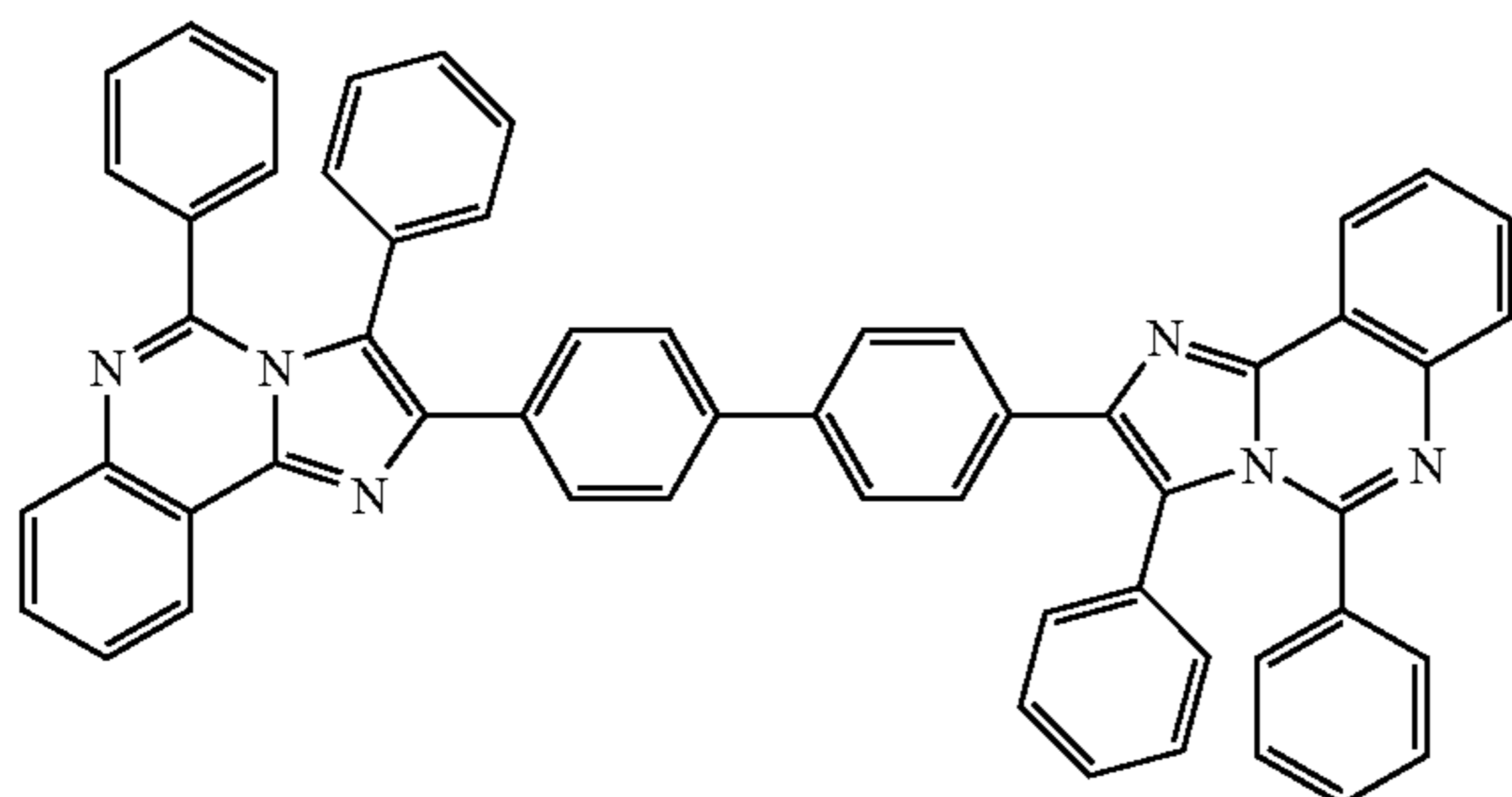
[compound 1-4-26]
