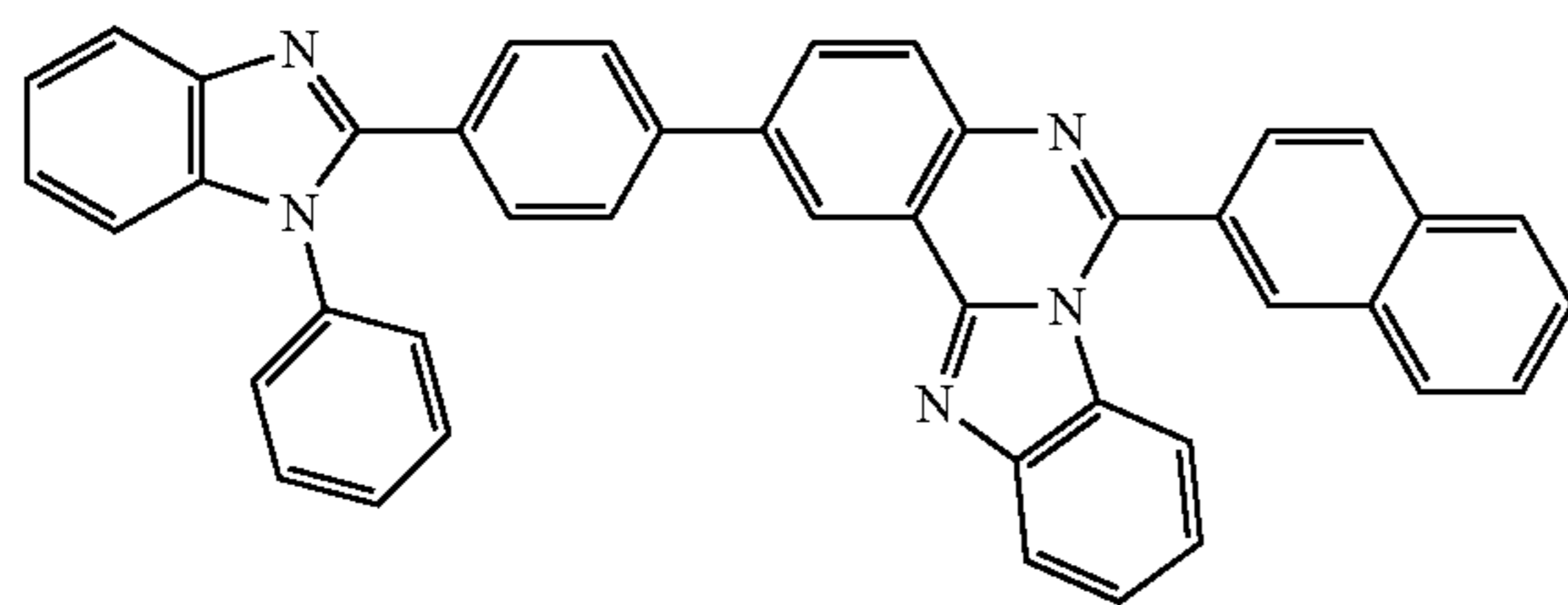
[compound 1-4-10]
