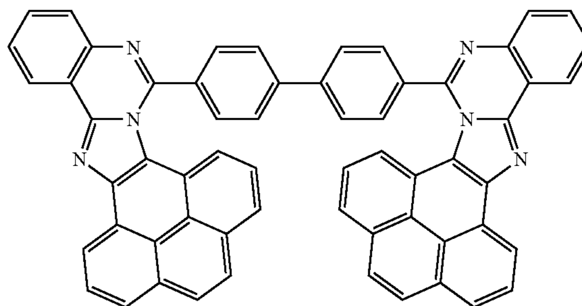
[compound 1-4-29]
