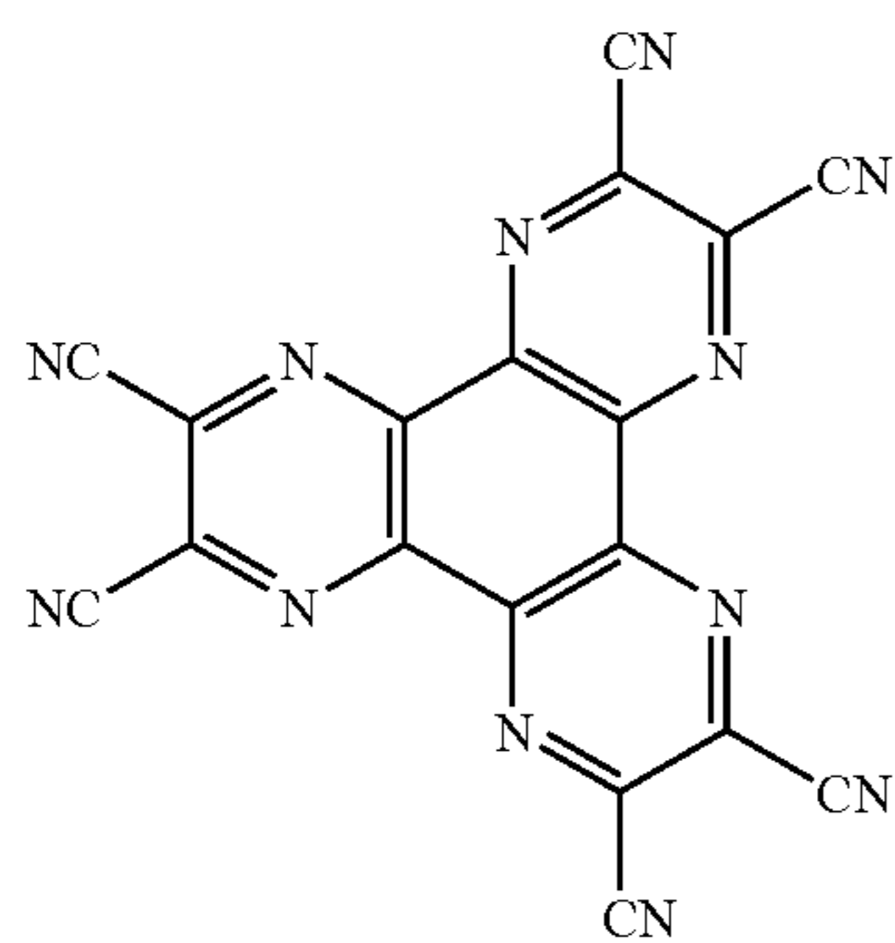
[Hexanitriple hexaazatriphenylene]
