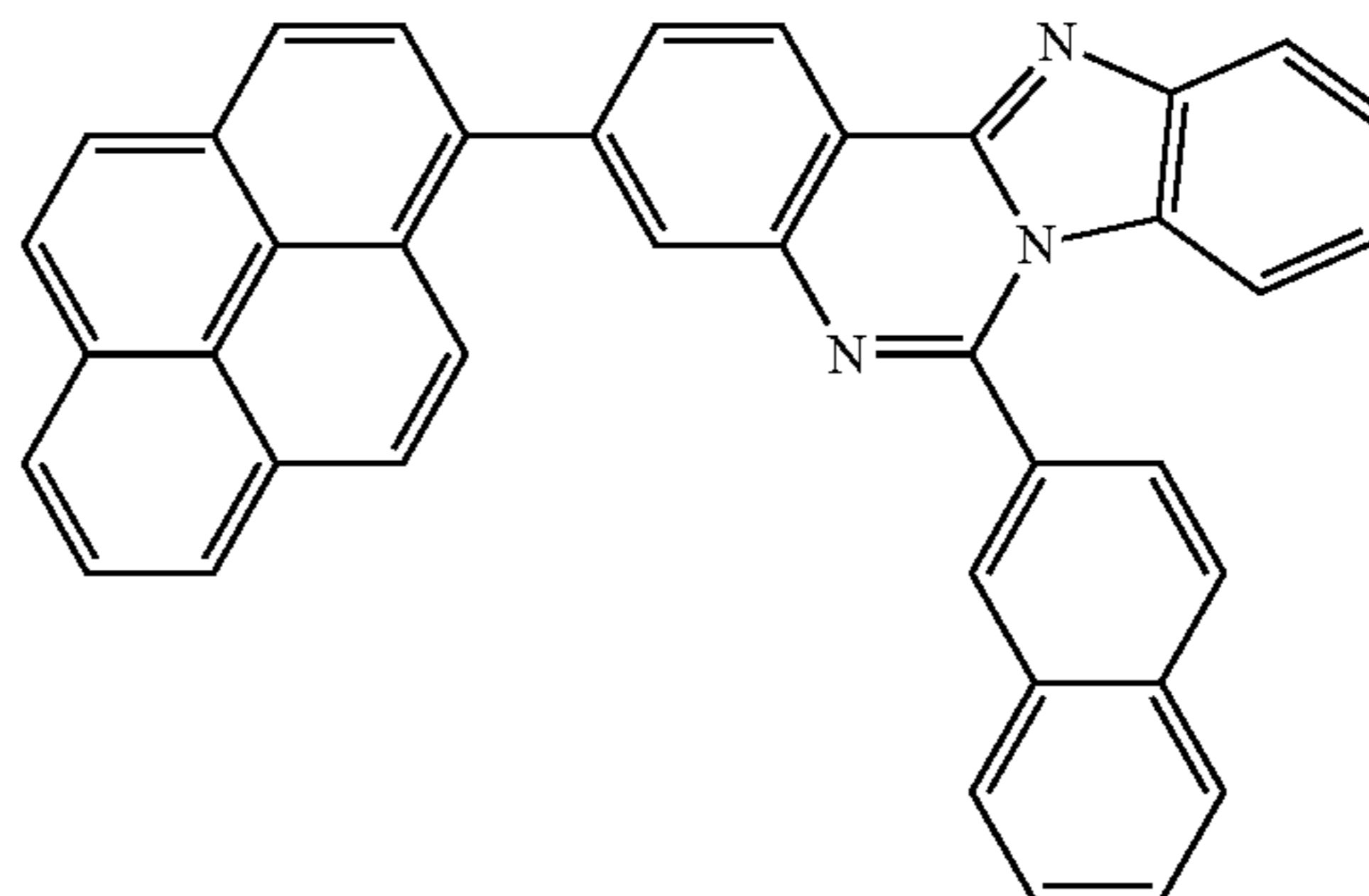
[compound 1-4-35]
