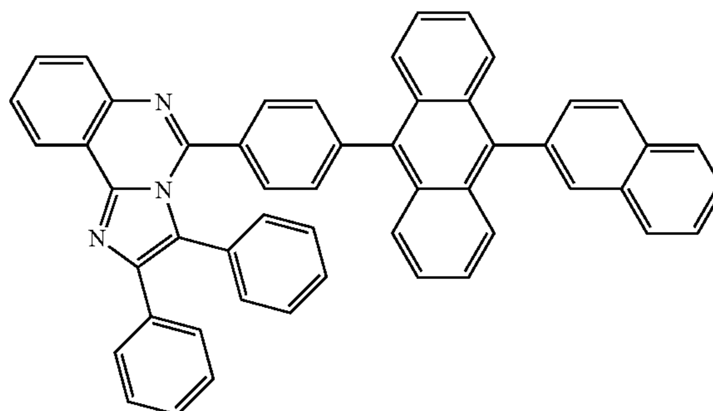
[compound 1-4-11]
