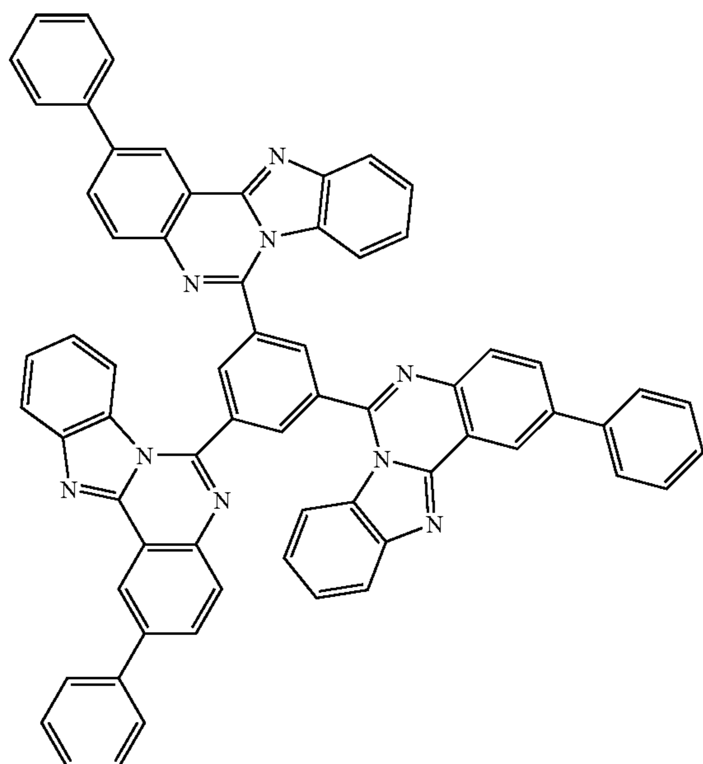
[compound 1-4-45]
