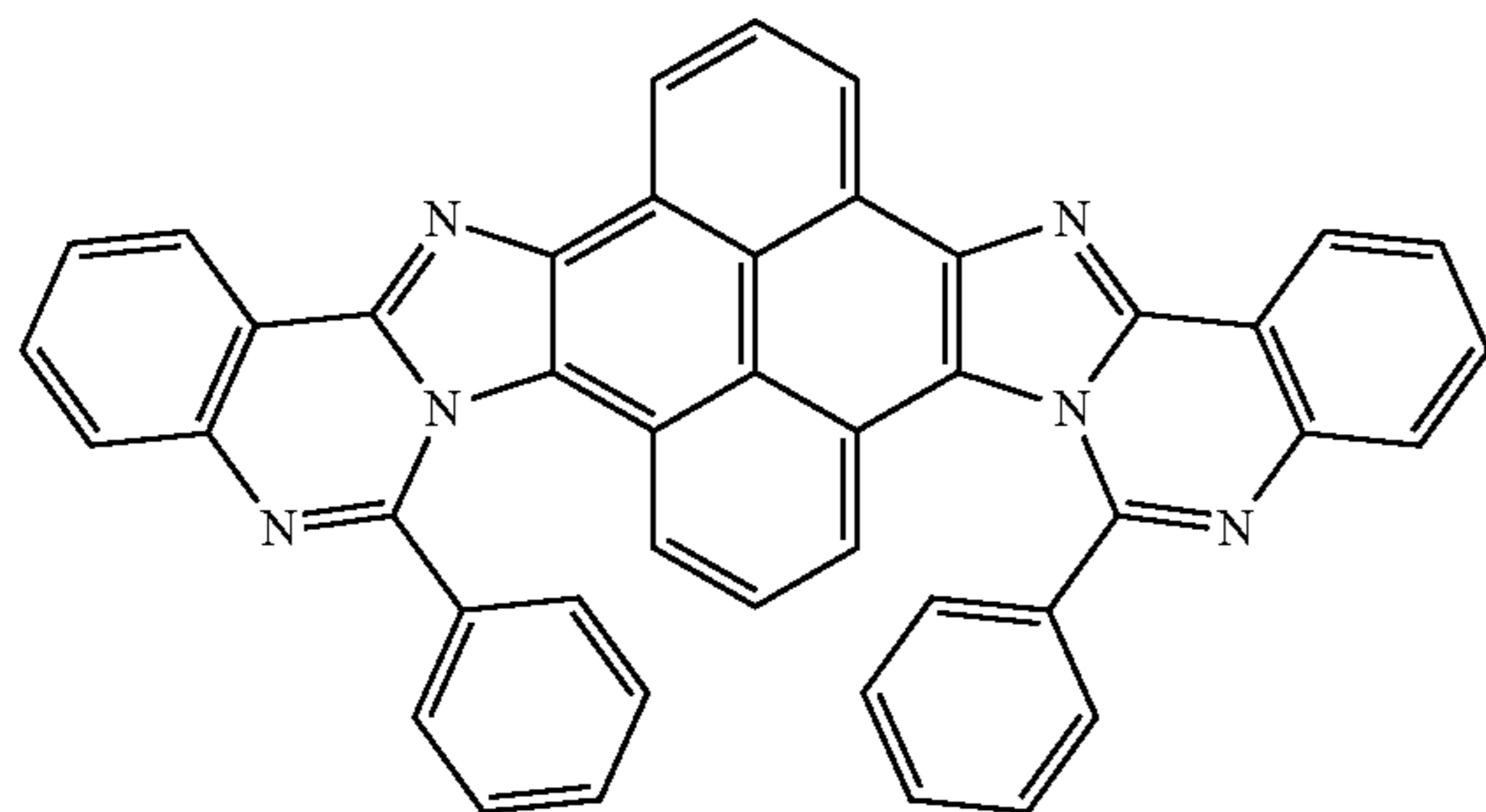
[compound 1-4-30]
