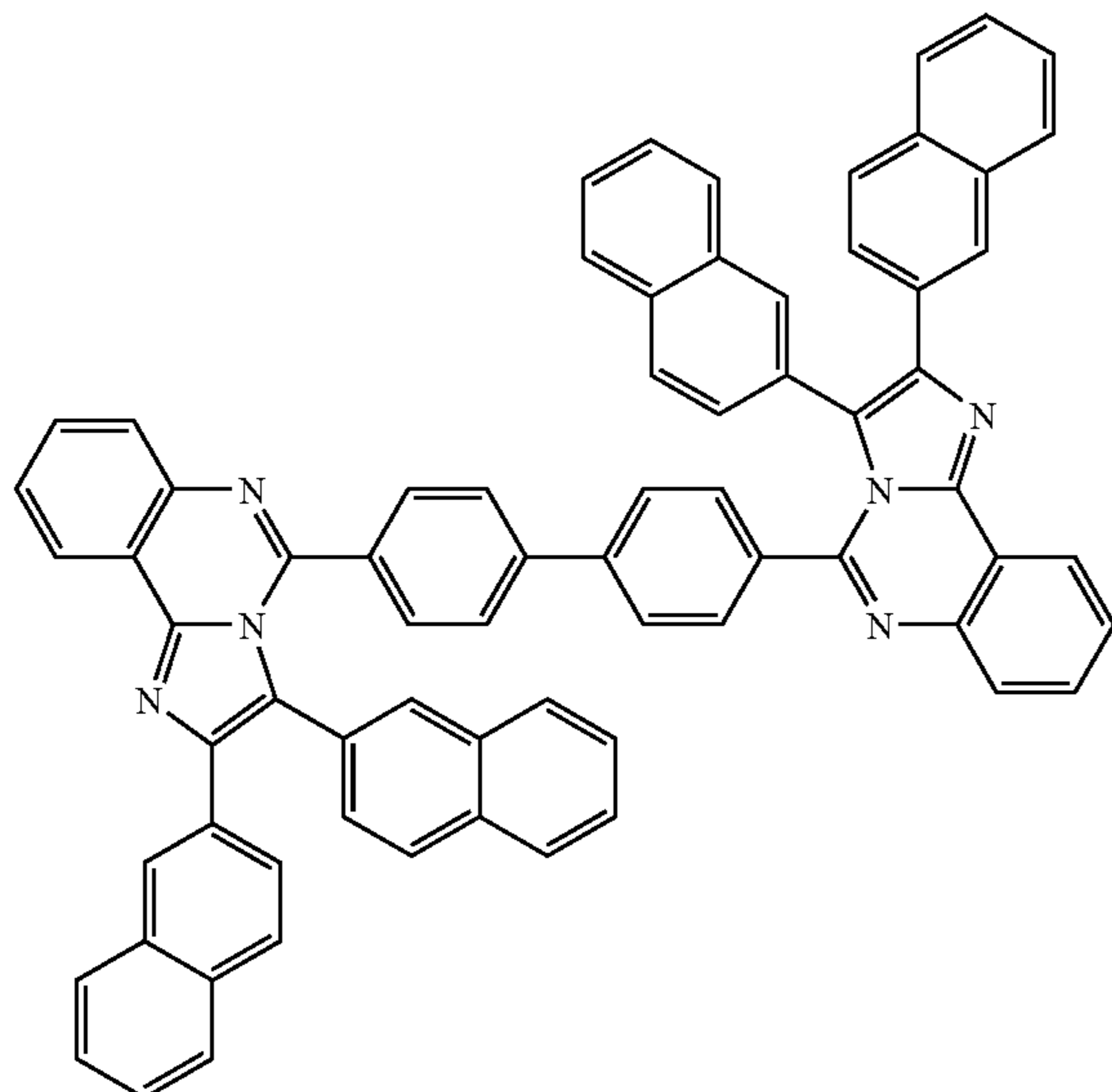
[compound 1-4-24]
