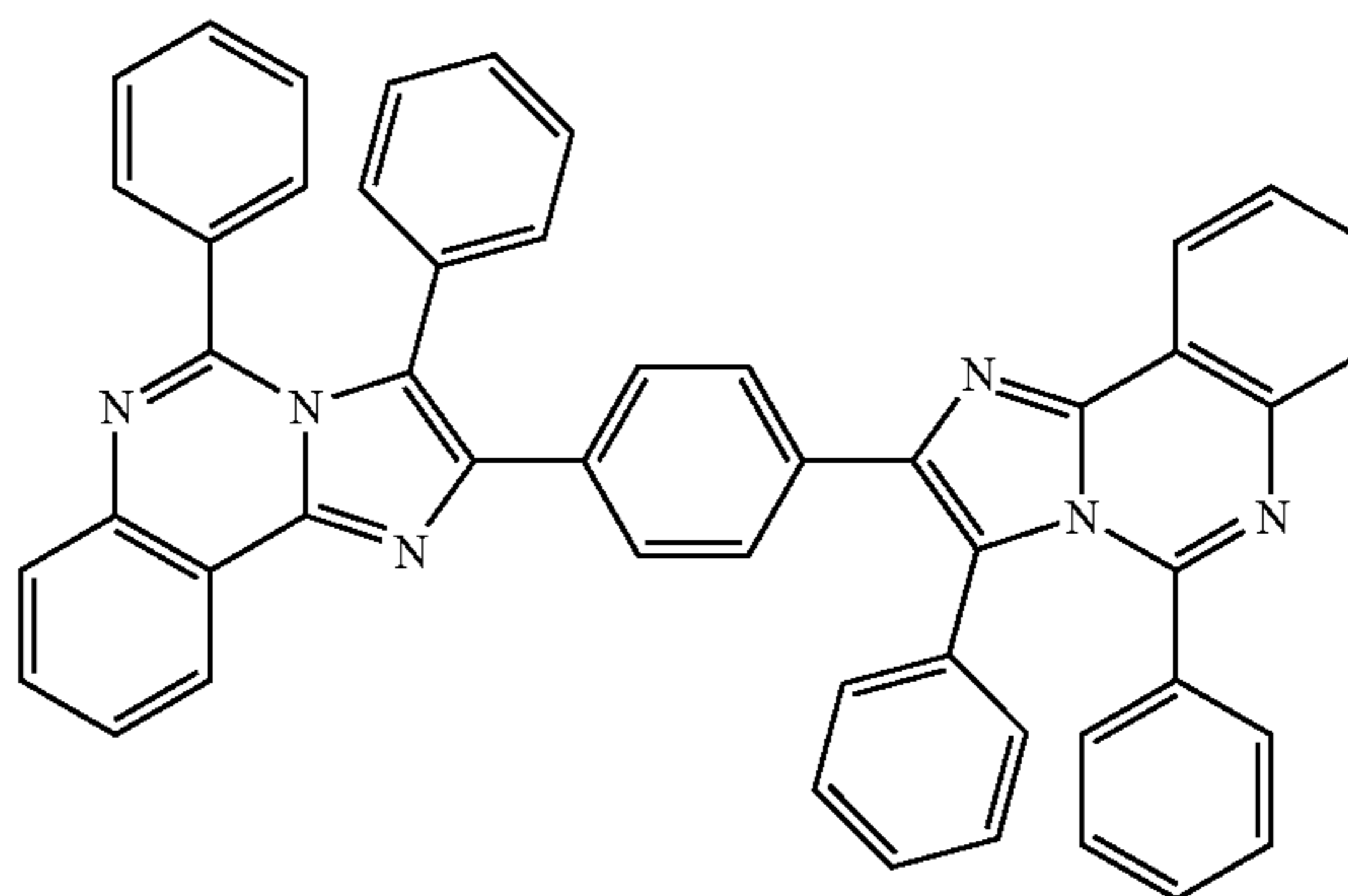
[compound 1-4-27]
