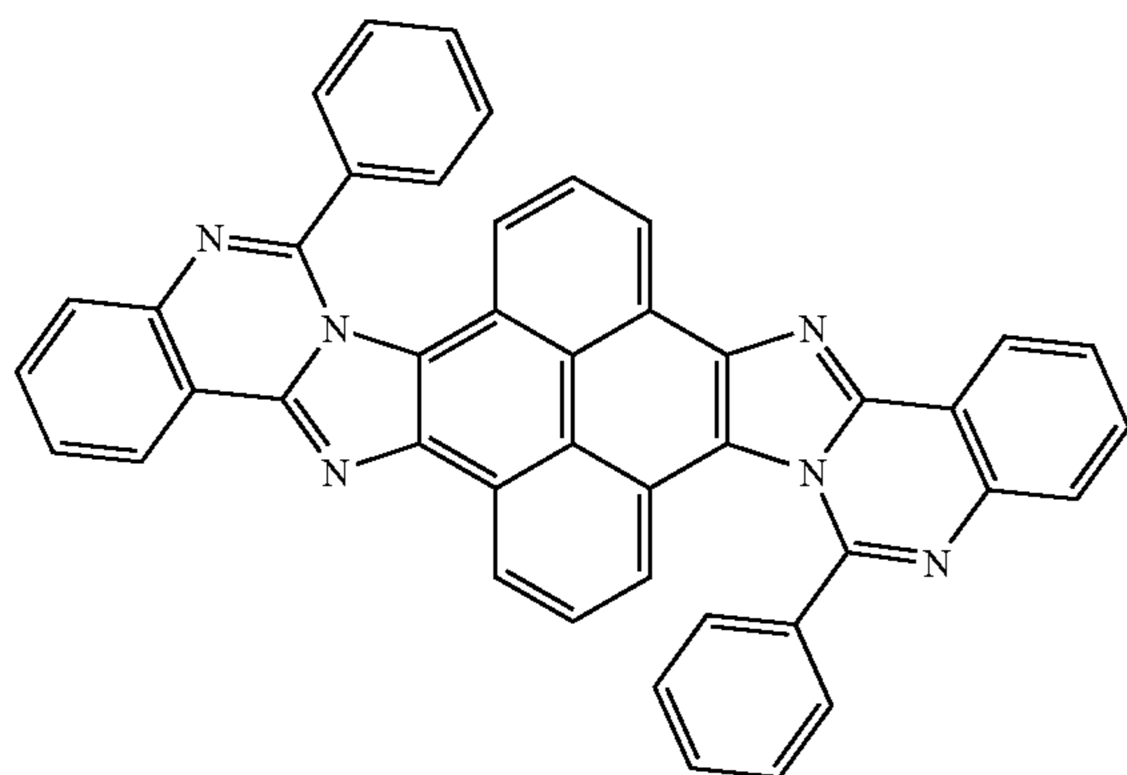
[compound 1-4-28]
