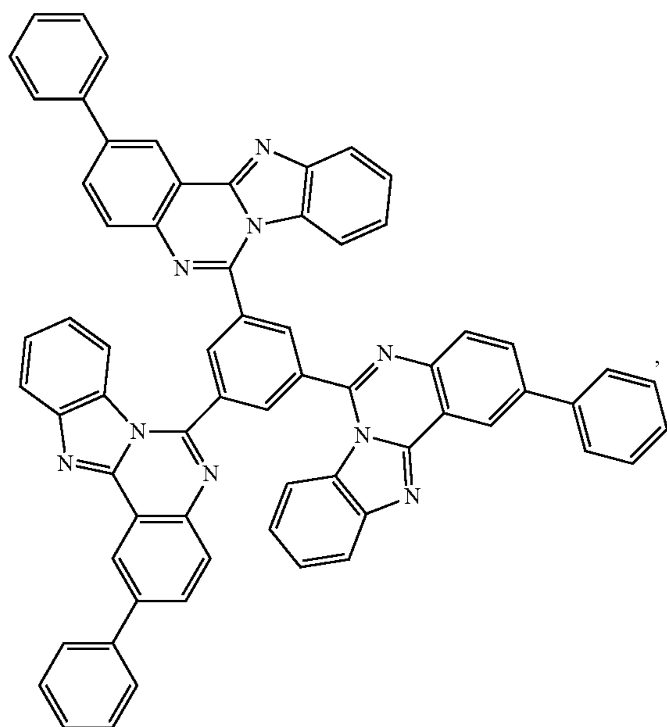
[compound 1-4-45]
