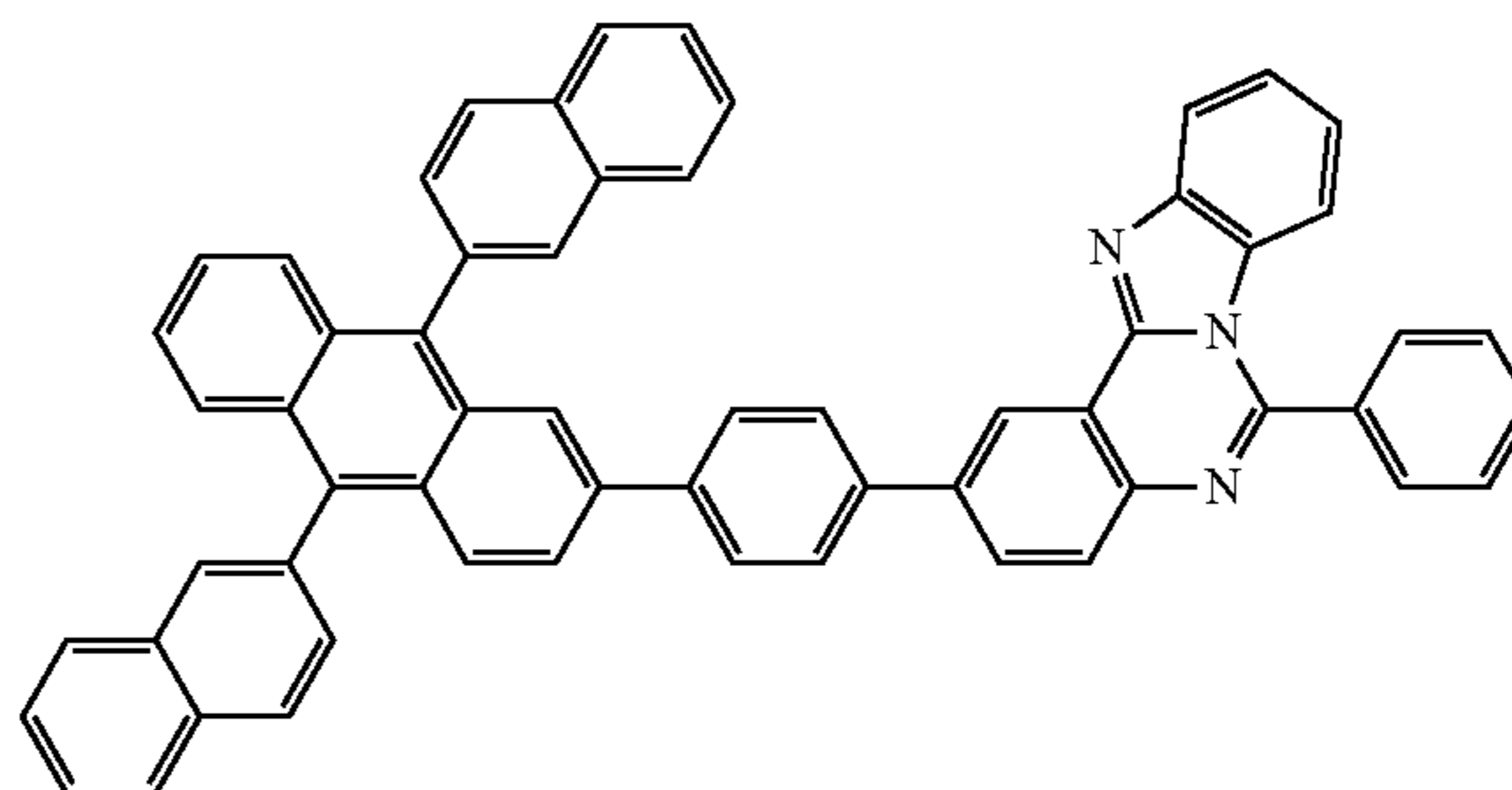
[compound 1-4-33]
