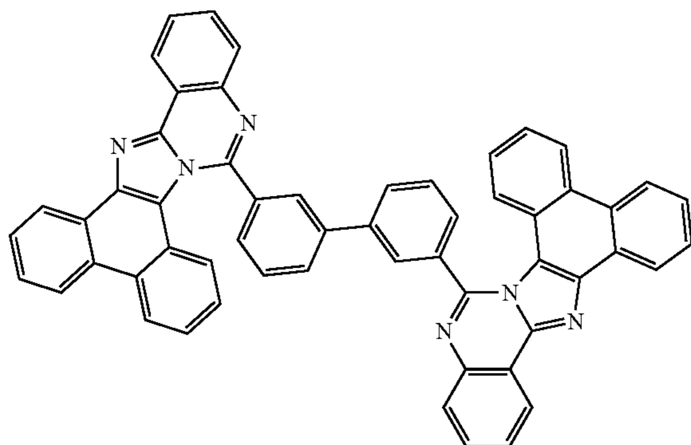
[compound 1-4-32]
