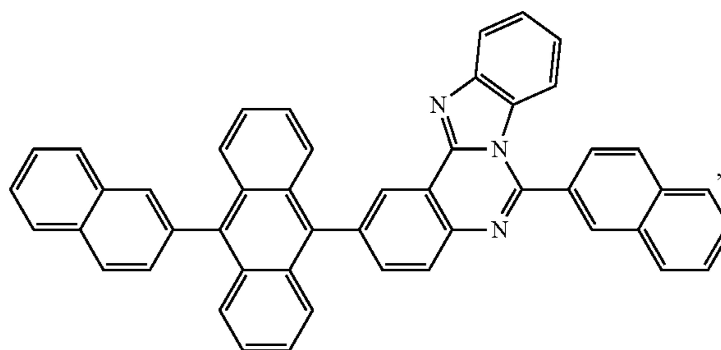
[compound 1-4-43]
