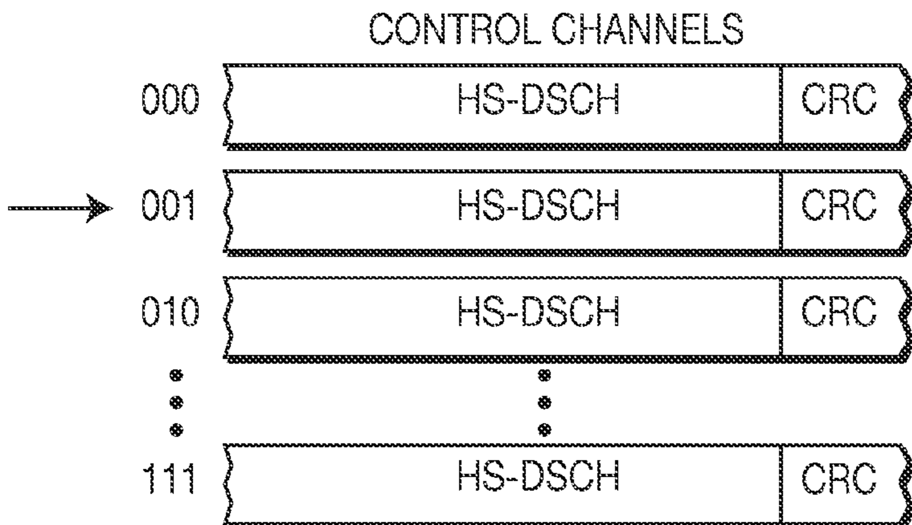
FIG. 1C PRIOR ART
